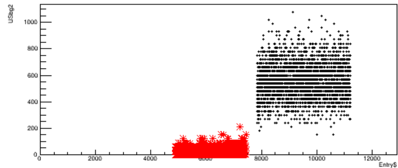
Run 5081, quartetwise: USbg2 vs time
