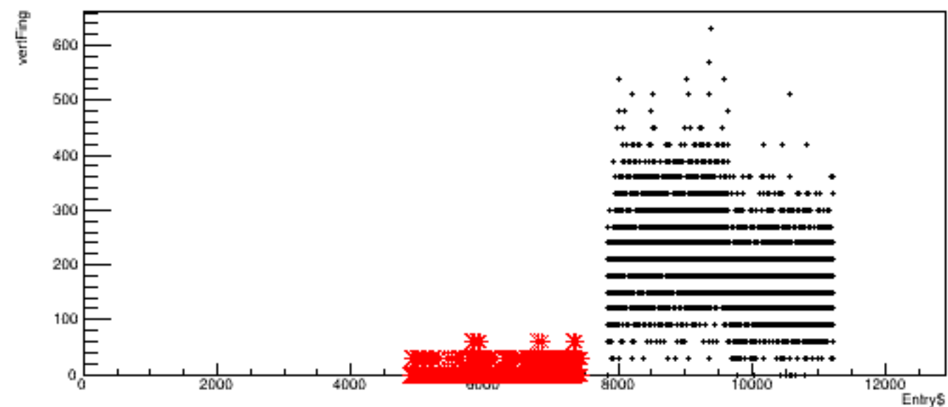
Run 5081, quartetwise: vertFing vs time
