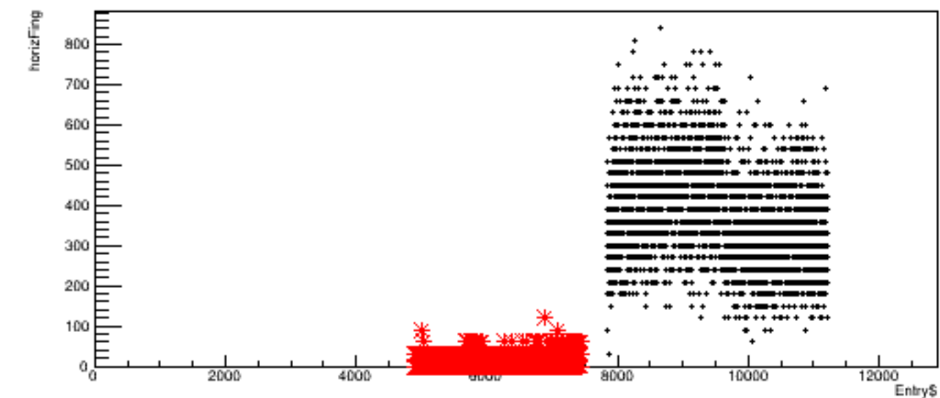
Run 5081, quartetwise: horizFing vs time
