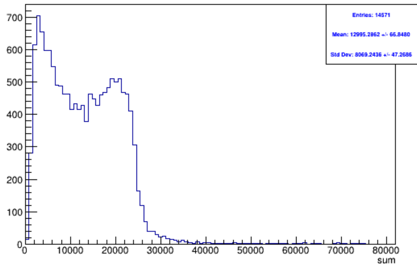
Run 5088 triggerwise, sums: All
