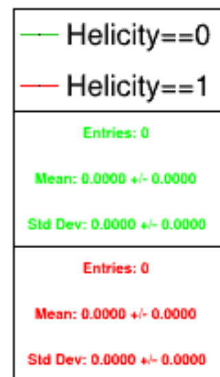
Run 5088 triggerwise, sums: Beam ON, Laser OFF
