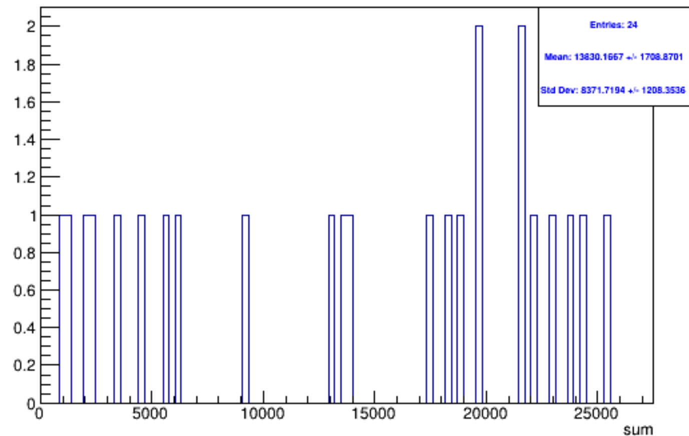
Run 5088 triggerwise, sums: Beam OFF
