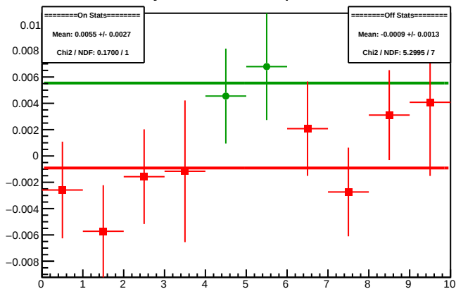
Cycle 5090.5: Multiplet Diffs
