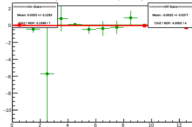
Cycle 5090.10: Multiplet Asyms
