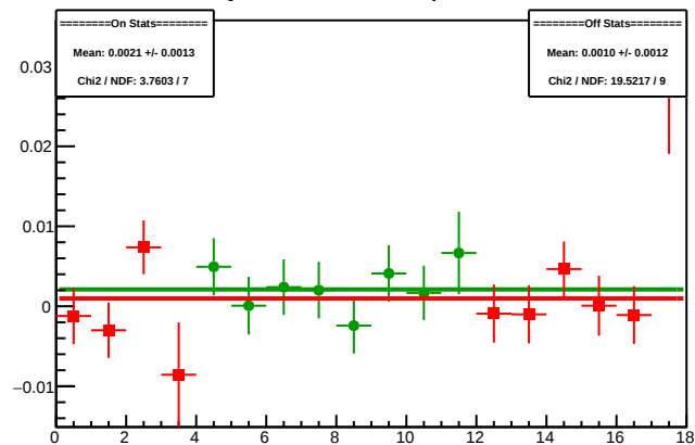
Cycle 5090.9: Multiplet Diffs
