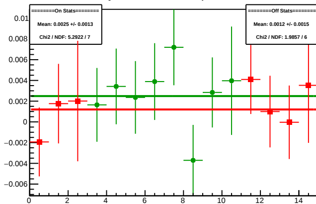
Cycle 5090.1: Multiplet Diffs
