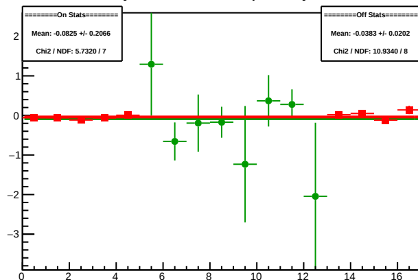
Cycle 5090.8: Multiplet Asyms
