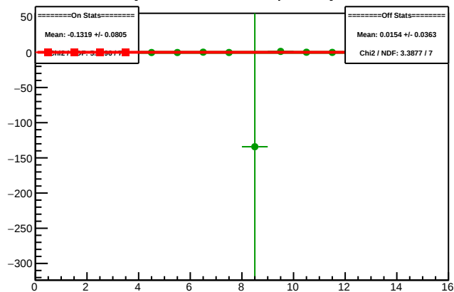
Cycle 5090.11: Multiplet Asyms
