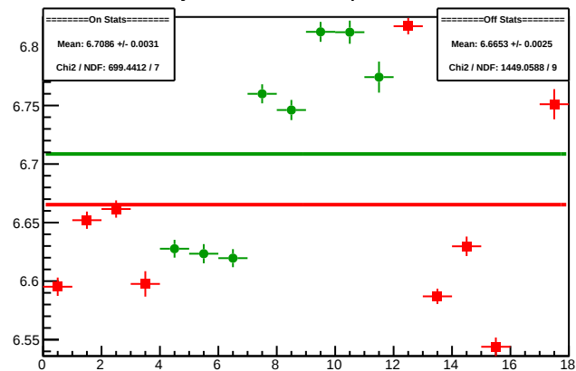
Cycle 5090.9: Multiplet Sums
