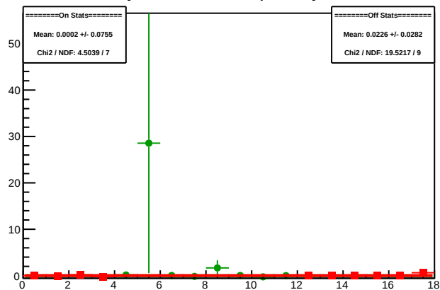
Cycle 5090.9: Multiplet Asyms
