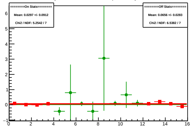
Cycle 5090.2: Multiplet Asyms
