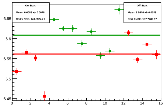
Cycle 5090.2: Multiplet Sums
