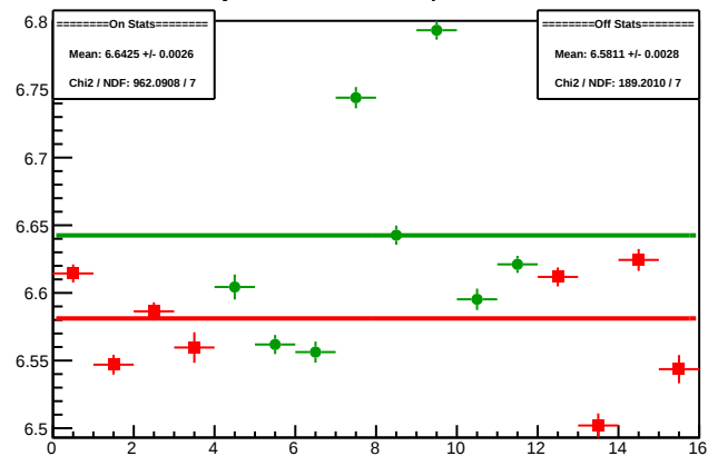
Cycle 5090.3: Multiplet Sums
