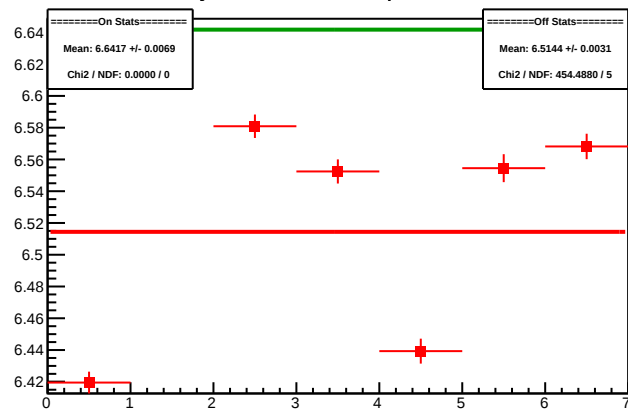
Cycle 5090.7: Multiplet Sums
