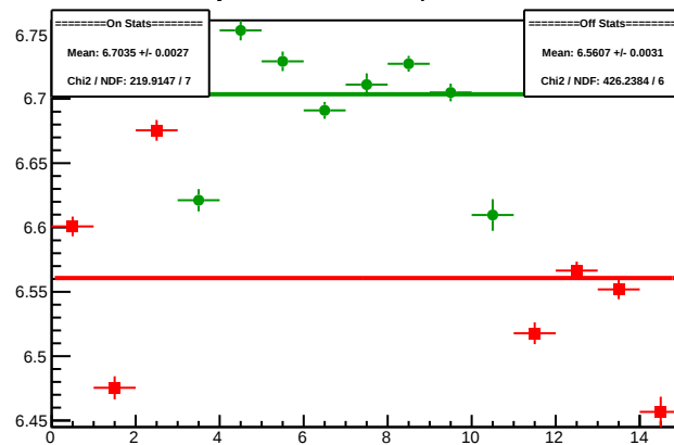
Cycle 5090.1: Multiplet Sums
