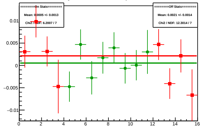
Cycle 5090.3: Multiplet Diffs
