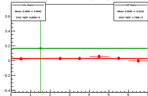
Cycle 5090.7: Multiplet Asyms
