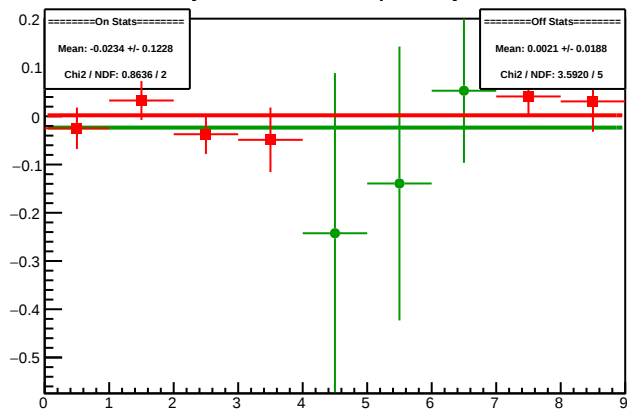
Cycle 5090.6: Multiplet Asyms
