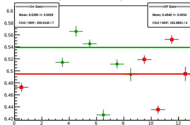
Cycle 5090.10: Multiplet Sums
