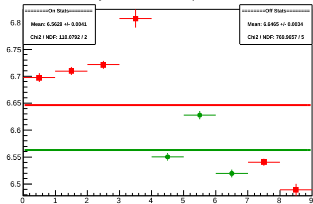
Cycle 5090.6: Multiplet Sums
