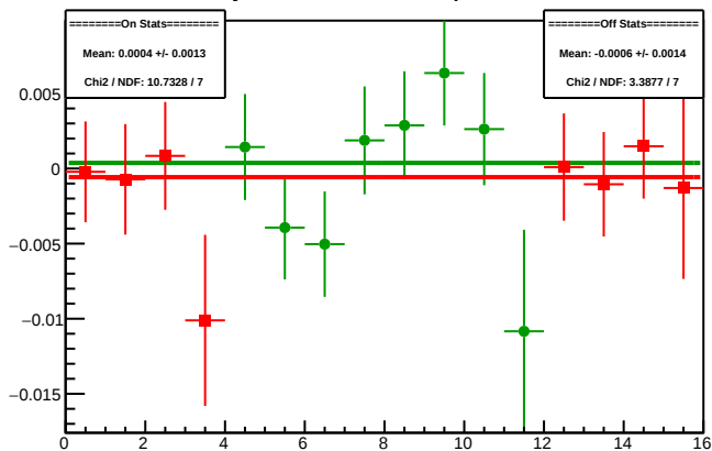
Cycle 5090.11: Multiplet Diffs
