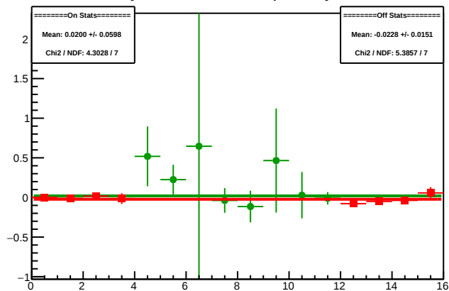
Cycle 5090.12: Multiplet Asyms
