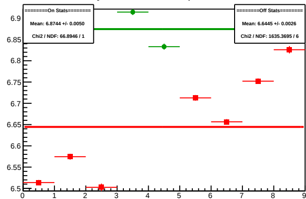
Cycle 5090.4: Multiplet Sums
