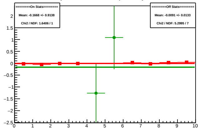
Cycle 5090.5: Multiplet Asyms
