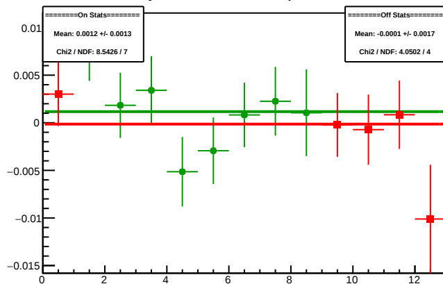
Cycle 5090.10: Multiplet Diffs
