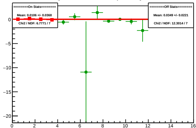
Cycle 5090.3: Multiplet Asyms
