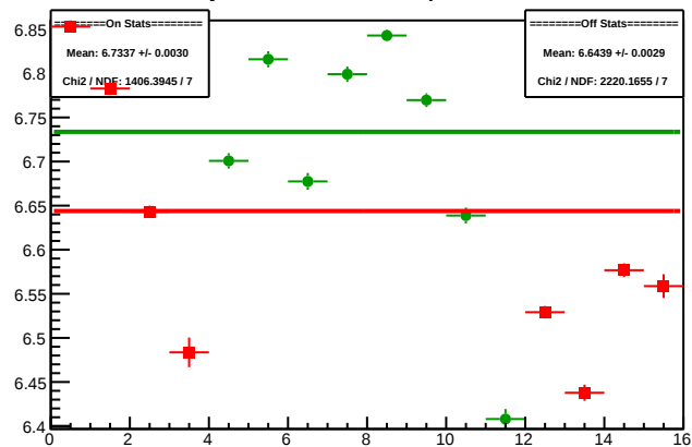
Cycle 5090.12: Multiplet Sums
