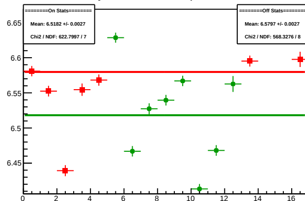
Cycle 5090.8: Multiplet Sums
