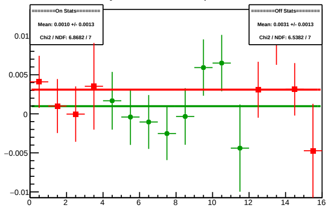
Cycle 5090.2: Multiplet Diffs
