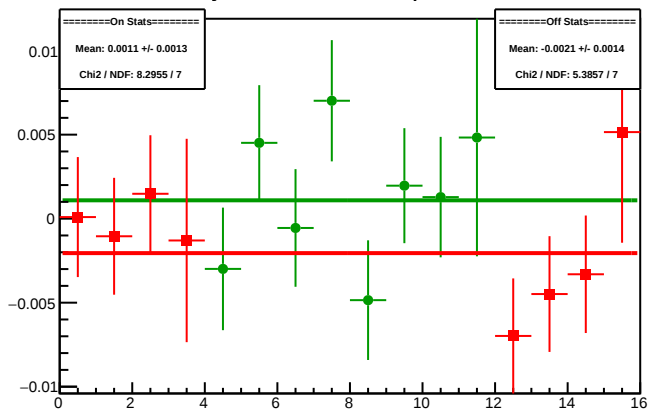
Cycle 5090.12: Multiplet Diffs
