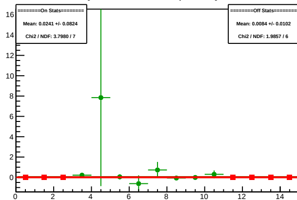
Cycle 5090.1: Multiplet Asyms
