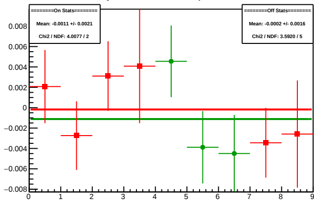
Cycle 5090.6: Multiplet Diffs
