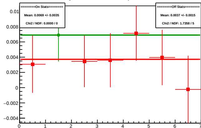
Cycle 5090.7: Multiplet Diffs
