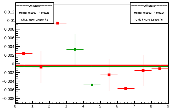
Cycle 5090.4: Multiplet Diffs
