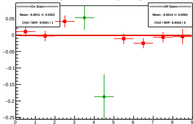
Cycle 5090.4: Multiplet Asyms
