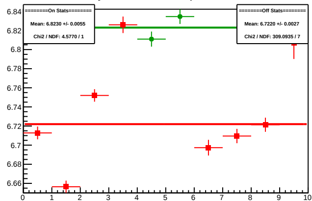
Cycle 5090.5: Multiplet Sums
