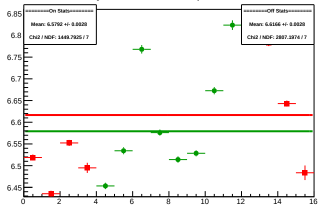
Cycle 5090.11: Multiplet Sums
