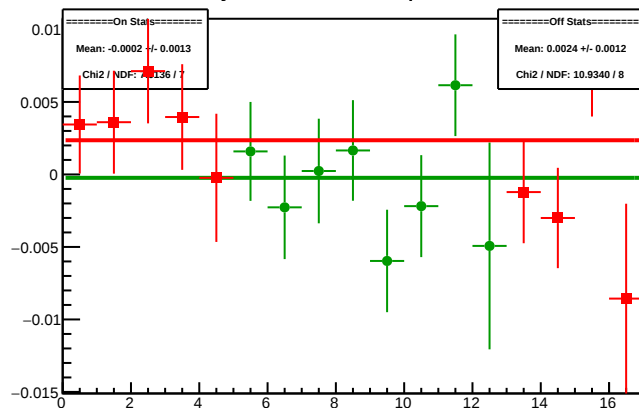
Cycle 5090.8: Multiplet Diffs
