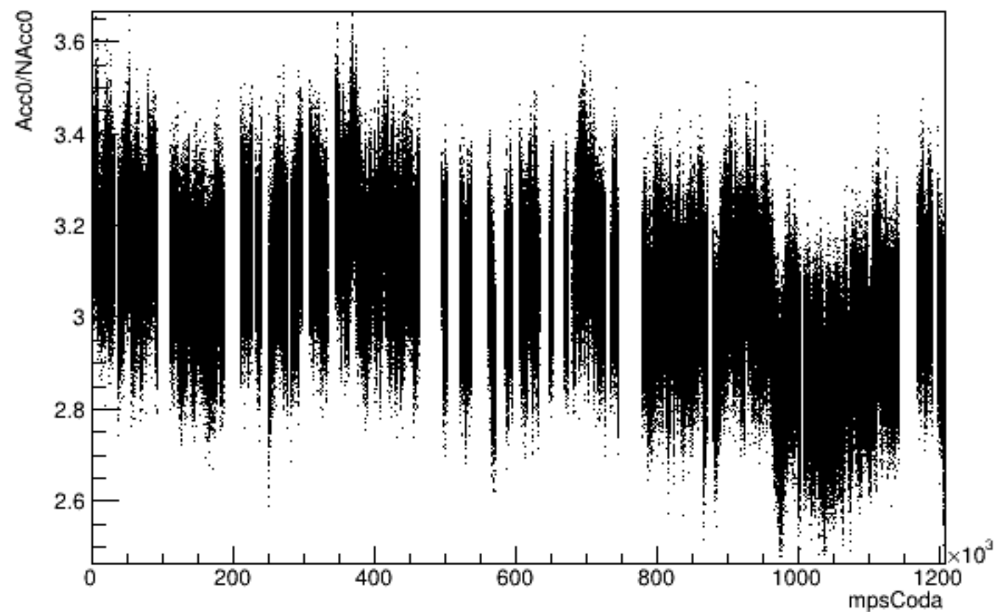
Run 5091 mpwise, Acc0 vs Time: All
