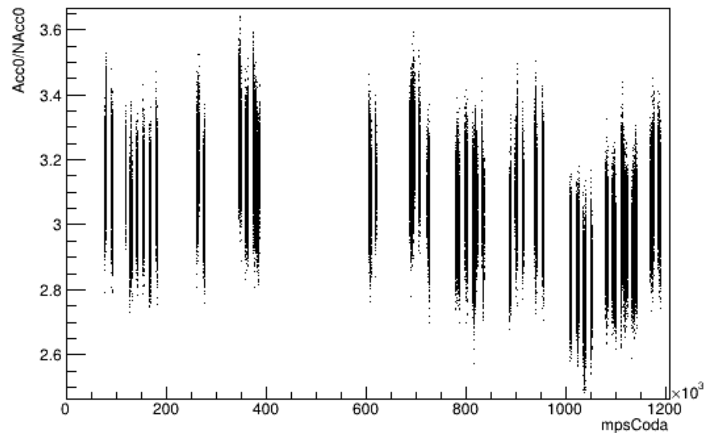
Run 5091 mpwise, Acc0 vs Time: Beam ON, Laser OFF
