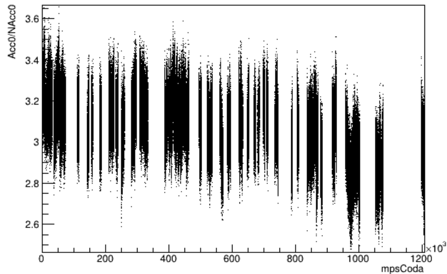
Run 5091 mpwise, Acc0 vs Time: Beam OFF
