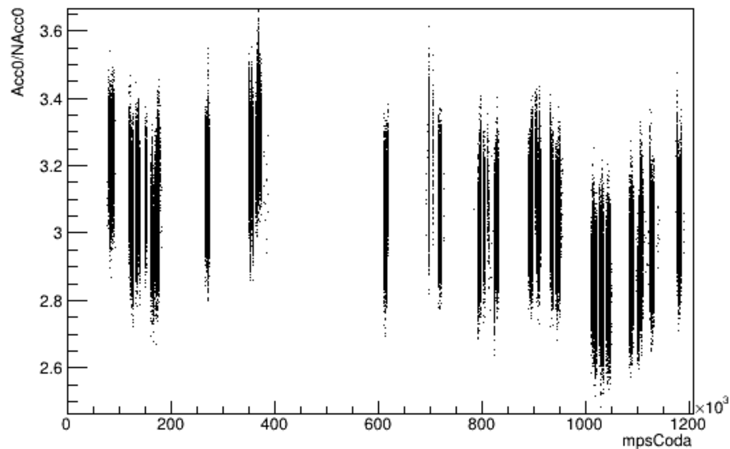
Run 5091 mpwise, Acc0 vs Time: Beam ON, Laser ON
