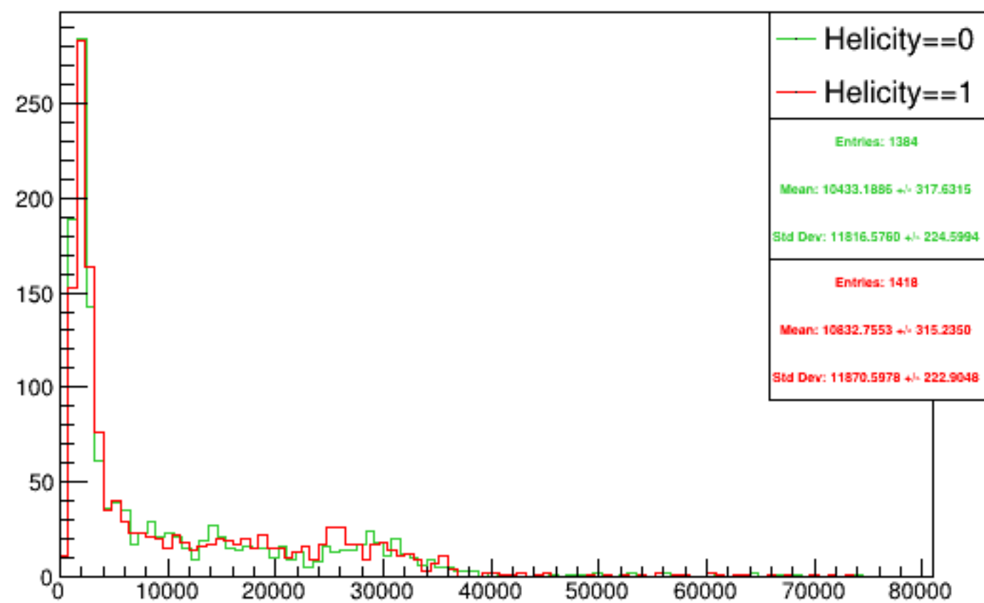
Run 5092 triggerwise, sums: Beam ON, Laser ON
