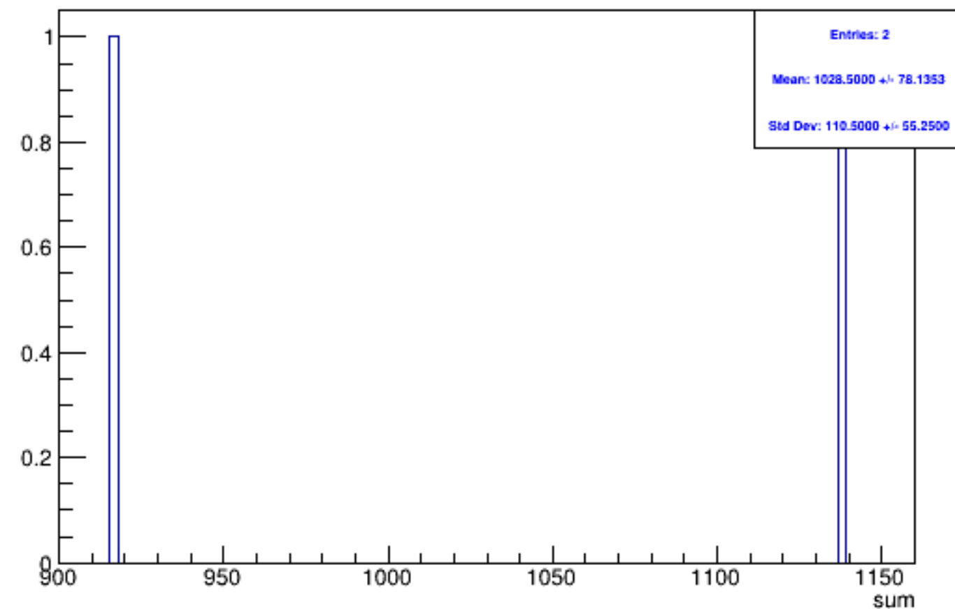
Run 5092 triggerwise, sums: Beam OFF
