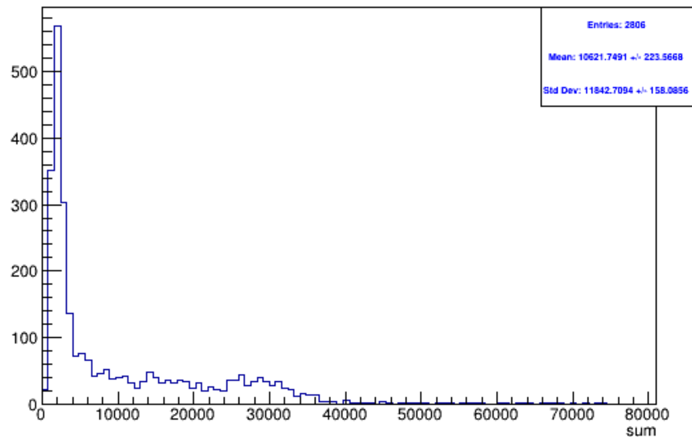
Run 5092 triggerwise, sums: All
