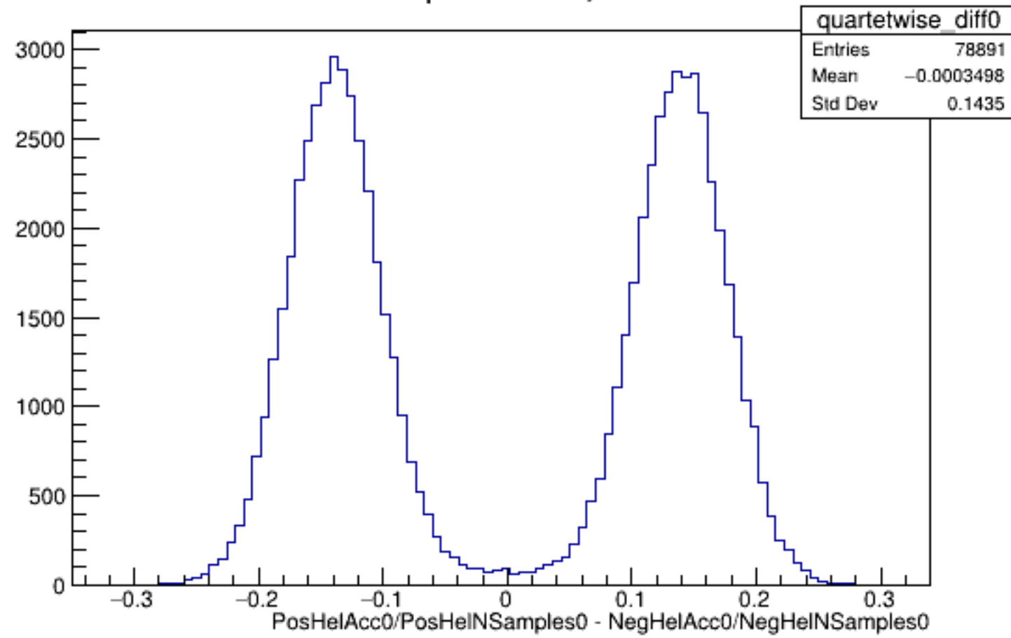
Run 5099 quartetwise, Diffs0: All
