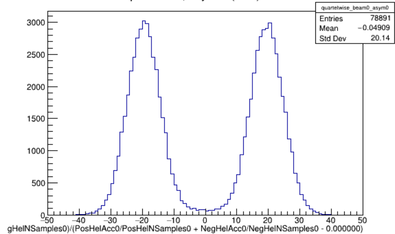
Run 5099 quartetwise, Asyms0 (Raw): Beam OFF
