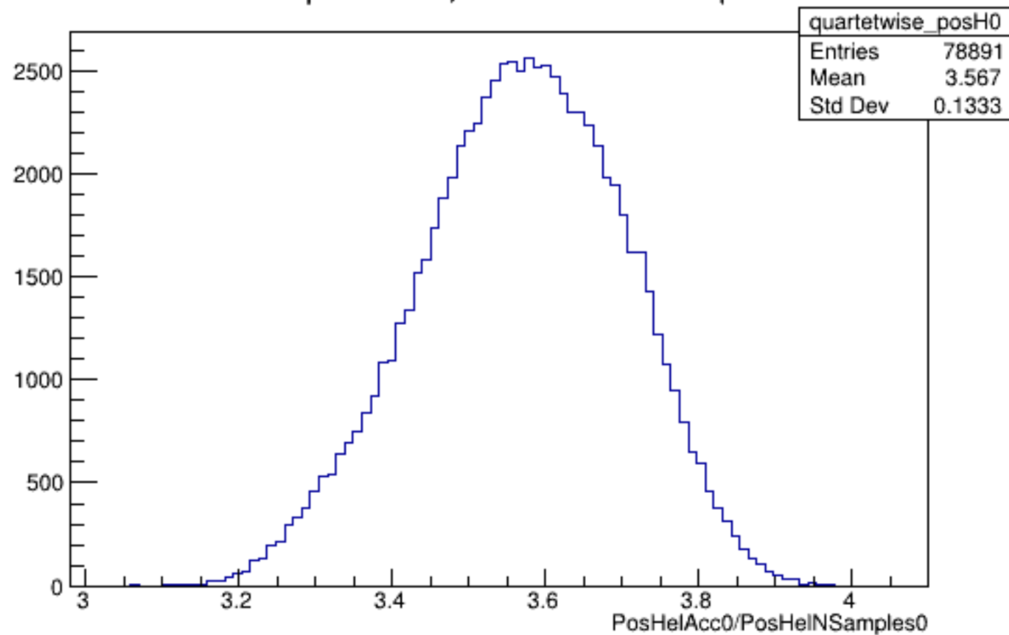
Run 5099 quartetwise, PosHelAcc0/NSamples0: All
