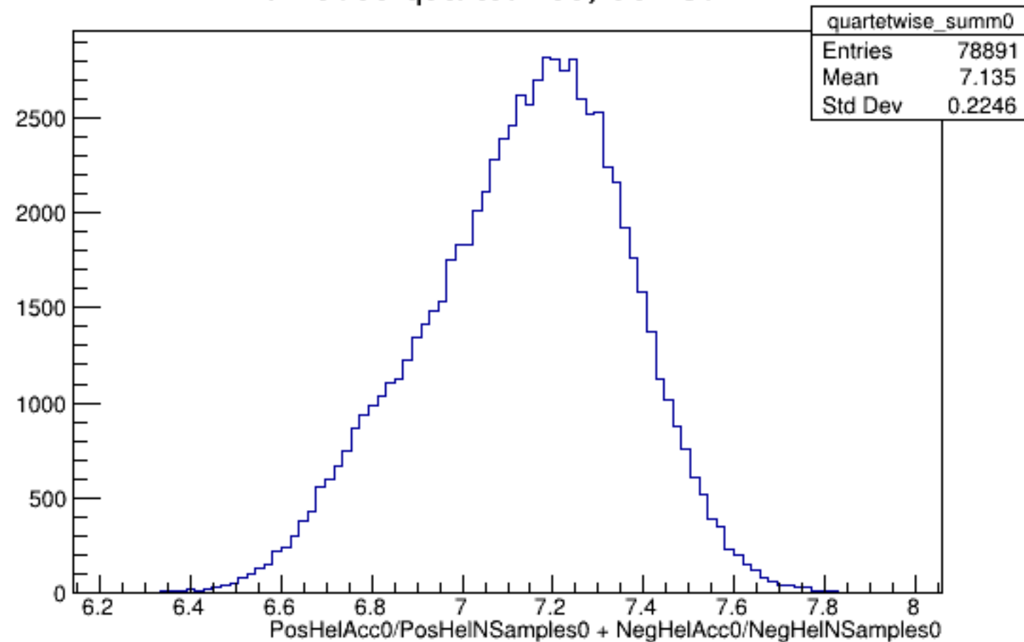
Run 5099 quartetwise, Sums0: All
