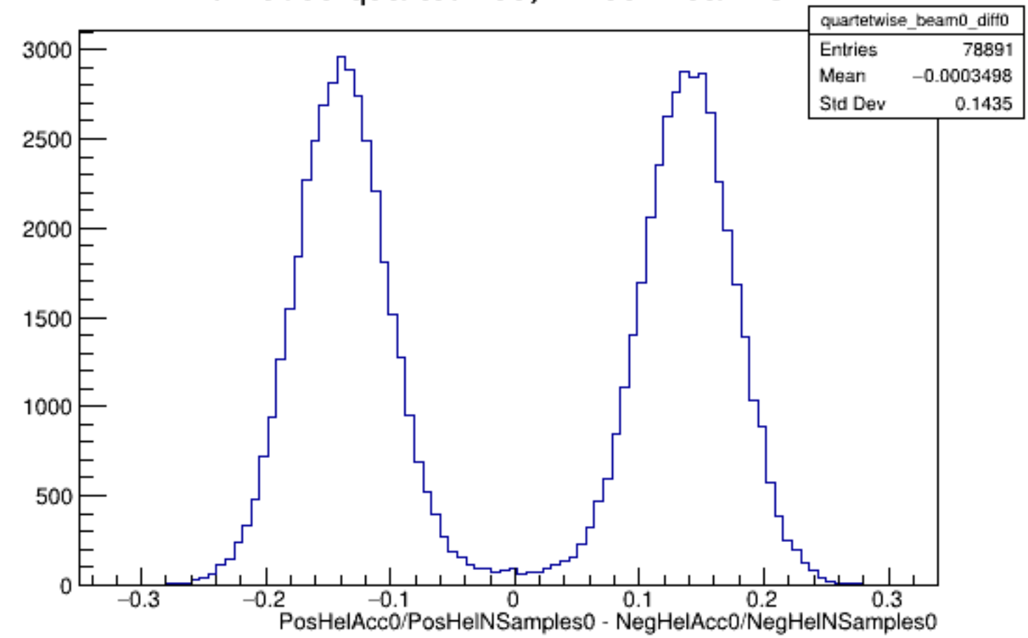
Run 5099 quartetwise, Diffs0: Beam OFF
