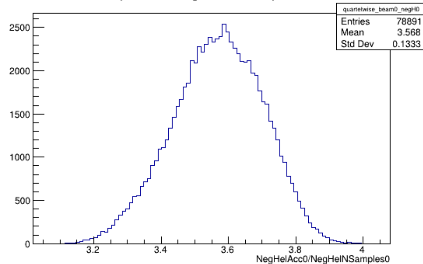
Run 5099 quartetwise, NegHelAcc0/NSamples0: Beam OFF
