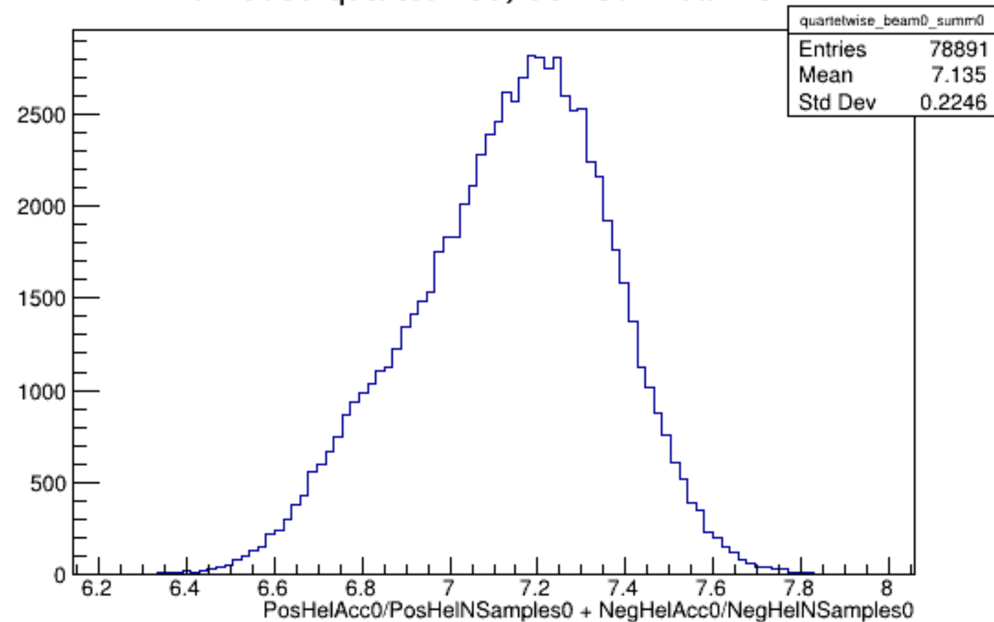
Run 5099 quartetwise, Sums0: Beam OFF
