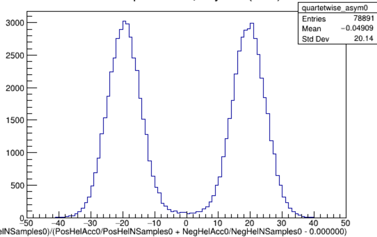
Run 5099 quartetwise, Asyms0 (Raw): All
