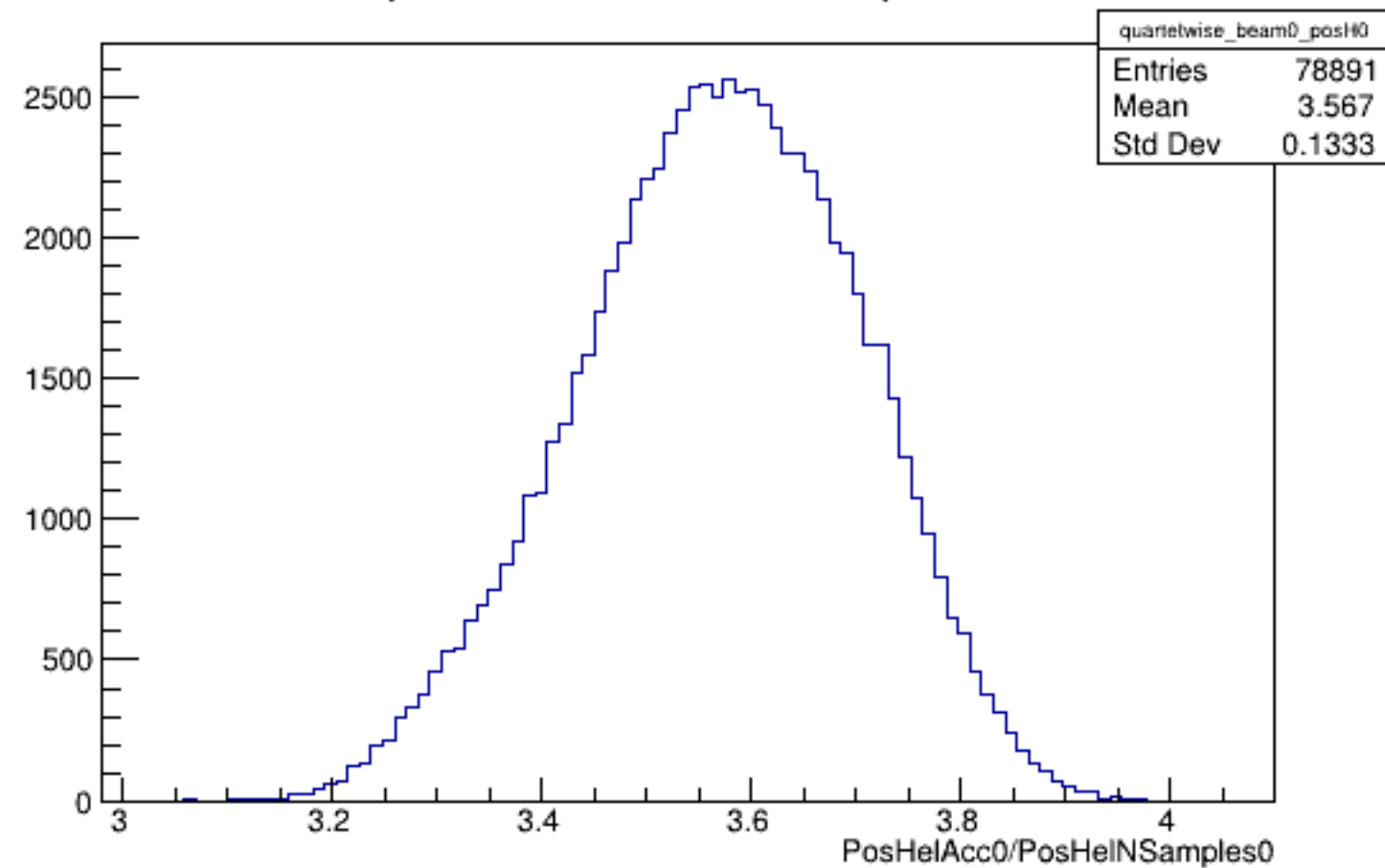
Run 5099 quartetwise, PosHelAcc0/NSamples0: Beam OFF
