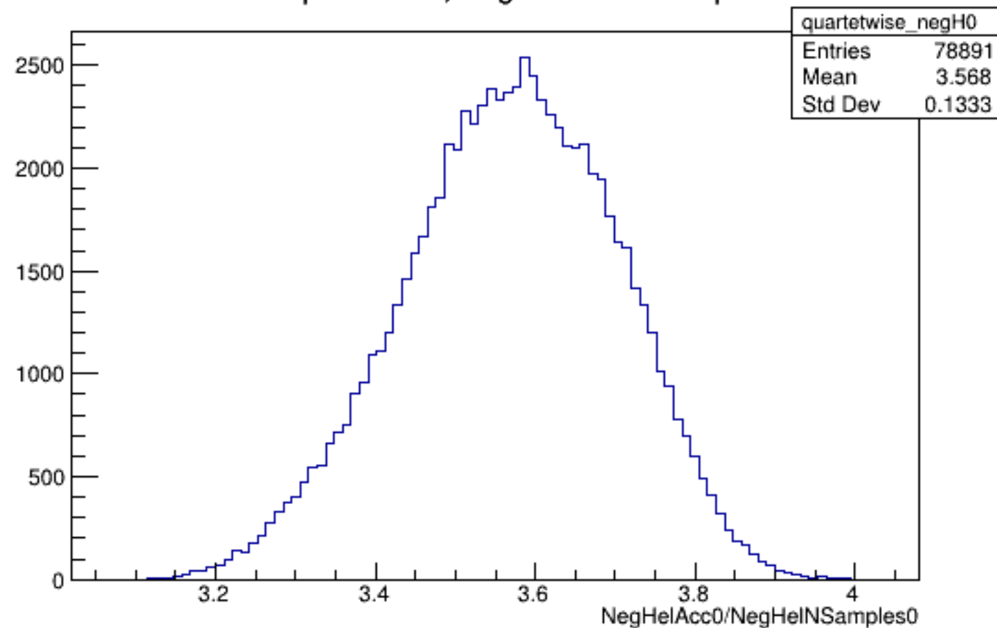
Run 5099 quartetwise, NegHelAcc0/NSamples0: All
