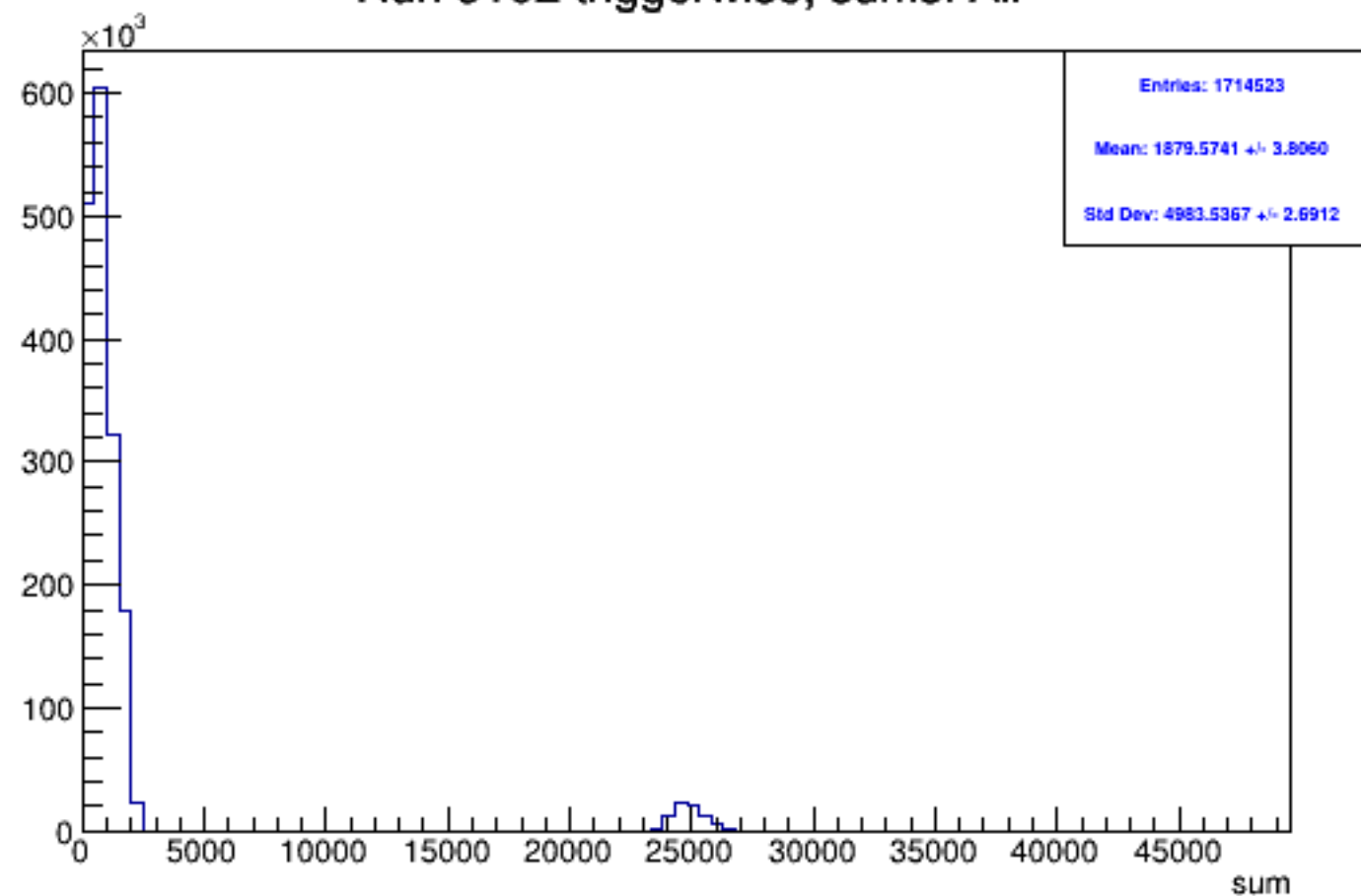
Run 5102 triggerwise, sums: All
