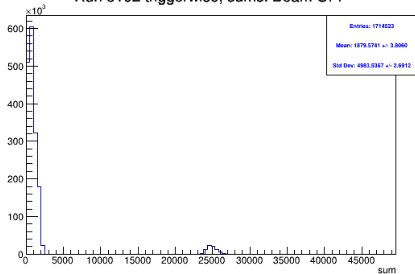
Run 5102 triggerwise, sums: Beam OFF
