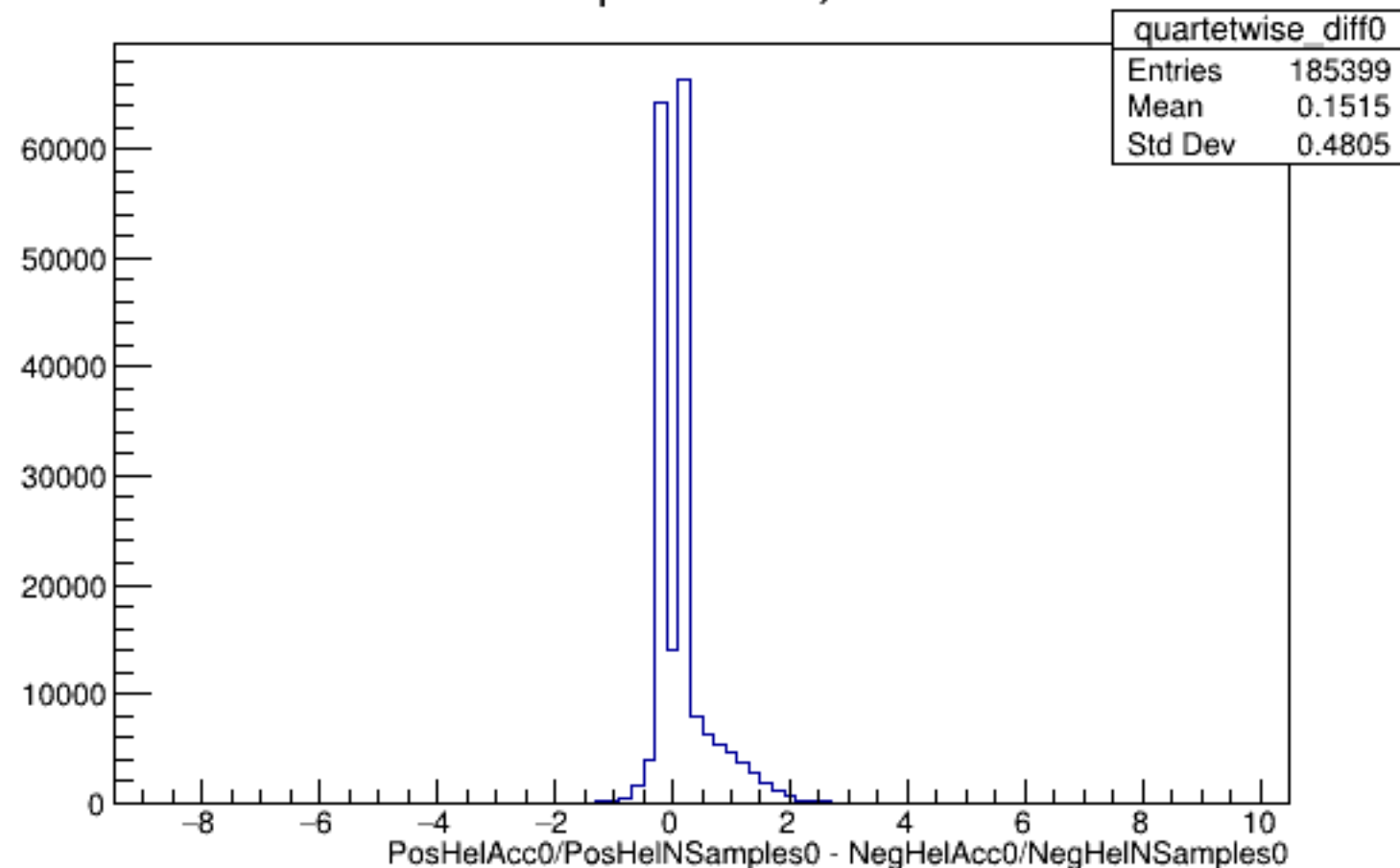
Run 5105 quartetwise, Diffs0: All
