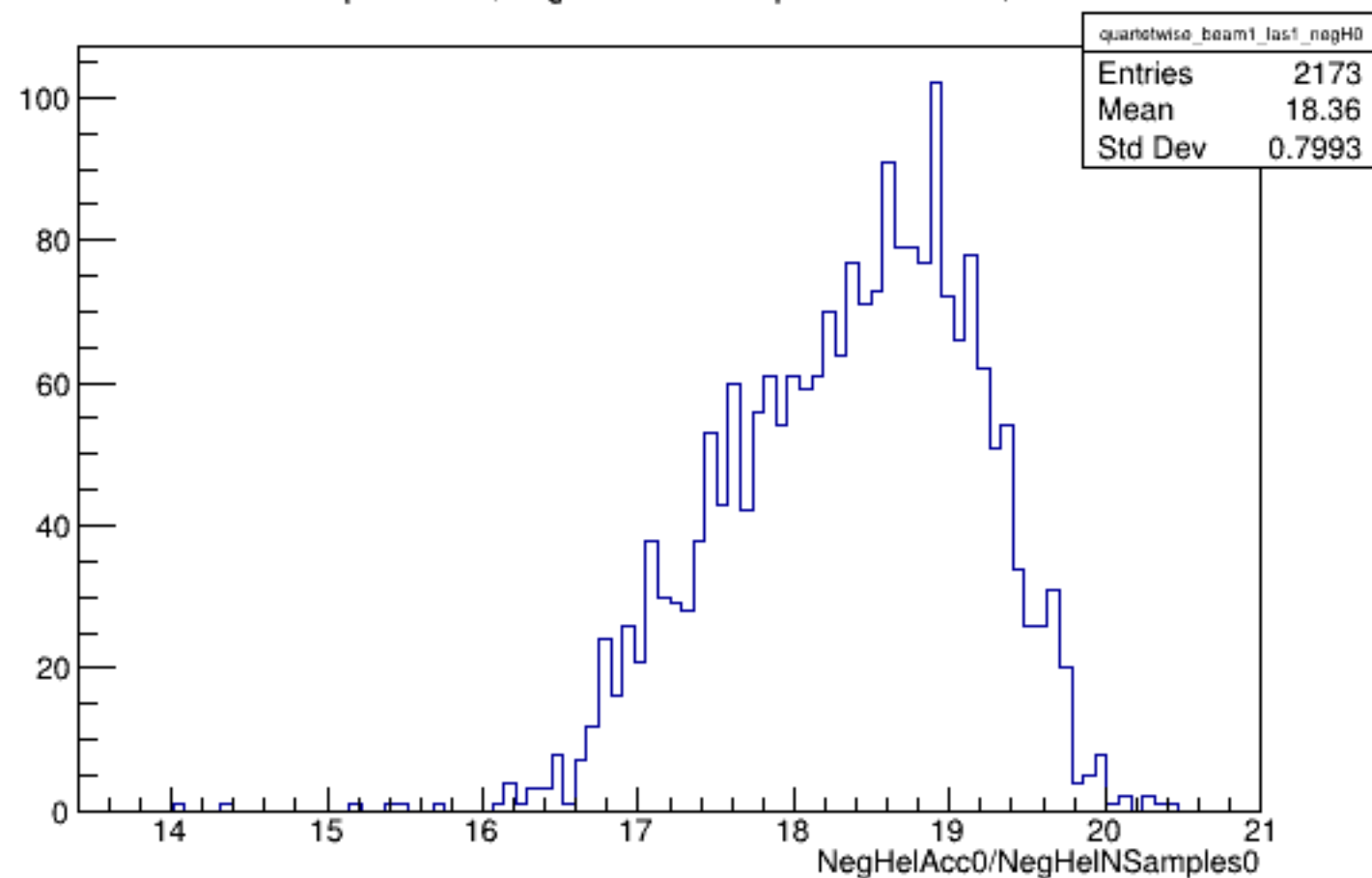
Run 5105 quartetwise, NegHelAcc0/NSamples0: Beam ON, Laser ON
