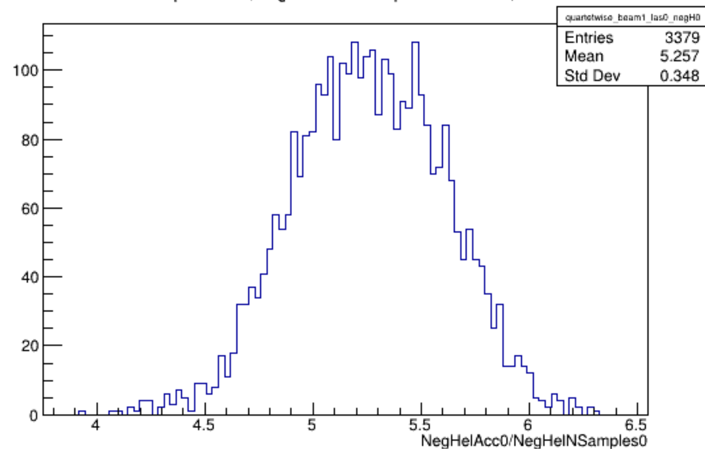
Run 5105 quartetwise, NegHelAcc0/NSamples0: Beam ON, Laser OFF
