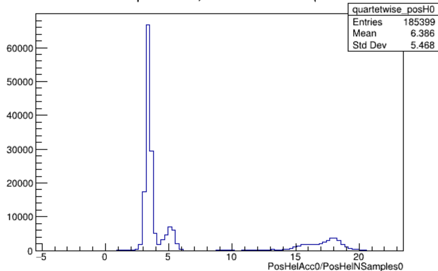
Run 5105 quartetwise, PosHelAcc0/NSamples0: All
