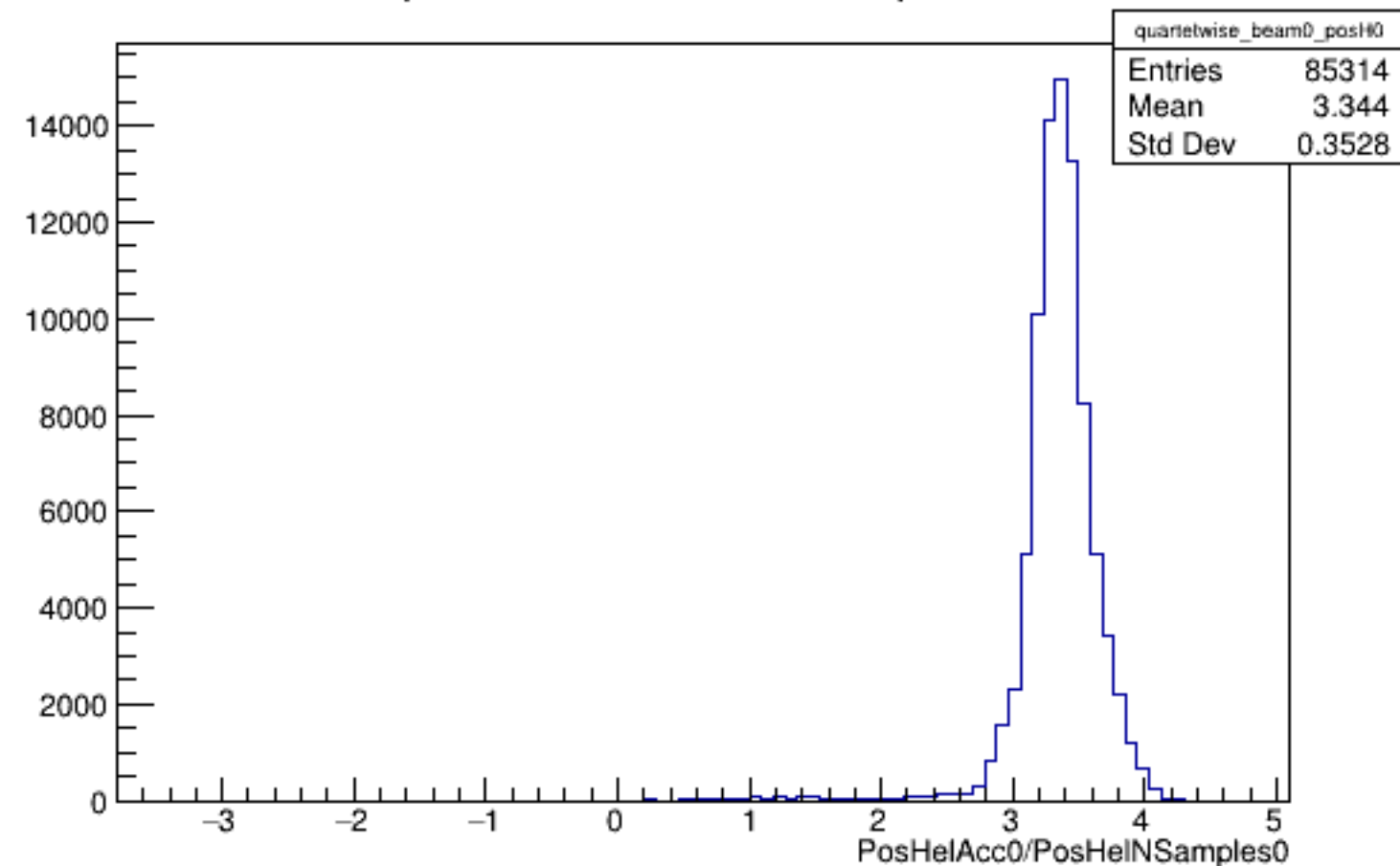
Run 5105 quartetwise, PosHelAcc0/NSamples0: Beam OFF
