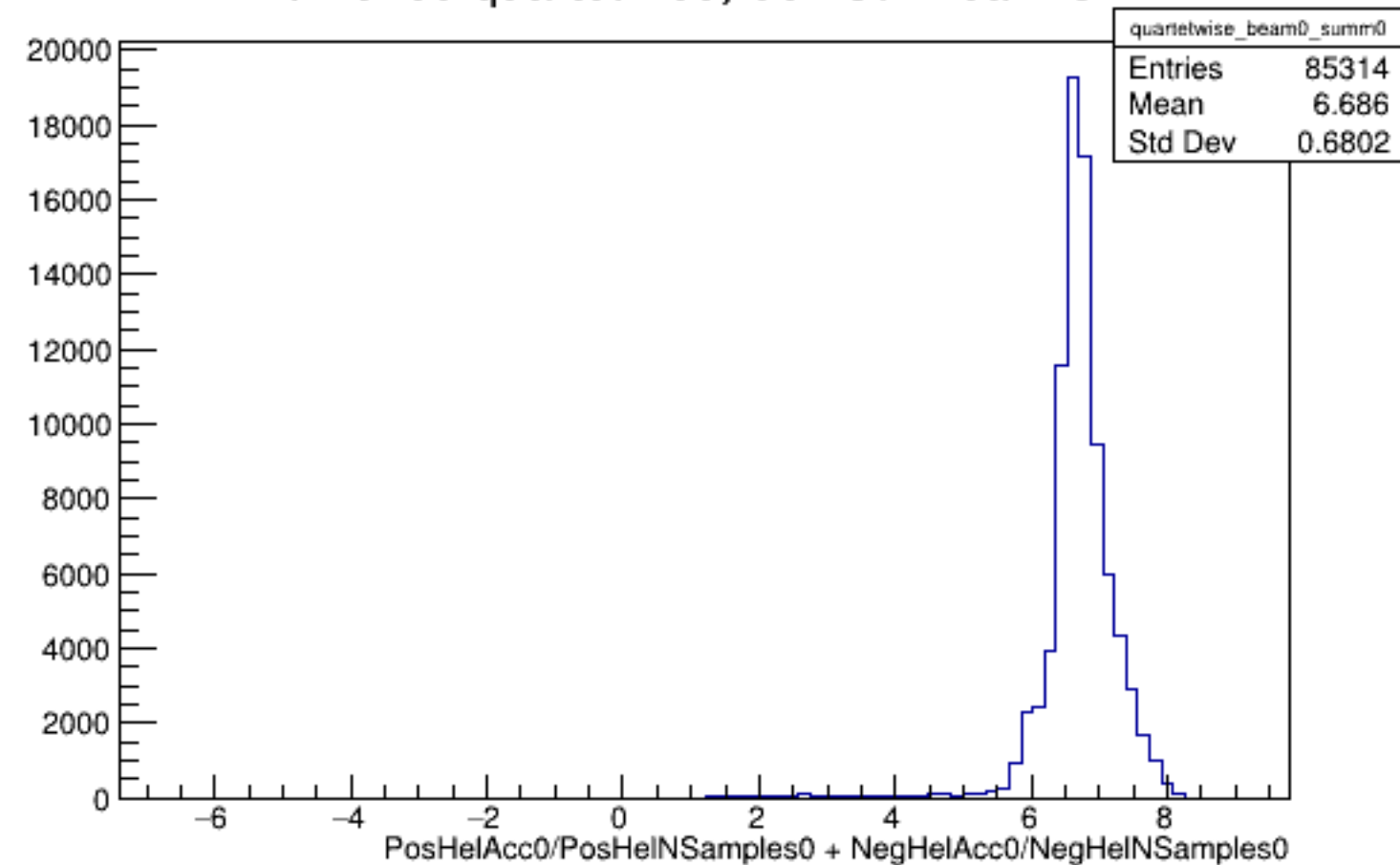
Run 5105 quartetwise, Sums0: Beam OFF
