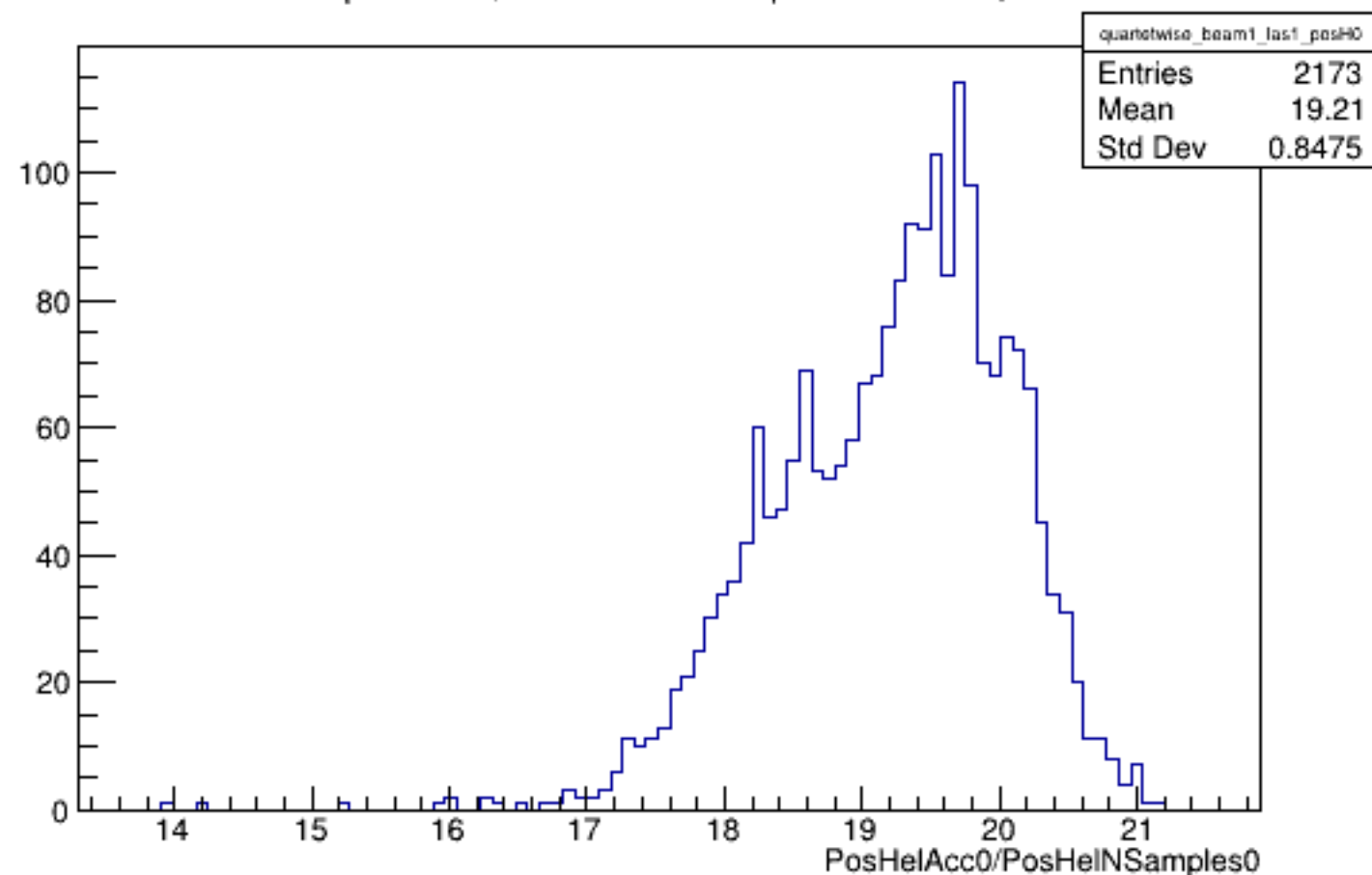
Run 5105 quartetwise, PosHelAcc0/NSamples0: Beam ON, Laser ON
