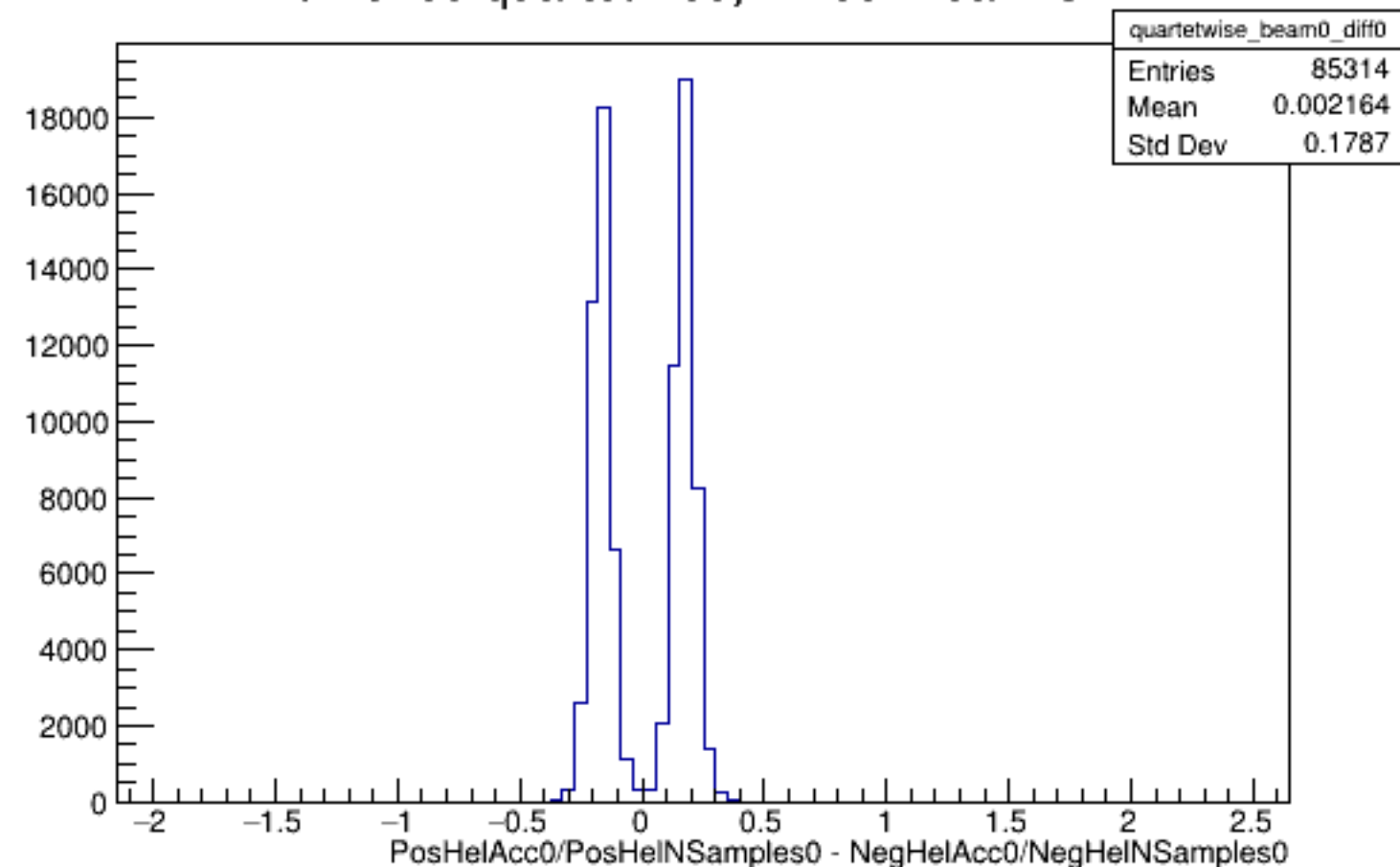
Run 5105 quartetwise, Diffs0: Beam OFF
