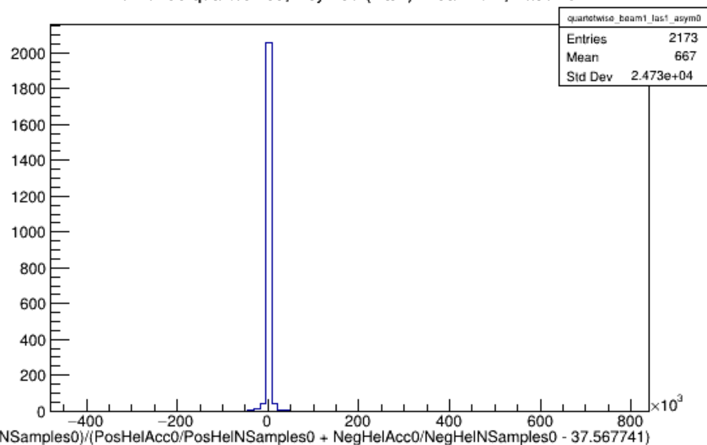
Run 5105 quartetwise, Asyms0 (Raw): Beam ON, Laser ON
