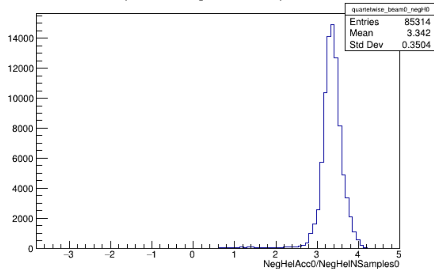
Run 5105 quartetwise, NegHelAcc0/NSamples0: Beam OFF
