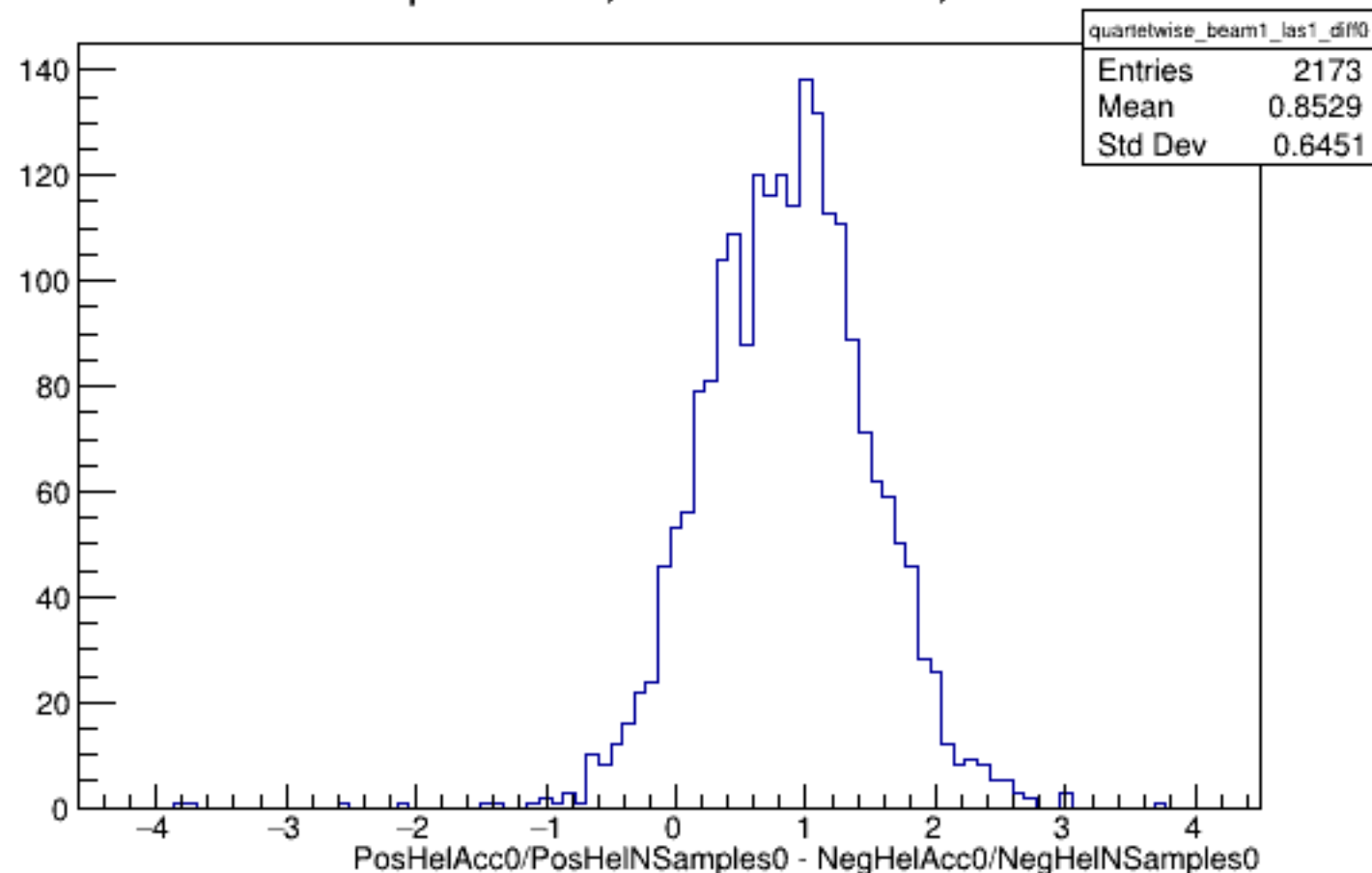
Run 5105 quartetwise, Diffs0: Beam ON, Laser ON
