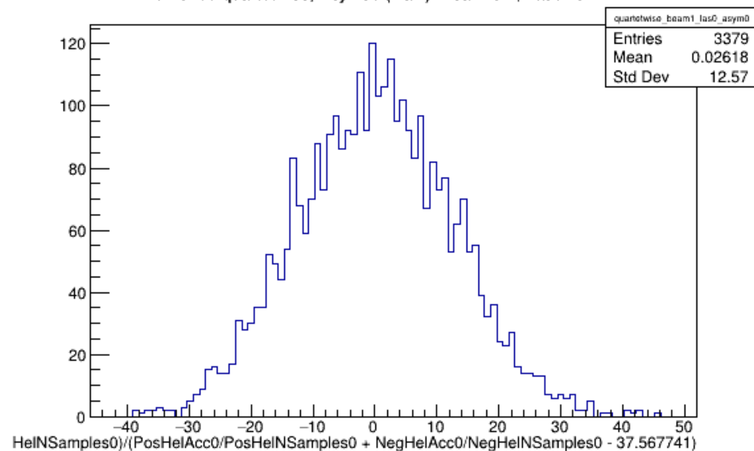
Run 5105 quartetwise, Asyms0 (Raw): Beam ON, Laser OFF
