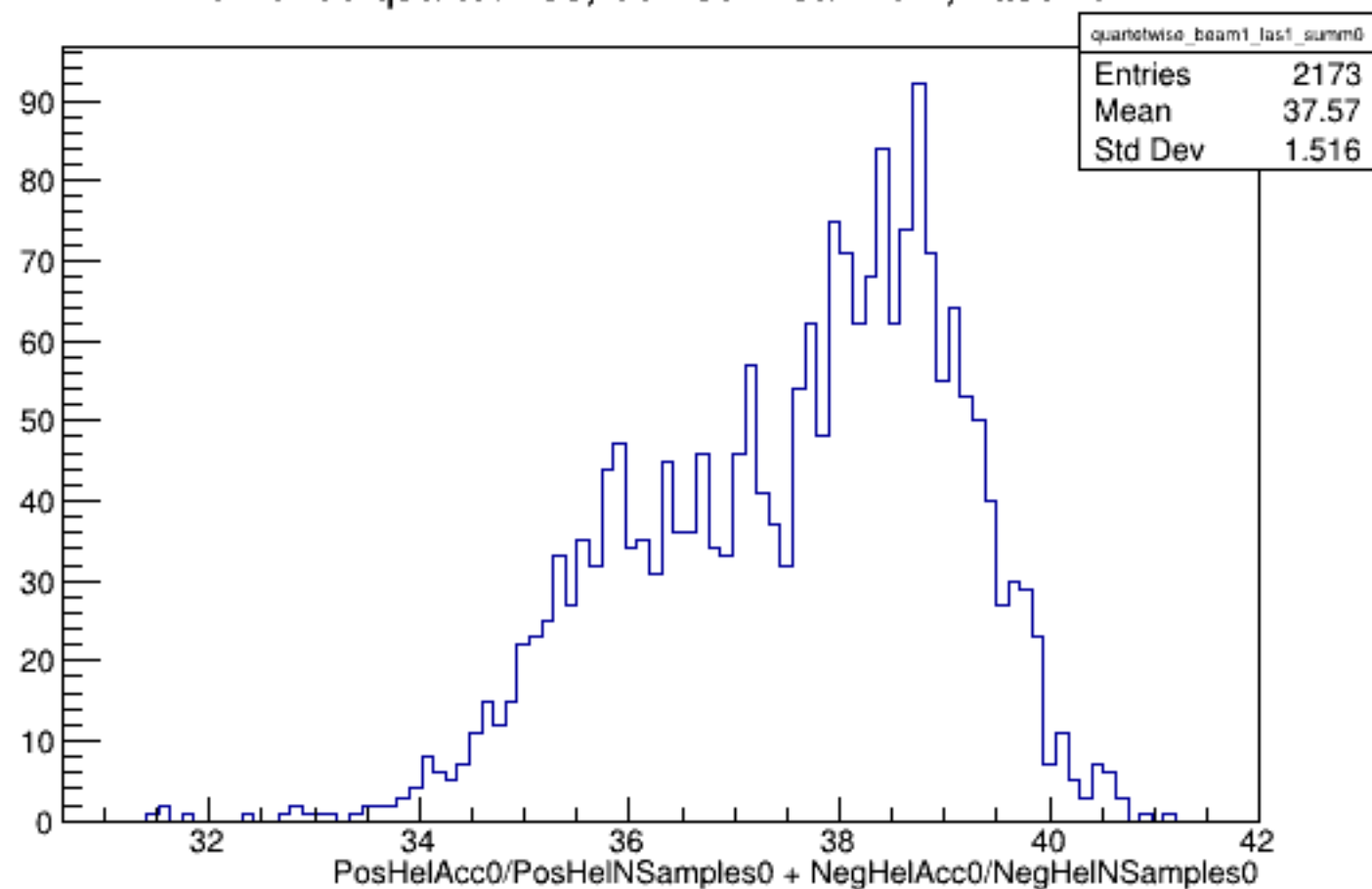
Run 5105 quartetwise, Sums0: Beam ON, Laser ON
