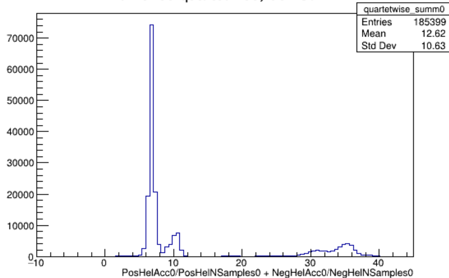
Run 5105 quartetwise, Sums0: All
