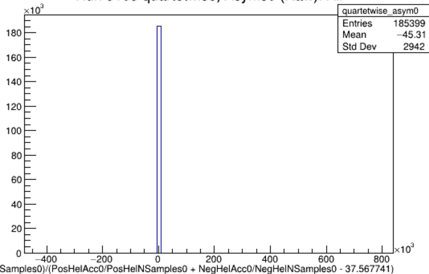
Run 5105 quartetwise, Asyms0 (Raw): All
