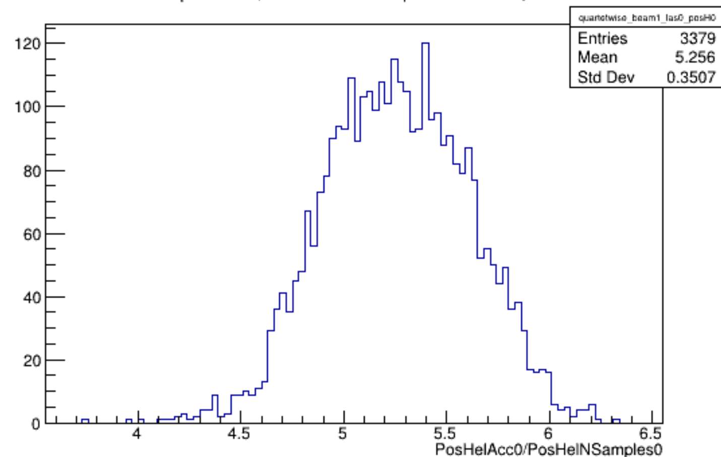
Run 5105 quartetwise, PosHelAcc0/NSamples0: Beam ON, Laser OFF
