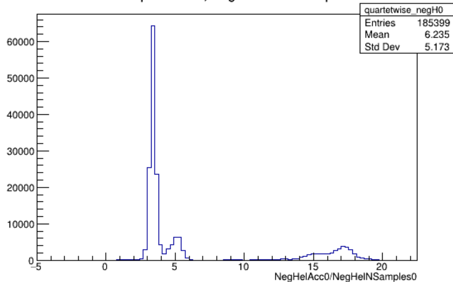
Run 5105 quartetwise, NegHelAcc0/NSamples0: All
