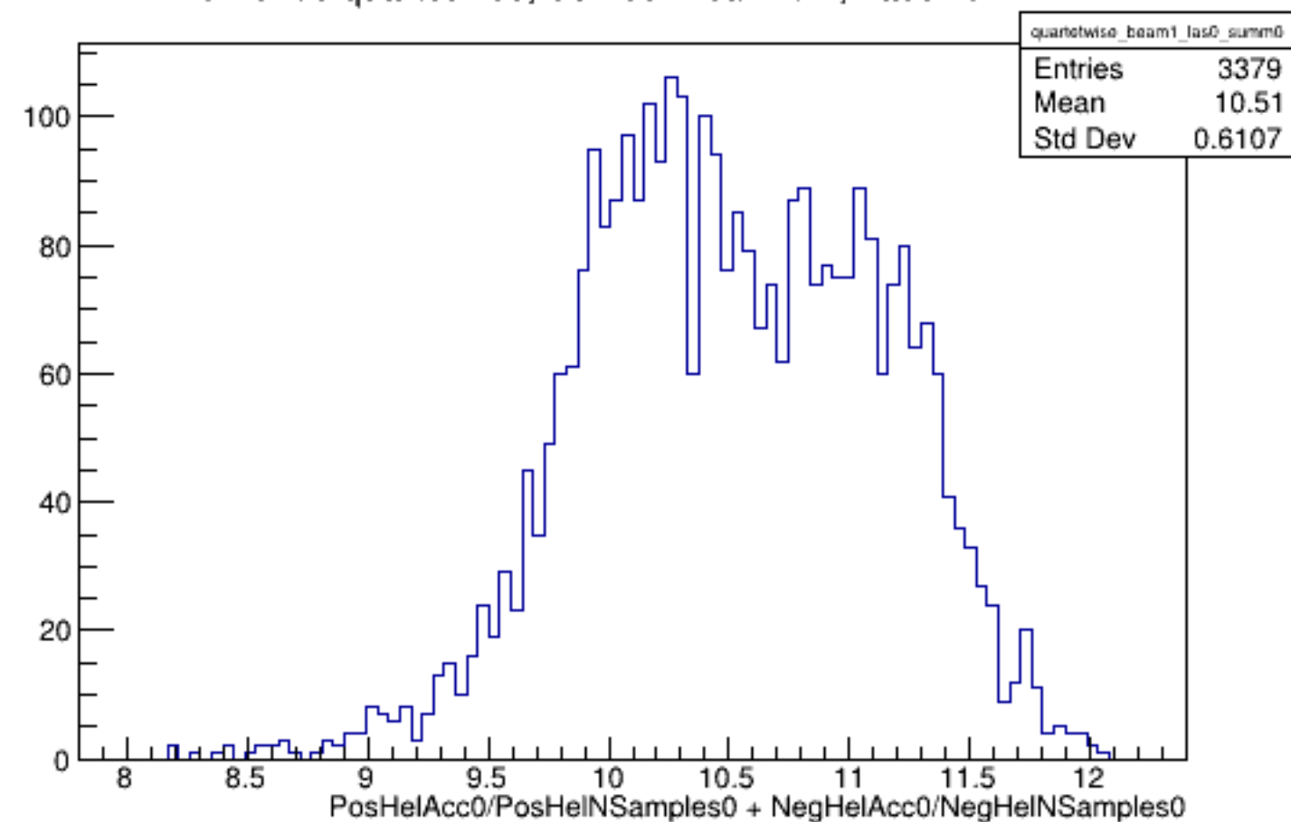
Run 5105 quartetwise, Sums0: Beam ON, Laser OFF
