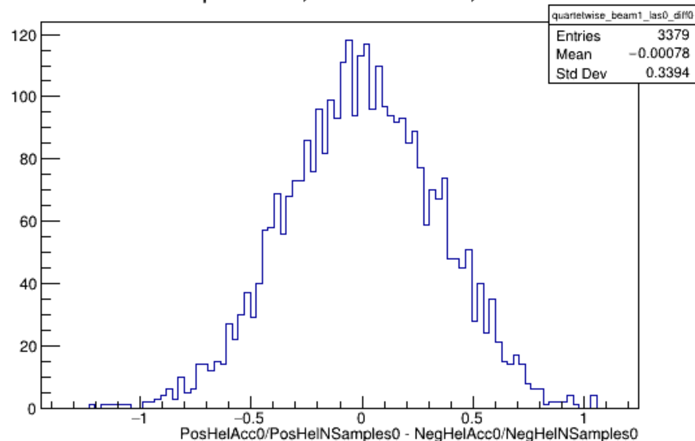
Run 5105 quartetwise, Diffs0: Beam ON, Laser OFF
