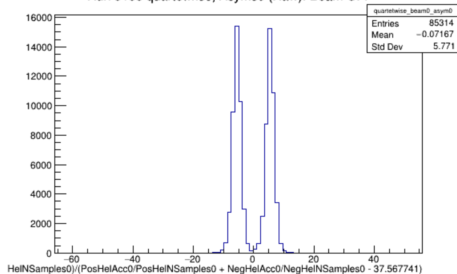
Run 5105 quartetwise, Asyms0 (Raw): Beam OFF
