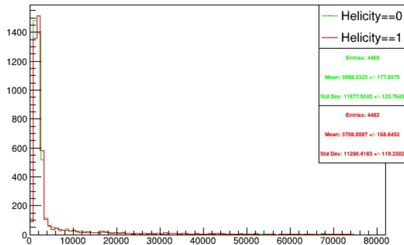
Run 5105 triggerwise, sums: Beam ON, Laser OFF
