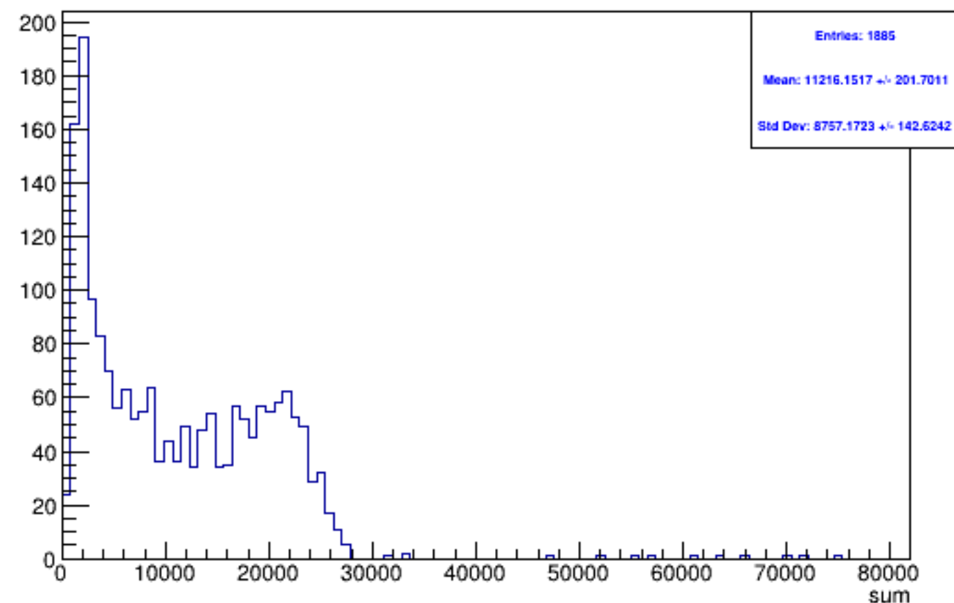
Run 5105 triggerwise, sums: Beam OFF
