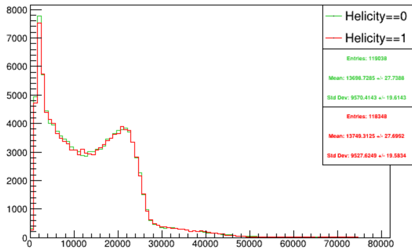
Run 5105 triggerwise, sums: Beam ON, Laser ON
