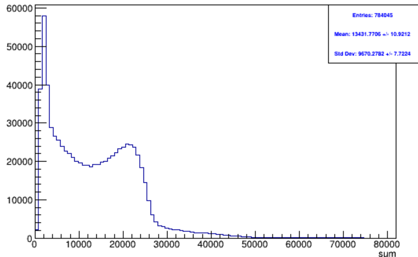
Run 5105 triggerwise, sums: All
