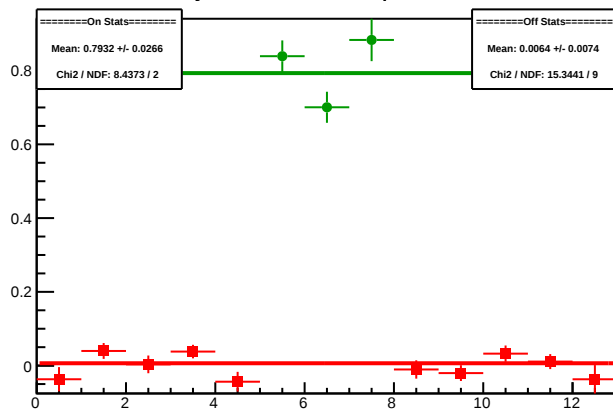
Cycle 5110.2: Multiplet Diffs
