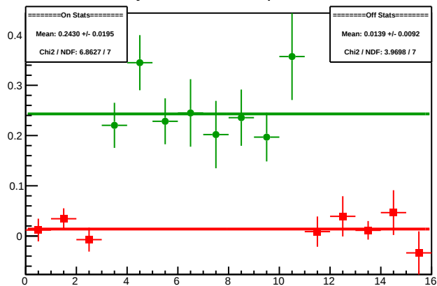
Cycle 5110.1: Multiplet Diffs
