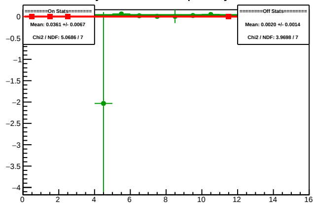
Cycle 5110.1: Multiplet Asyms
