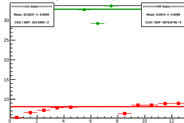
Cycle 5110.2: Multiplet Sums
