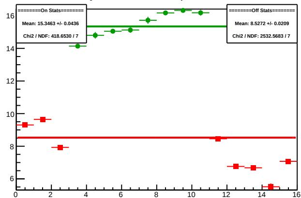
Cycle 5110.1: Multiplet Sums
