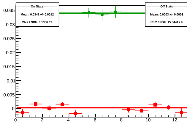
Cycle 5110.2: Multiplet Asyms
