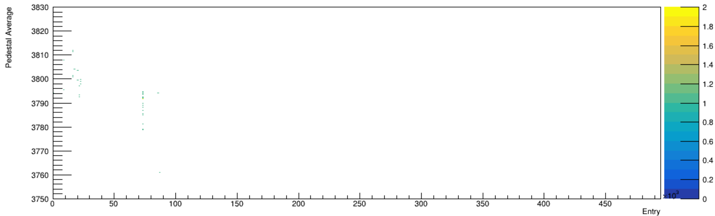
Run 5114, snapshots: Pedestal vs. Time
