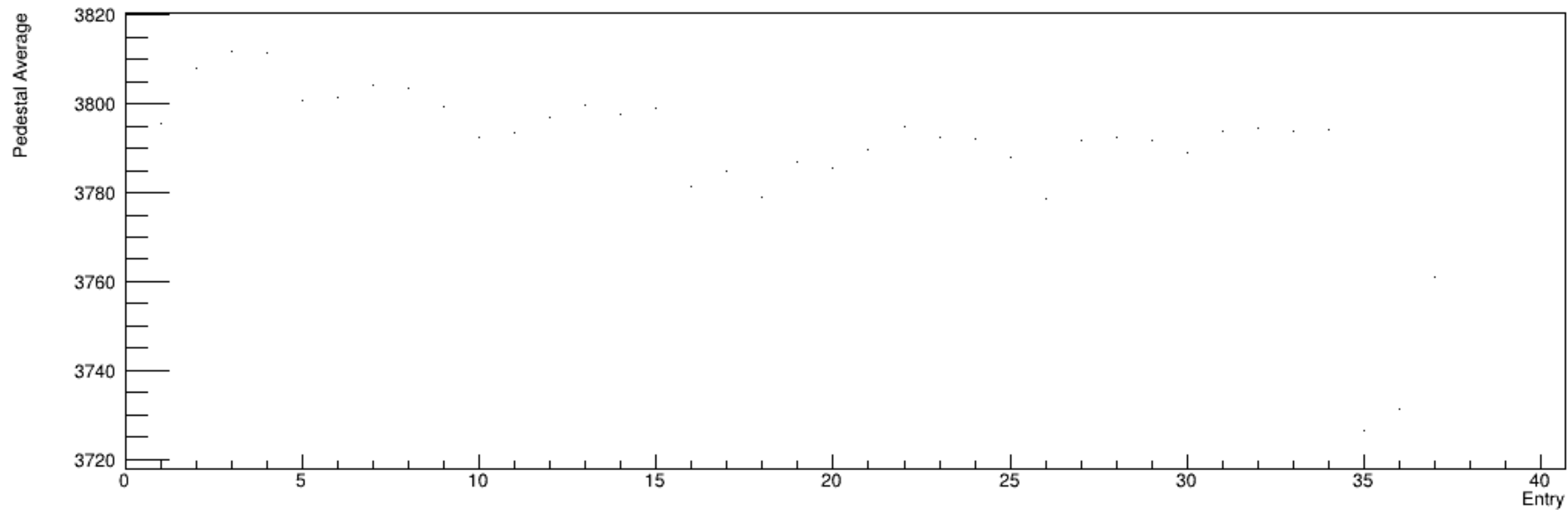
Run 5114, snapshots: Pedestal vs. Time
