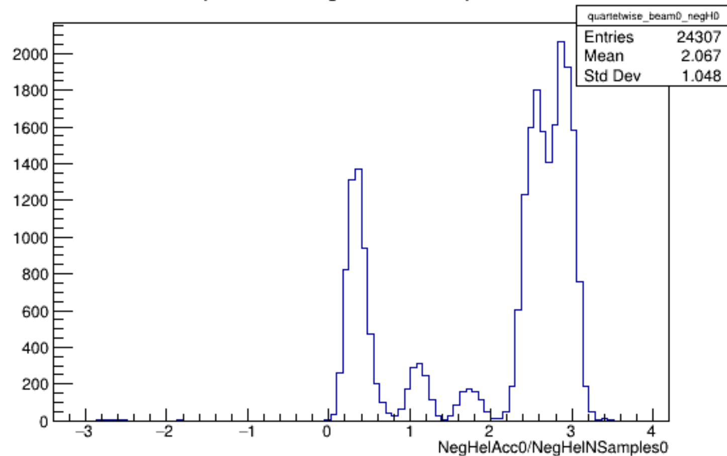
Run 5118 quartetwise, NegHelAcc0/NSamples0: Beam OFF
