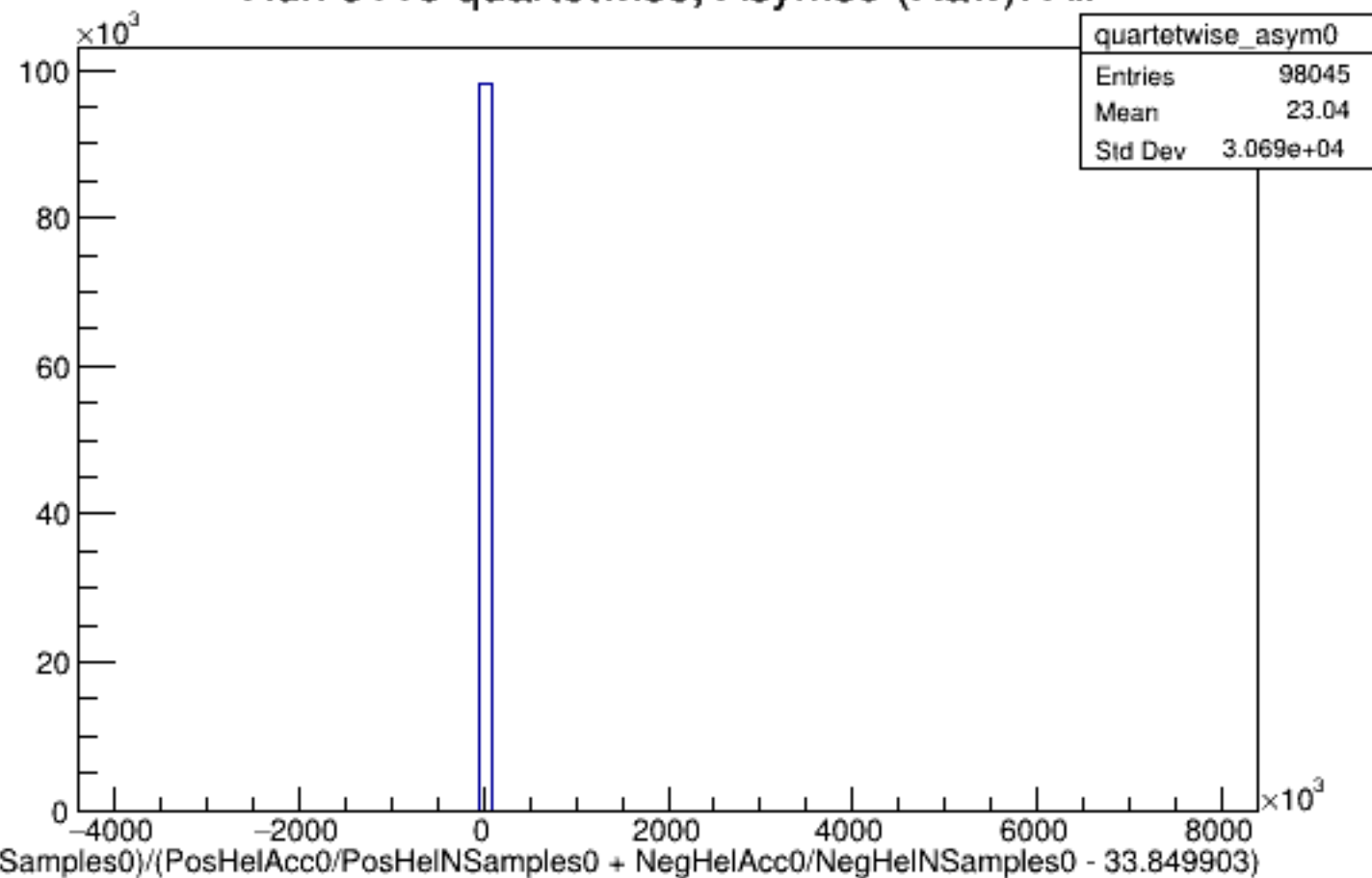
Run 5118 quartetwise, Asyms0 (Raw): All
