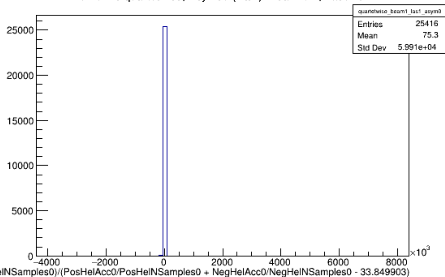
Run 5118 quartetwise, Asyms0 (Raw): Beam ON, Laser ON
