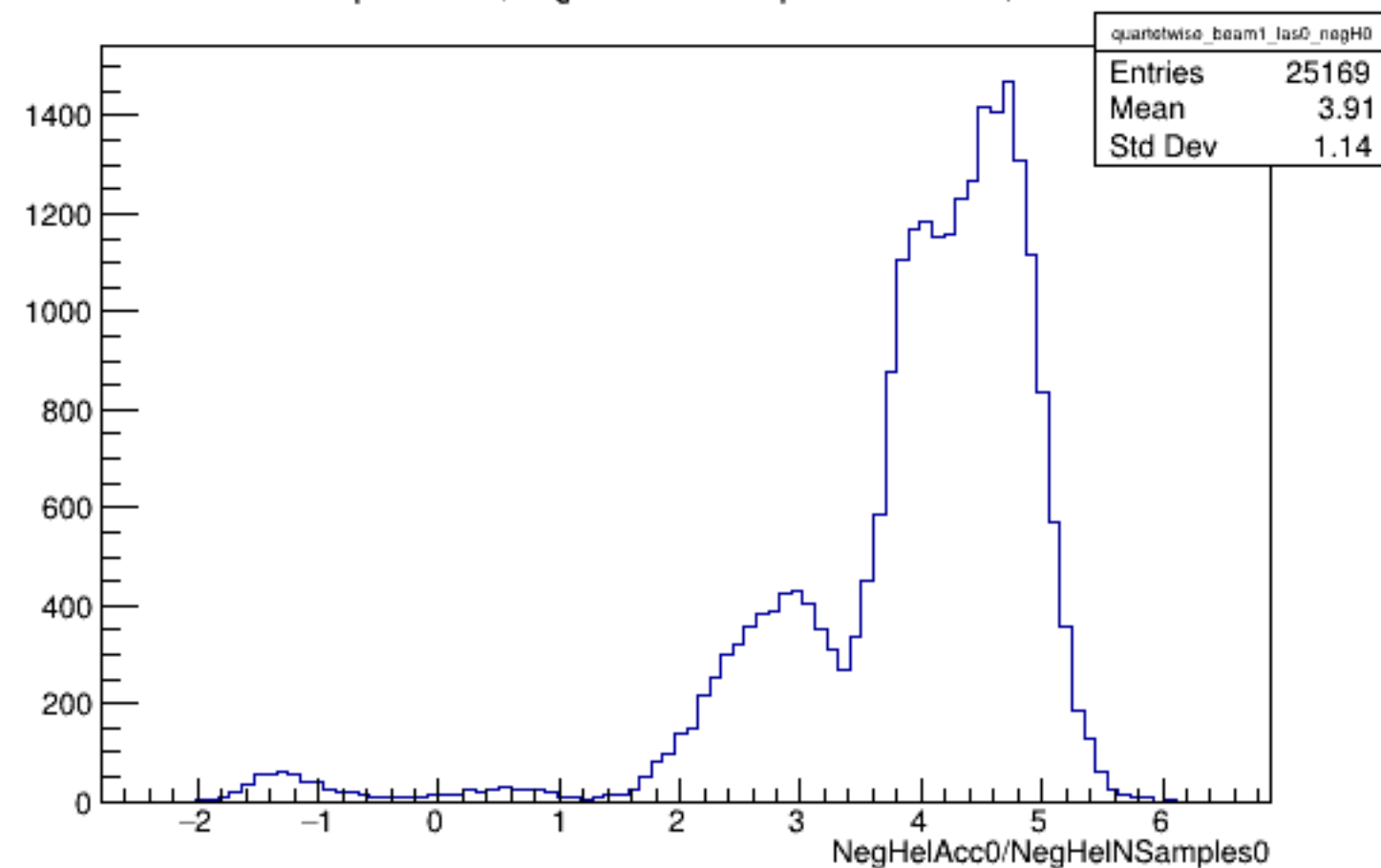
Run 5118 quartetwise, NegHelAcc0/NSamples0: Beam ON, Laser OFF
