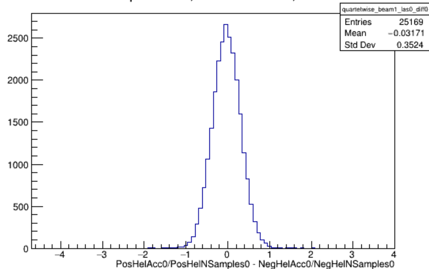
Run 5118 quartetwise, Diffs0: Beam ON, Laser OFF
