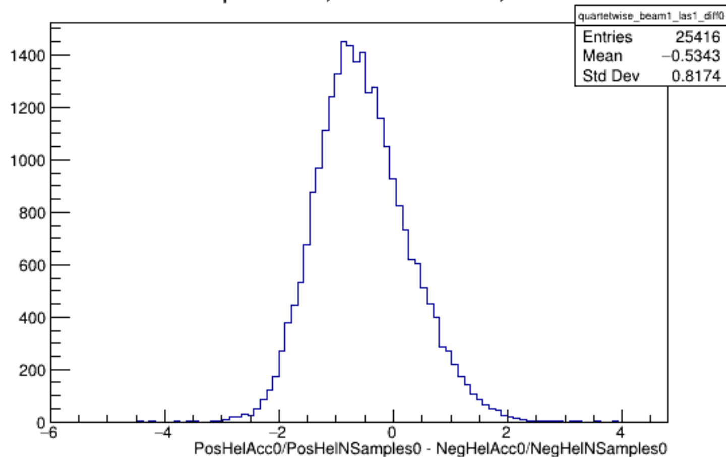
Run 5118 quartetwise, Diffs0: Beam ON, Laser ON
