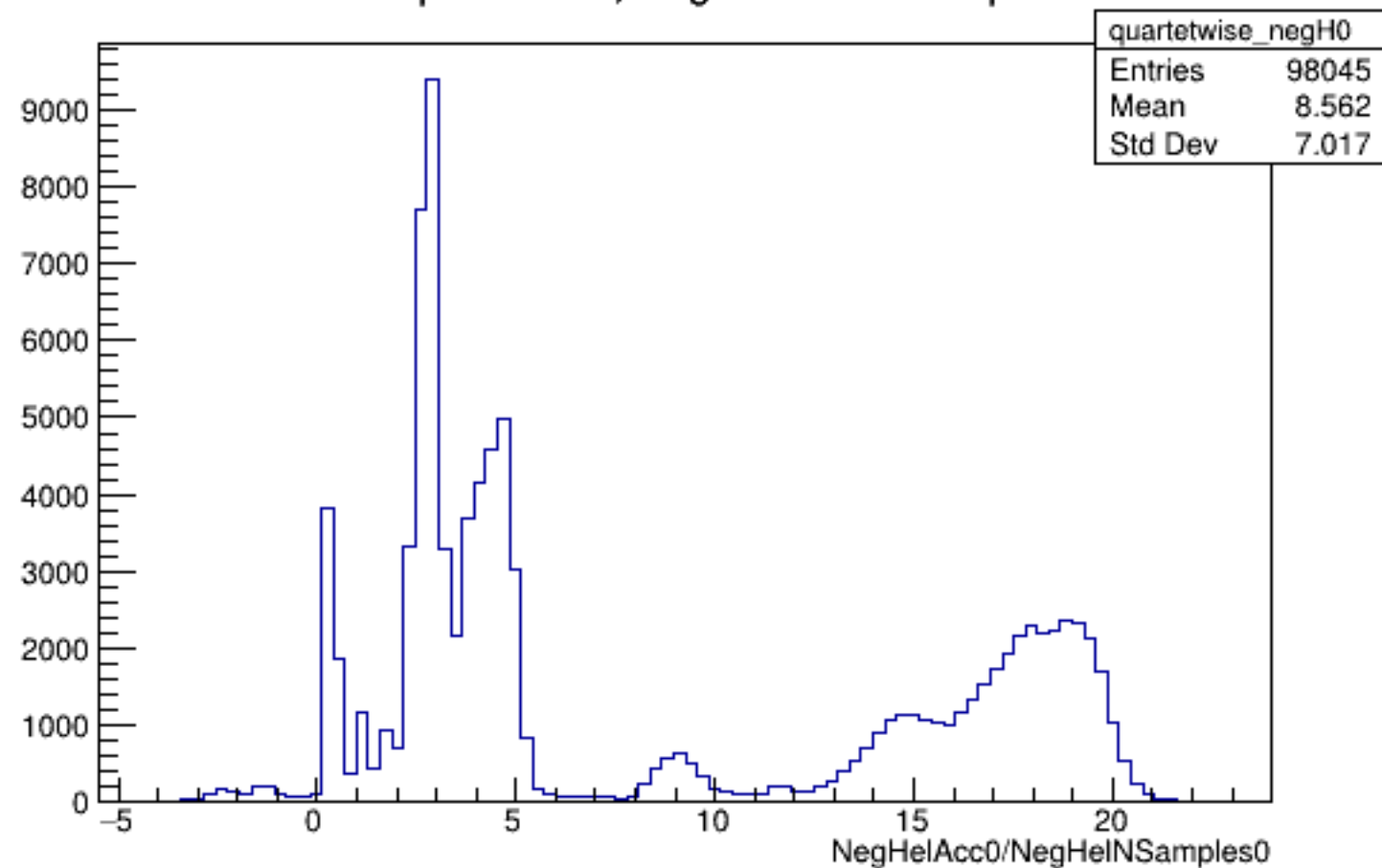
Run 5118 quartetwise, NegHelAcc0/NSamples0: All
