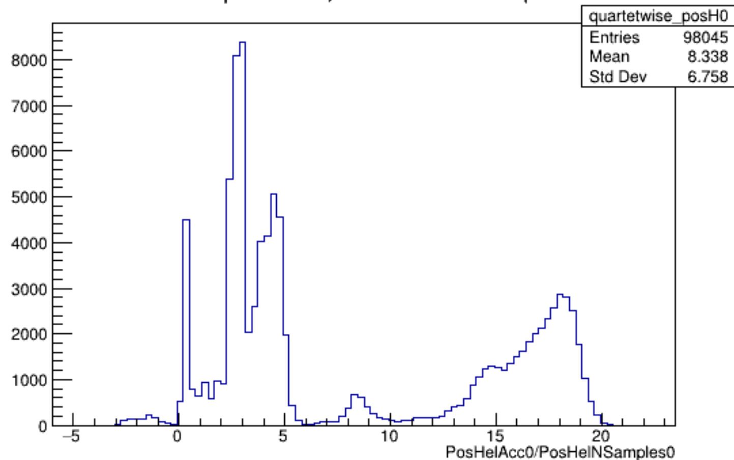
Run 5118 quartetwise, PosHelAcc0/NSamples0: All
