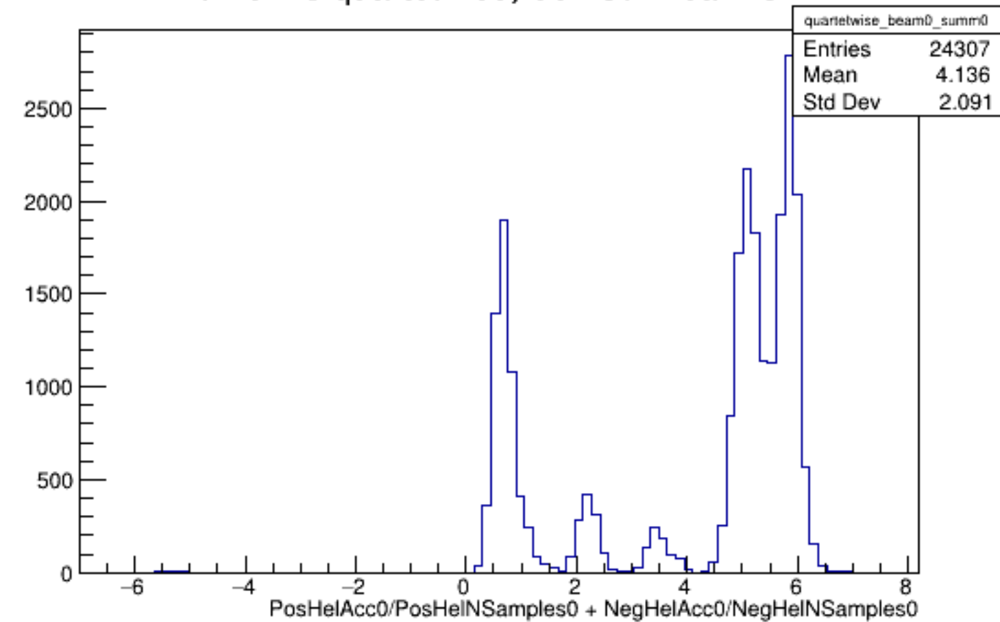
Run 5118 quartetwise, Sums0: Beam OFF
