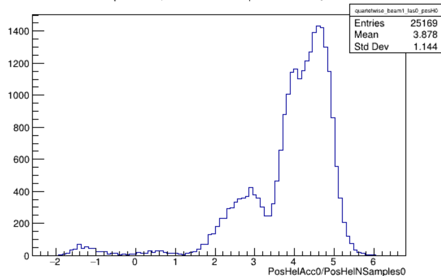
Run 5118 quartetwise, PosHelAcc0/NSamples0: Beam ON, Laser OFF
