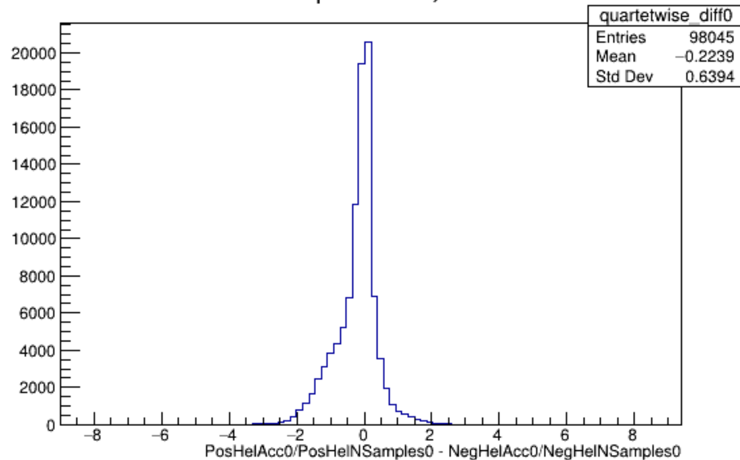
Run 5118 quartetwise, Diffs0: All
