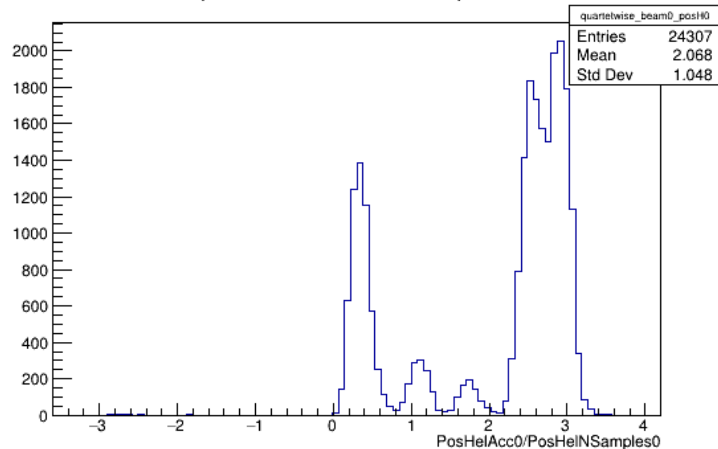
Run 5118 quartetwise, PosHelAcc0/NSamples0: Beam OFF
