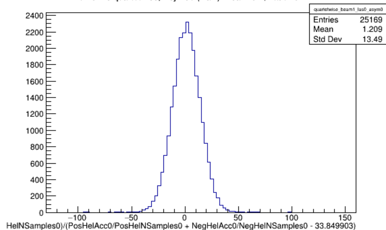
Run 5118 quartetwise, Asyms0 (Raw): Beam ON, Laser OFF
