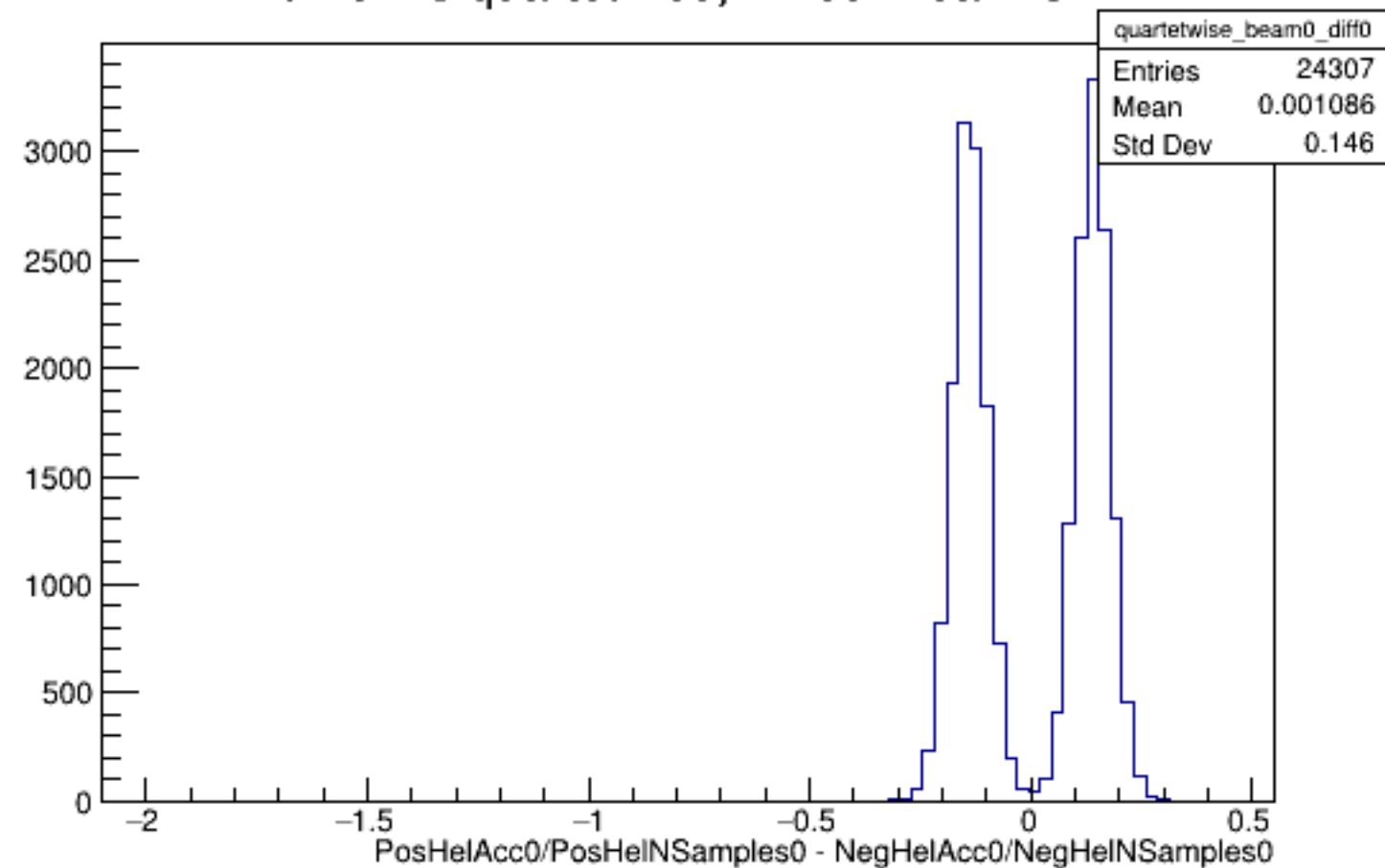
Run 5118 quartetwise, Diffs0: Beam OFF
