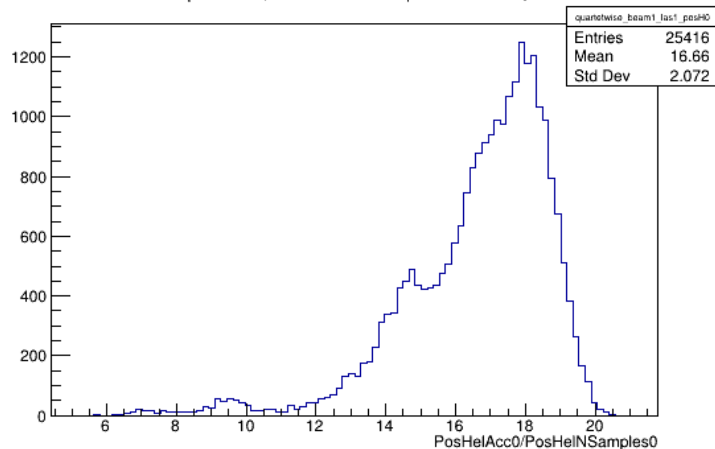
Run 5118 quartetwise, PosHelAcc0/NSamples0: Beam ON, Laser ON
