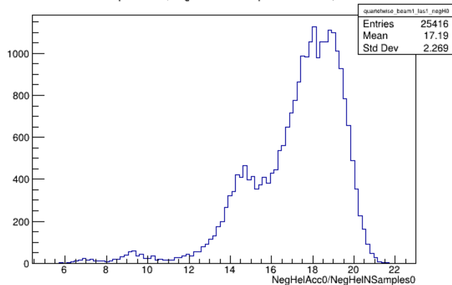
Run 5118 quartetwise, NegHelAcc0/NSamples0: Beam ON, Laser ON
