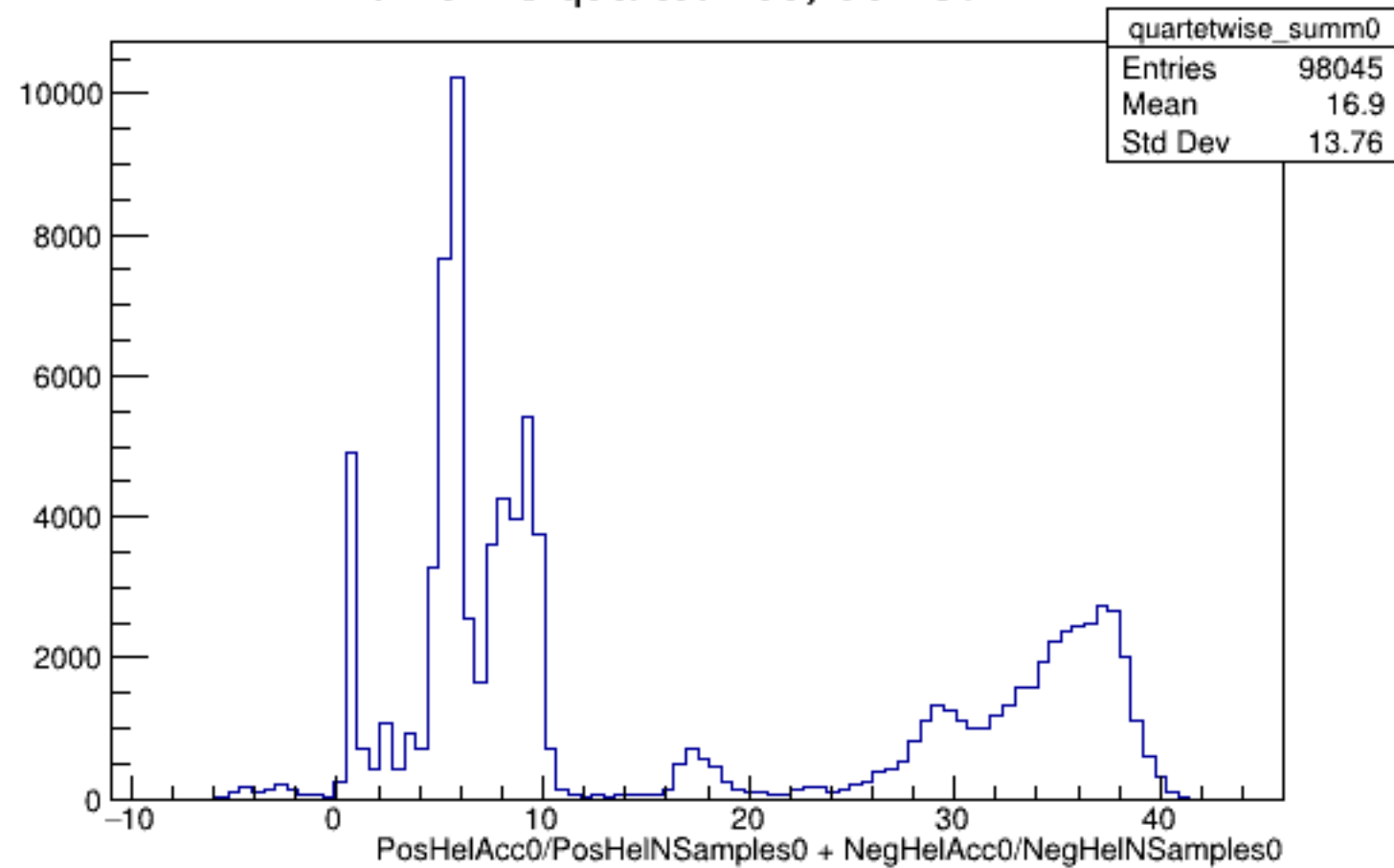
Run 5118 quartetwise, Sums0: All
