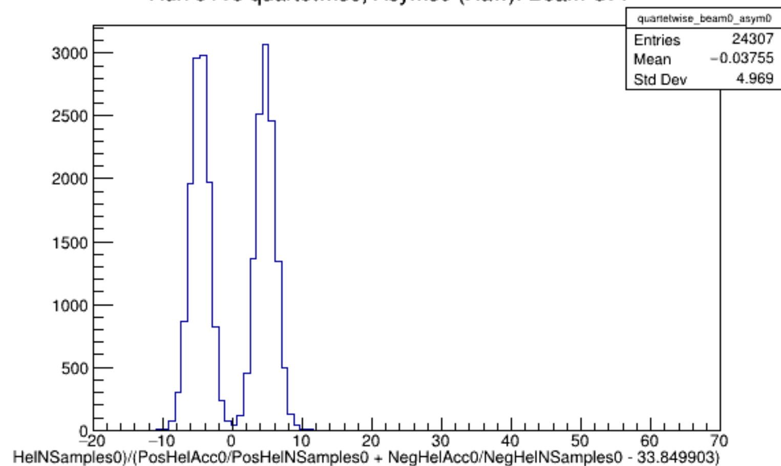
Run 5118 quartetwise, Asyms0 (Raw): Beam OFF
