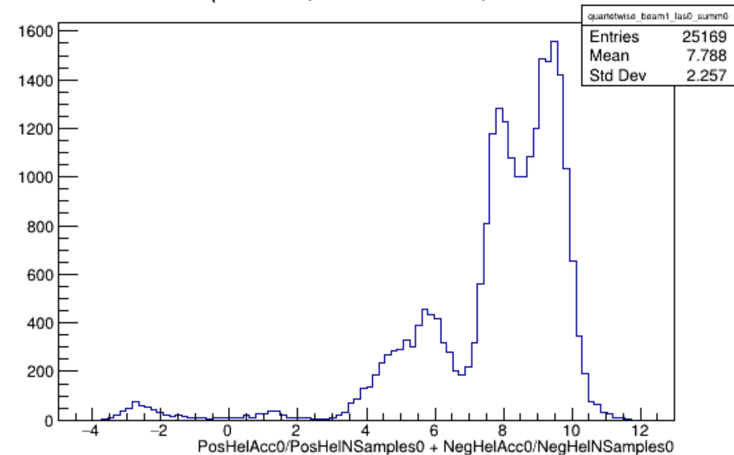
Run 5118 quartetwise, Sums0: Beam ON, Laser OFF
