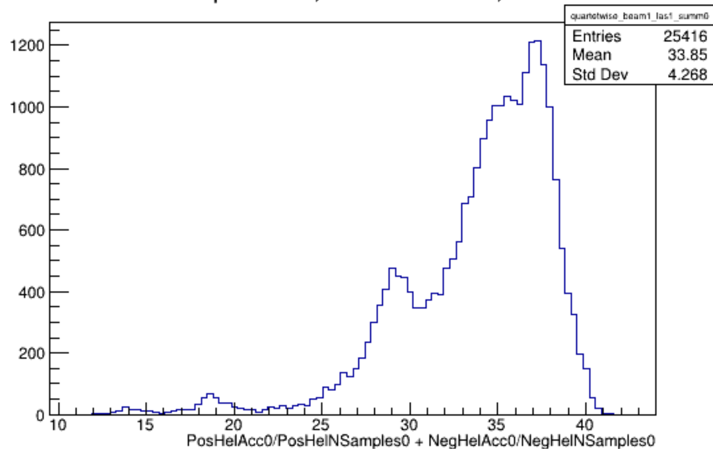
Run 5118 quartetwise, Sums0: Beam ON, Laser ON
