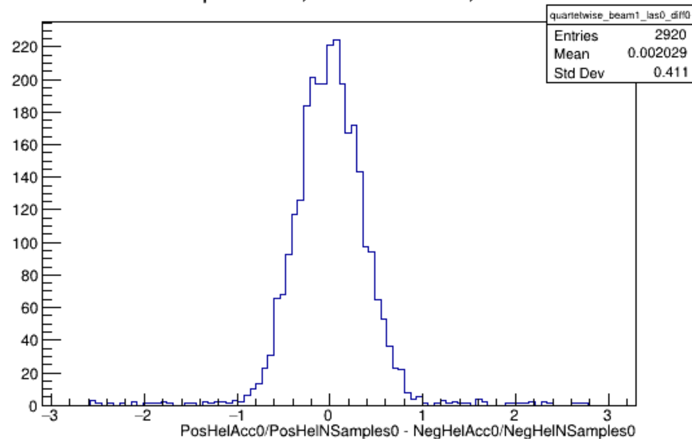
Run 5120 quartetwise, Diffs0: Beam ON, Laser OFF
