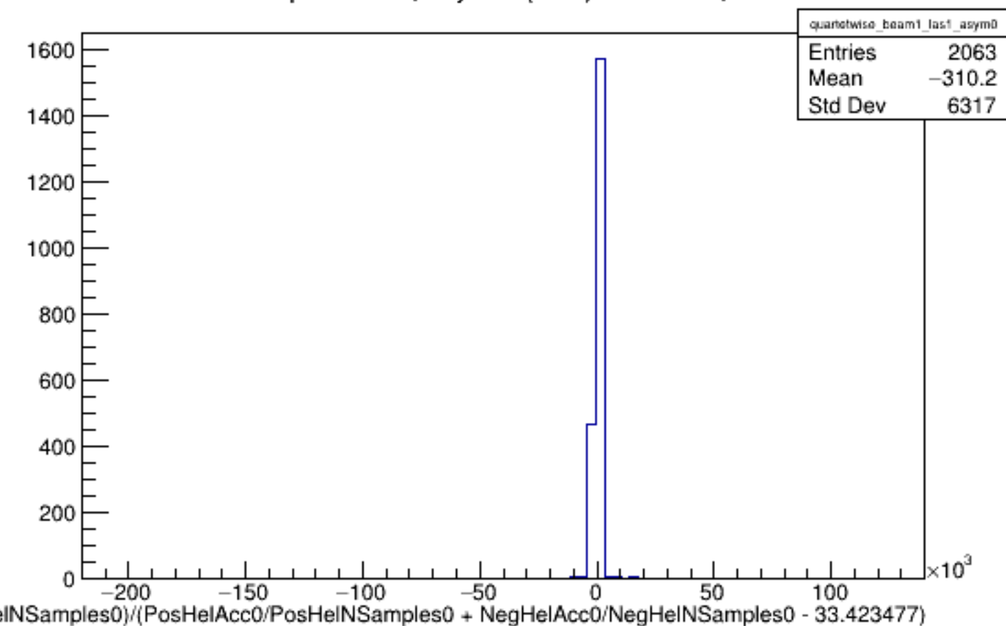
Run 5120 quartetwise, Asyms0 (Raw): Beam ON, Laser ON
