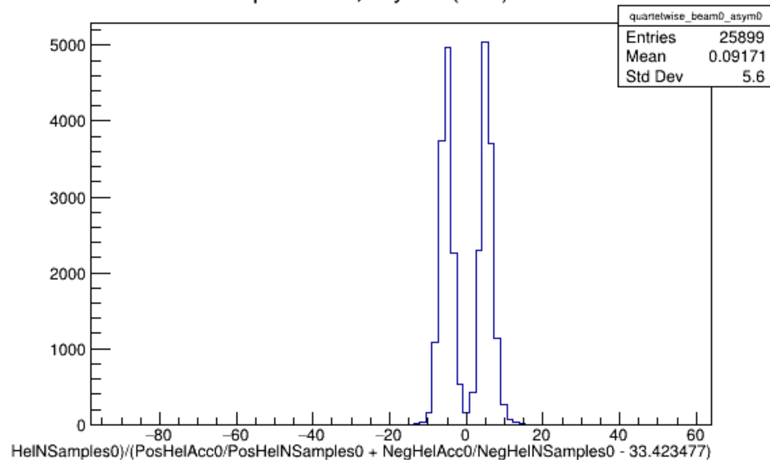
Run 5120 quartetwise, Asyms0 (Raw): Beam OFF
