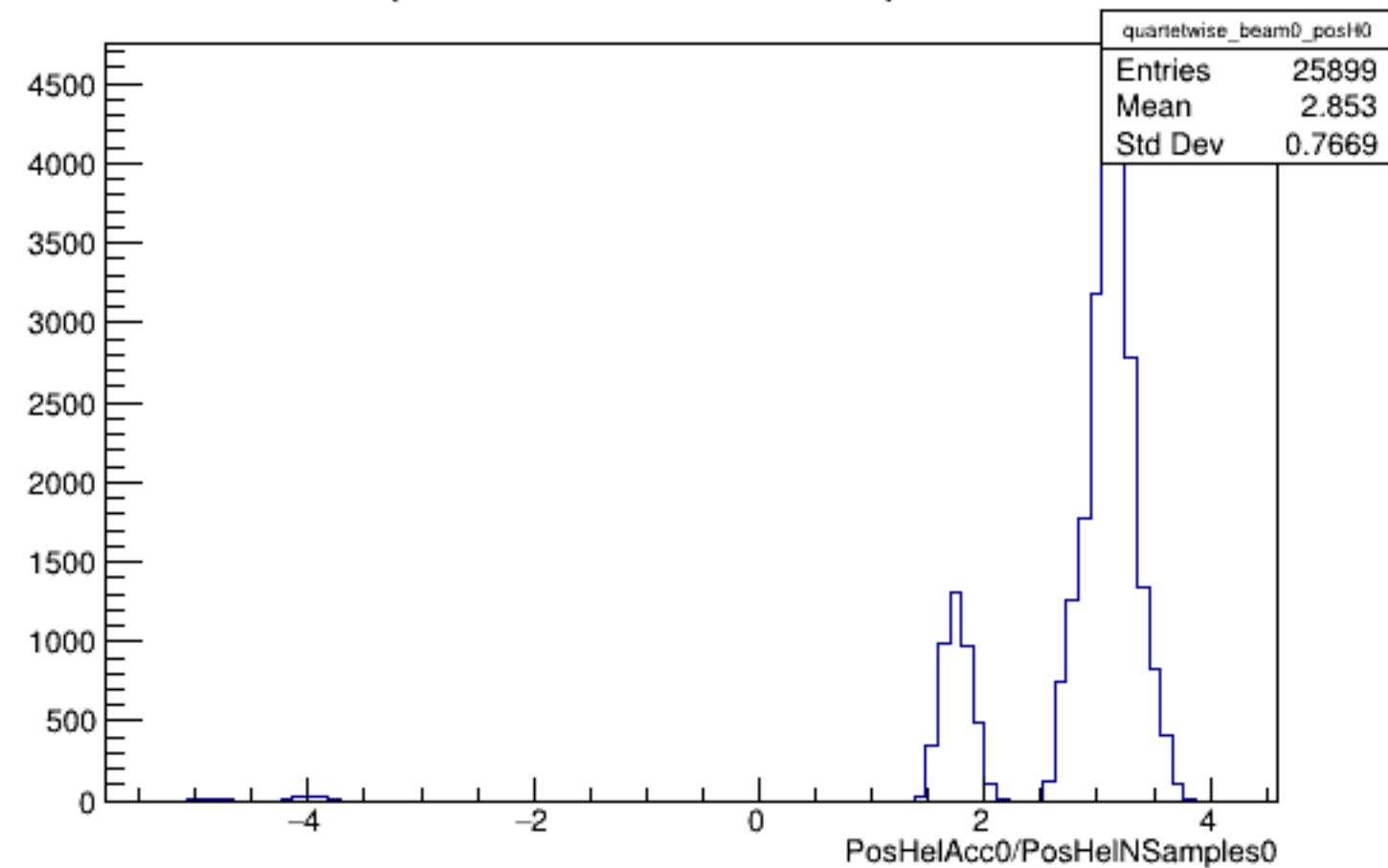
Run 5120 quartetwise, PosHelAcc0/NSamples0: Beam OFF
