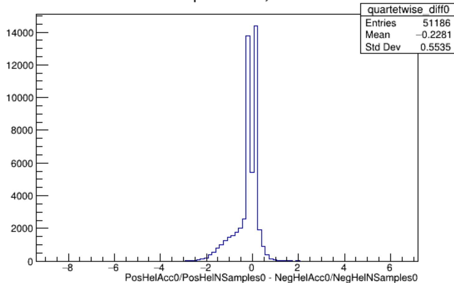
Run 5120 quartetwise, Diffs0: All
