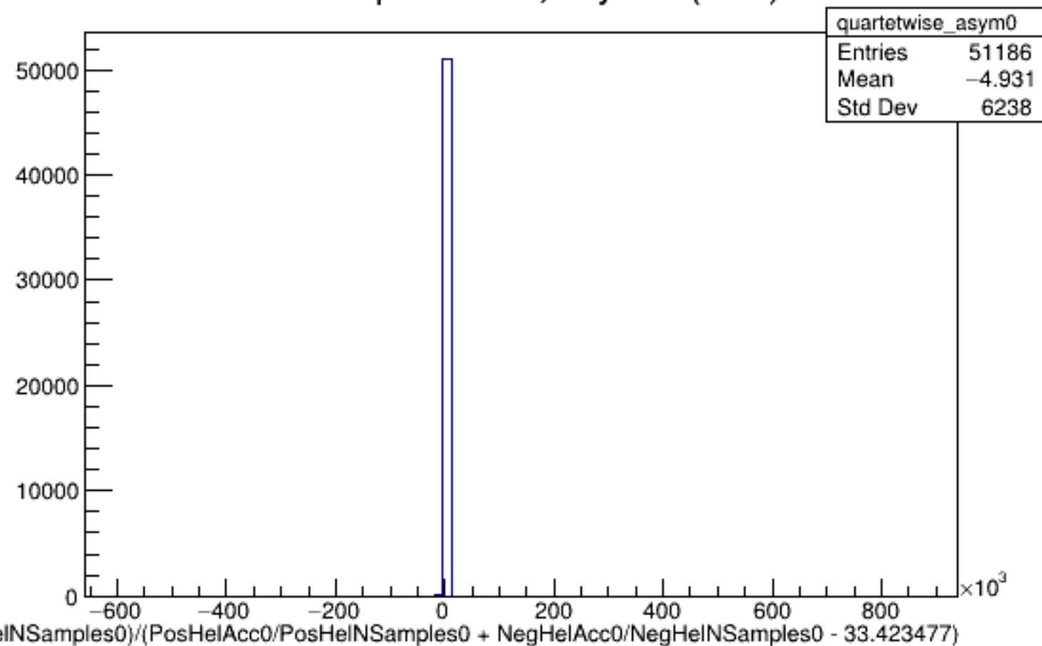
Run 5120 quartetwise, Asyms0 (Raw): All
