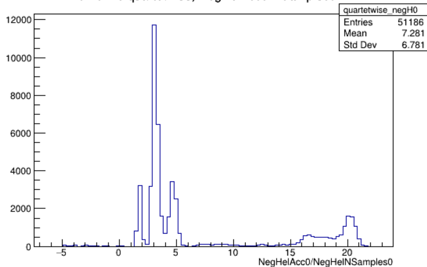
Run 5120 quartetwise, NegHelAcc0/NSamples0: All
