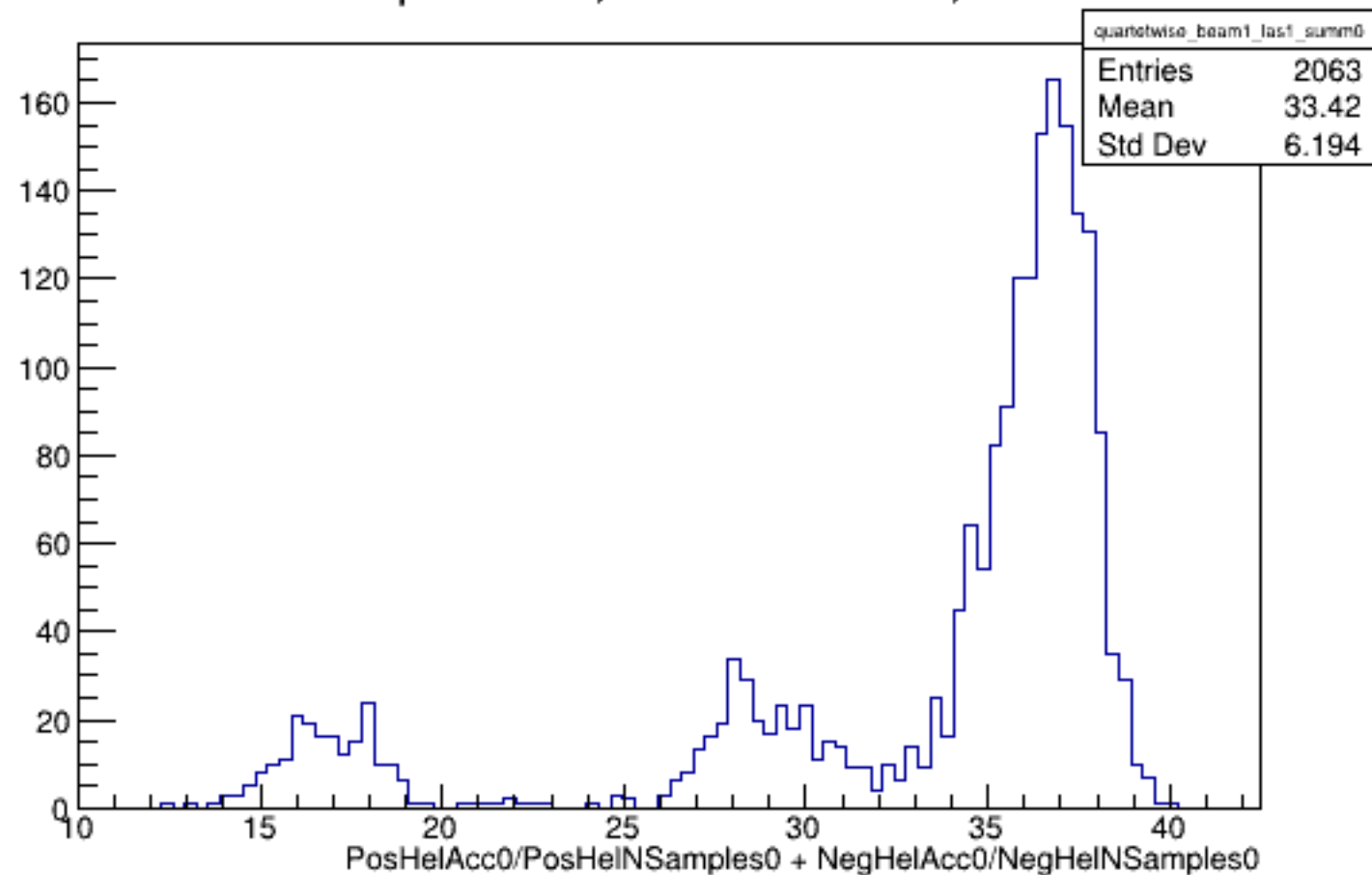
Run 5120 quartetwise, Sums0: Beam ON, Laser ON
