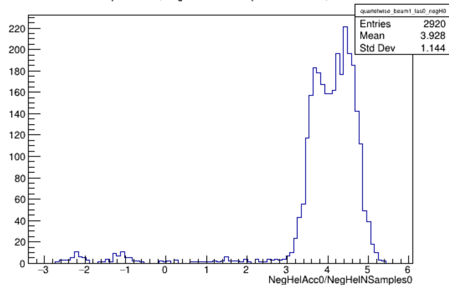
Run 5120 quartetwise, NegHelAcc0/NSamples0: Beam ON, Laser OFF
