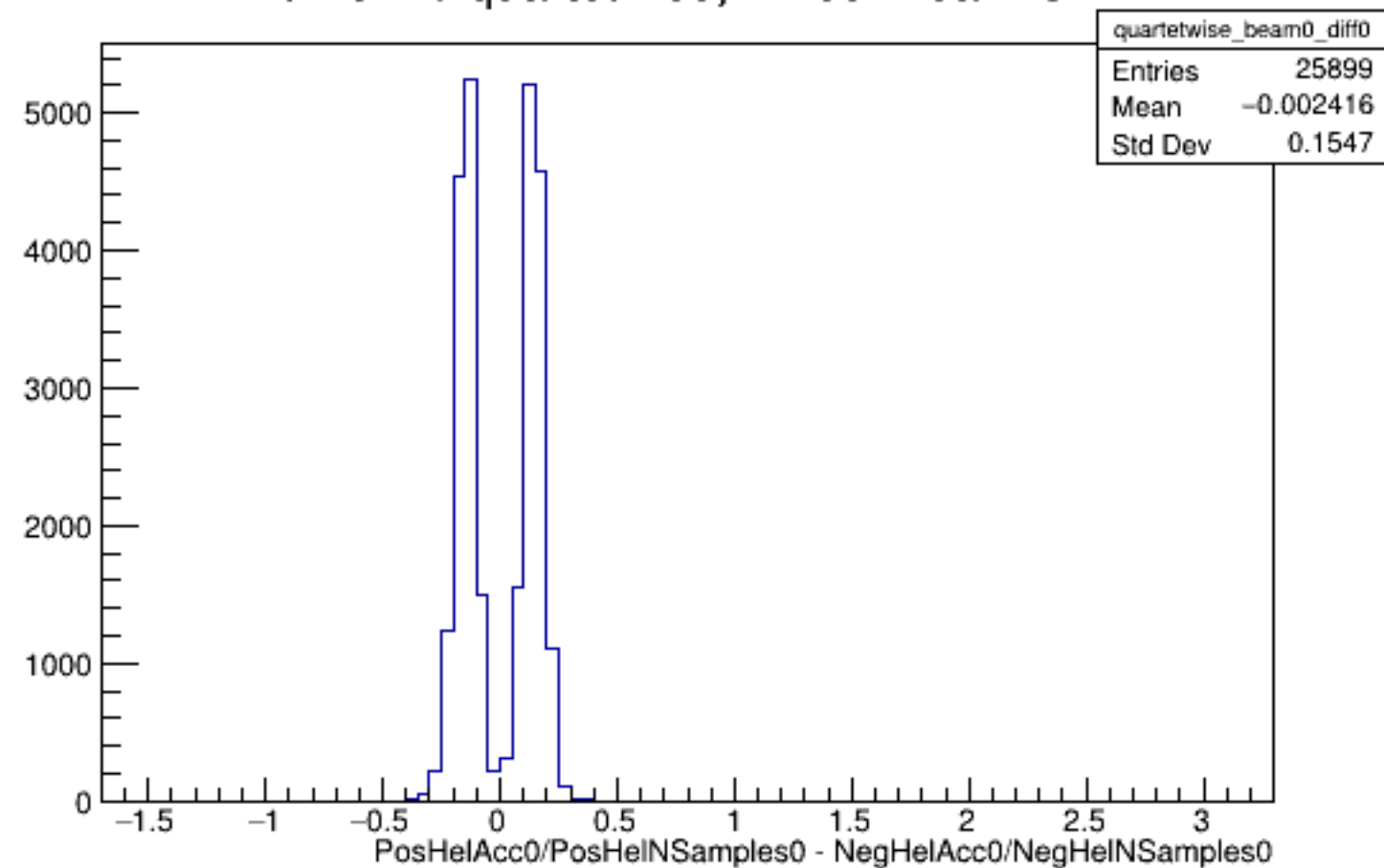
Run 5120 quartetwise, Diffs0: Beam OFF
