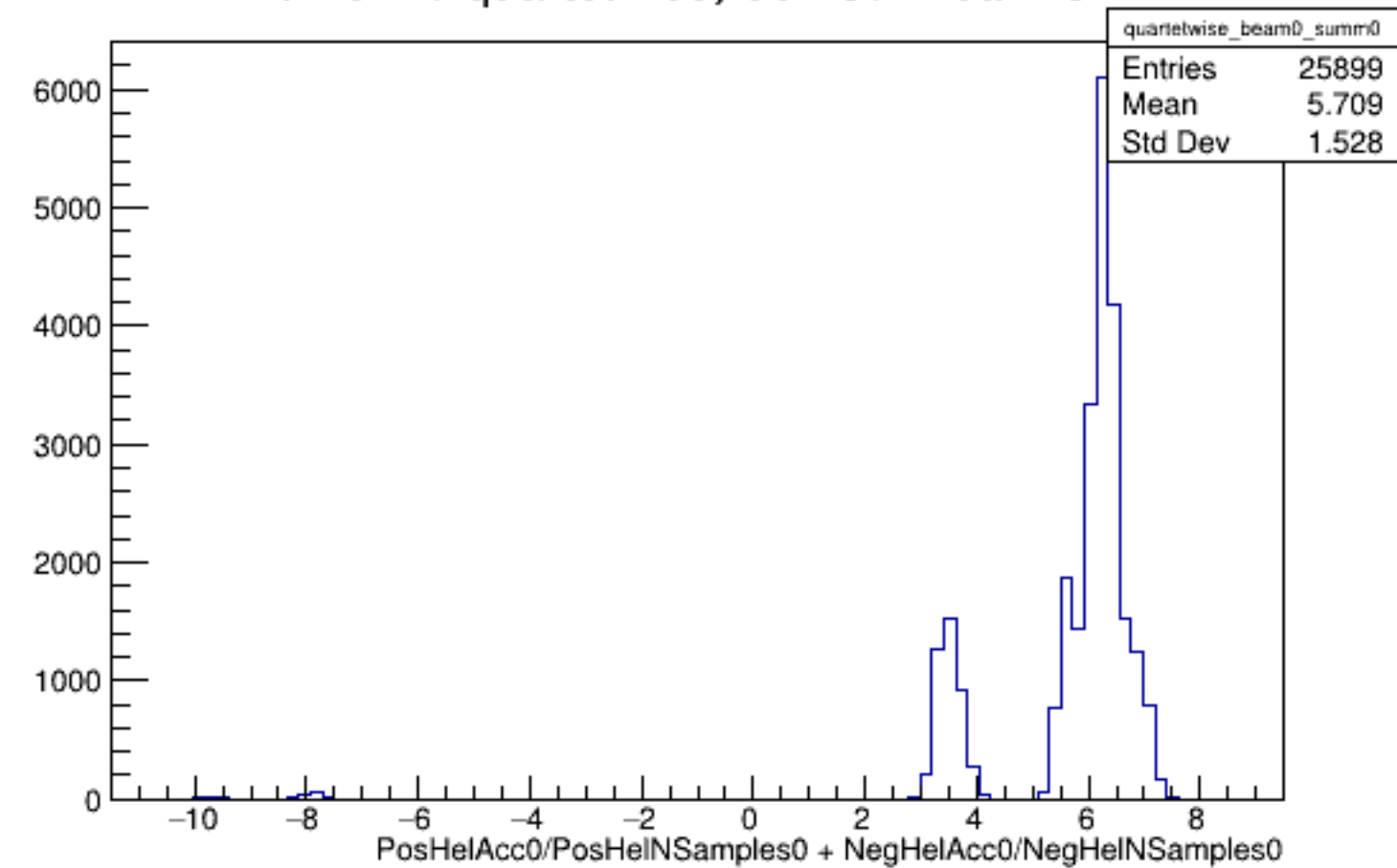
Run 5120 quartetwise, Sums0: Beam OFF
