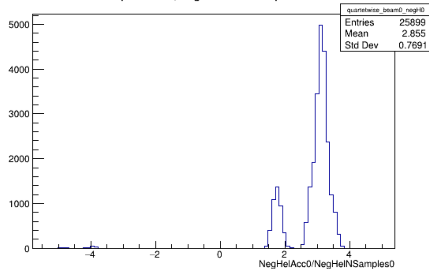
Run 5120 quartetwise, NegHelAcc0/NSamples0: Beam OFF
