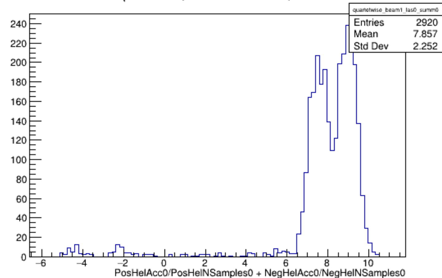
Run 5120 quartetwise, Sums0: Beam ON, Laser OFF
