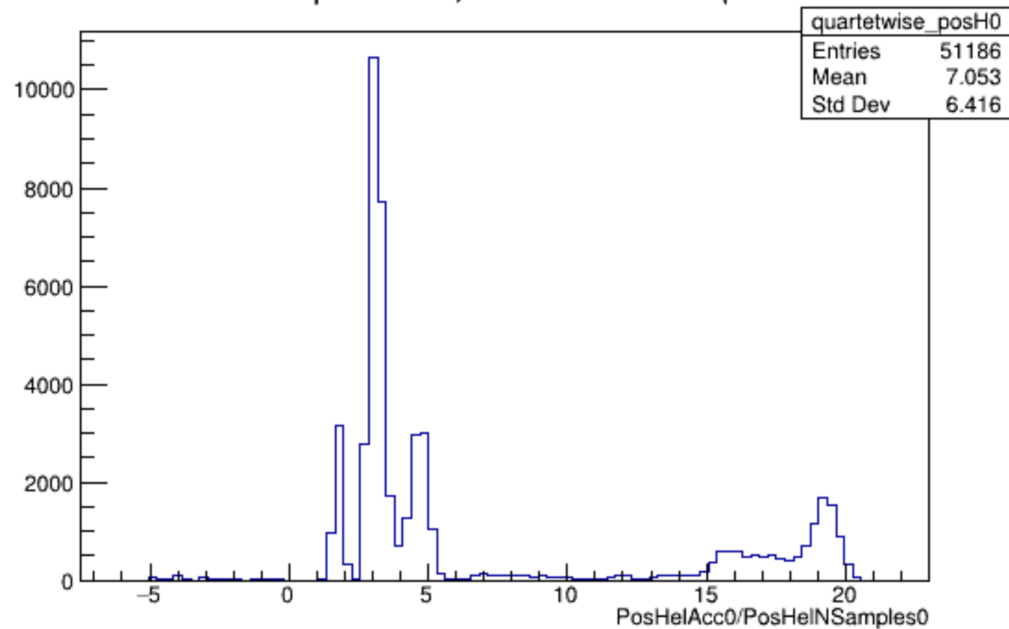
Run 5120 quartetwise, PosHelAcc0/NSamples0: All
