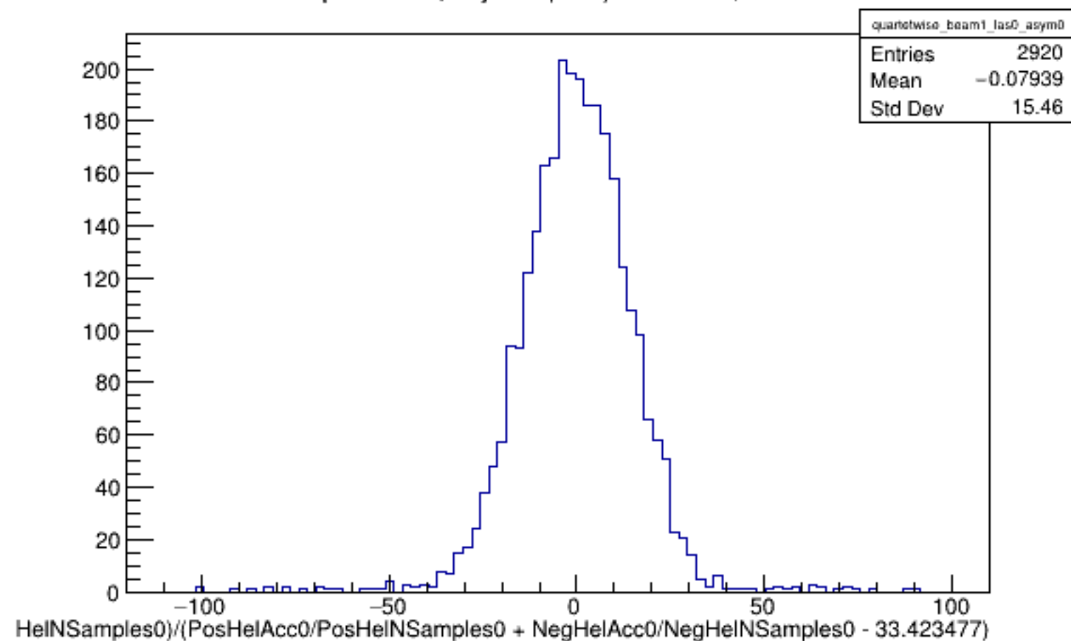
Run 5120 quartetwise, Asyms0 (Raw): Beam ON, Laser OFF
