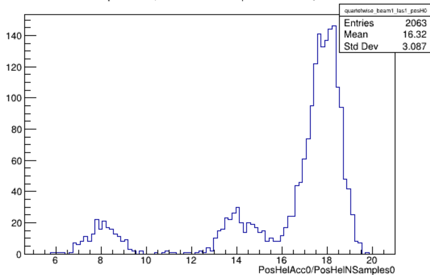
Run 5120 quartetwise, PosHelAcc0/NSamples0: Beam ON, Laser ON
