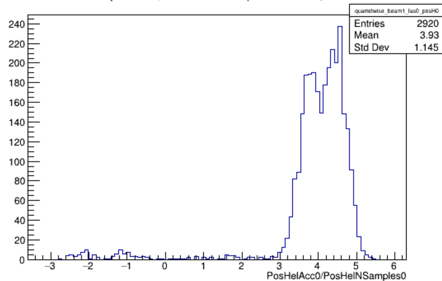
Run 5120 quartetwise, PosHelAcc0/NSamples0: Beam ON, Laser OFF
