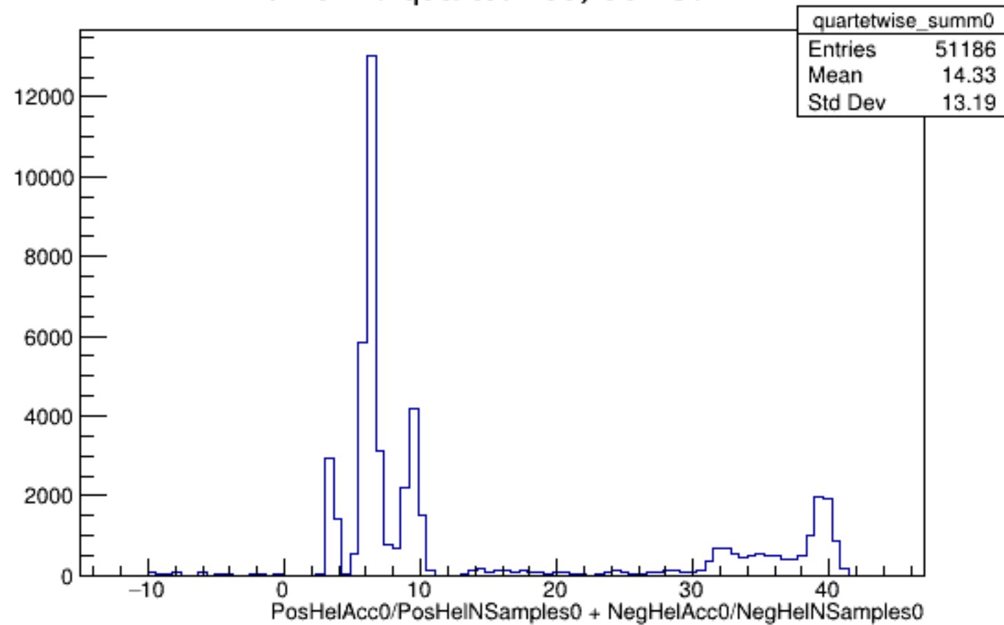
Run 5120 quartetwise, Sums0: All
