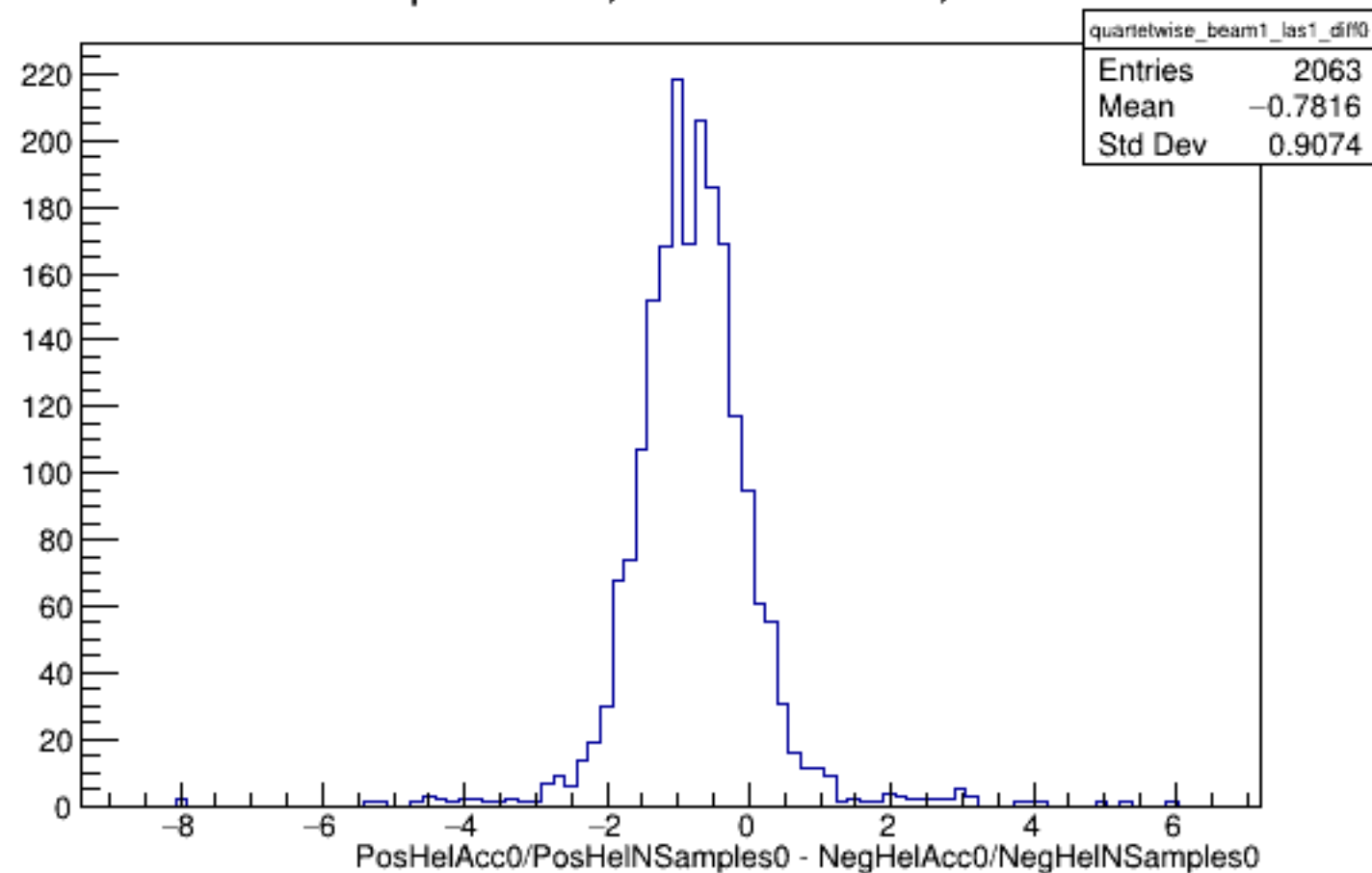
Run 5120 quartetwise, Diffs0: Beam ON, Laser ON
