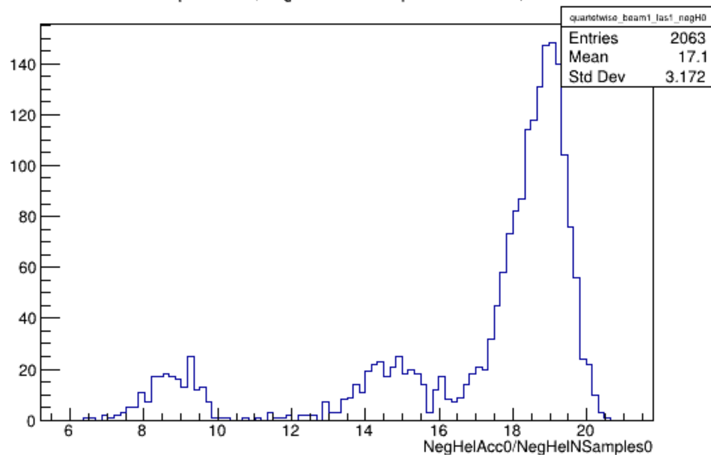
Run 5120 quartetwise, NegHelAcc0/NSamples0: Beam ON, Laser ON
