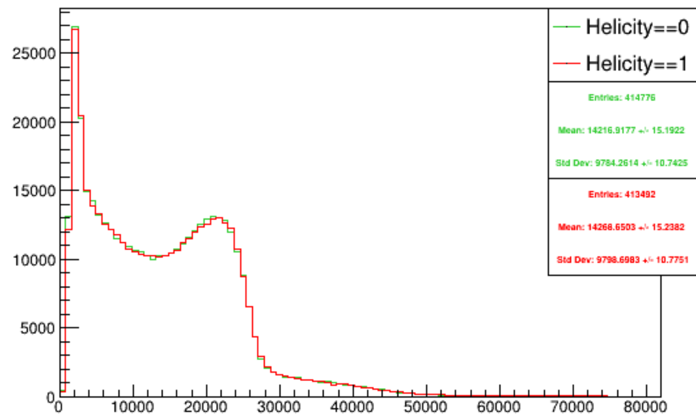
Run 5129 triggerwise, sums: Beam ON, Laser ON
