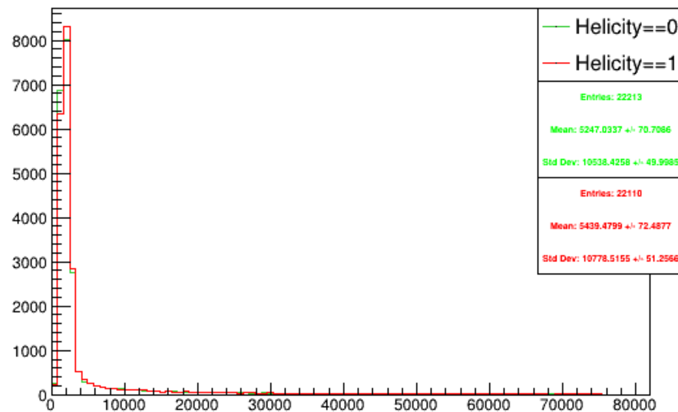
Run 5129 triggerwise, sums: Beam ON, Laser OFF
