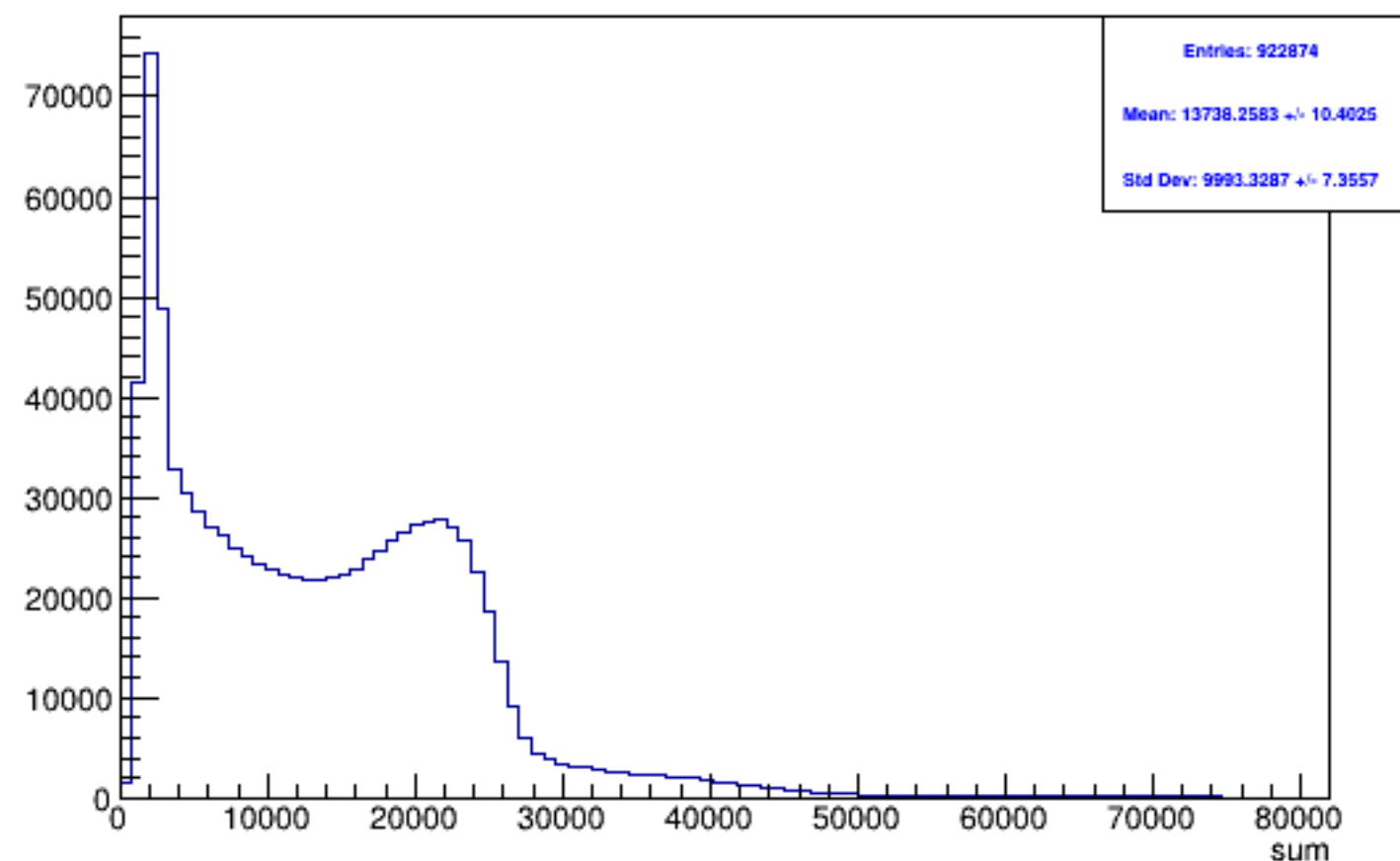
Run 5129 triggerwise, sums: All
