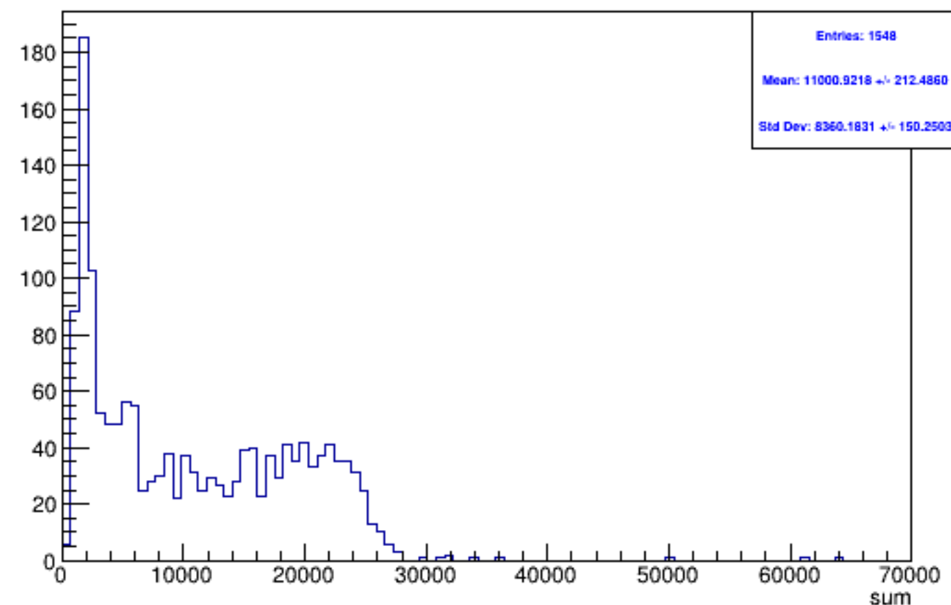
Run 5129 triggerwise, sums: Beam OFF
