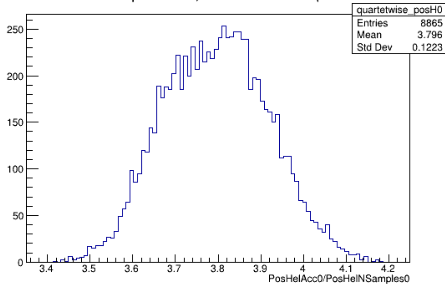
Run 5132 quartetwise, PosHelAcc0/NSamples0: All
