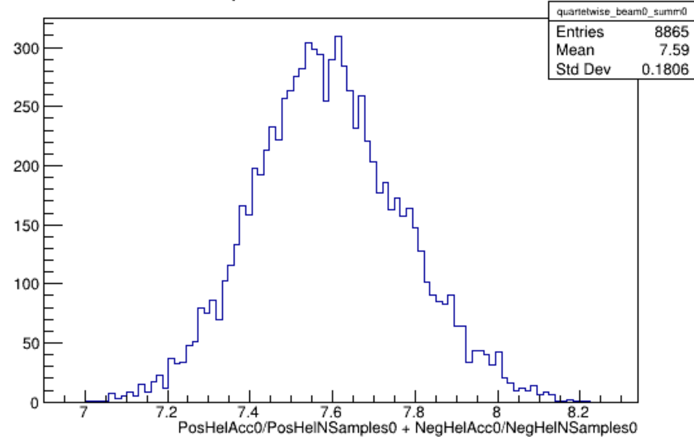
Run 5132 quartetwise, Sums0: Beam OFF
