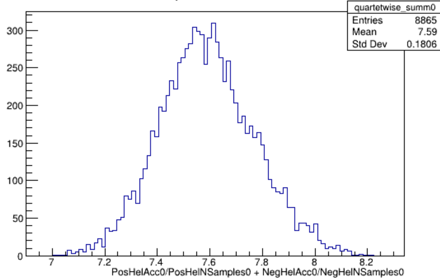
Run 5132 quartetwise, Sums0: All
