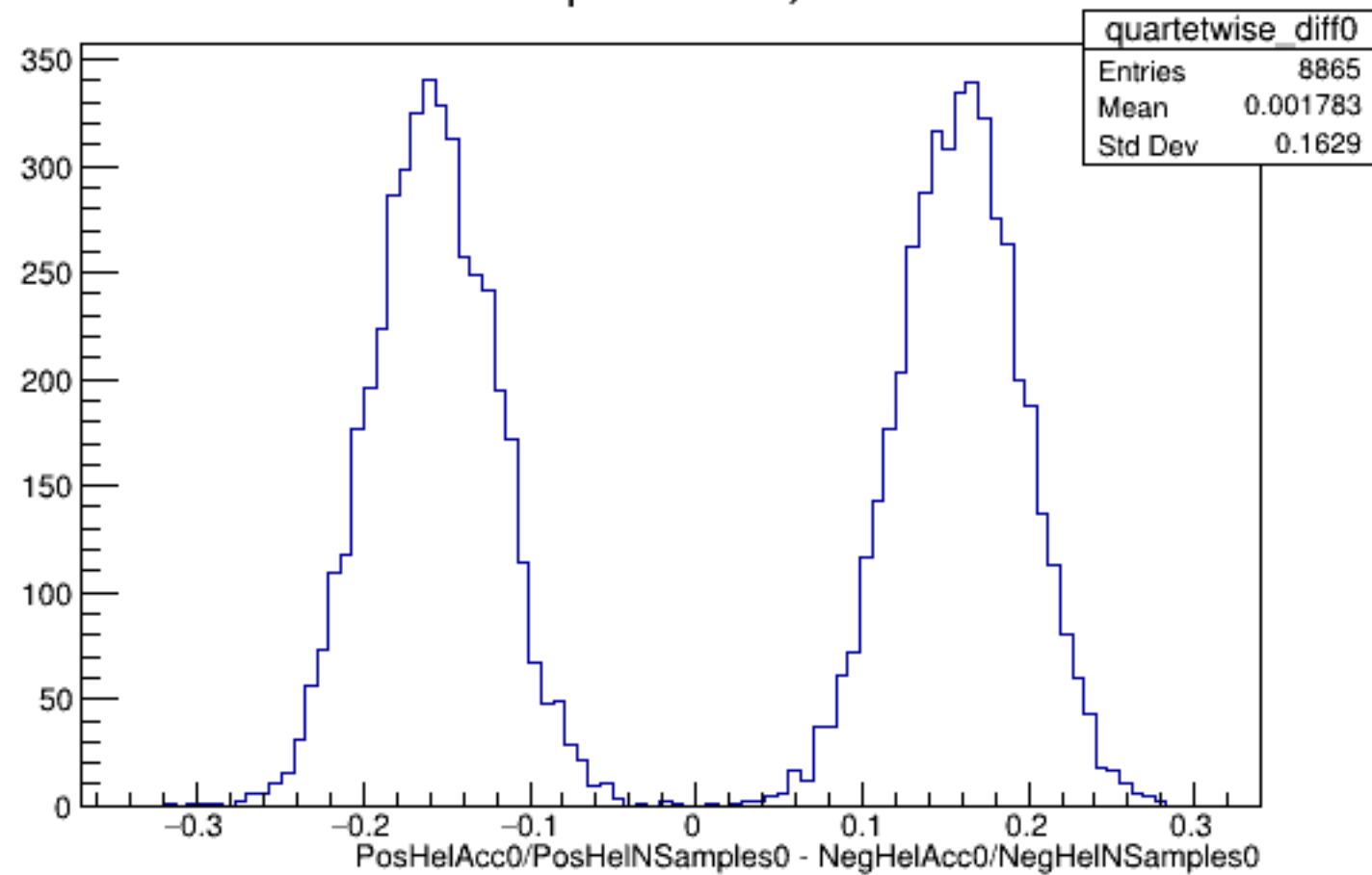
Run 5132 quartetwise, Diffs0: All
