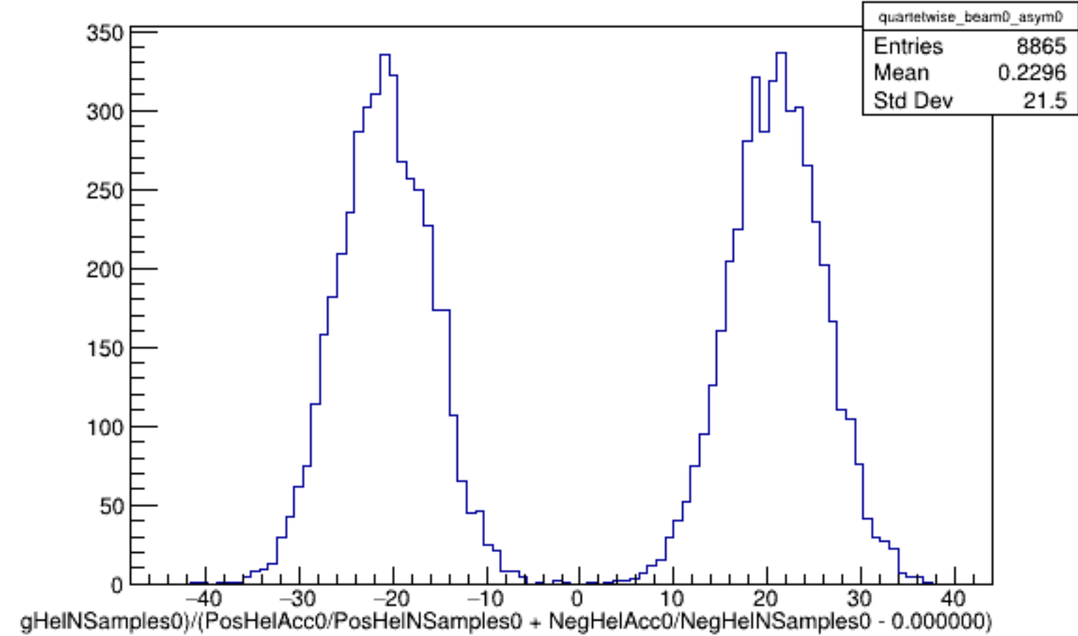
Run 5132 quartetwise, Asyms0 (Raw): Beam OFF
