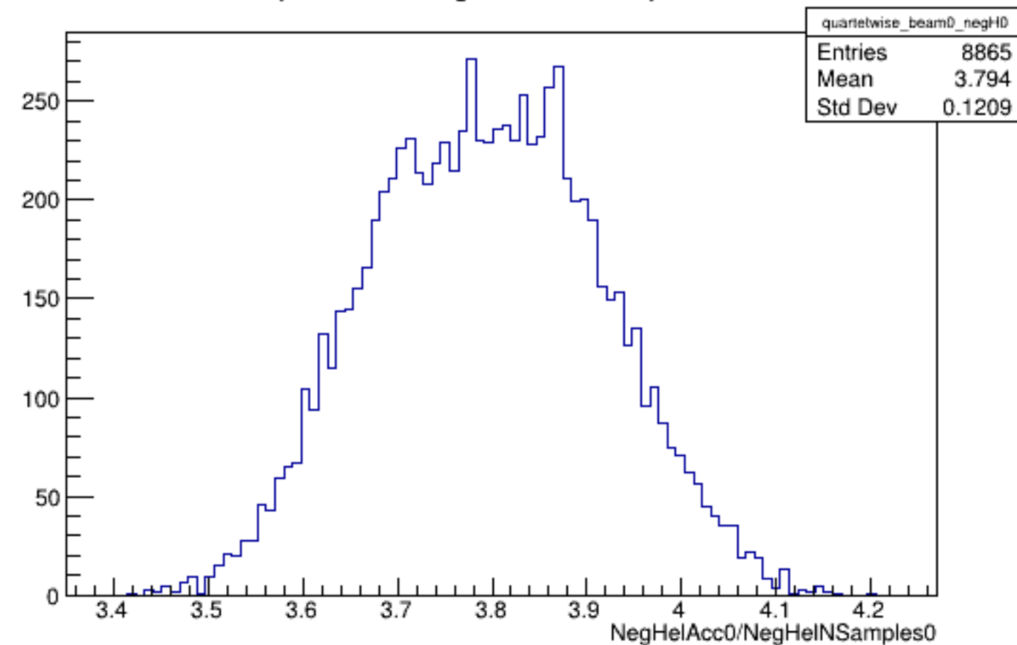
Run 5132 quartetwise, NegHelAcc0/NSamples0: Beam OFF
