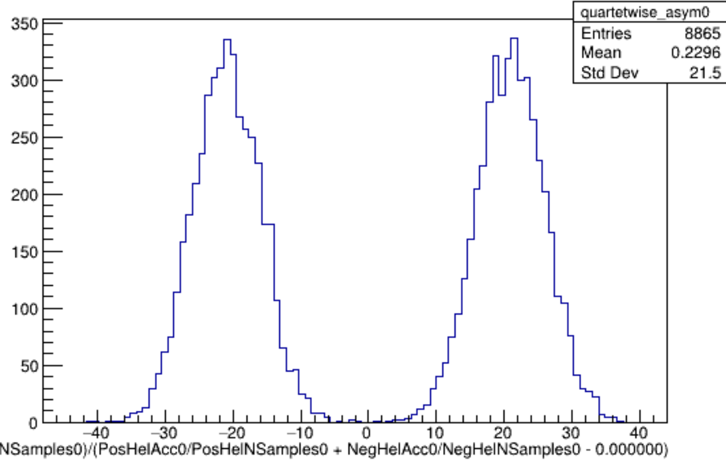
Run 5132 quartetwise, Asyms0 (Raw): All
