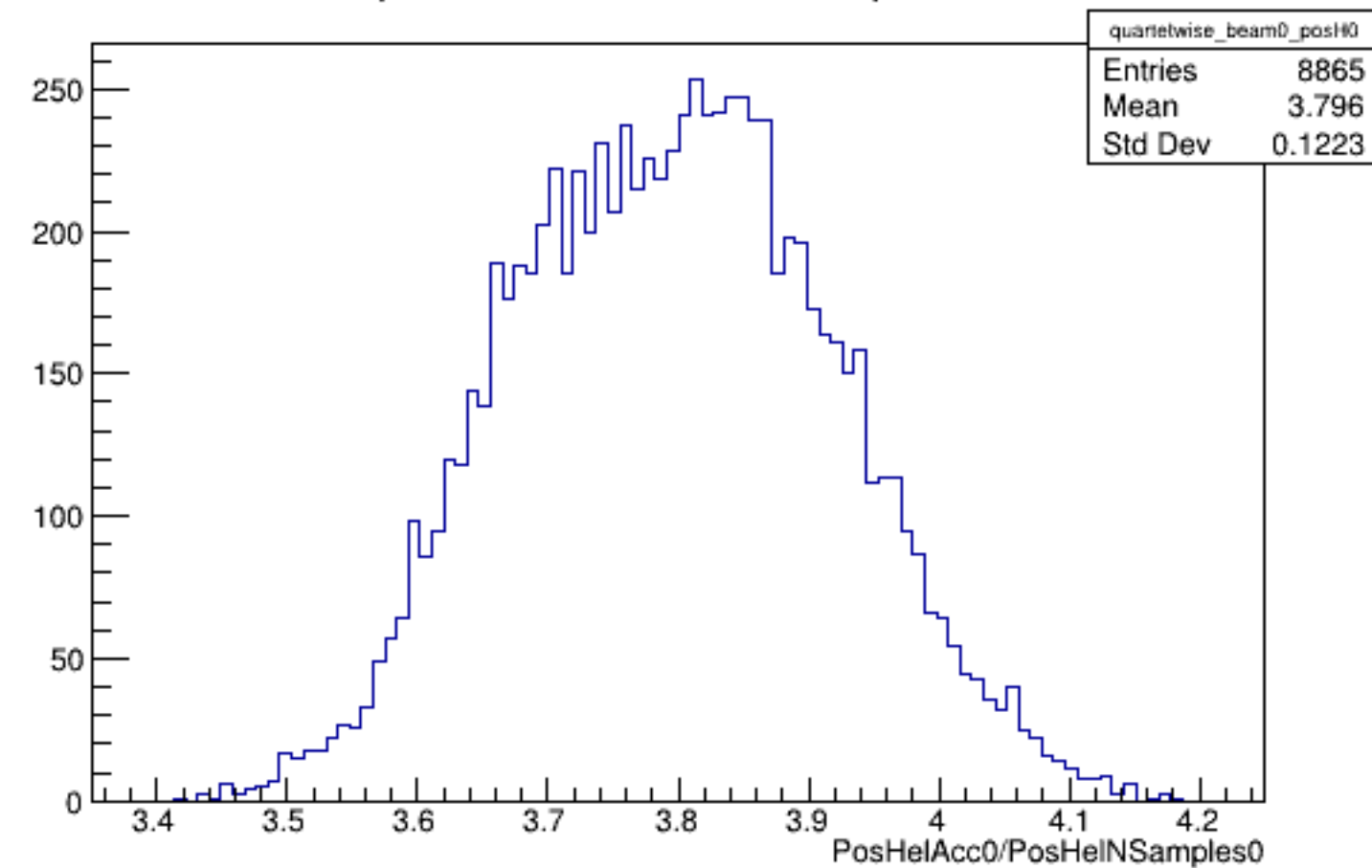
Run 5132 quartetwise, PosHelAcc0/NSamples0: Beam OFF
