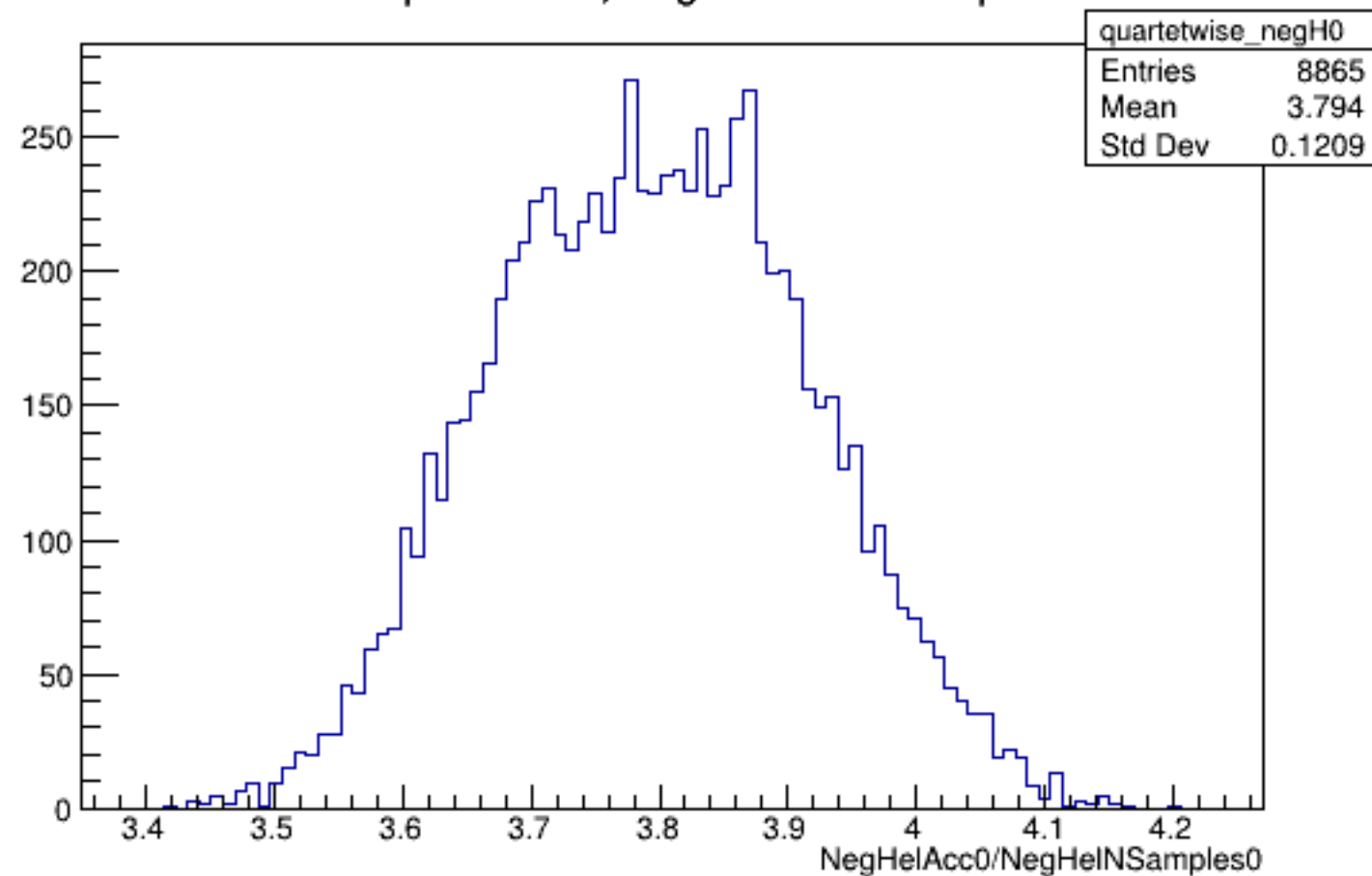
Run 5132 quartetwise, NegHelAcc0/NSamples0: All
