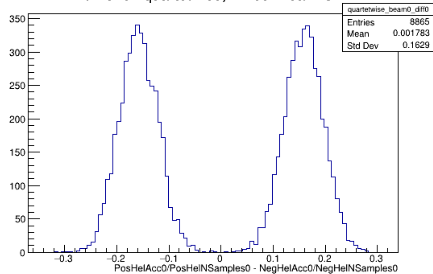
Run 5132 quartetwise, Diffs0: Beam OFF
