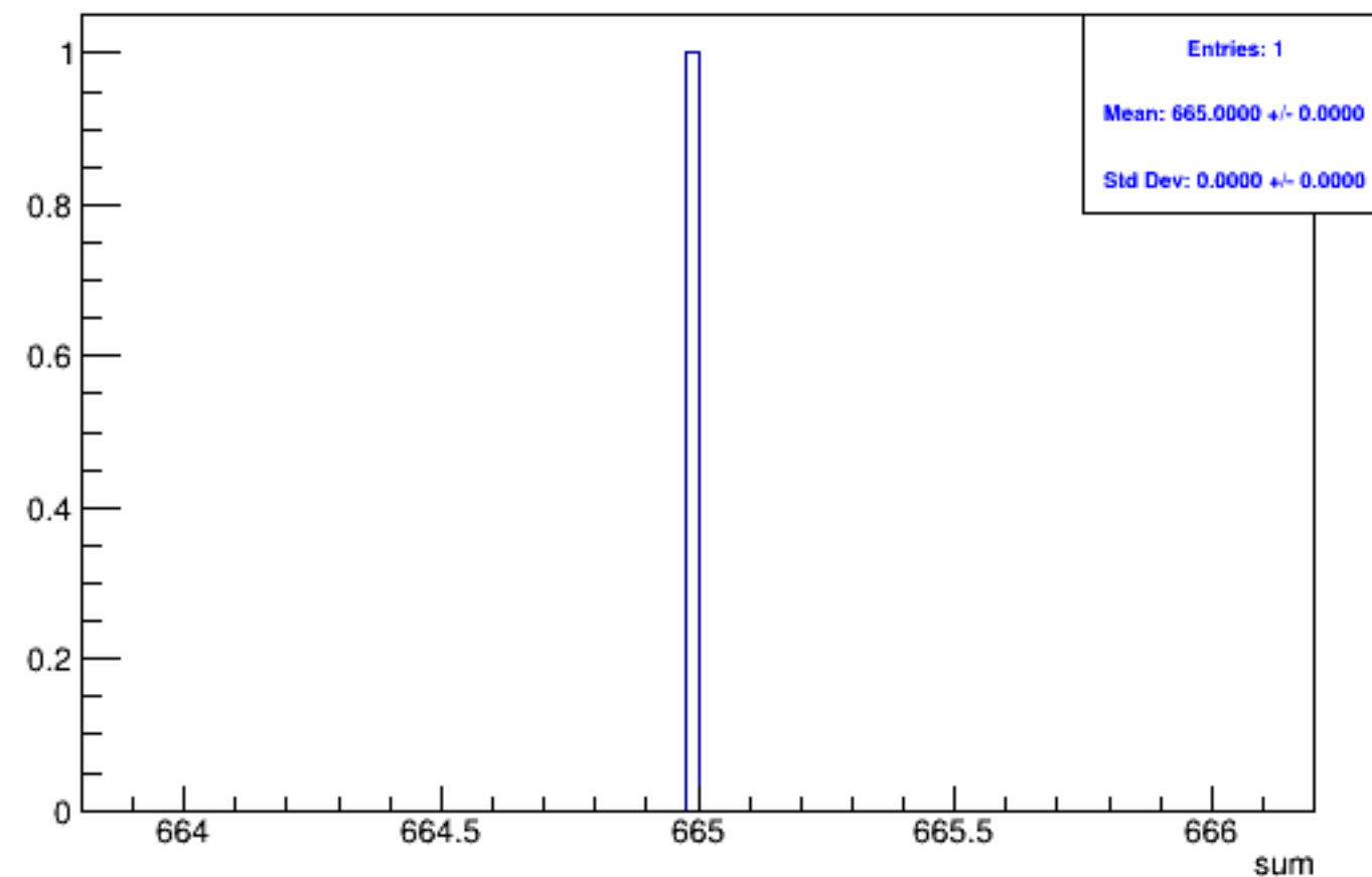
Run 5137 triggerwise, sums: Beam OFF
