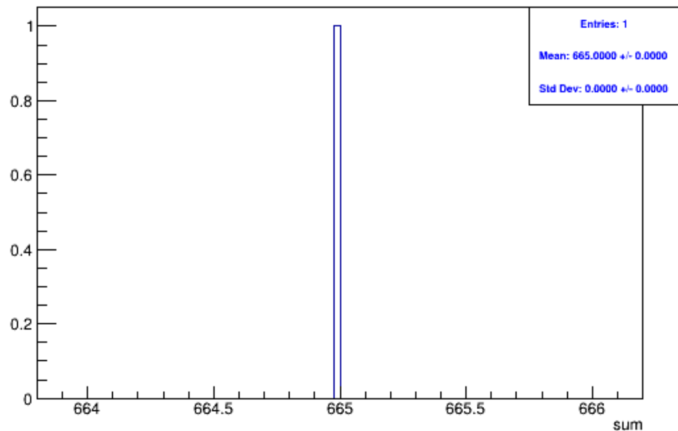
Run 5137 triggerwise, sums: All
