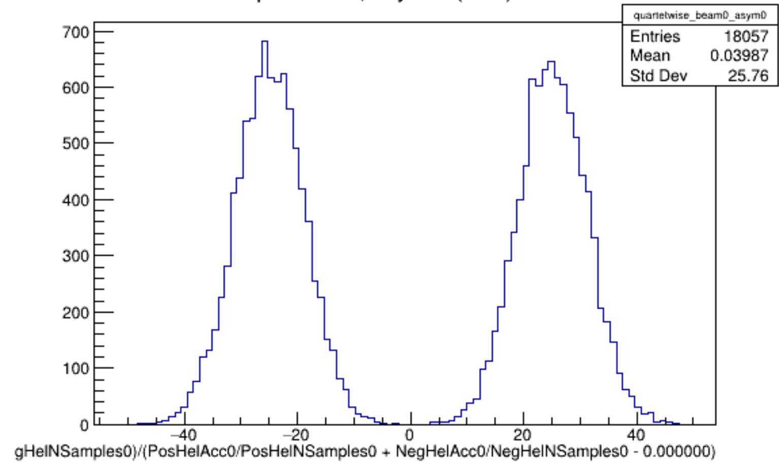
Run 5142 quartetwise, Asyms0 (Raw): Beam OFF
