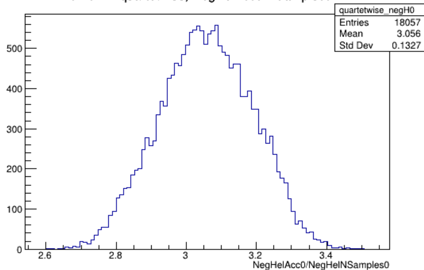
Run 5142 quartetwise, NegHelAcc0/NSamples0: All
