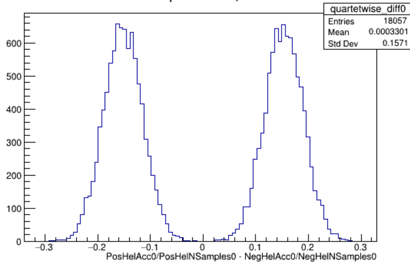
Run 5142 quartetwise, Diffs0: All
