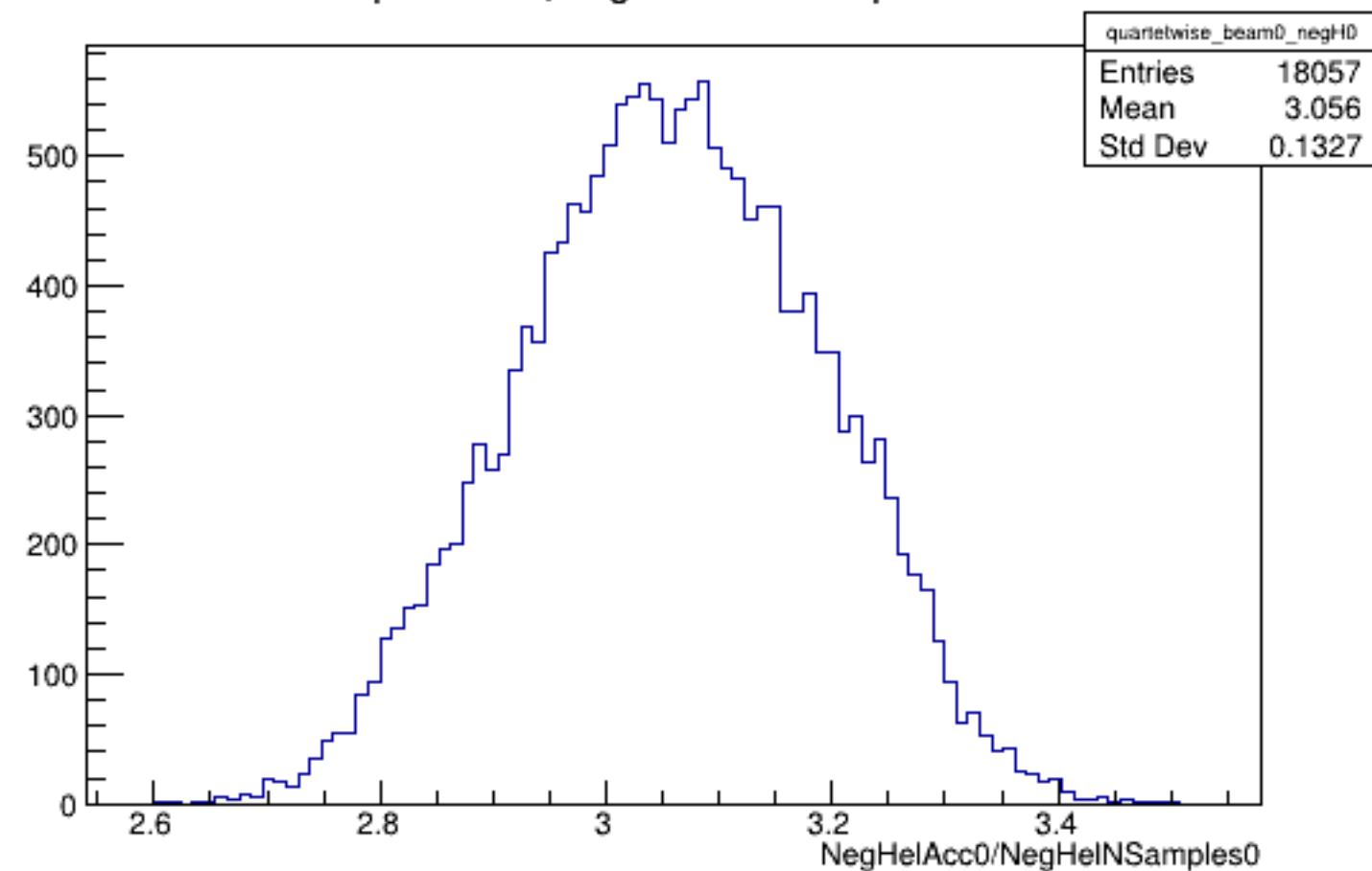
Run 5142 quartetwise, NegHelAcc0/NSamples0: Beam OFF
