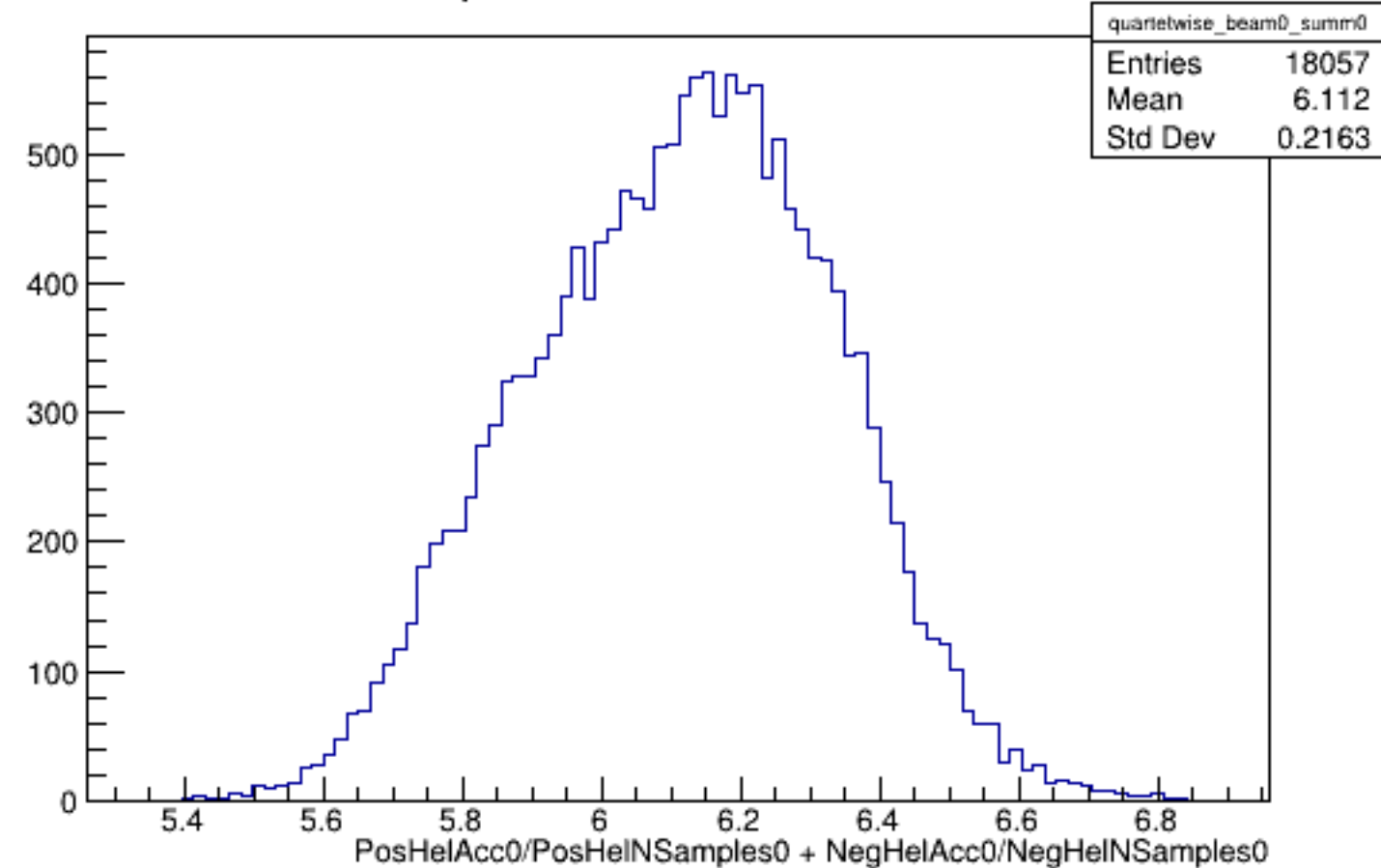
Run 5142 quartetwise, Sums0: Beam OFF
