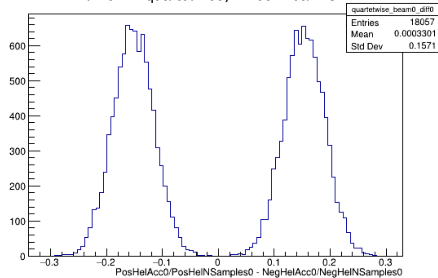
Run 5142 quartetwise, Diffs0: Beam OFF
