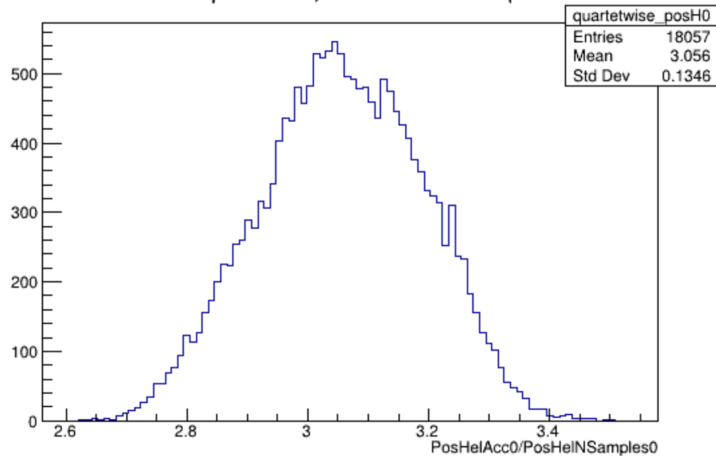
Run 5142 quartetwise, PosHelAcc0/NSamples0: All
