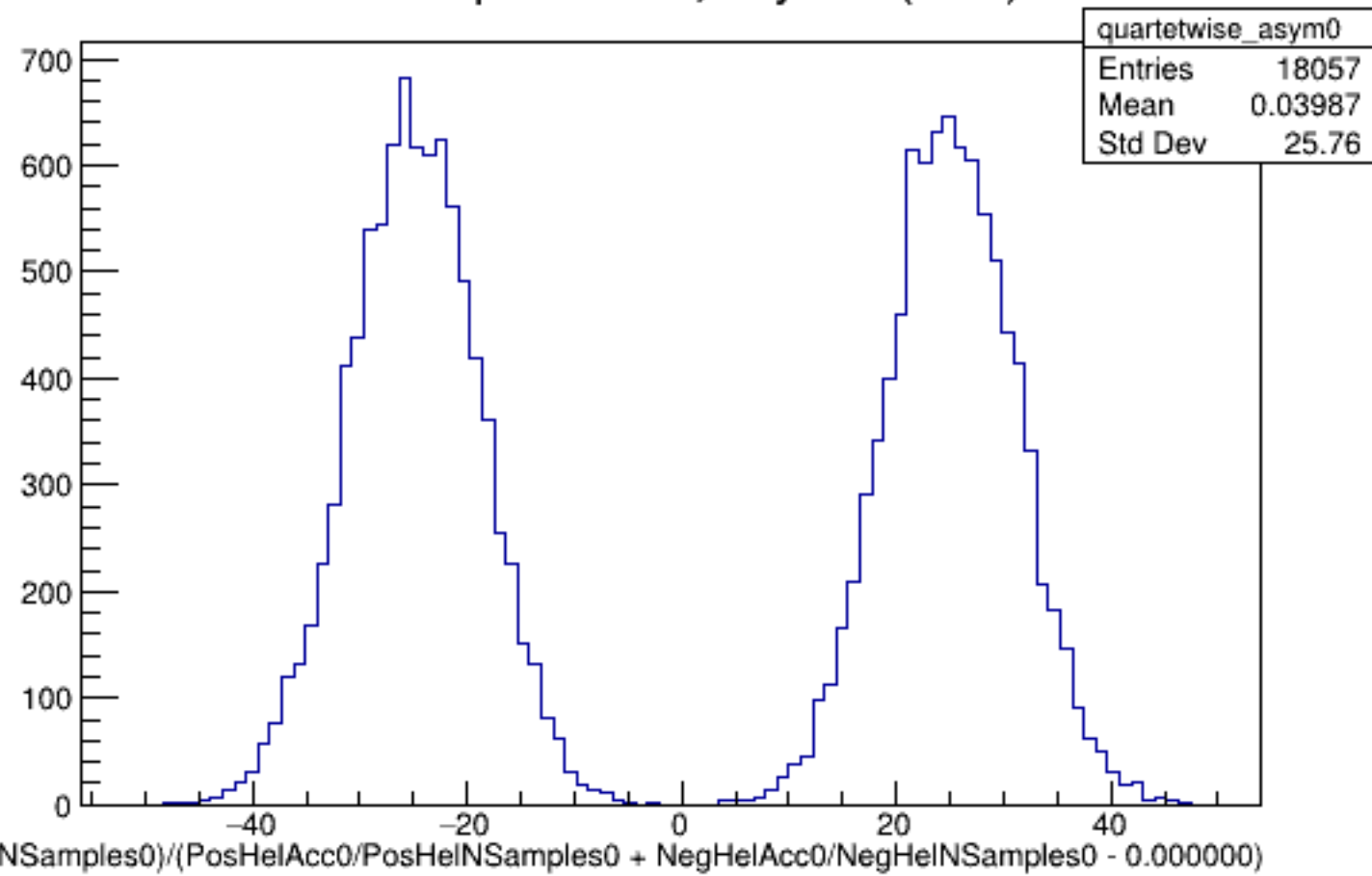
Run 5142 quartetwise, Asyms0 (Raw): All
