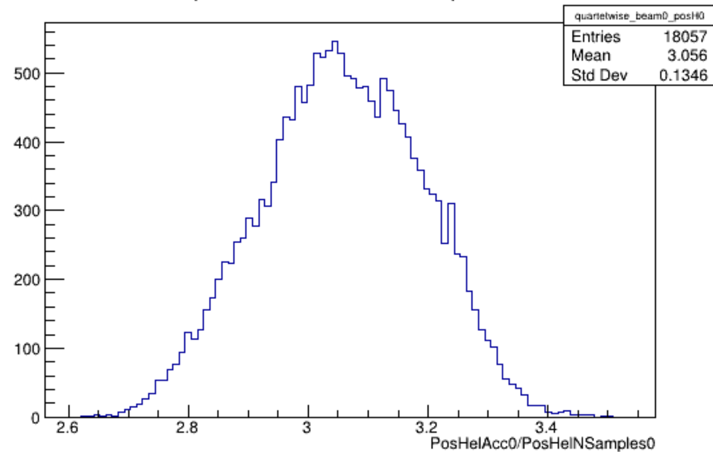
Run 5142 quartetwise, PosHelAcc0/NSamples0: Beam OFF
