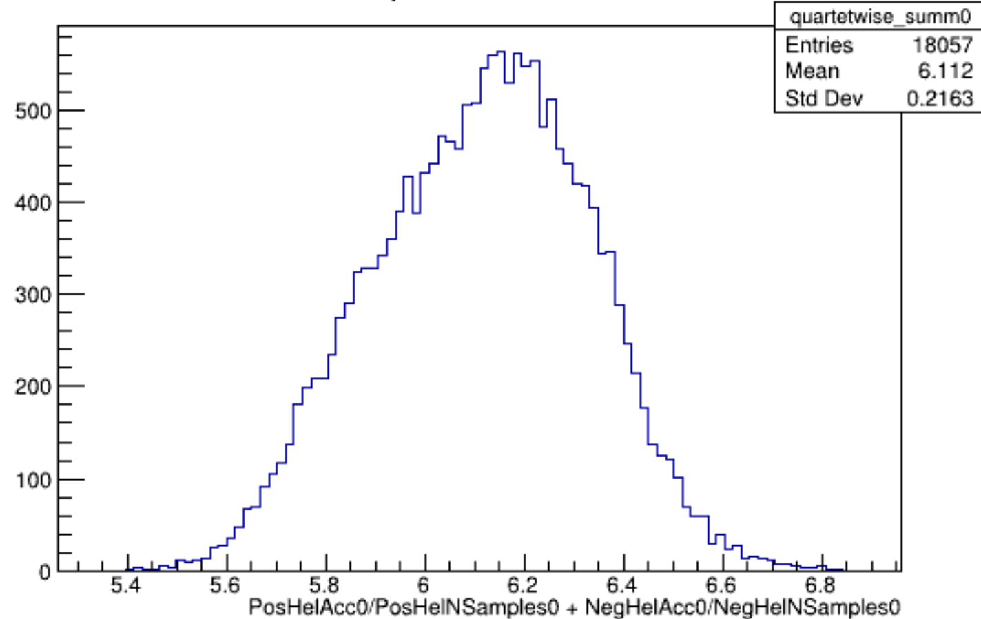
Run 5142 quartetwise, Sums0: All
