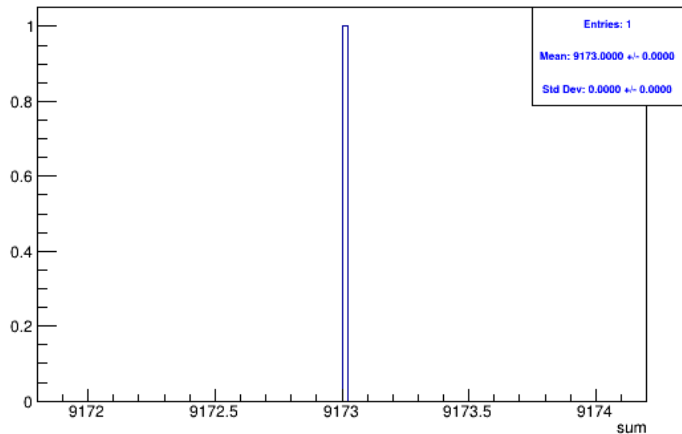
Run 5142 triggerwise, sums: All
