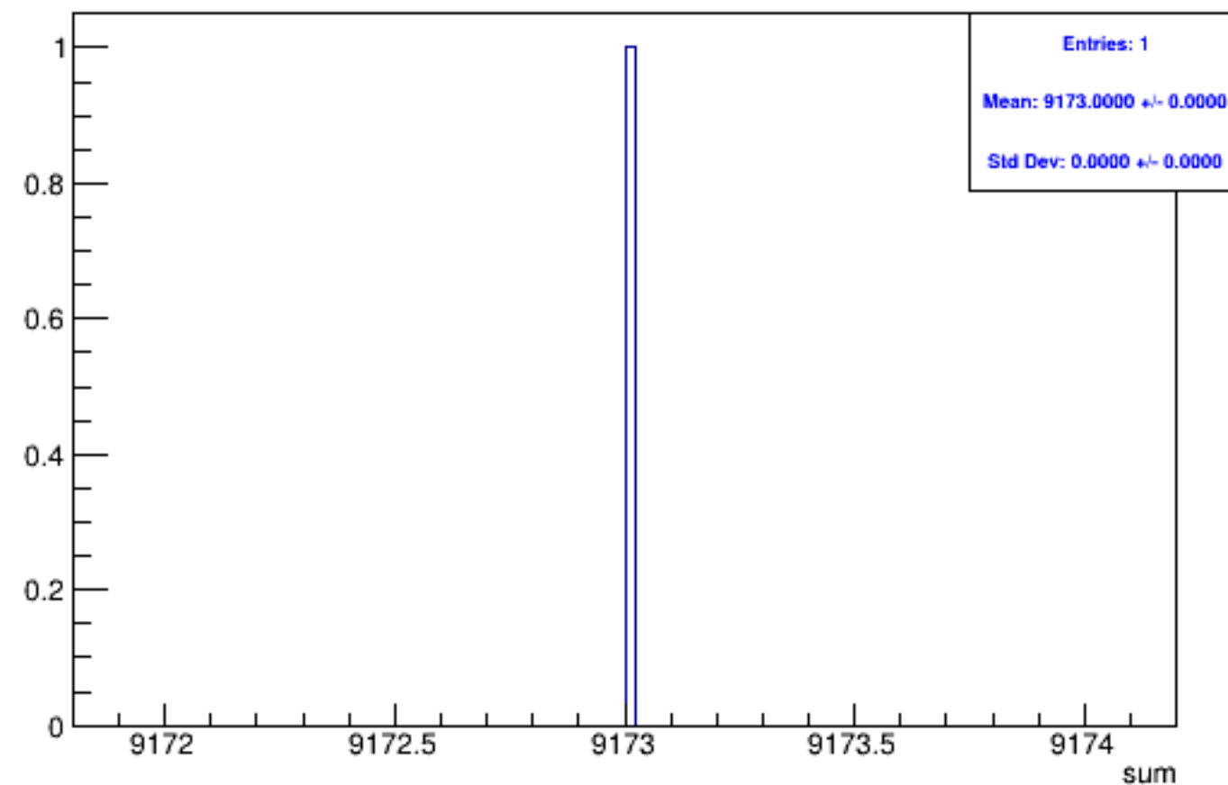
Run 5142 triggerwise, sums: Beam OFF
