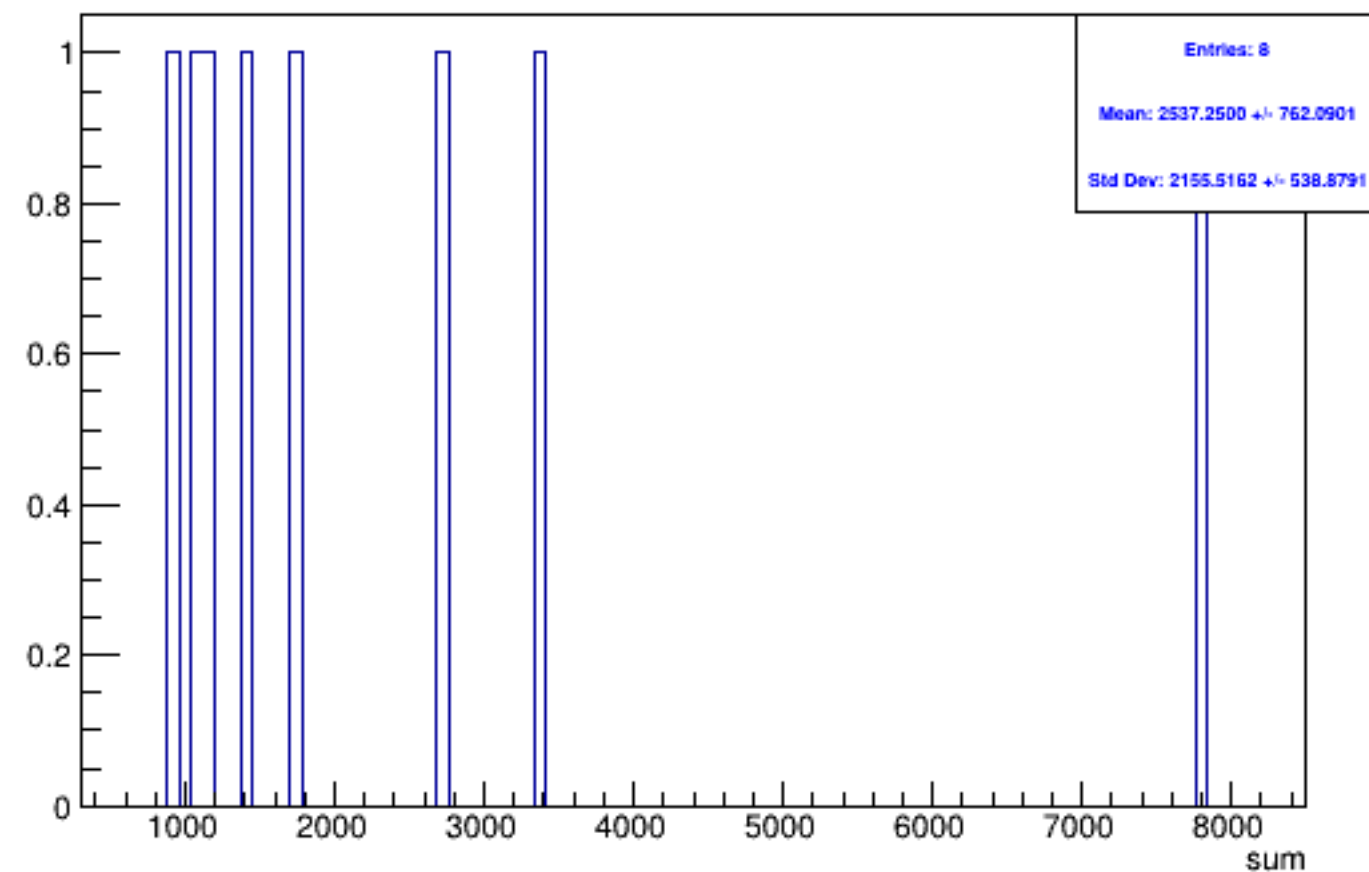
Run 5146 triggerwise, sums: Beam OFF
