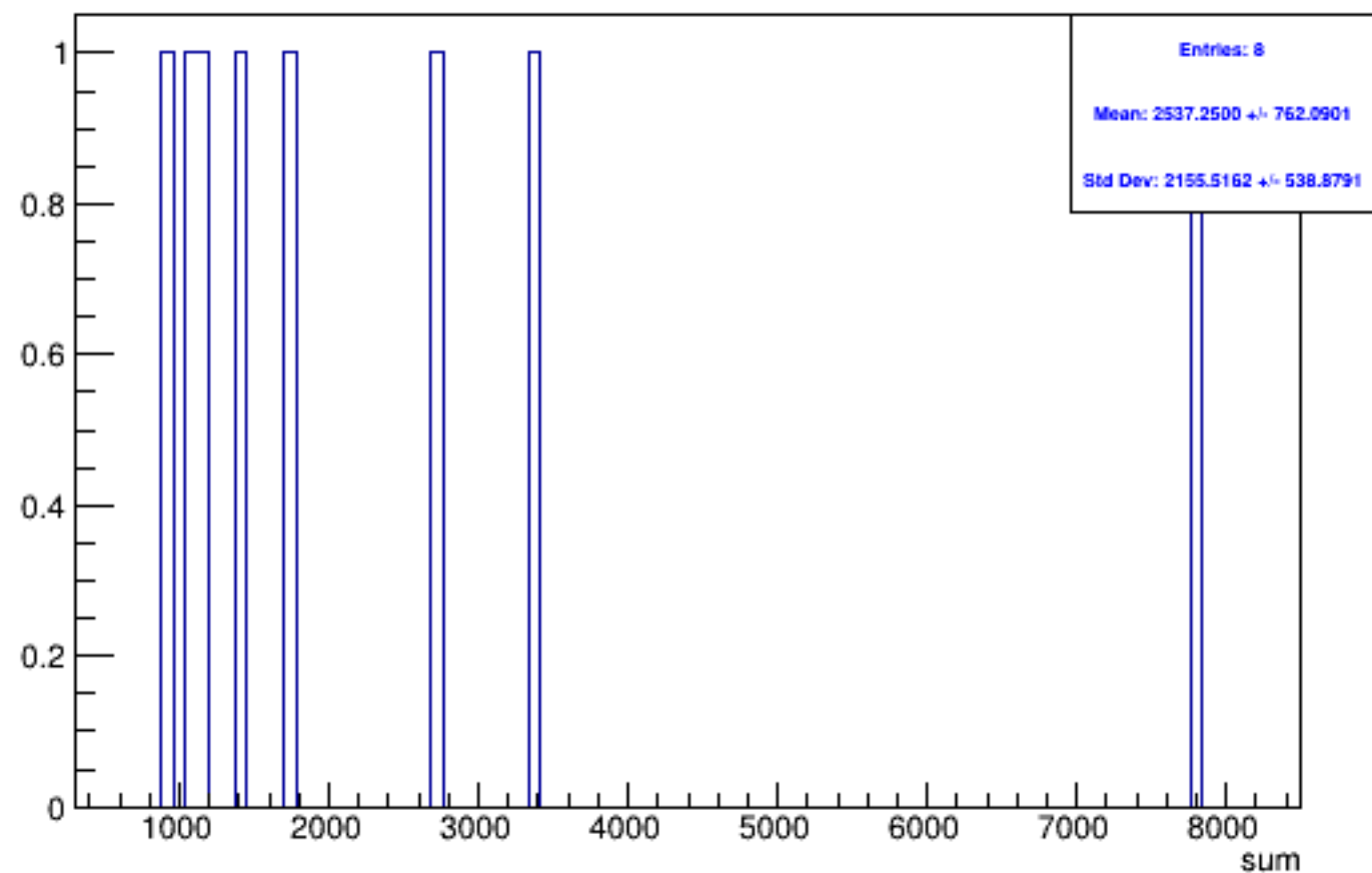
Run 5146 triggerwise, sums: All
