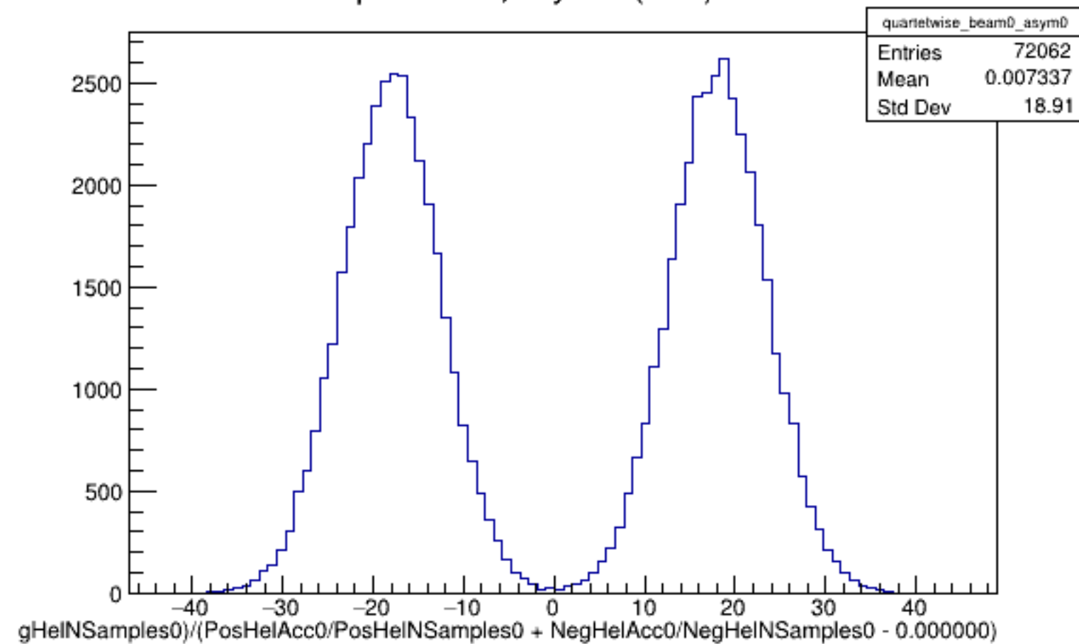
Run 5150 quartetwise, Asyms0 (Raw): Beam OFF
