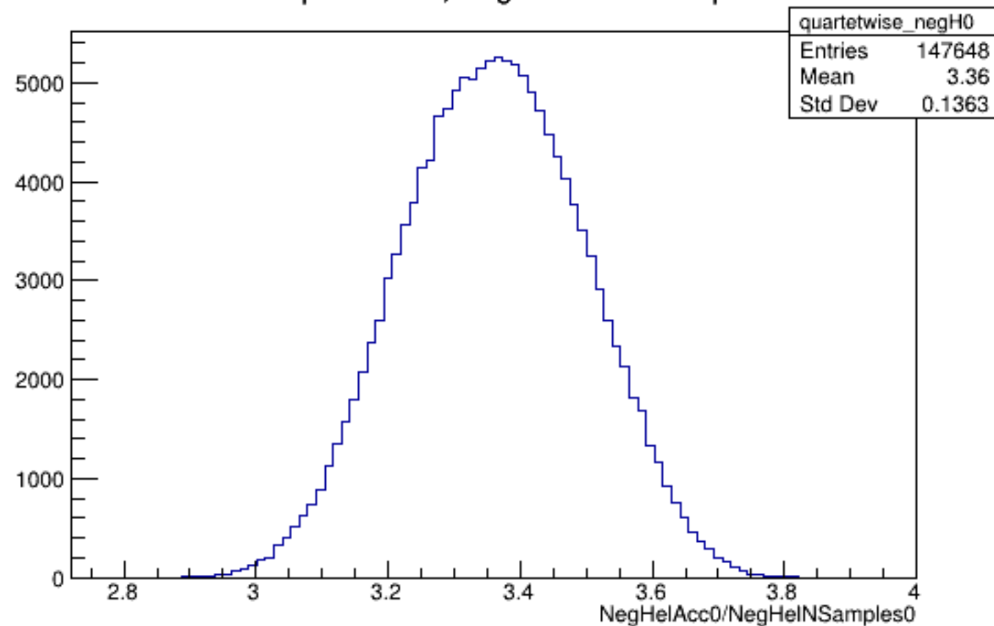
Run 5150 quartetwise, NegHelAcc0/NSamples0: All
