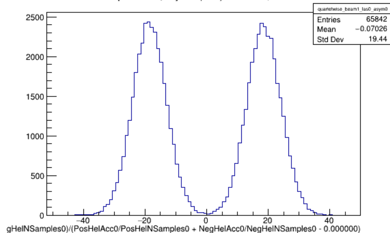
Run 5150 quartetwise, Asyms0 (Raw): Beam ON, Laser OFF
