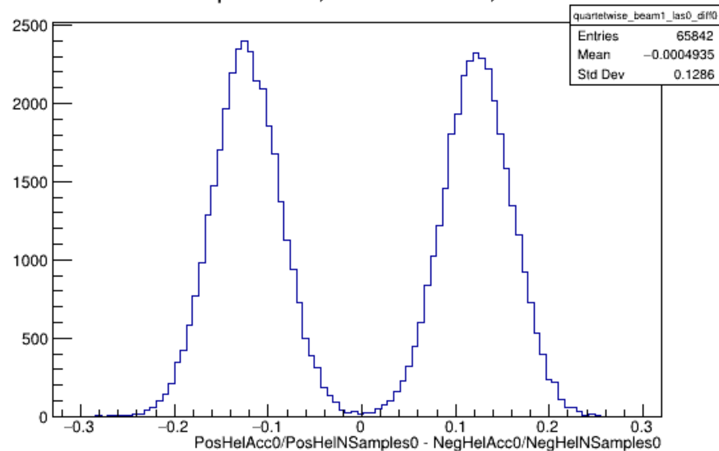
Run 5150 quartetwise, Diffs0: Beam ON, Laser OFF
