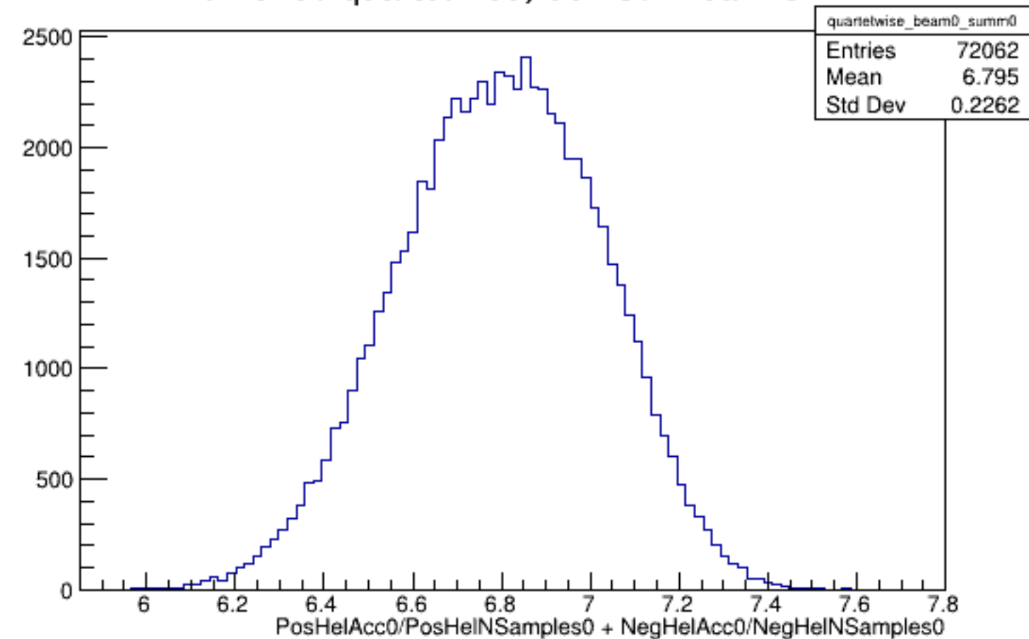
Run 5150 quartetwise, Sums0: Beam OFF
