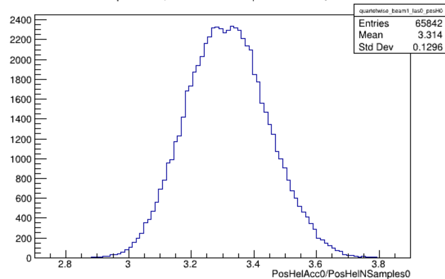
Run 5150 quartetwise, PosHelAcc0/NSamples0: Beam ON, Laser OFF
