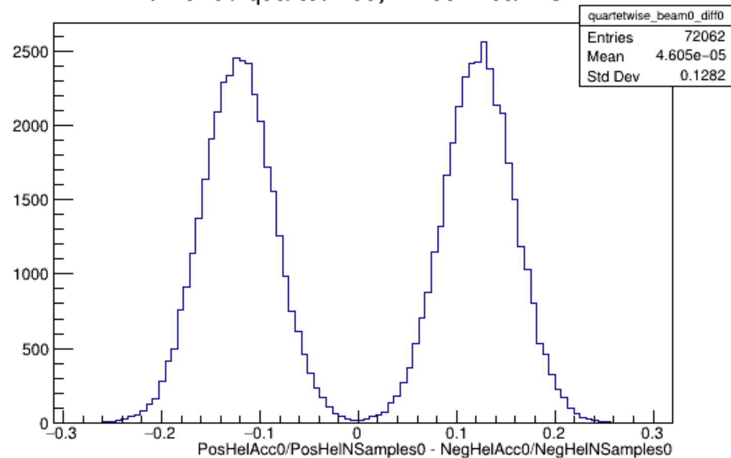
Run 5150 quartetwise, Diffs0: Beam OFF
