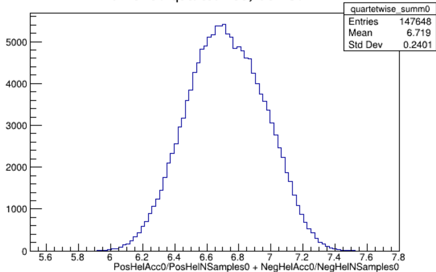
Run 5150 quartetwise, Sums0: All
