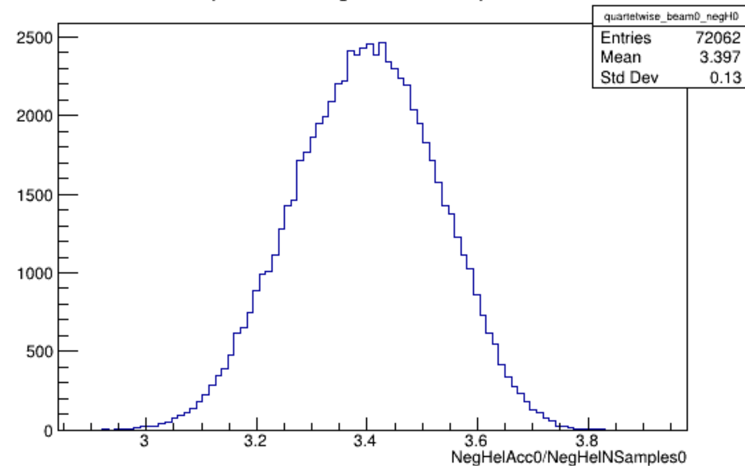
Run 5150 quartetwise, NegHelAcc0/NSamples0: Beam OFF
