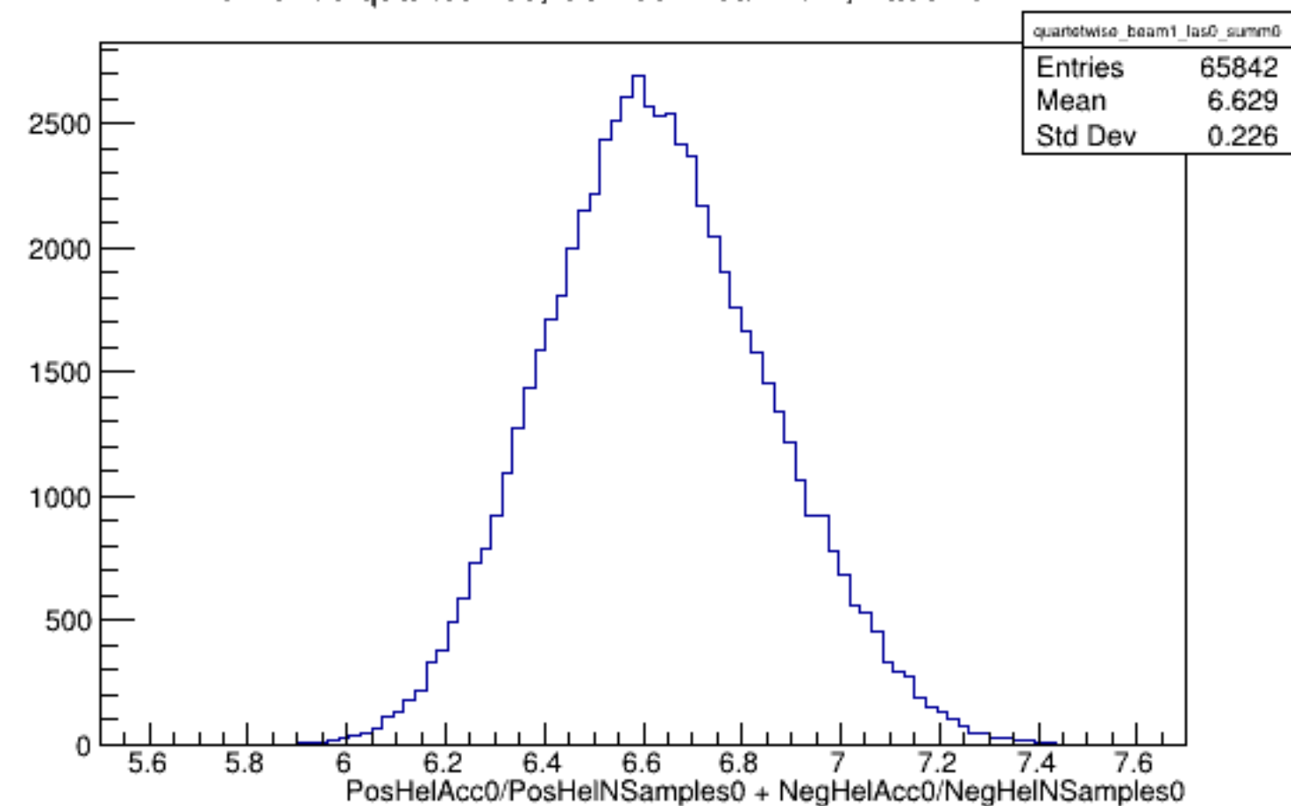
Run 5150 quartetwise, Sums0: Beam ON, Laser OFF
