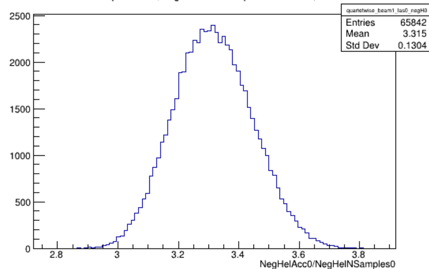
Run 5150 quartetwise, NegHelAcc0/NSamples0: Beam ON, Laser OFF
