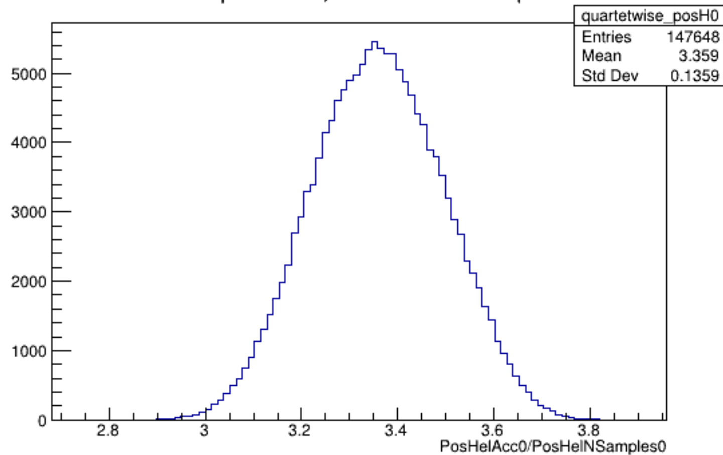
Run 5150 quartetwise, PosHelAcc0/NSamples0: All
