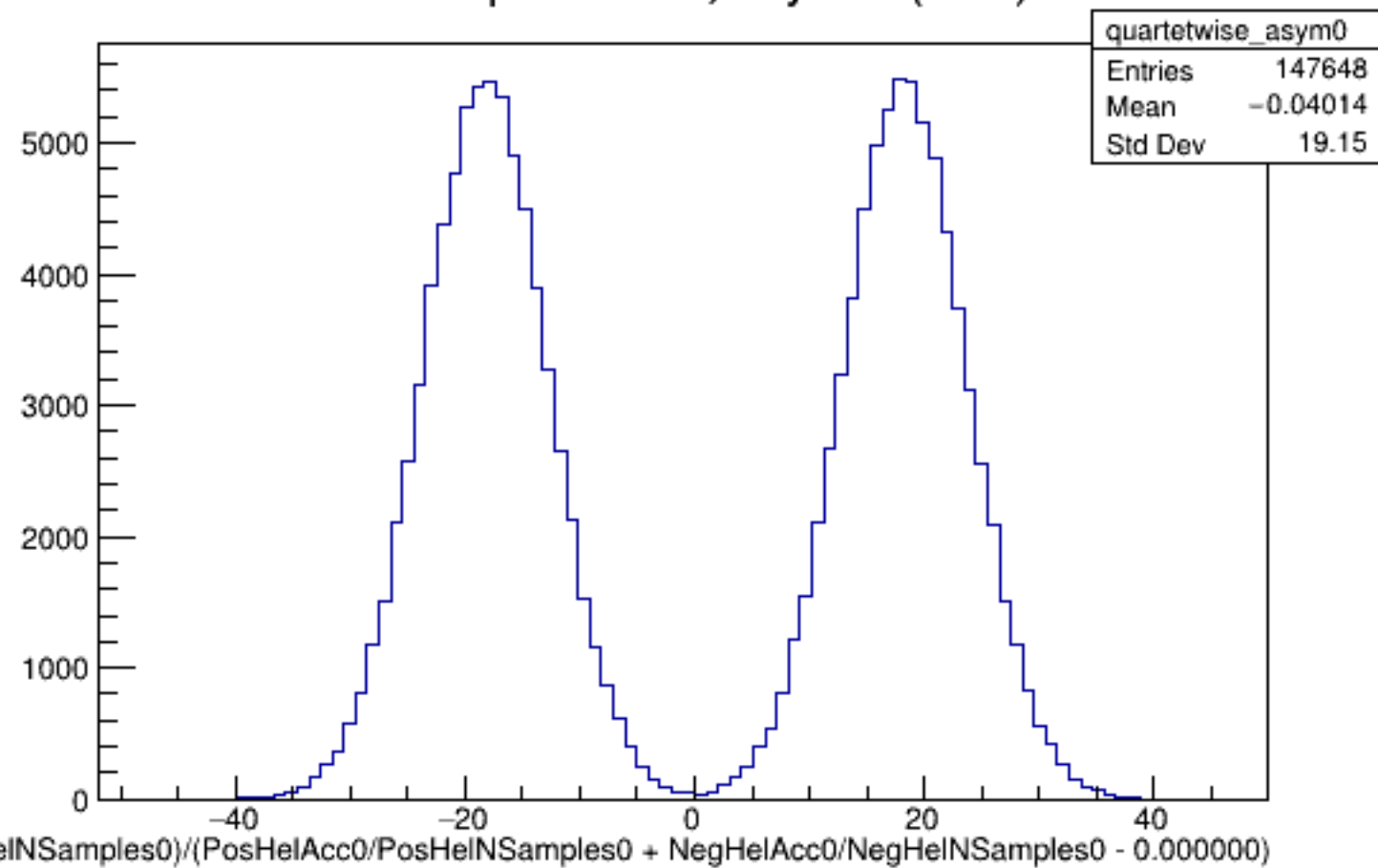
Run 5150 quartetwise, Asyms0 (Raw): All
