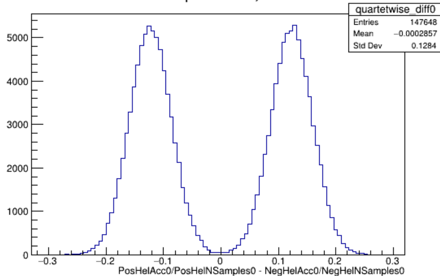
Run 5150 quartetwise, Diffs0: All
