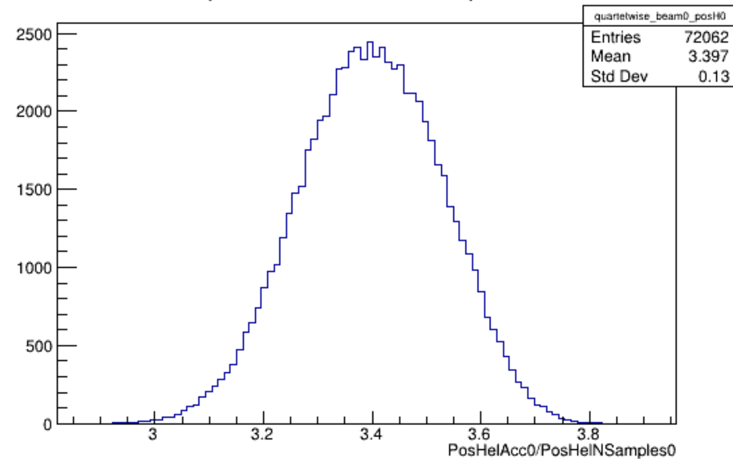
Run 5150 quartetwise, PosHelAcc0/NSamples0: Beam OFF
