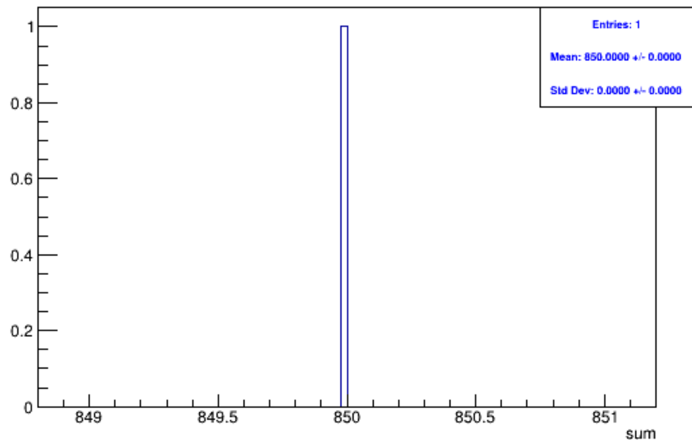
Run 5150 triggerwise, sums: All
