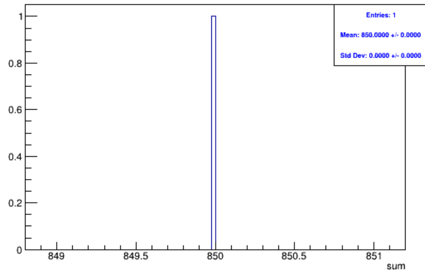
Run 5150 triggerwise, sums: Beam OFF
