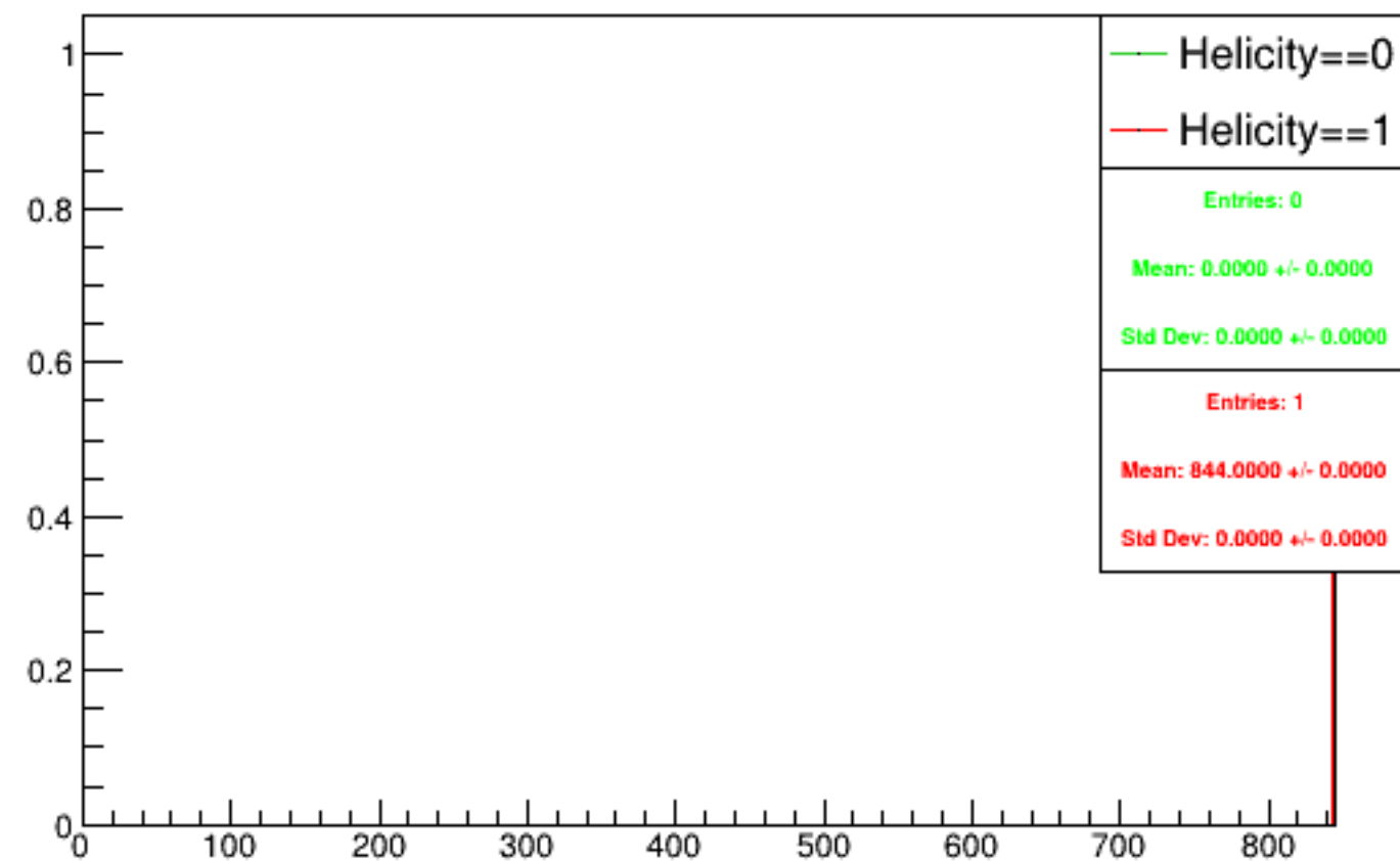
Run 5155 triggerwise, sums: Beam ON, Laser OFF
