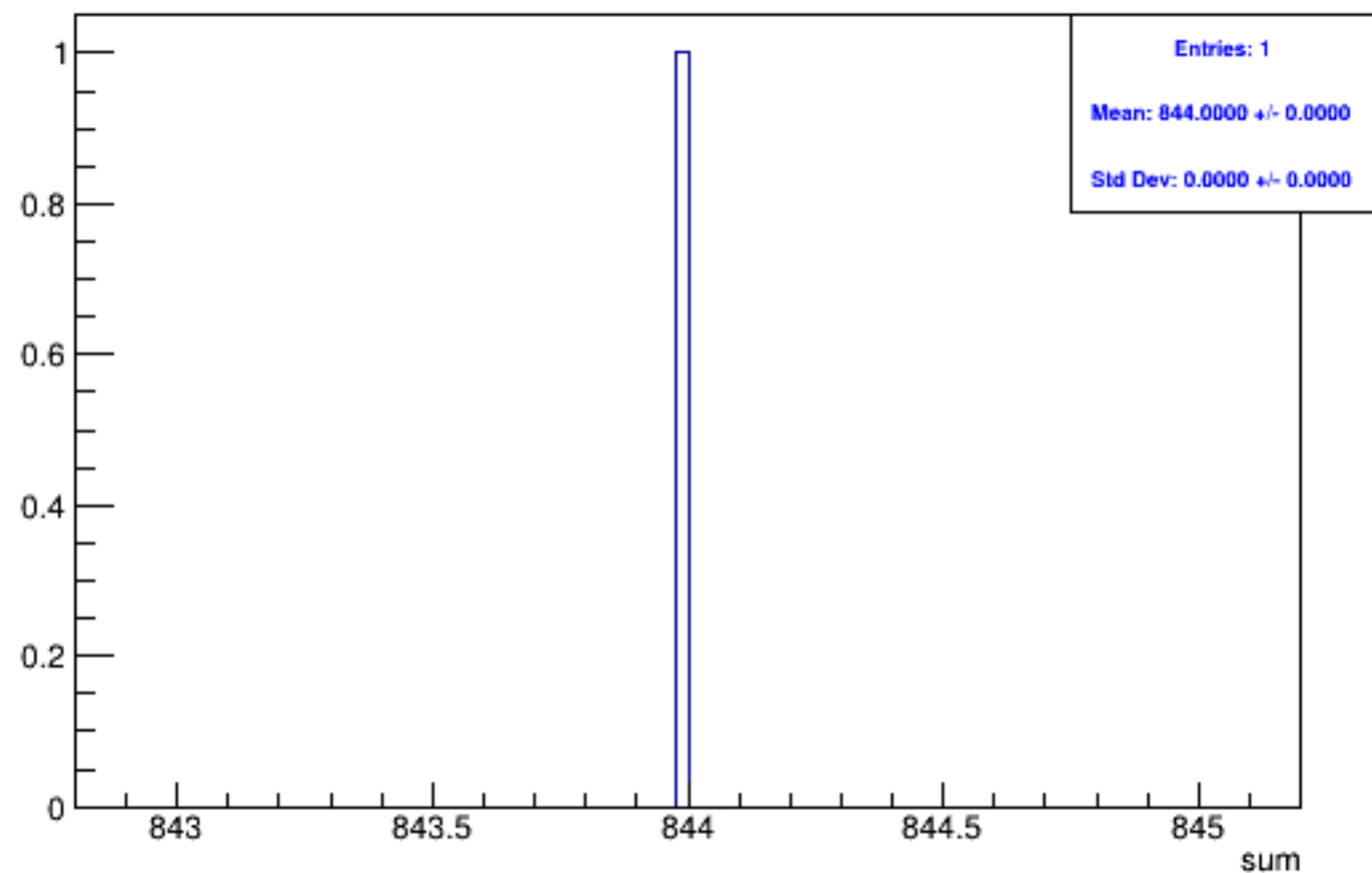
Run 5155 triggerwise, sums: All
