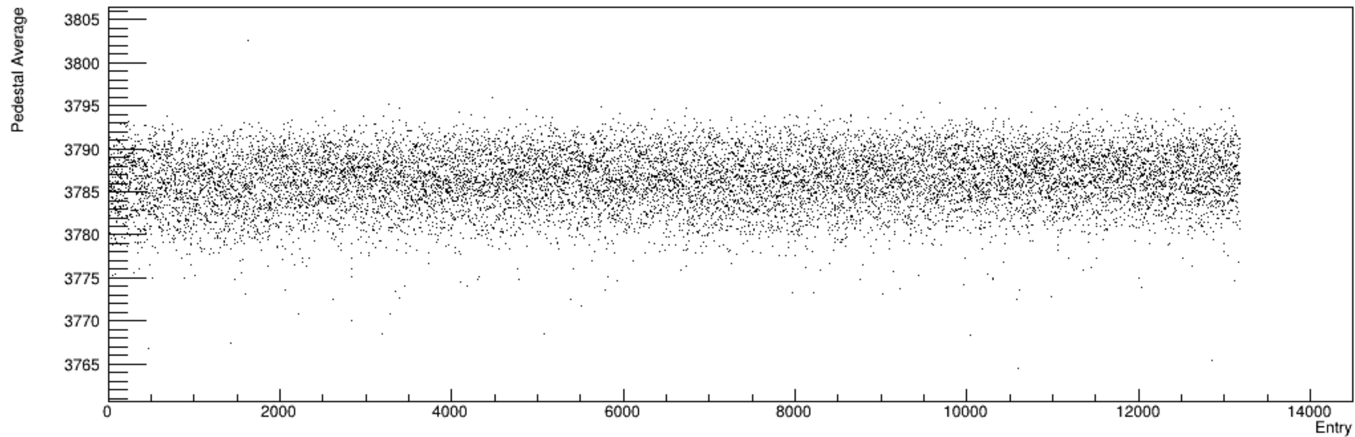
Run 5156, snapshots: Pedestal vs. Time
