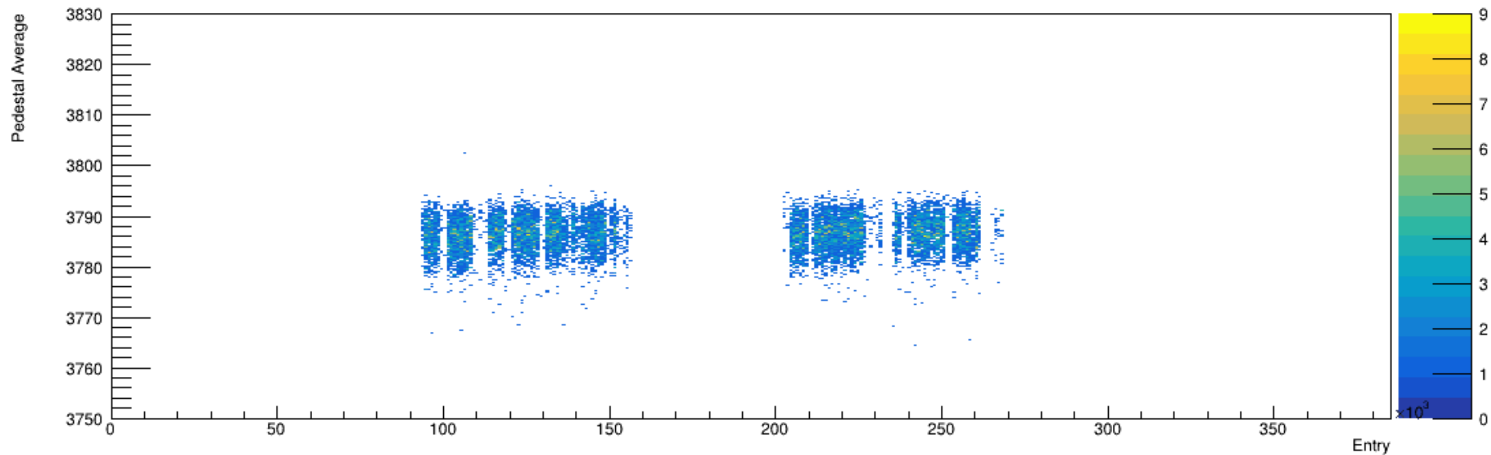
Run 5156, snapshots: Pedestal vs. Time
