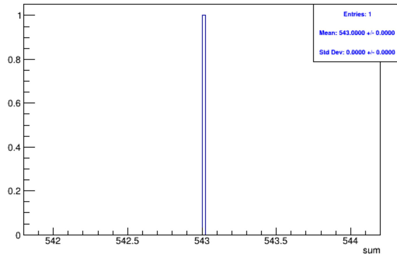
Run 5157 triggerwise, sums: Beam OFF
