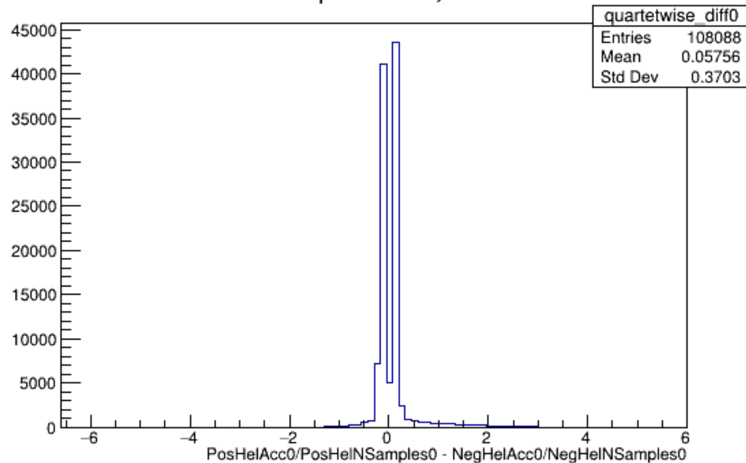
Run 5158 quartetwise, Diffs0: All
