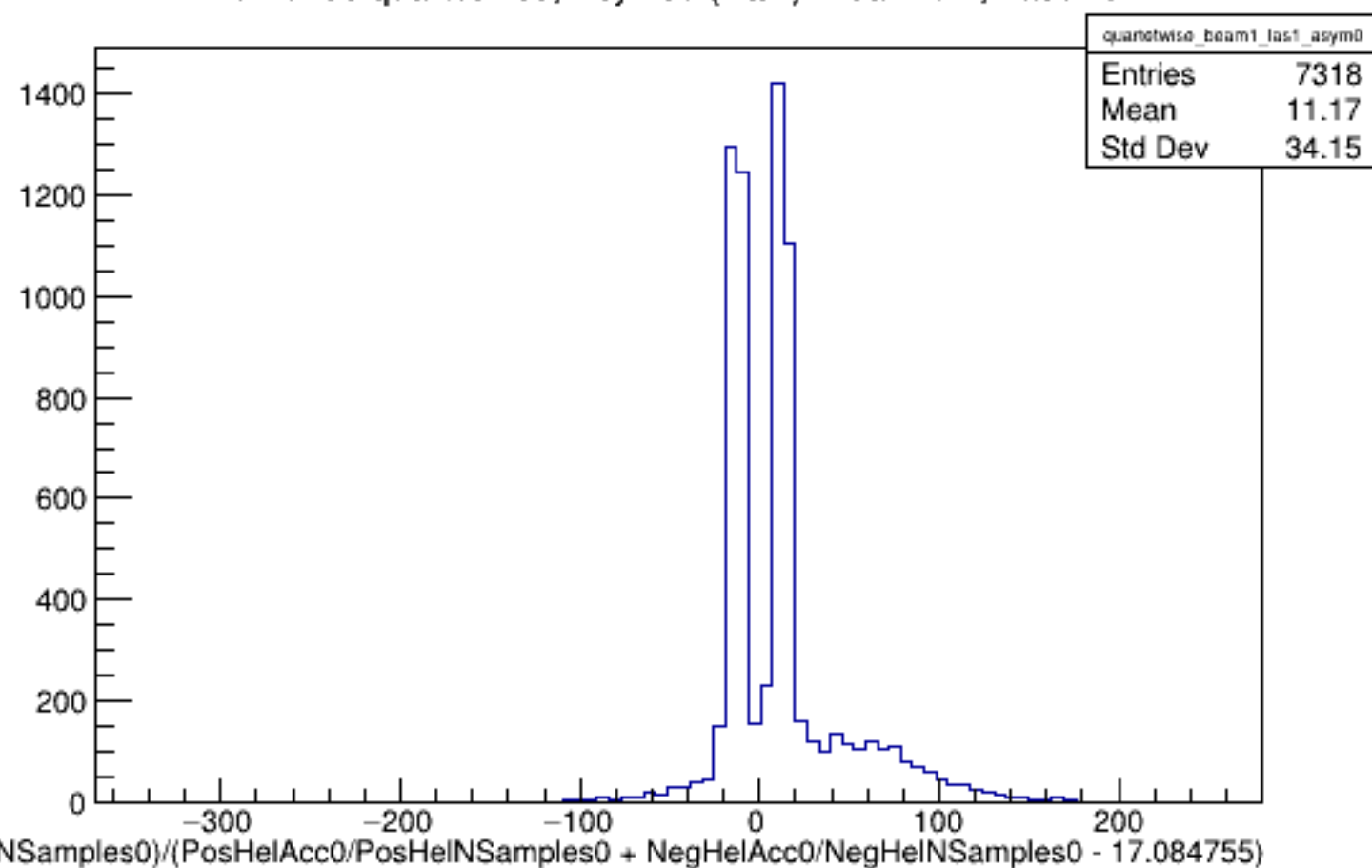
Run 5158 quartetwise, Asyms0 (Raw): Beam ON, Laser ON
