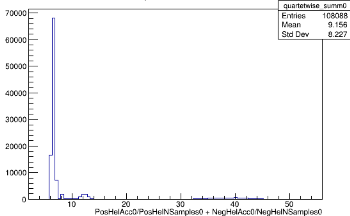
Run 5158 quartetwise, Sums0: All
