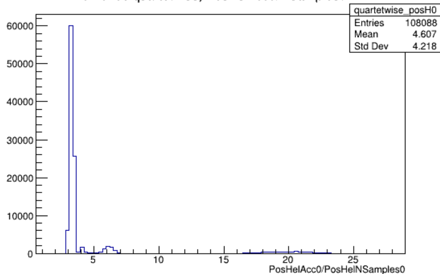
Run 5158 quartetwise, PosHelAcc0/NSamples0: All
