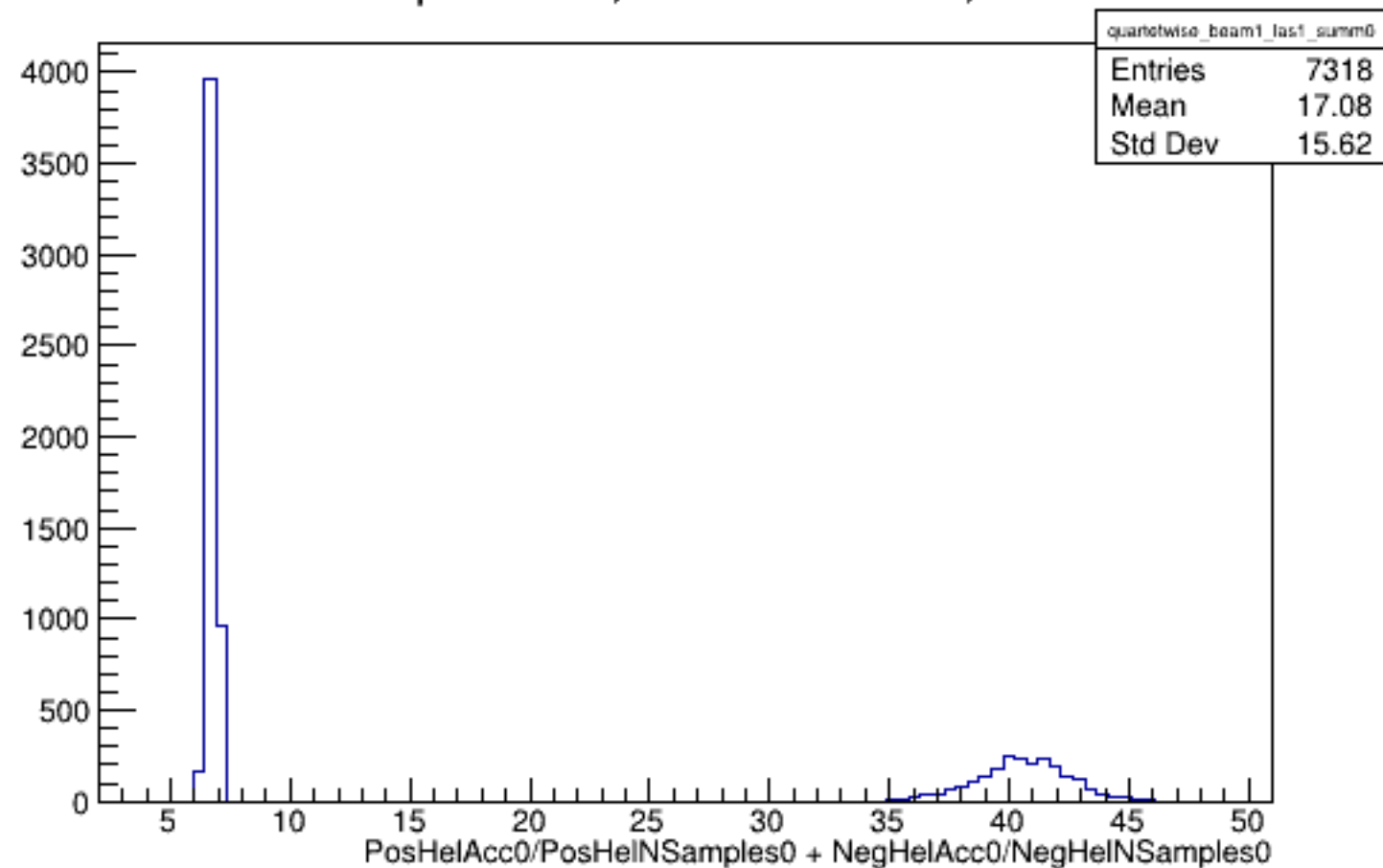
Run 5158 quartetwise, Sums0: Beam ON, Laser ON
