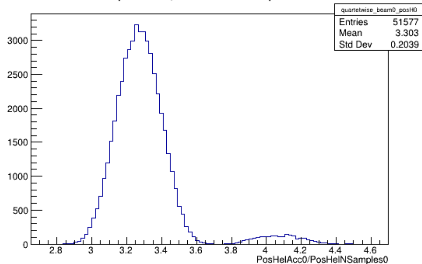
Run 5158 quartetwise, PosHelAcc0/NSamples0: Beam OFF
