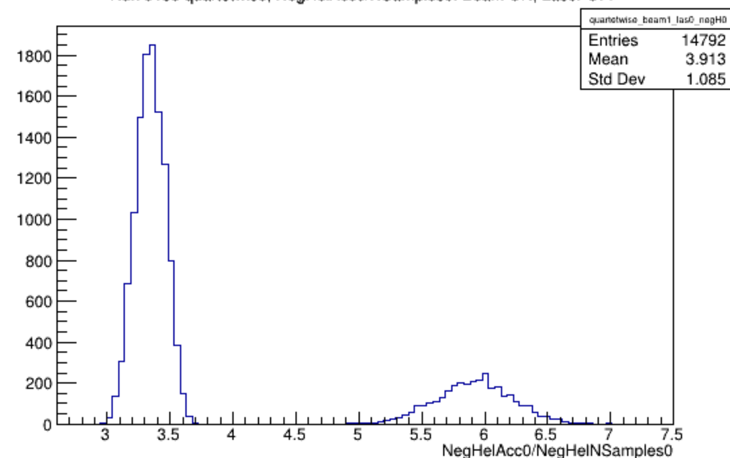
Run 5158 quartetwise, NegHelAcc0/NSamples0: Beam ON, Laser OFF
