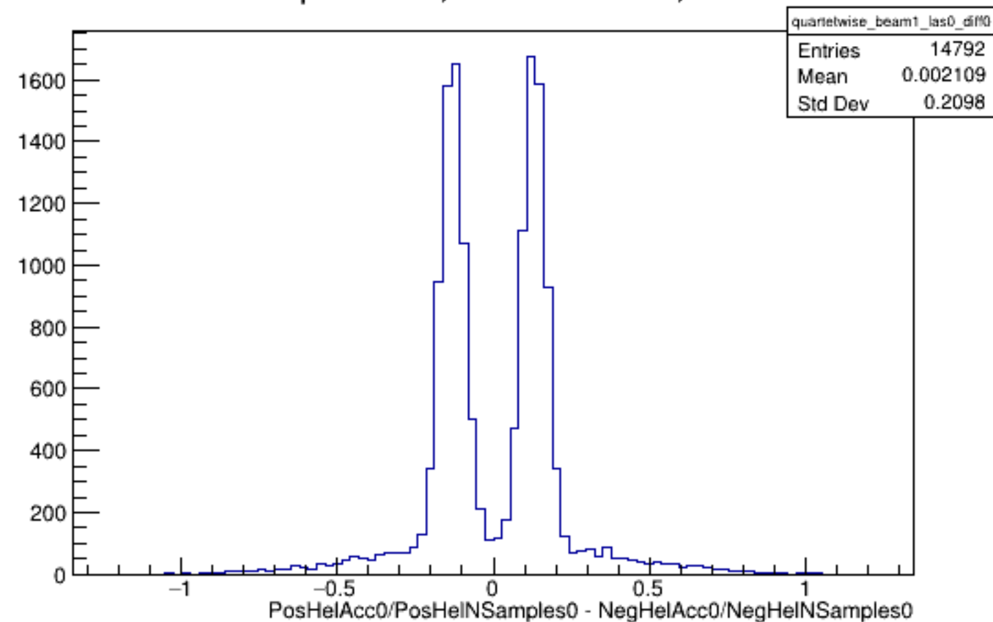
Run 5158 quartetwise, Diffs0: Beam ON, Laser OFF
