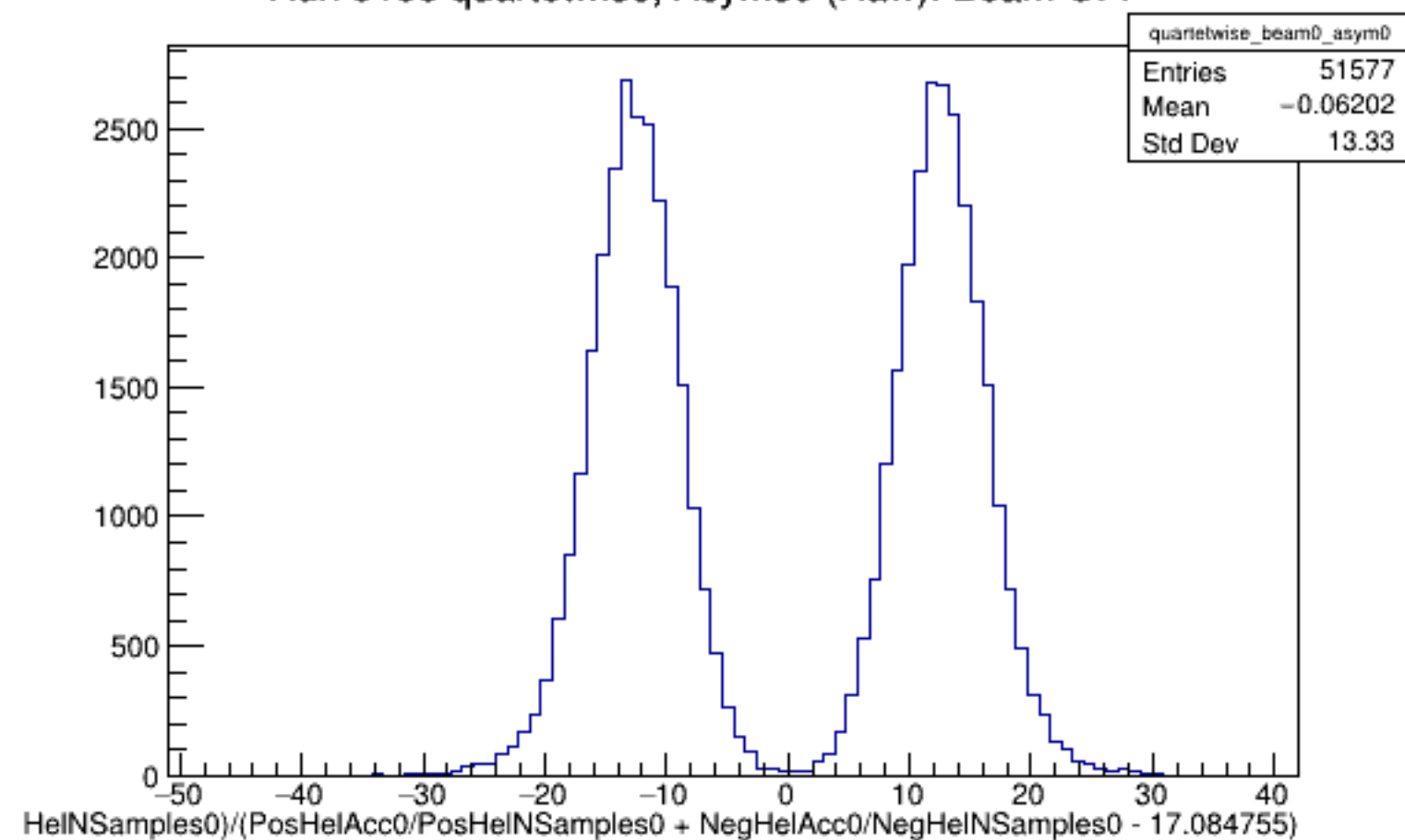
Run 5158 quartetwise, Asyms0 (Raw): Beam OFF
