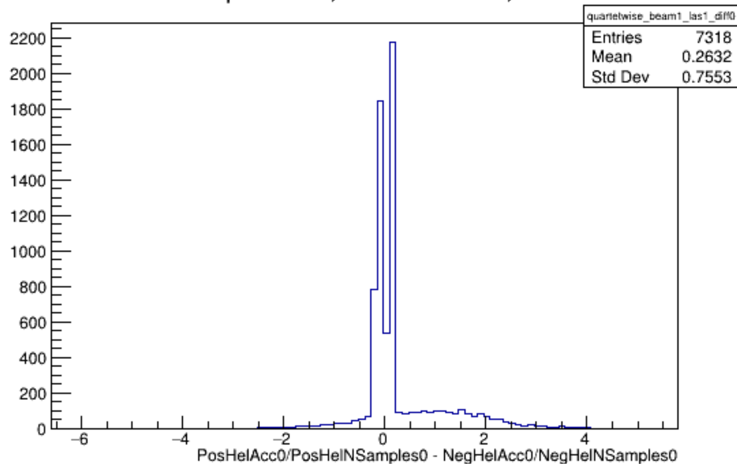
Run 5158 quartetwise, Diffs0: Beam ON, Laser ON
