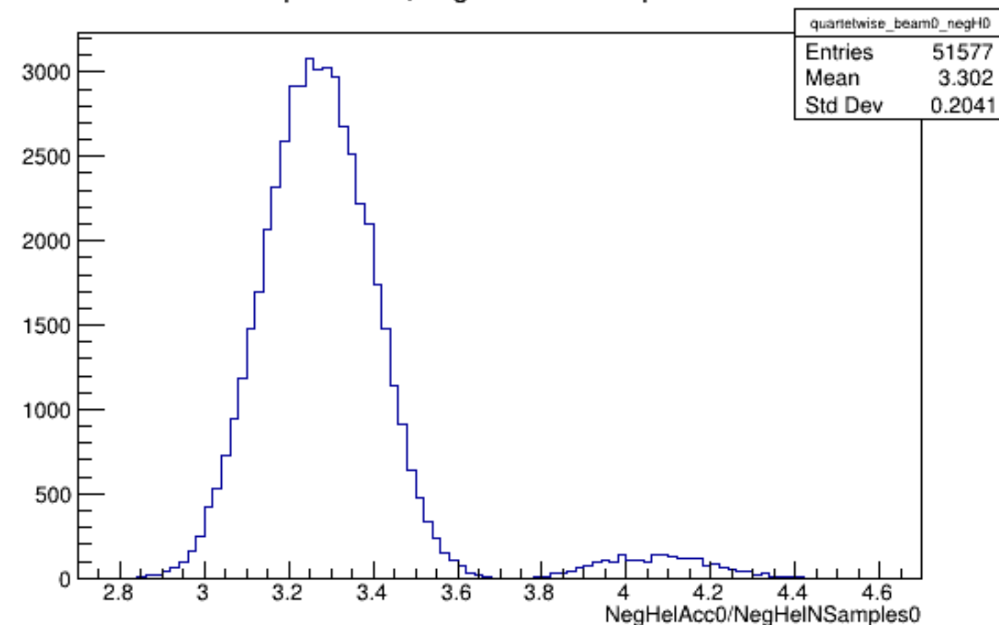
Run 5158 quartetwise, NegHelAcc0/NSamples0: Beam OFF
