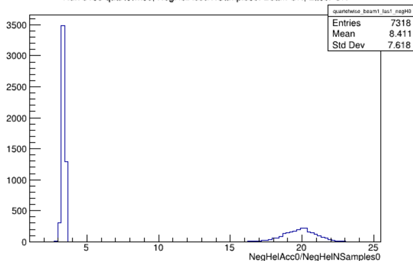
Run 5158 quartetwise, NegHelAcc0/NSamples0: Beam ON, Laser ON
