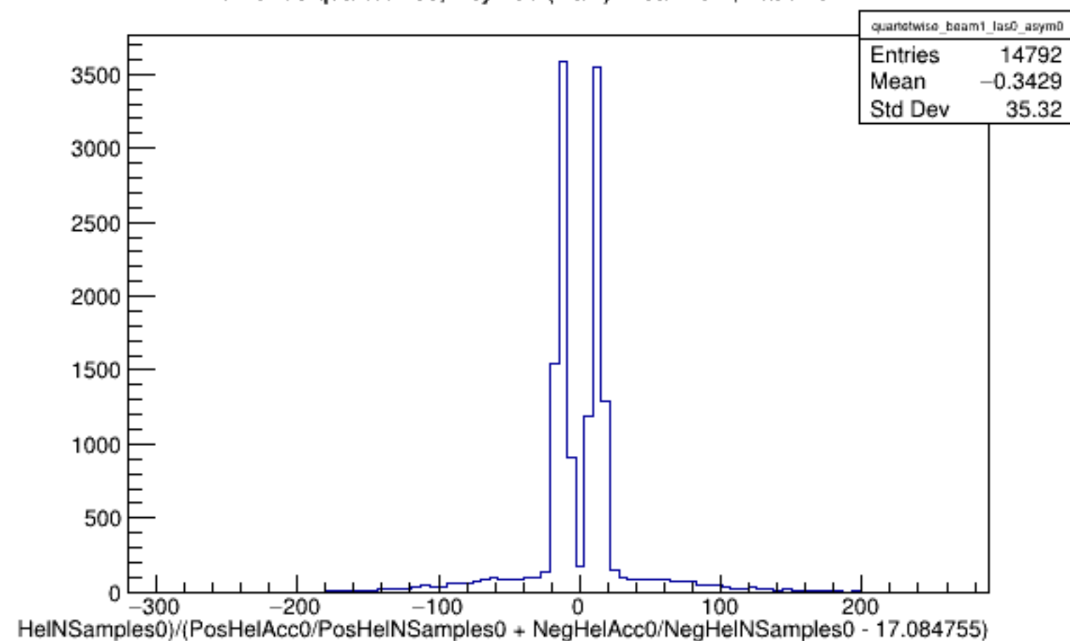
Run 5158 quartetwise, Asyms0 (Raw): Beam ON, Laser OFF
