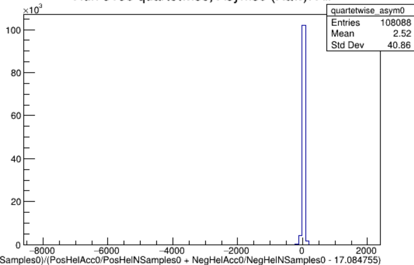
Run 5158 quartetwise, Asyms0 (Raw): All
