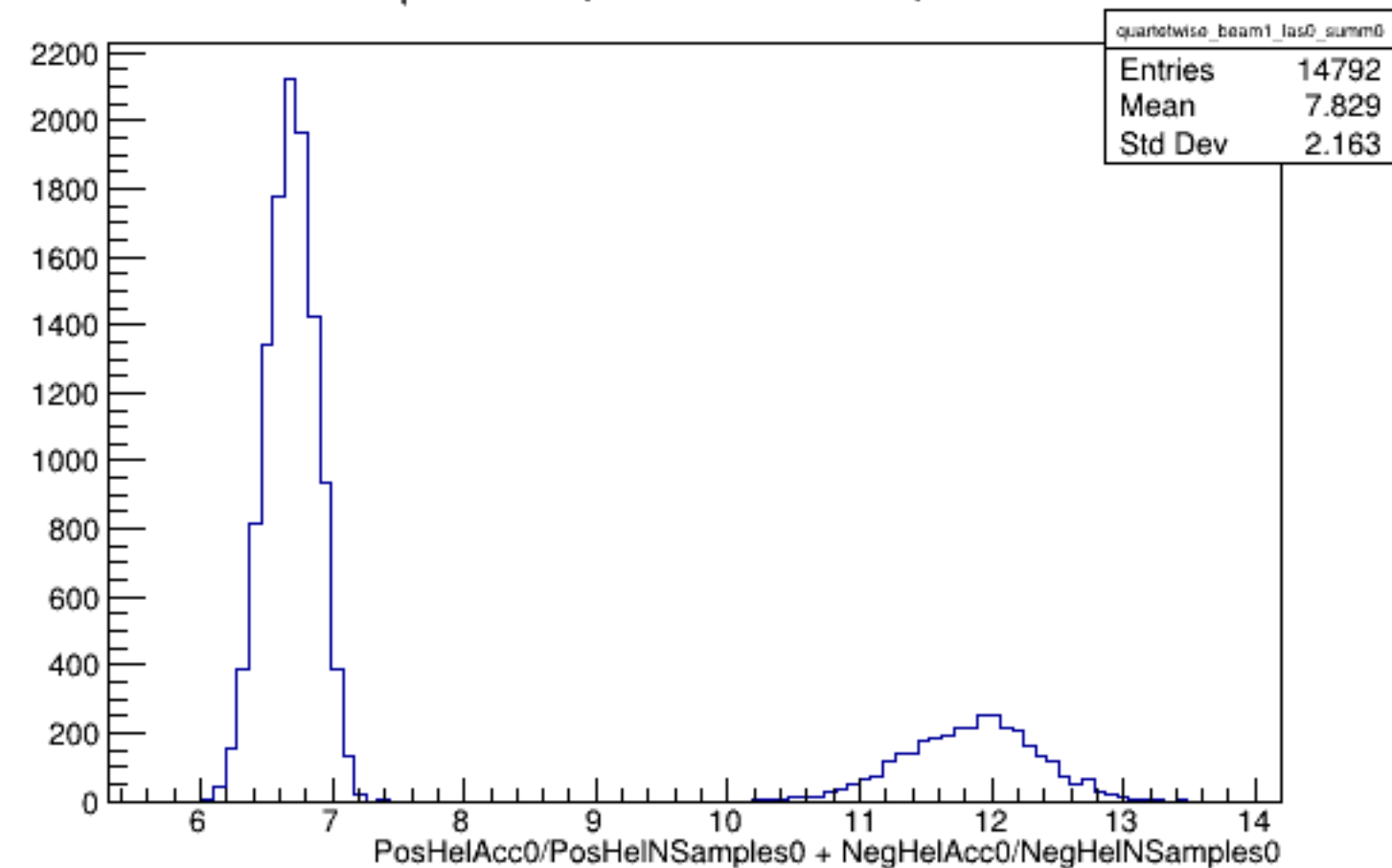
Run 5158 quartetwise, Sums0: Beam ON, Laser OFF
