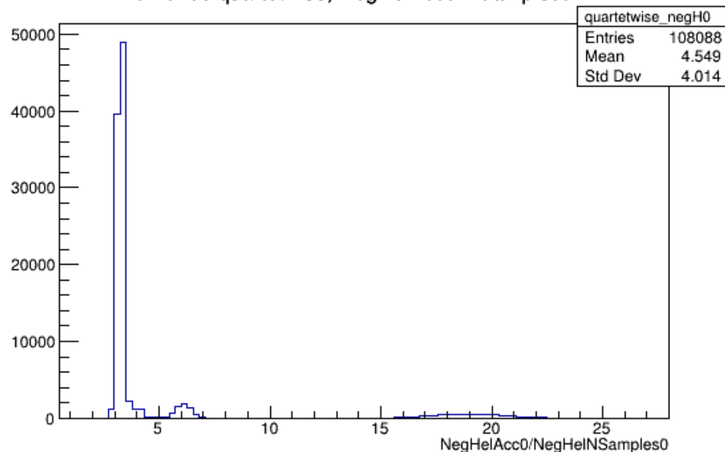
Run 5158 quartetwise, NegHelAcc0/NSamples0: All
