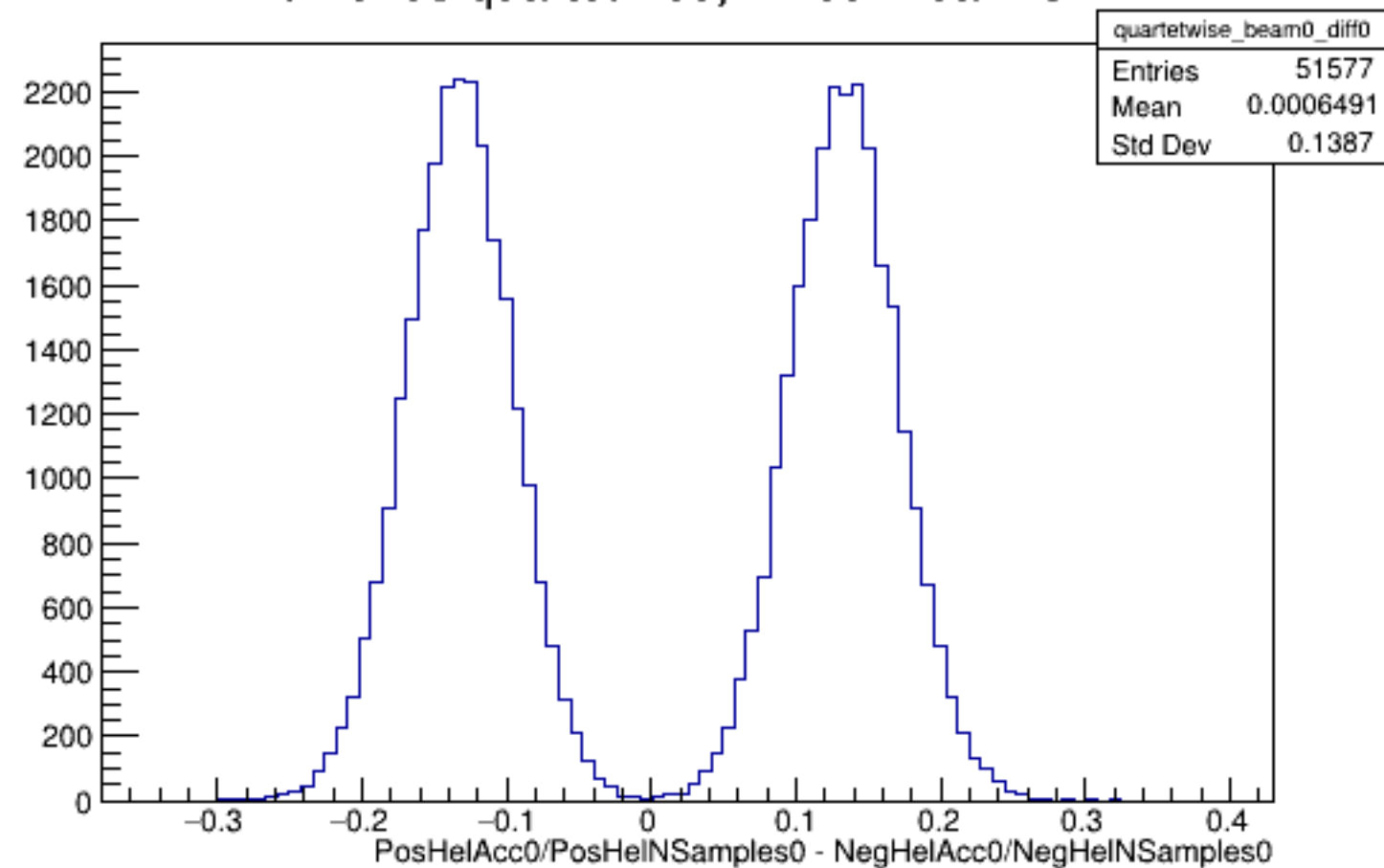
Run 5158 quartetwise, Diffs0: Beam OFF
