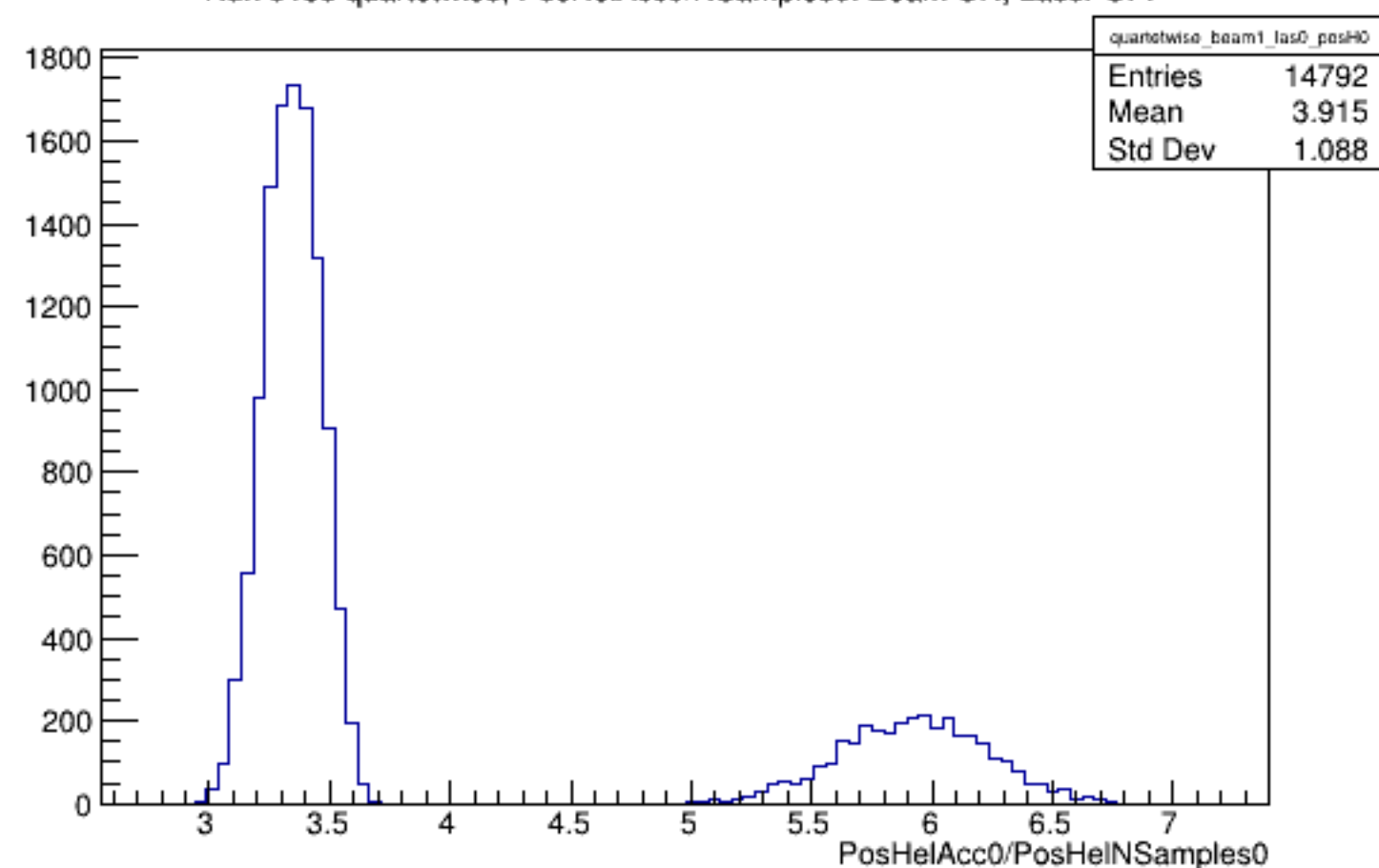
Run 5158 quartetwise, PosHelAcc0/NSamples0: Beam ON, Laser OFF
