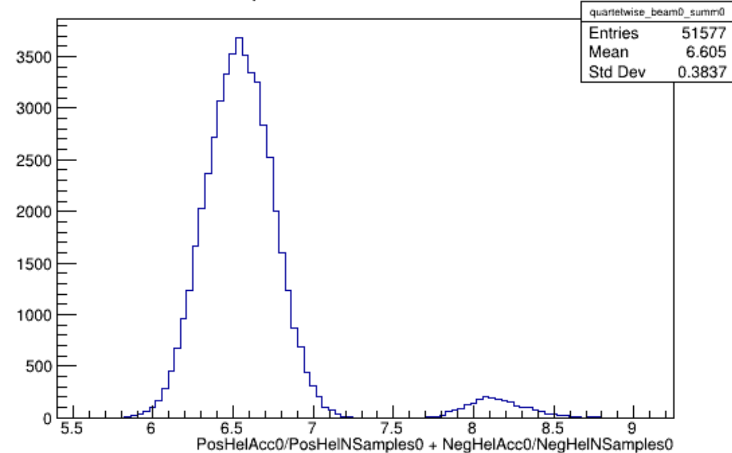
Run 5158 quartetwise, Sums0: Beam OFF
