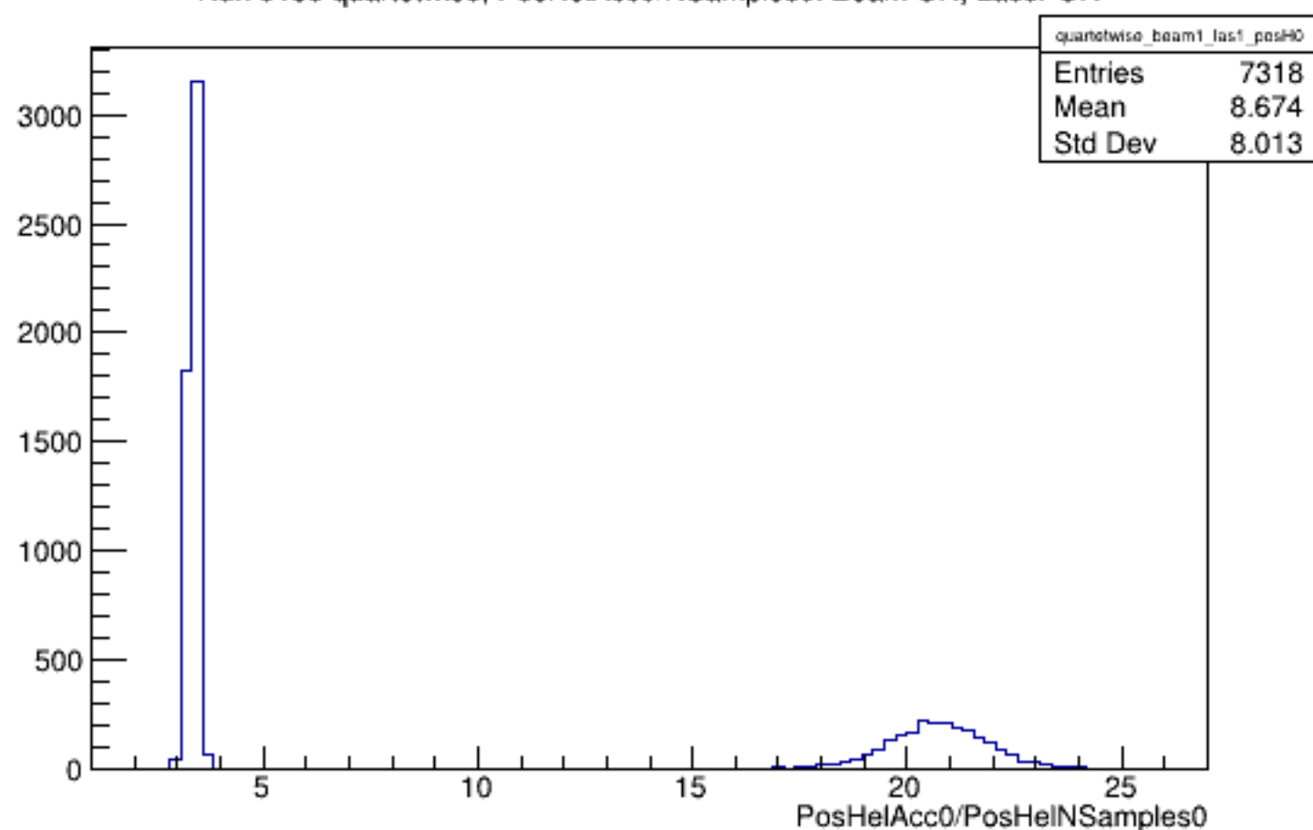
Run 5158 quartetwise, PosHelAcc0/NSamples0: Beam ON, Laser ON
