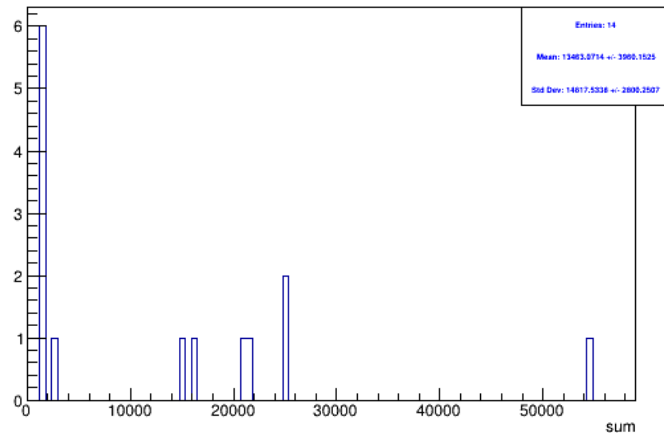
Run 5158 triggerwise, sums: Beam OFF
