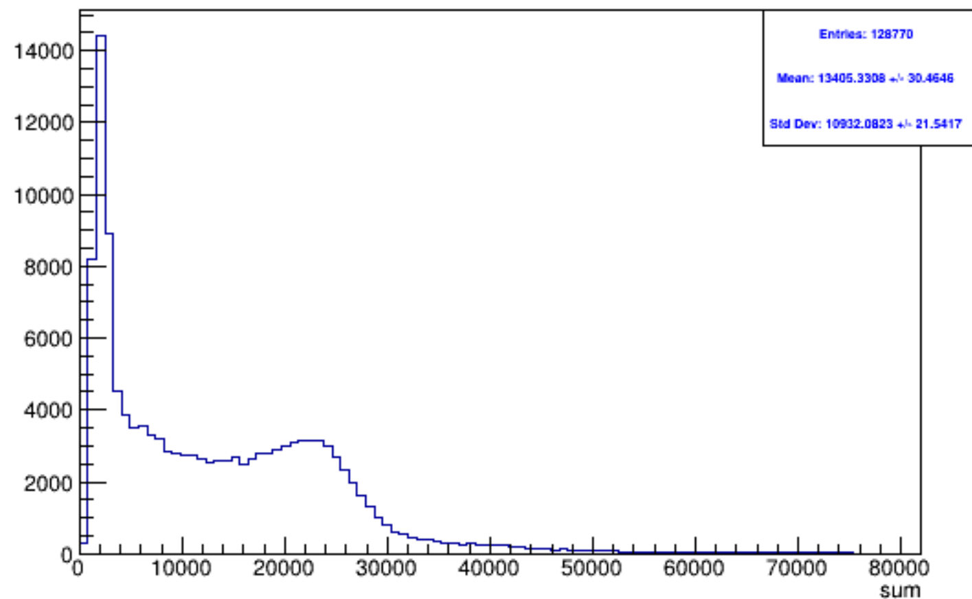
Run 5158 triggerwise, sums: All
