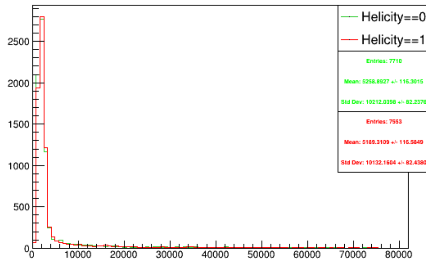
Run 5158 triggerwise, sums: Beam ON, Laser OFF
