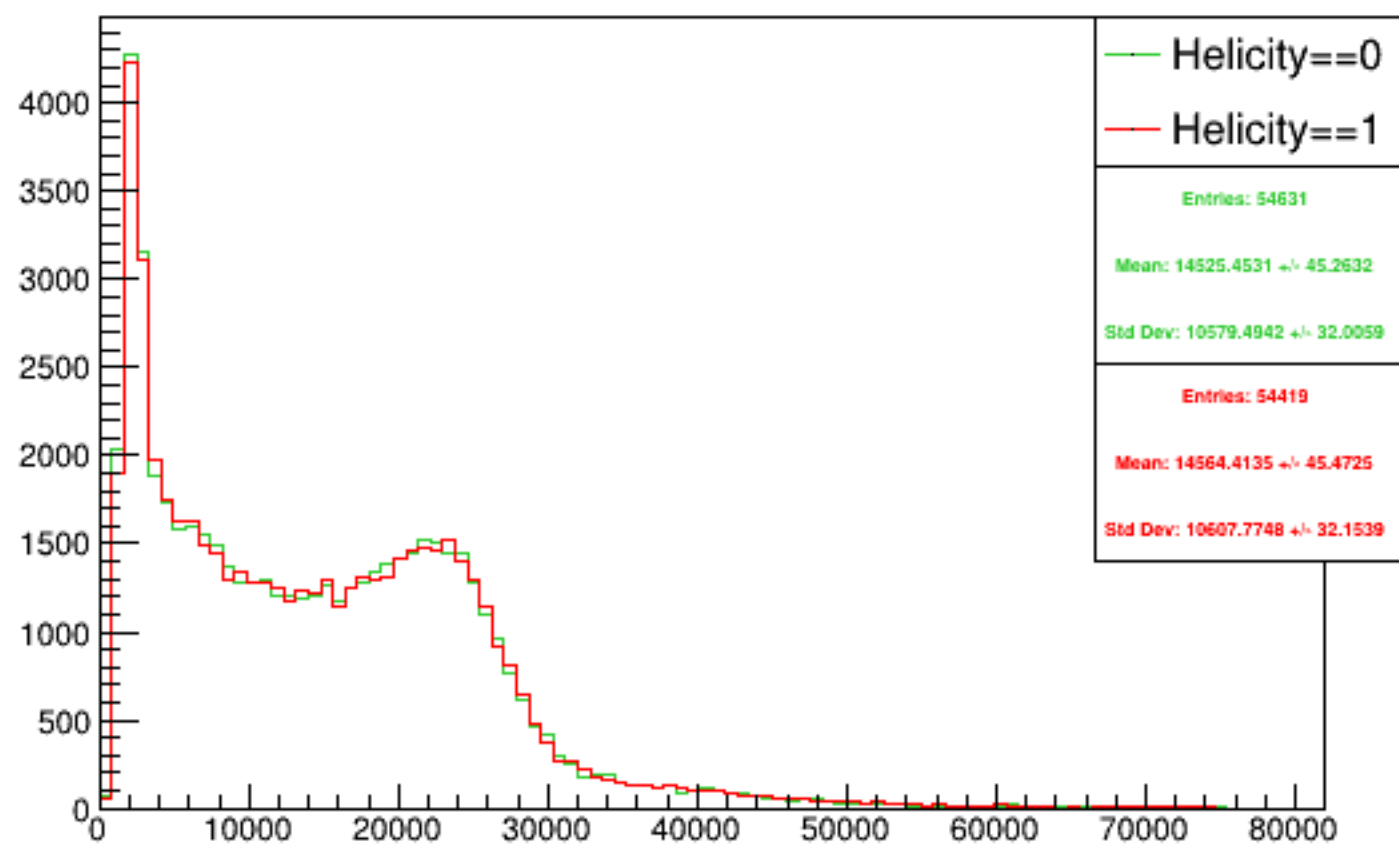
Run 5158 triggerwise, sums: Beam ON, Laser ON
