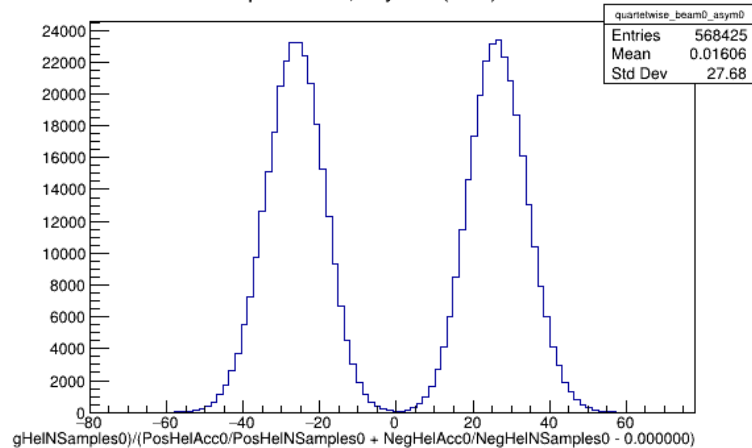
Run 5164 quartetwise, Asyms0 (Raw): Beam OFF
