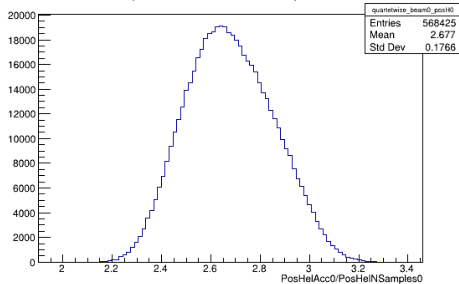
Run 5164 quartetwise, PosHelAcc0/NSamples0: Beam OFF
