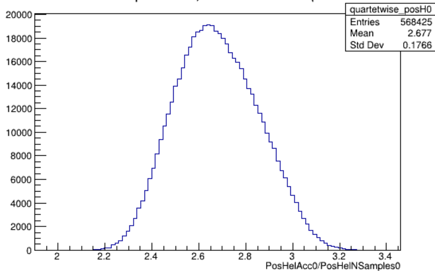
Run 5164 quartetwise, PosHelAcc0/NSamples0: All
