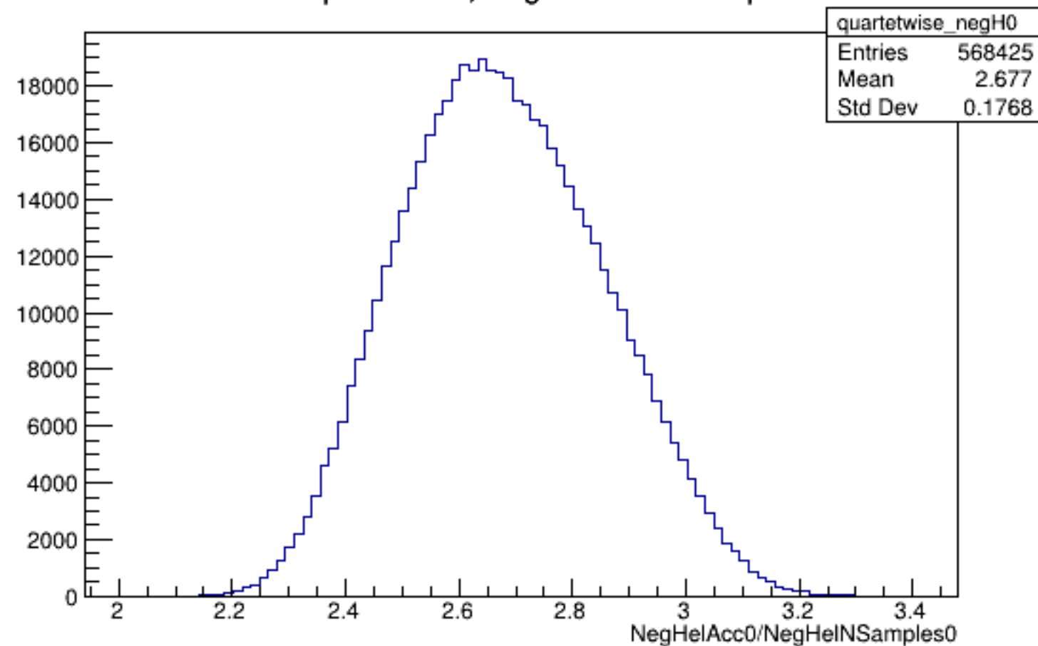
Run 5164 quartetwise, NegHelAcc0/NSamples0: All
