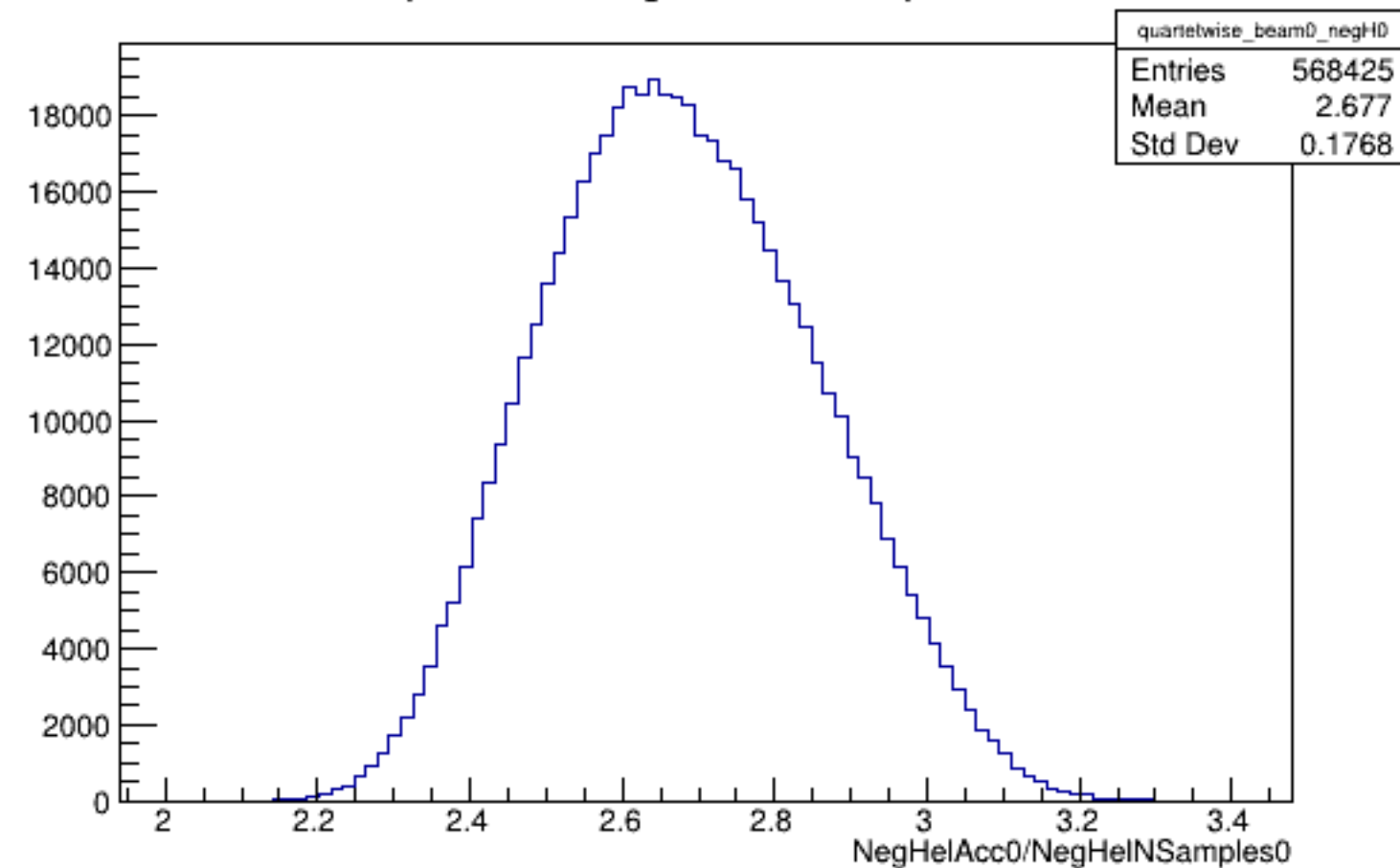
Run 5164 quartetwise, NegHelAcc0/NSamples0: Beam OFF
