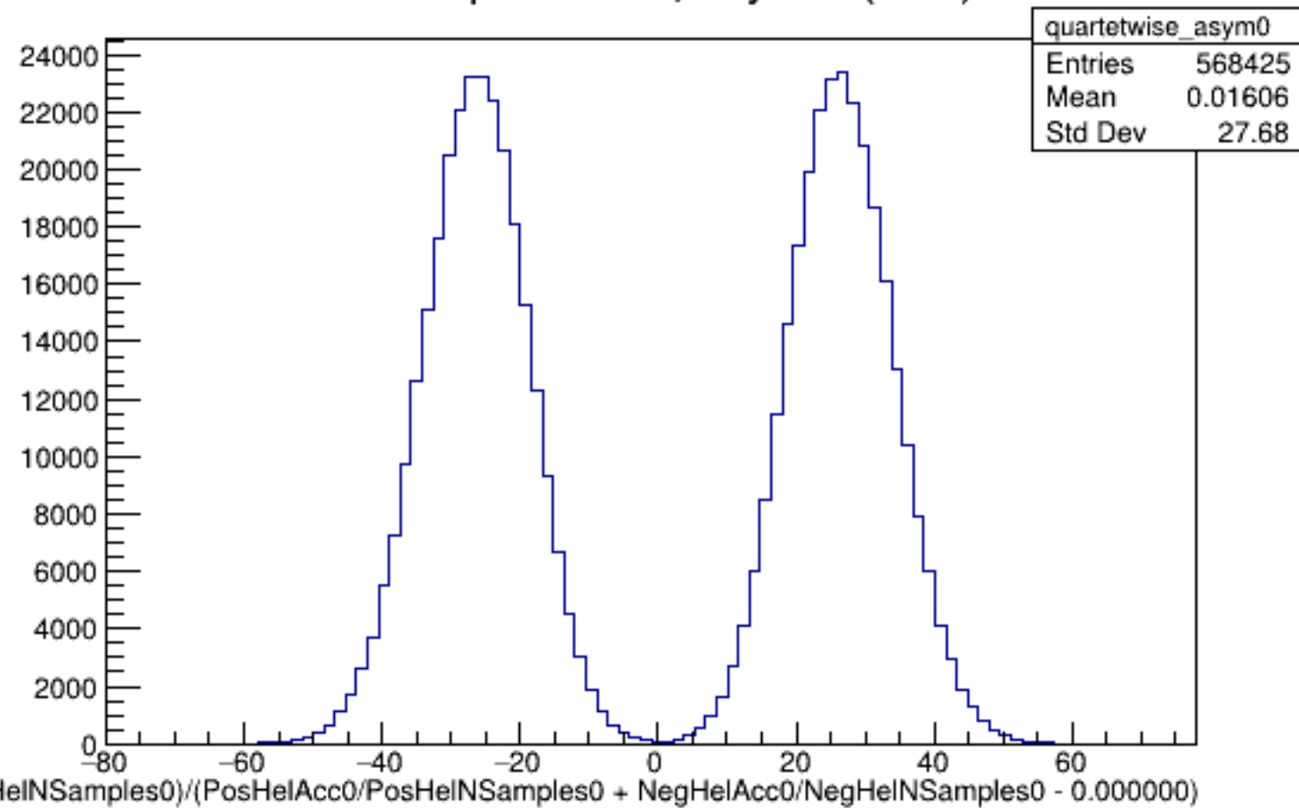
Run 5164 quartetwise, Asyms0 (Raw): All
