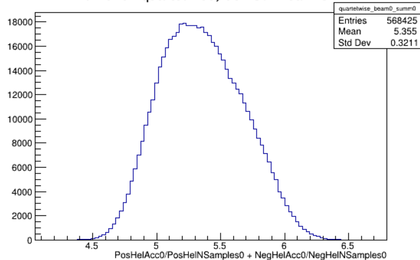
Run 5164 quartetwise, Sums0: Beam OFF
