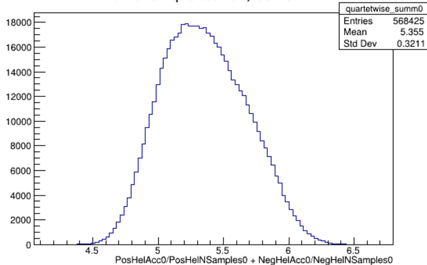
Run 5164 quartetwise, Sums0: All
