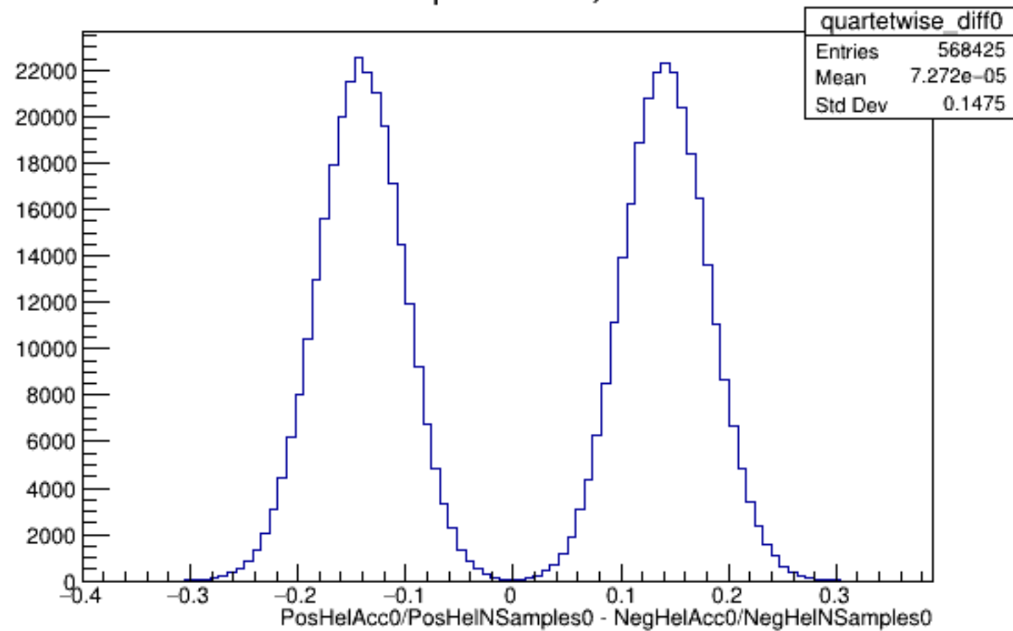
Run 5164 quartetwise, Diffs0: All
