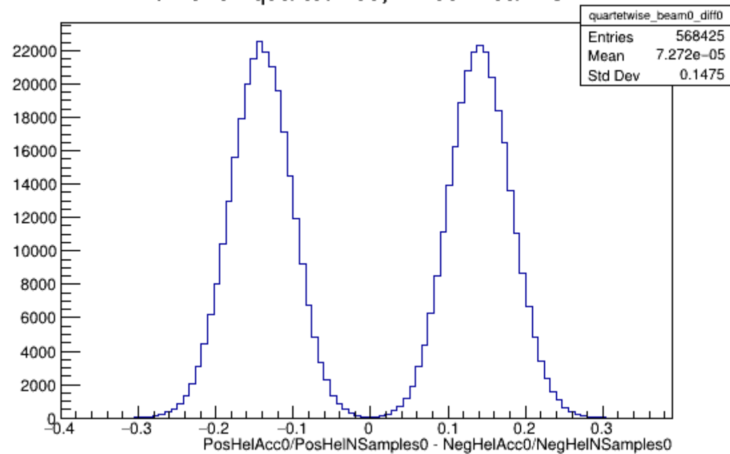
Run 5164 quartetwise, Diffs0: Beam OFF
