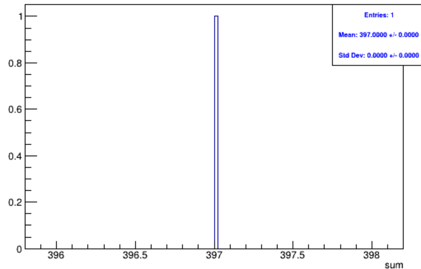
Run 5166 triggerwise, sums: Beam OFF
