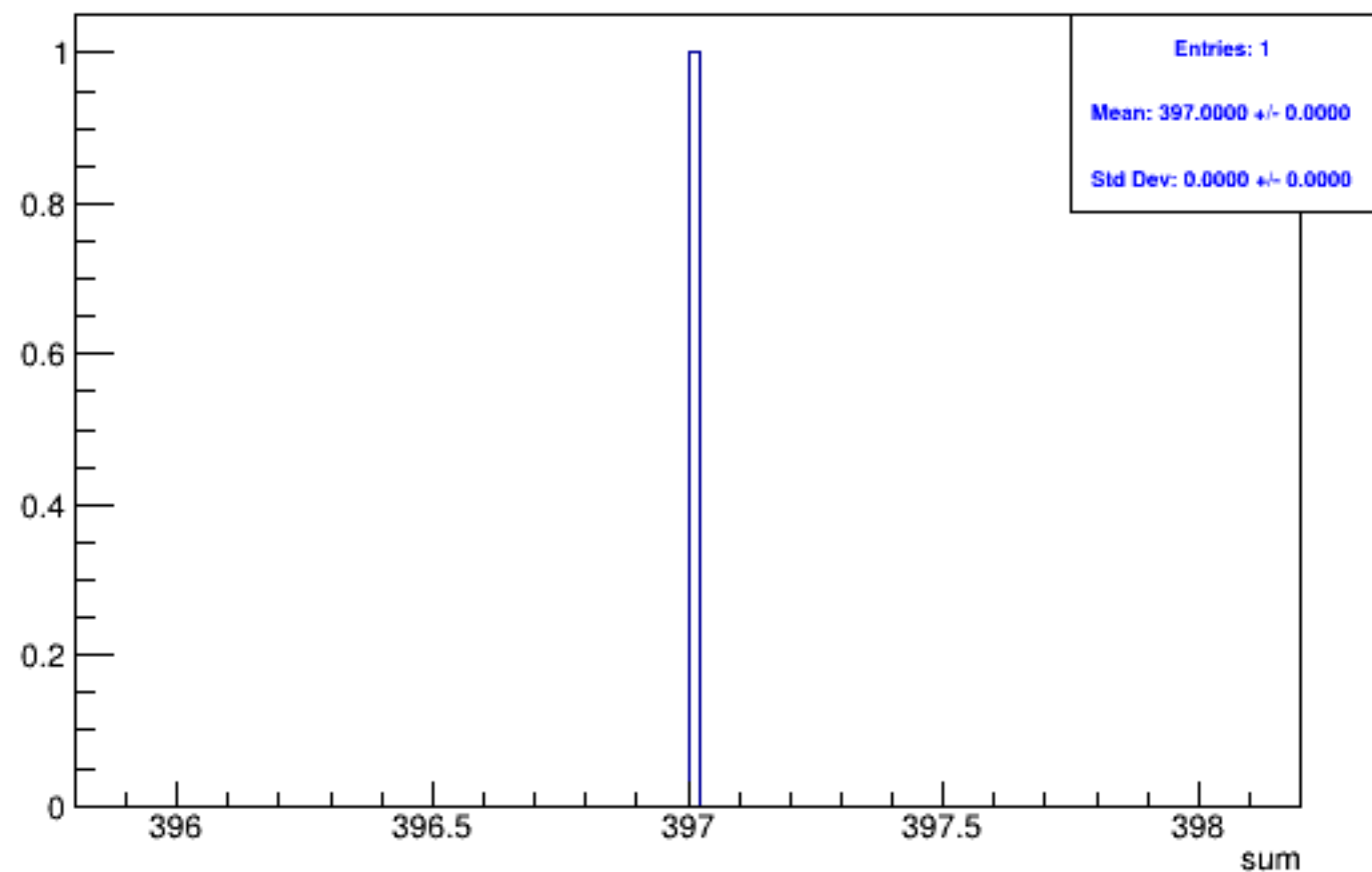
Run 5166 triggerwise, sums: All
