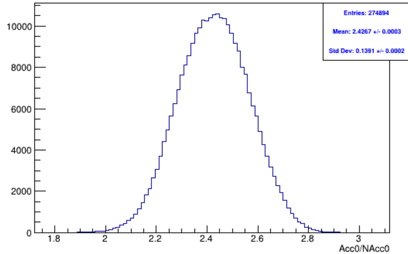
Run 5167 mpwise, acc0: All
