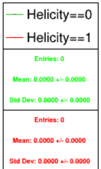
Run 5167 mpwise, acc0: Beam ON, Laser OFF
