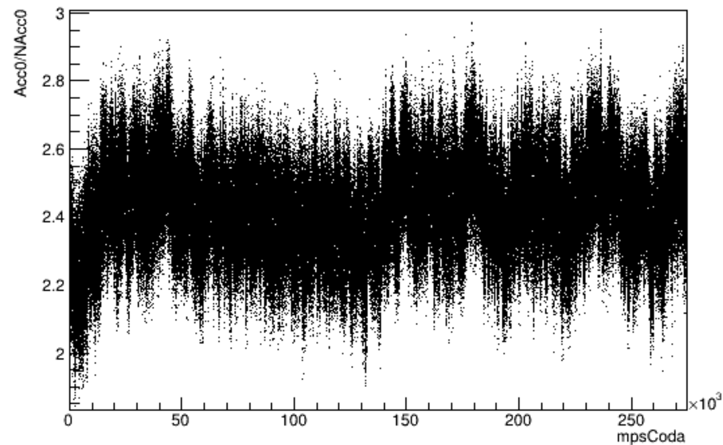
Run 5167 mpswise, Acc0 vs Time: Beam OFF
