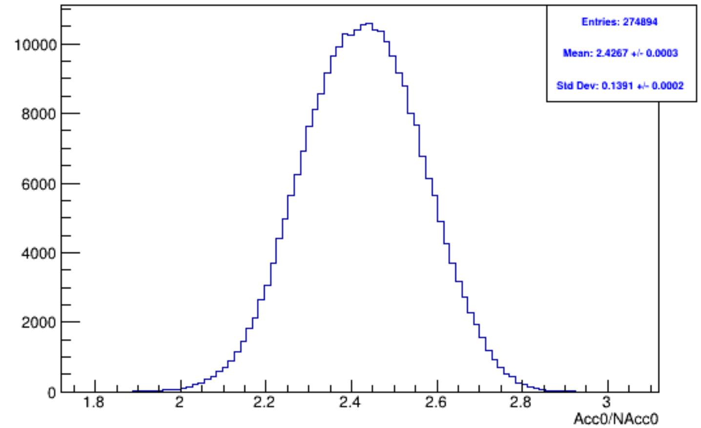
Run 5167 mpwise, acc0: Beam OFF
