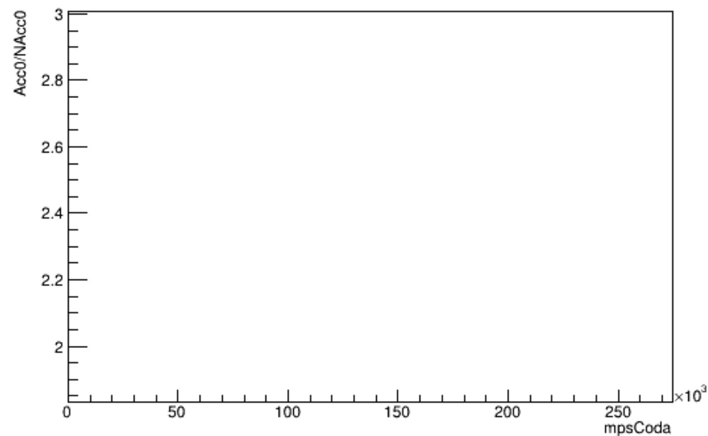
Run 5167 mpswise, Acc0 vs Time: Beam ON, Laser OFF
