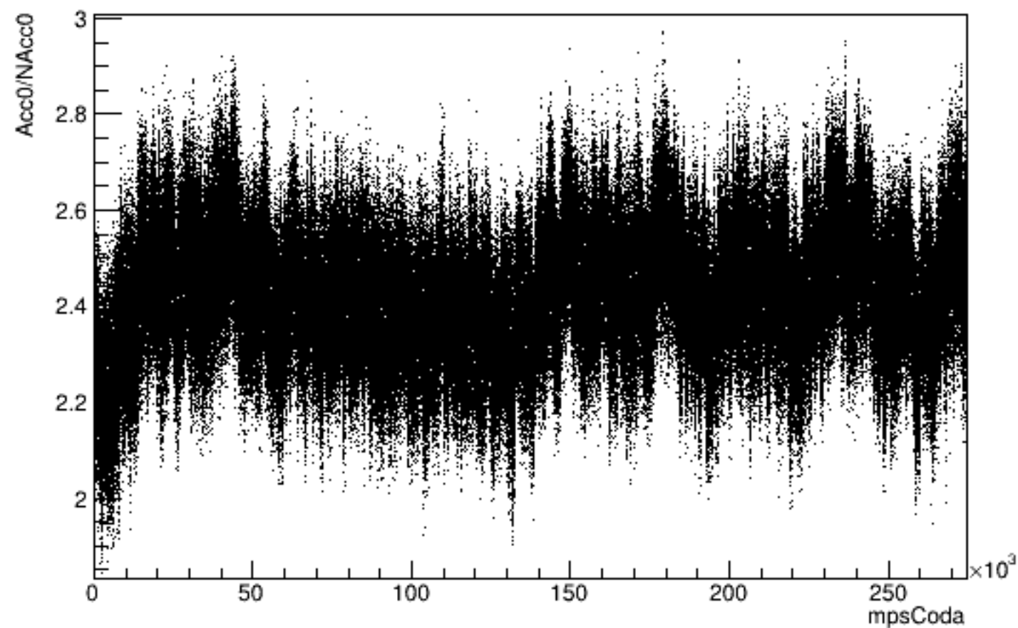
Run 5167 mpswise, Acc0 vs Time: All
