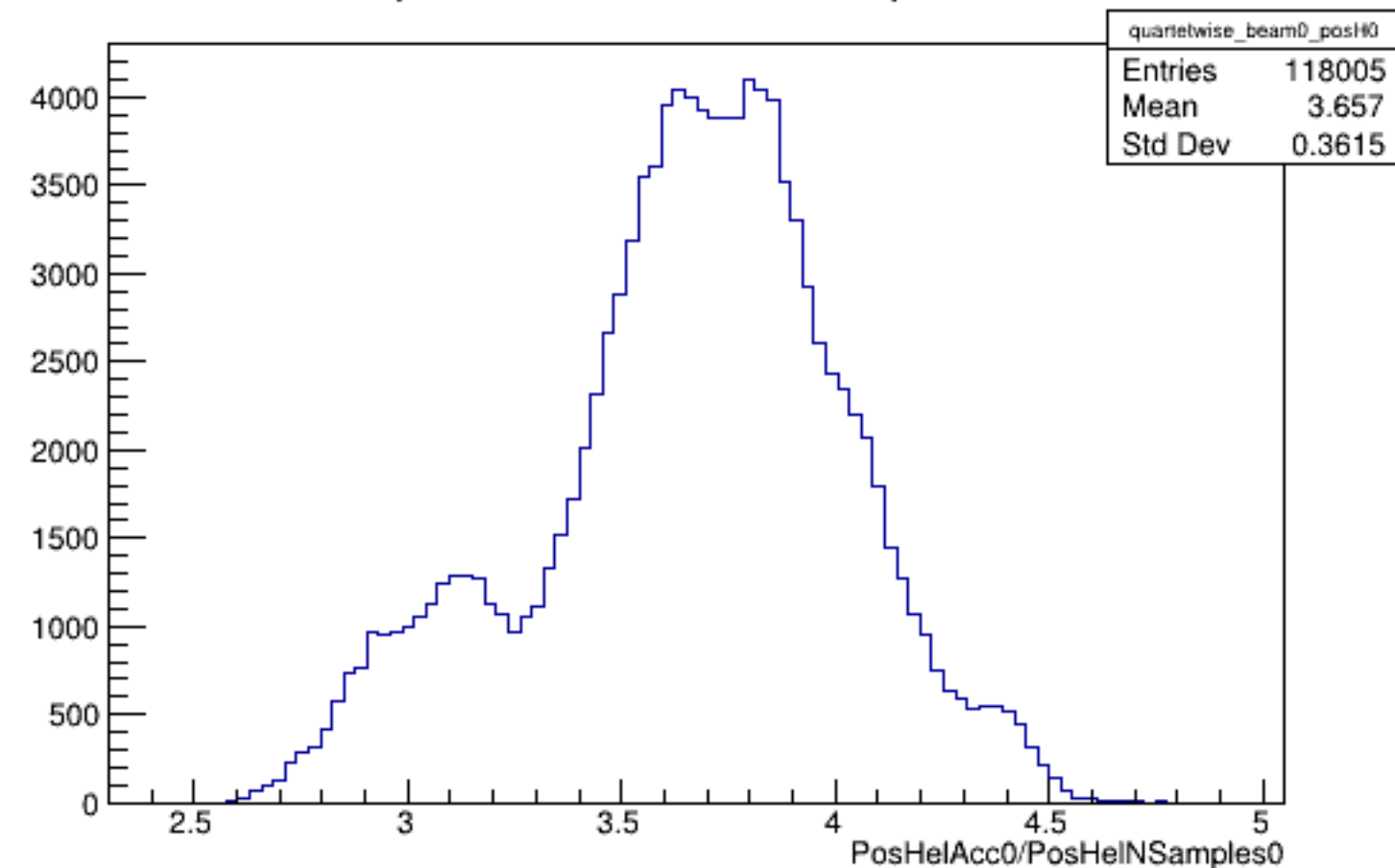
Run 5170 quartetwise, PosHelAcc0/NSamples0: Beam OFF
