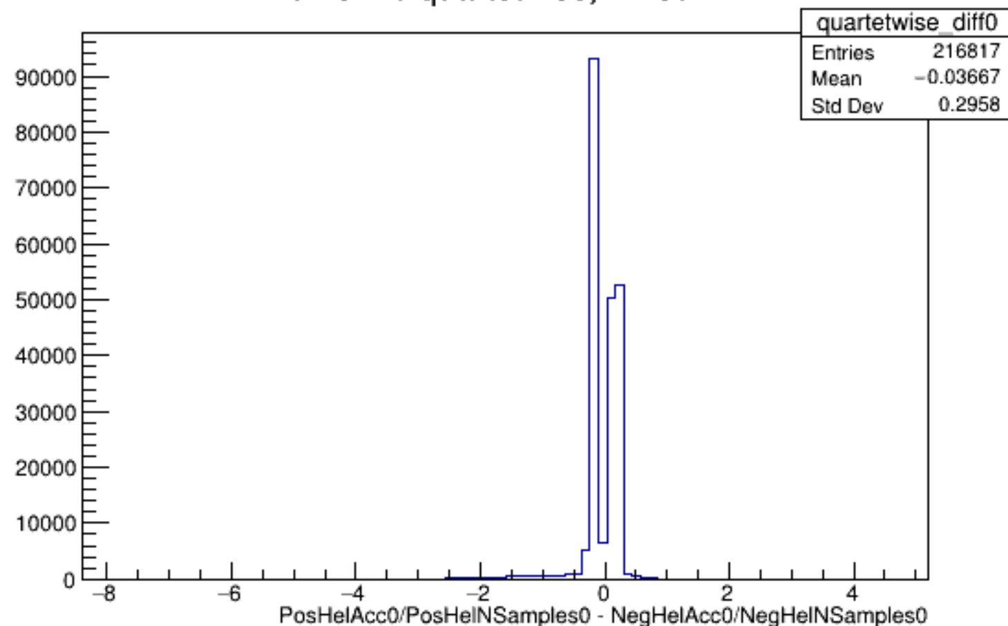
Run 5170 quartetwise, Diffs0: All
