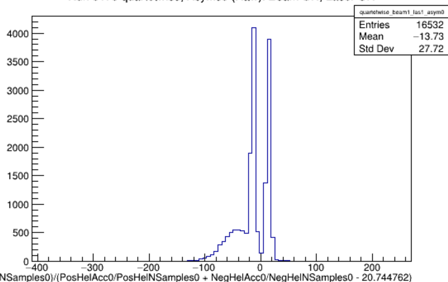
Run 5170 quartetwise, Asyms0 (Raw): Beam ON, Laser ON
