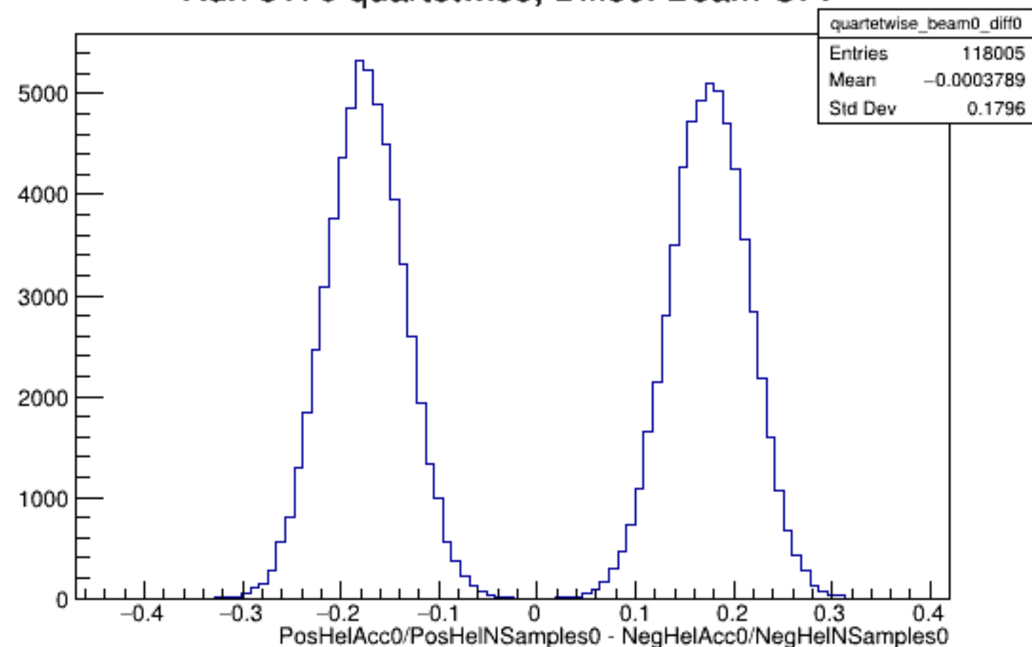
Run 5170 quartetwise, Diffs0: Beam OFF
