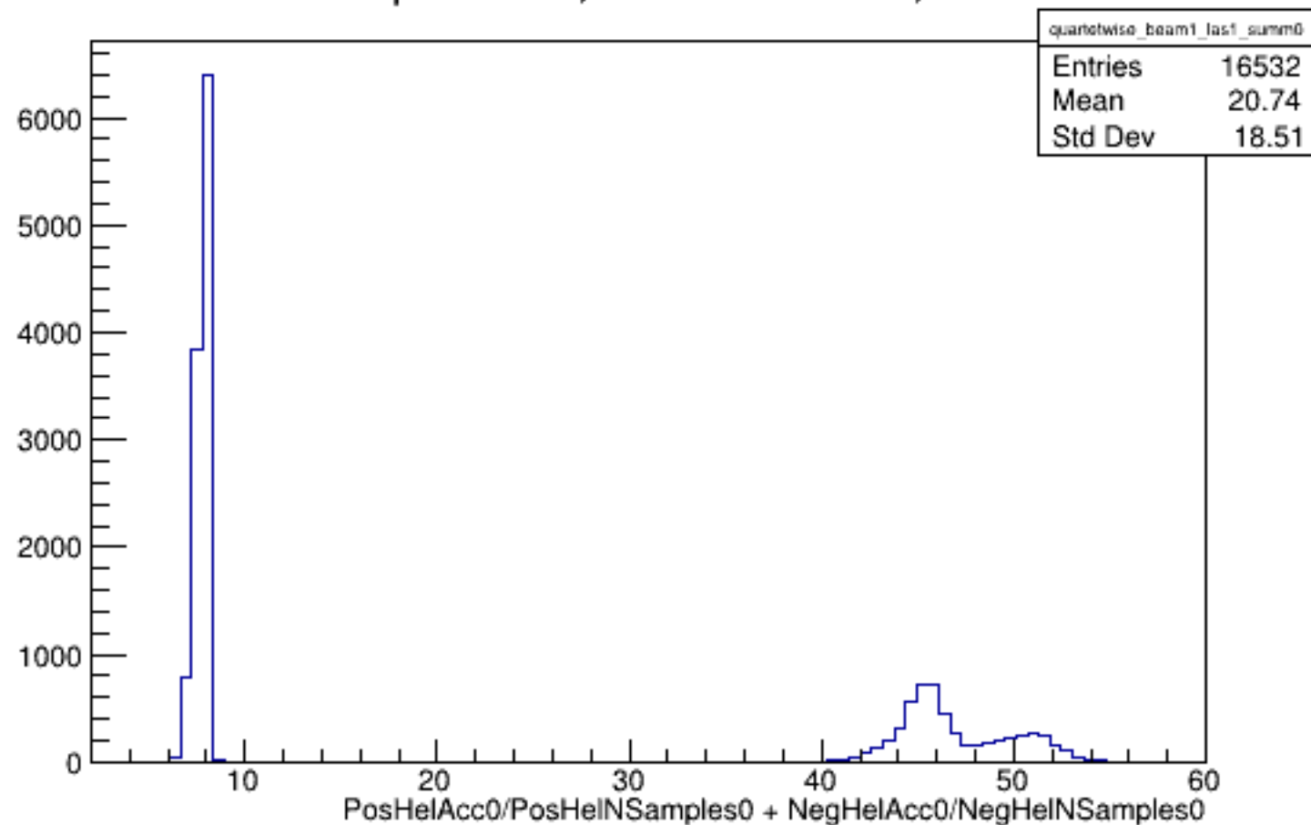
Run 5170 quartetwise, Sums0: Beam ON, Laser ON
