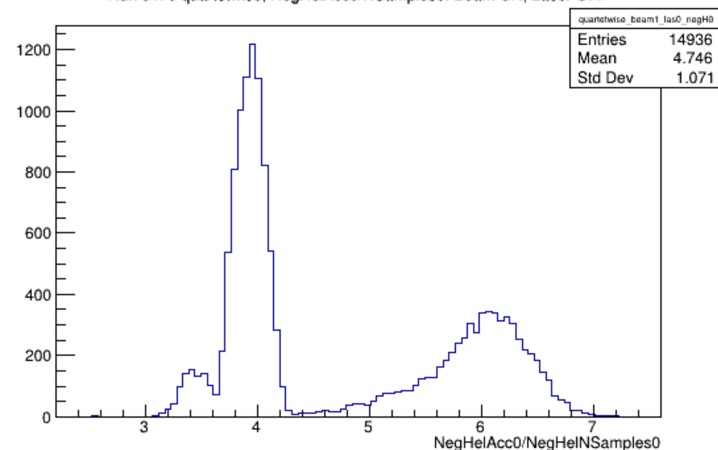
Run 5170 quartetwise, NegHelAcc0/NSamples0: Beam ON, Laser OFF
