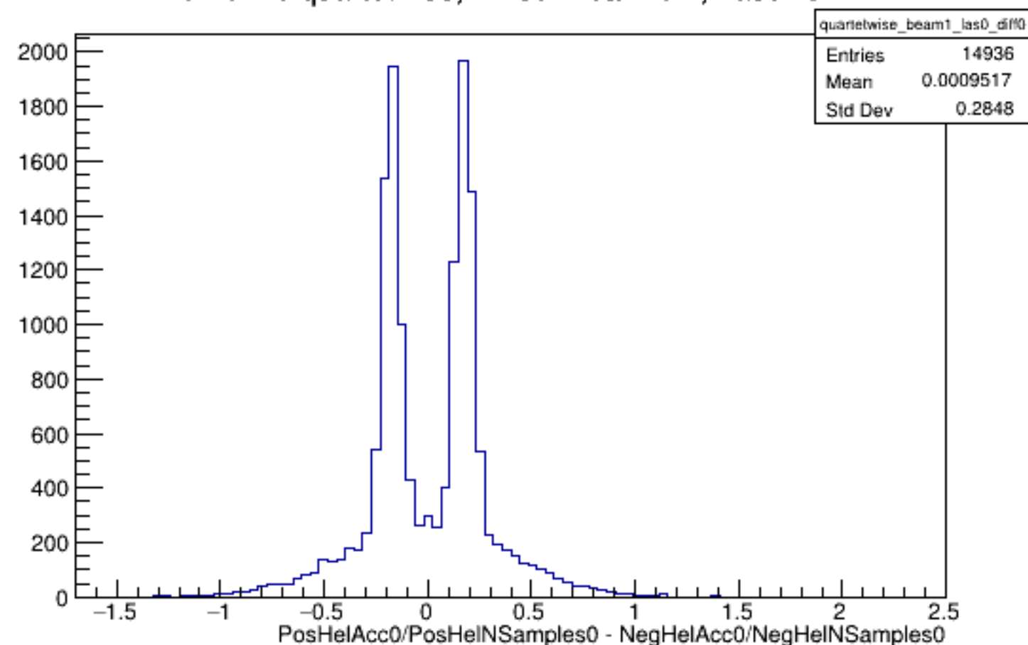
Run 5170 quartetwise, Diffs0: Beam ON, Laser OFF
