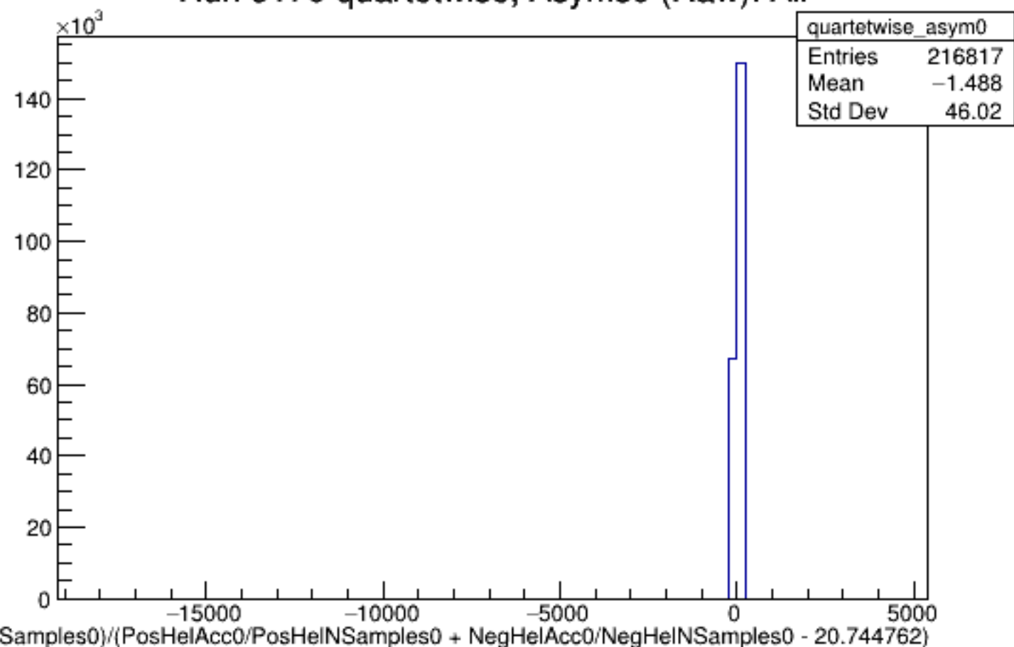
Run 5170 quartetwise, Asyms0 (Raw): All
