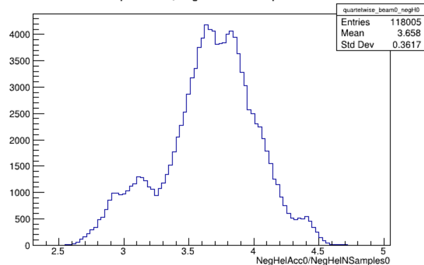
Run 5170 quartetwise, NegHelAcc0/NSamples0: Beam OFF
