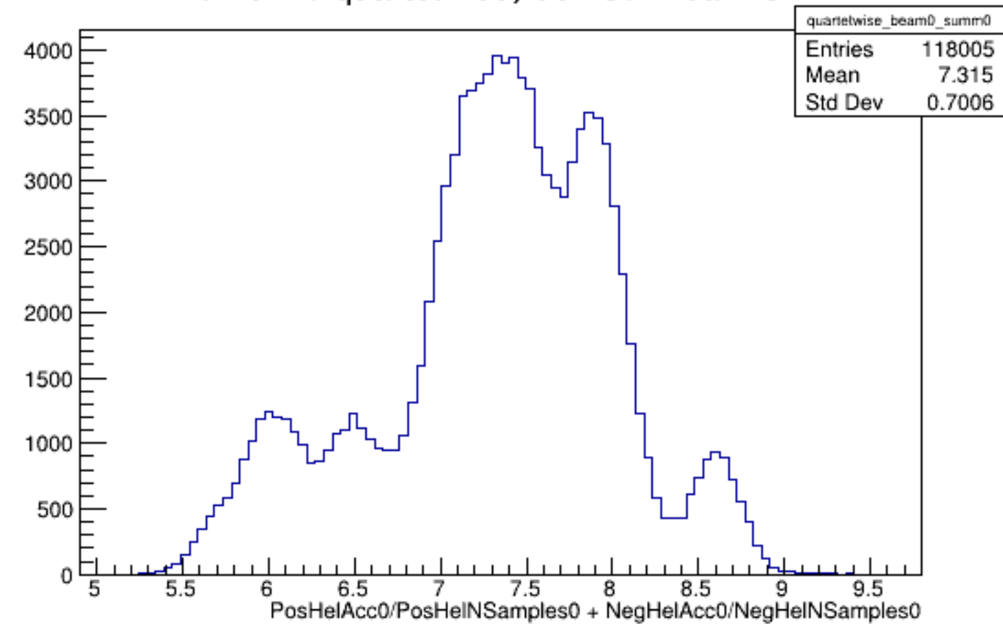
Run 5170 quartetwise, Sums0: Beam OFF
