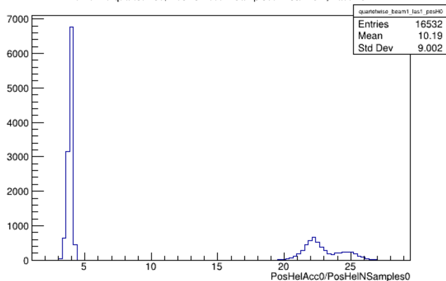
Run 5170 quartetwise, PosHelAcc0/NSamples0: Beam ON, Laser ON
