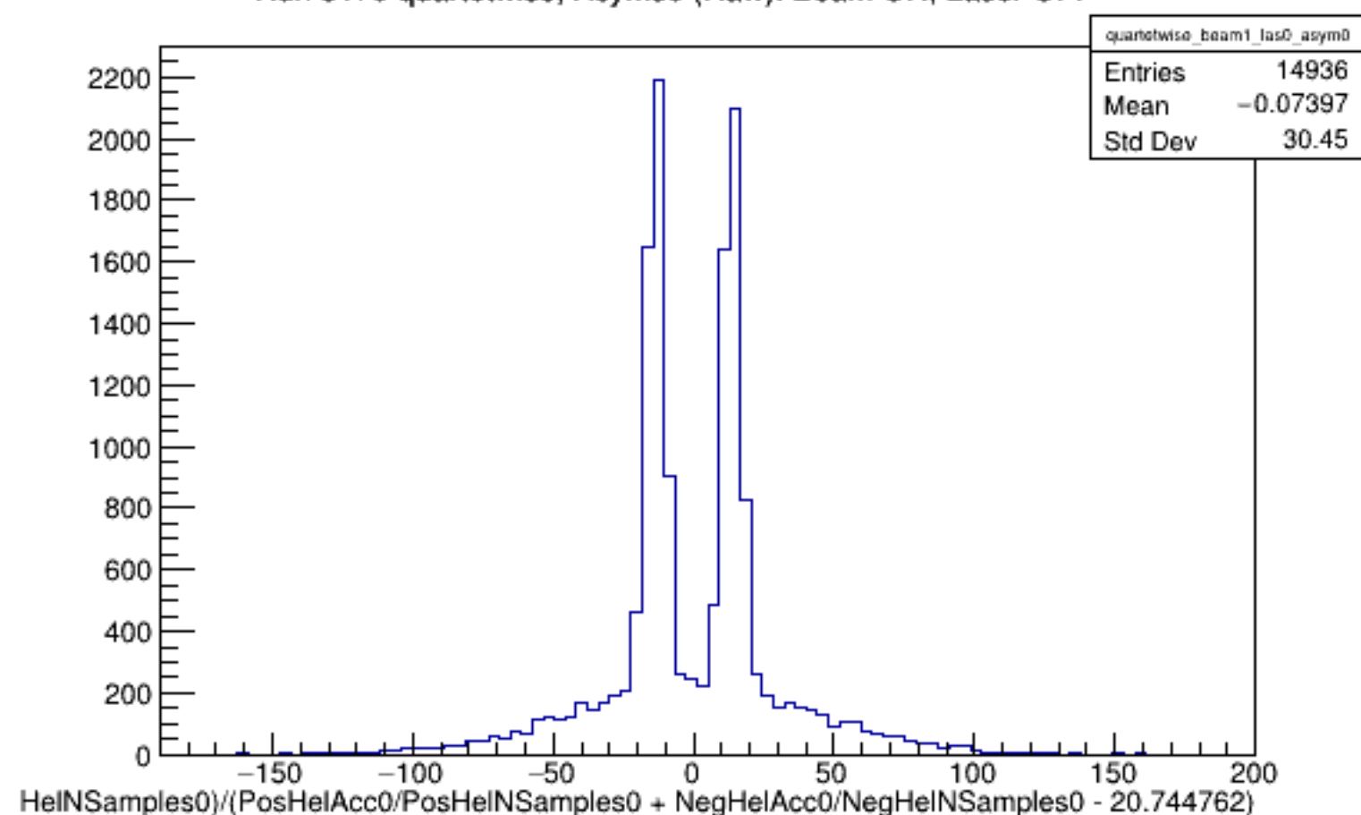
Run 5170 quartetwise, Asyms0 (Raw): Beam ON, Laser OFF
