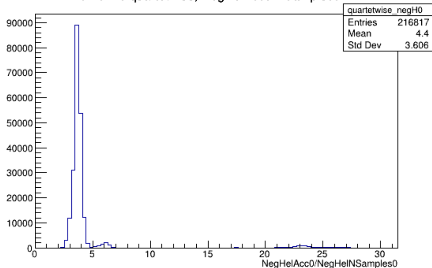
Run 5170 quartetwise, NegHelAcc0/NSamples0: All
