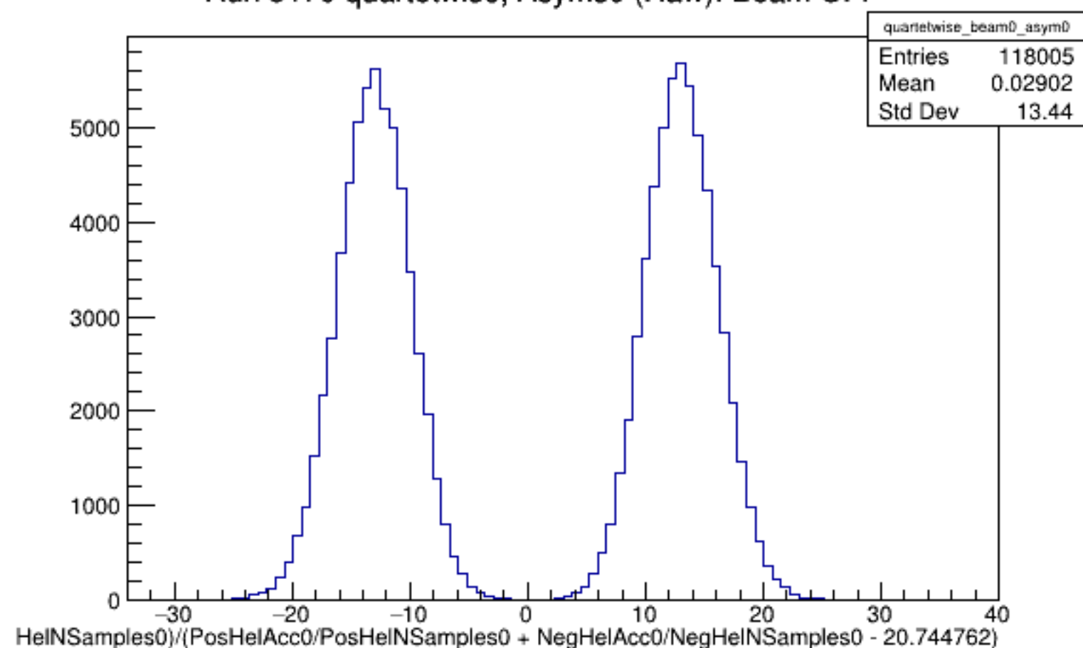
Run 5170 quartetwise, Asyms0 (Raw): Beam OFF
