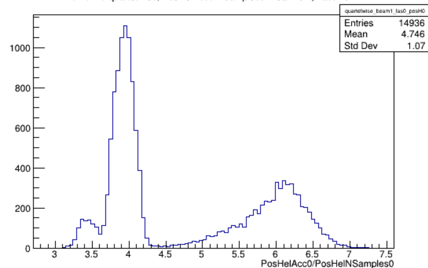
Run 5170 quartetwise, PosHelAcc0/NSamples0: Beam ON, Laser OFF
