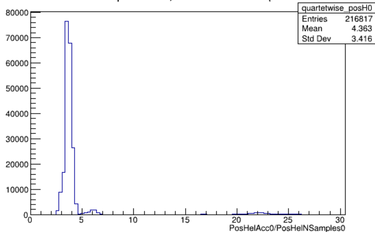
Run 5170 quartetwise, PosHelAcc0/NSamples0: All
