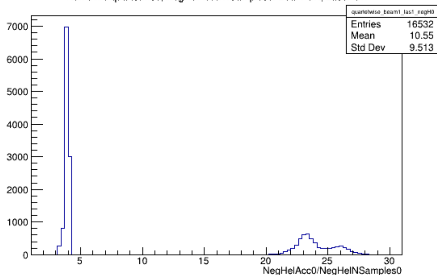
Run 5170 quartetwise, NegHelAcc0/NSamples0: Beam ON, Laser ON
