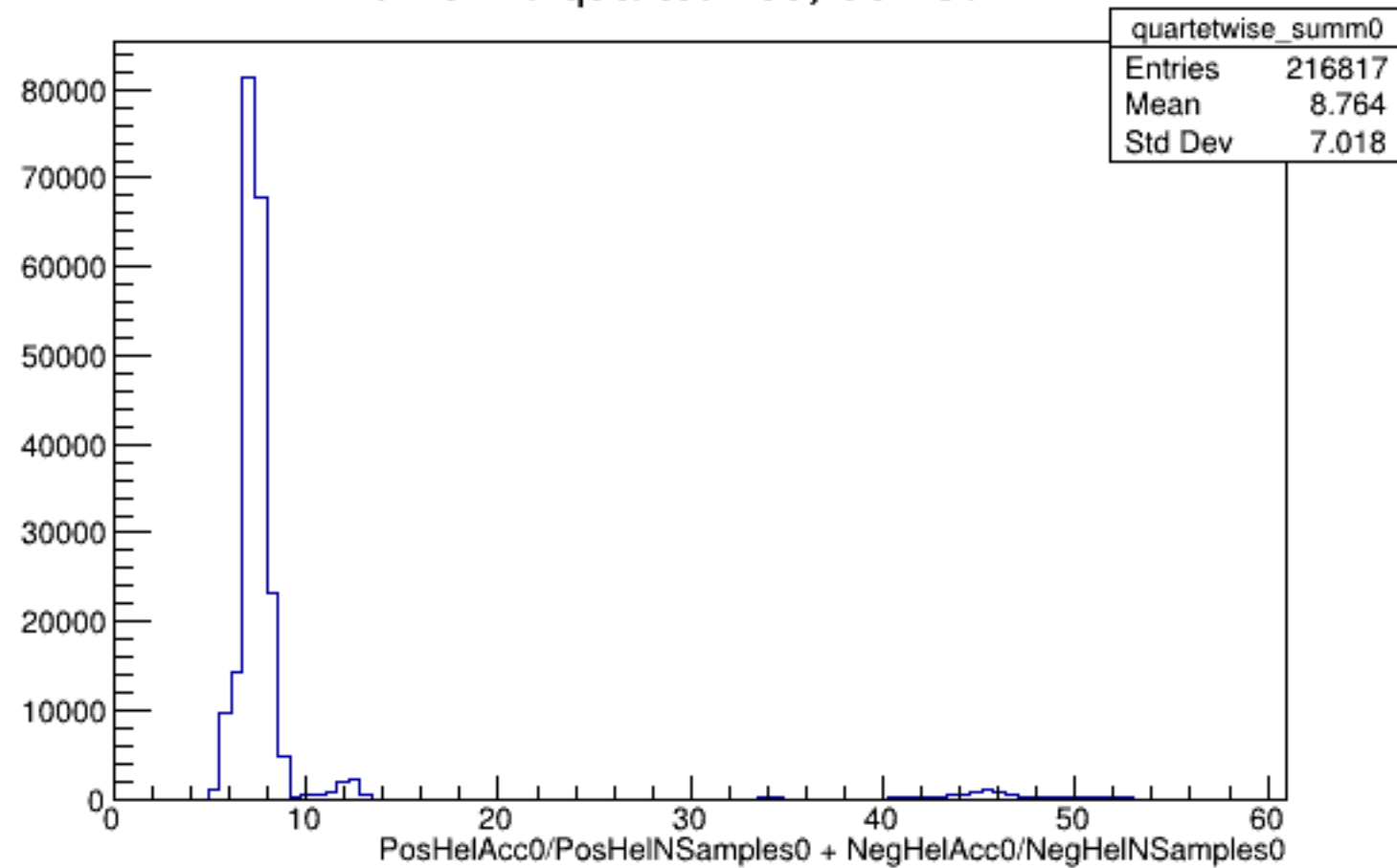
Run 5170 quartetwise, Sums0: All
