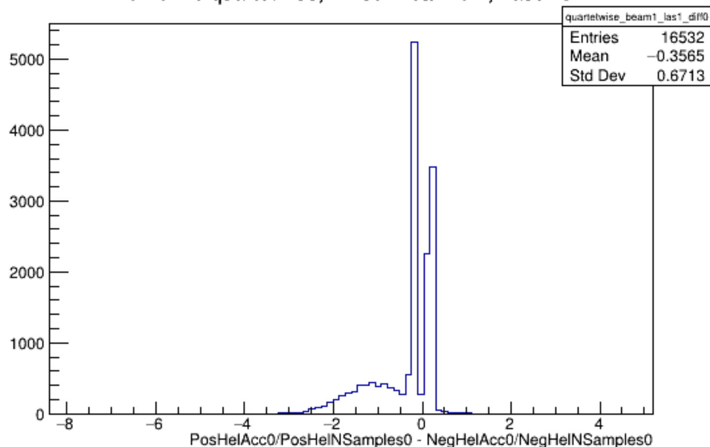
Run 5170 quartetwise, Diffs0: Beam ON, Laser ON
