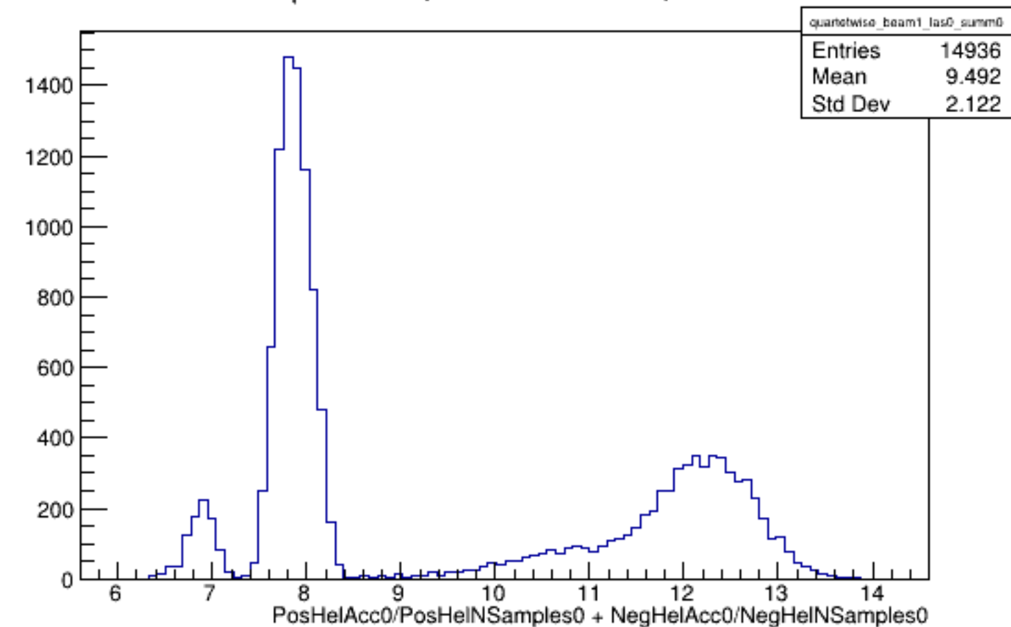
Run 5170 quartetwise, Sums0: Beam ON, Laser OFF
