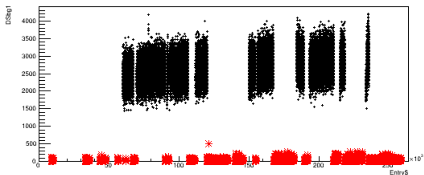
Run 5172, quartetwise: DSbg1 vs time
