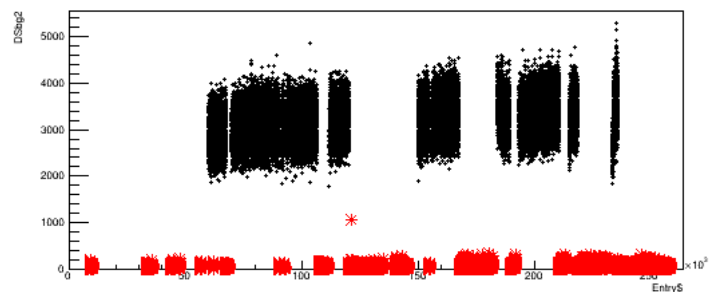
Run 5172, quartetwise: DSbg2 vs time
