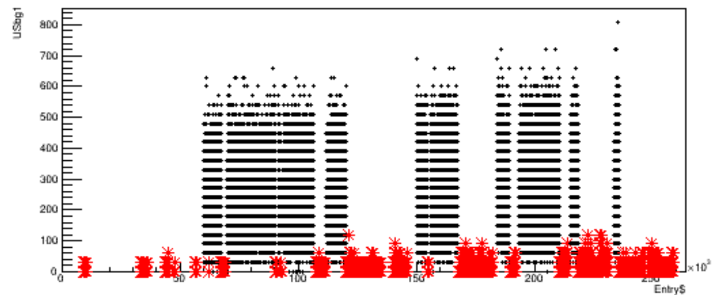
Run 5172, quartetwise: USbg1 vs time
