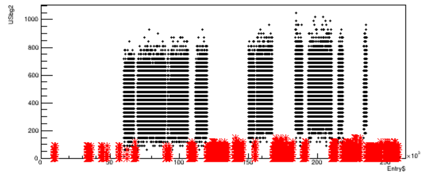
Run 5172, quartetwise: USbg2 vs time
