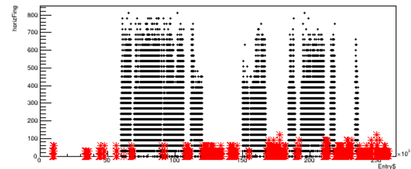
Run 5172, quartetwise: horizFing vs time
