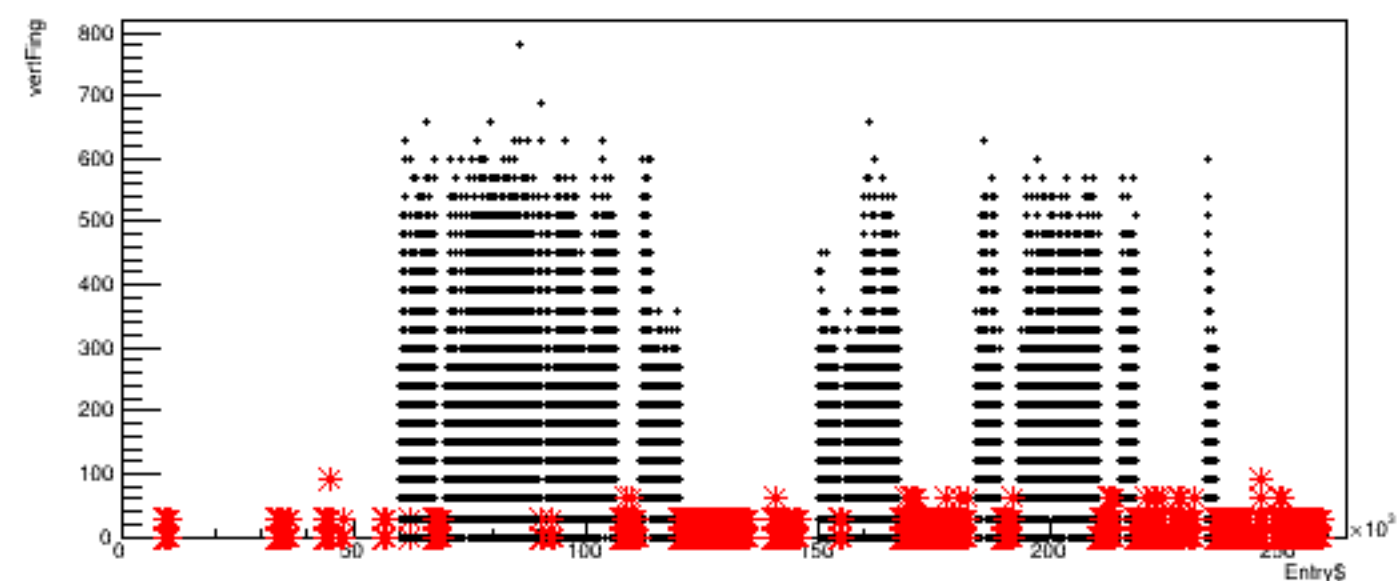
Run 5172, quartetwise: vertFing vs time
