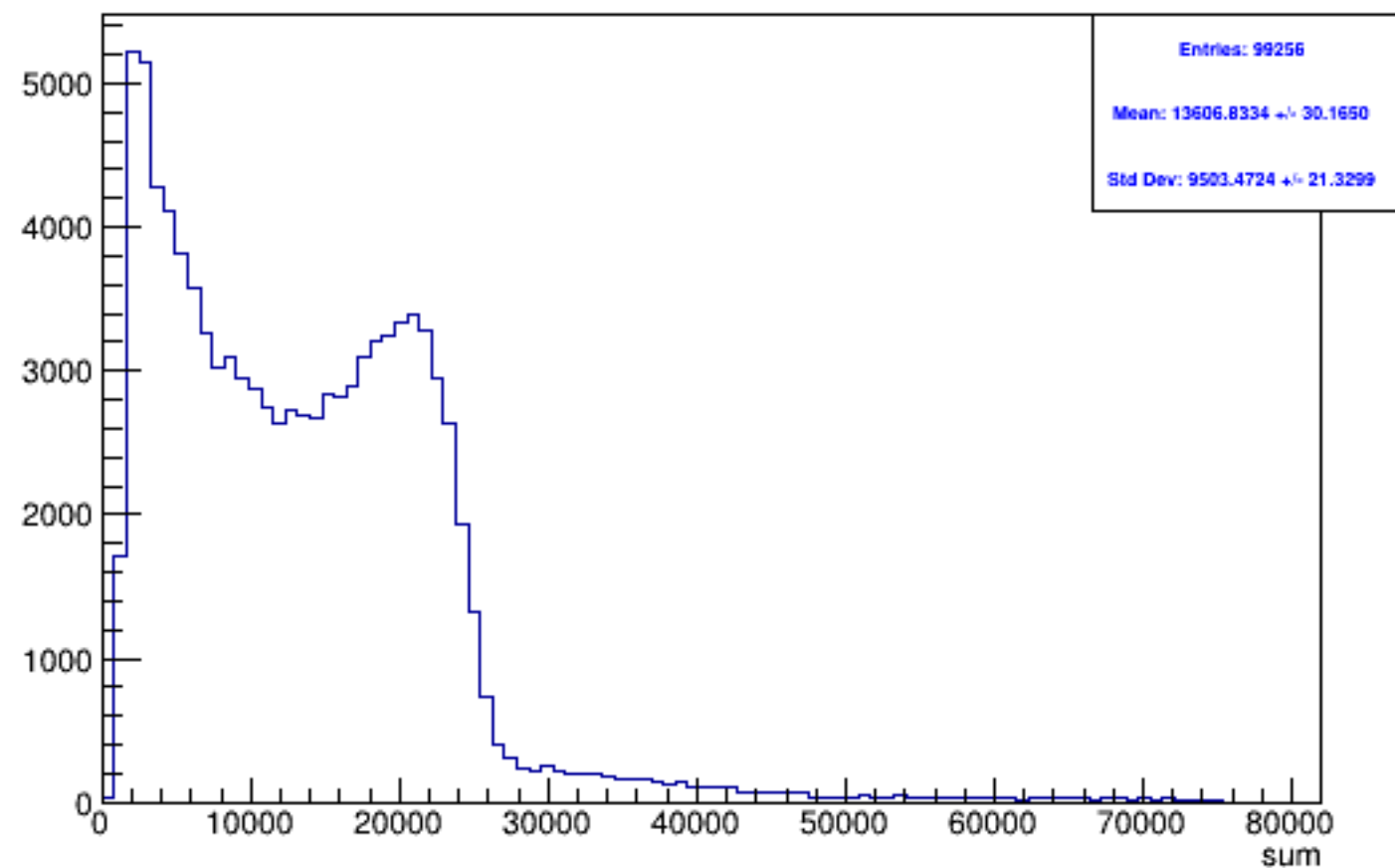
Run 5173 triggerwise, sums: All
