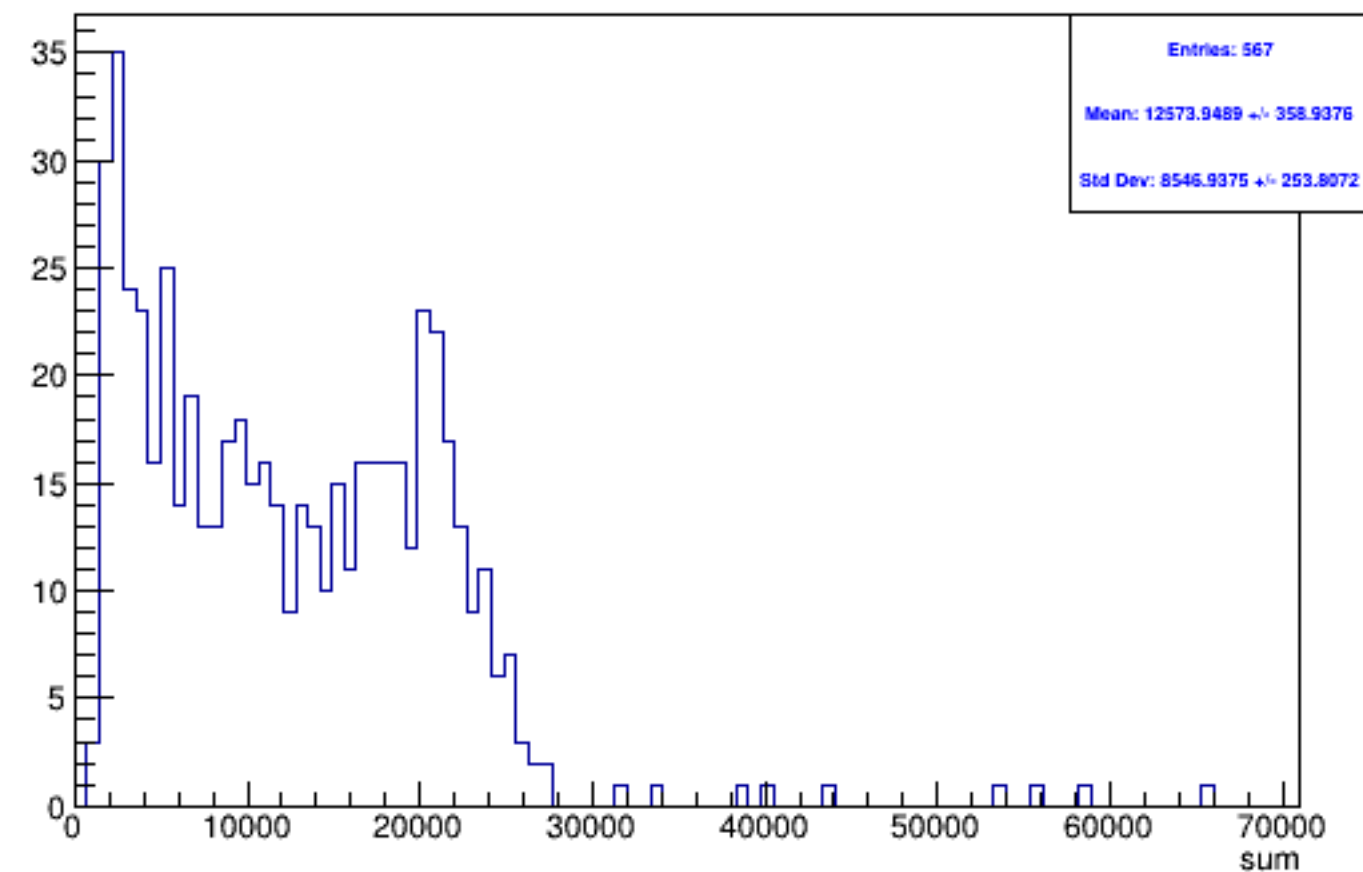
Run 5173 triggerwise, sums: Beam OFF
