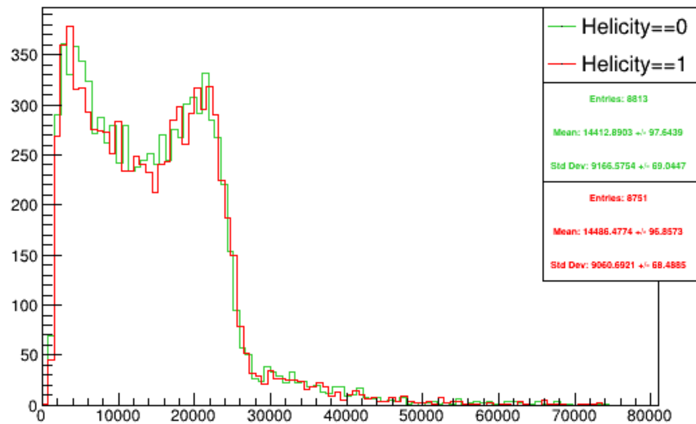
Run 5173 triggerwise, sums: Beam ON, Laser ON
