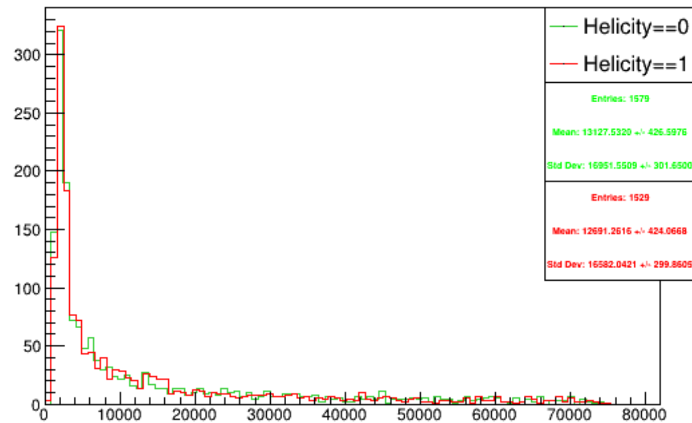
Run 5173 triggerwise, sums: Beam ON, Laser OFF
