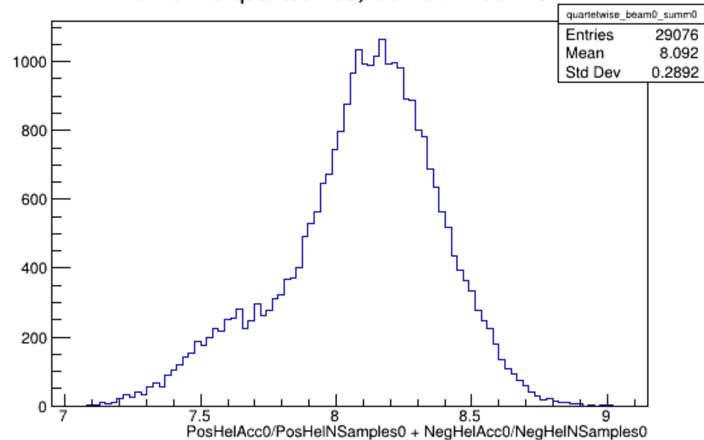
Run 5175 quartetwise, Sums0: Beam OFF
