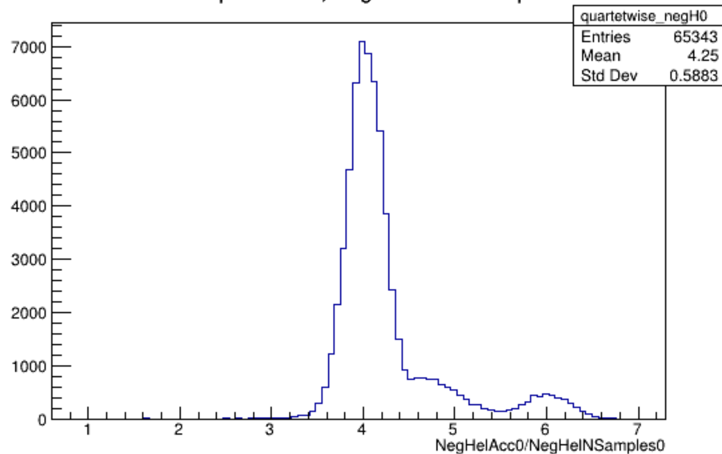
Run 5175 quartetwise, NegHelAcc0/NSamples0: All
