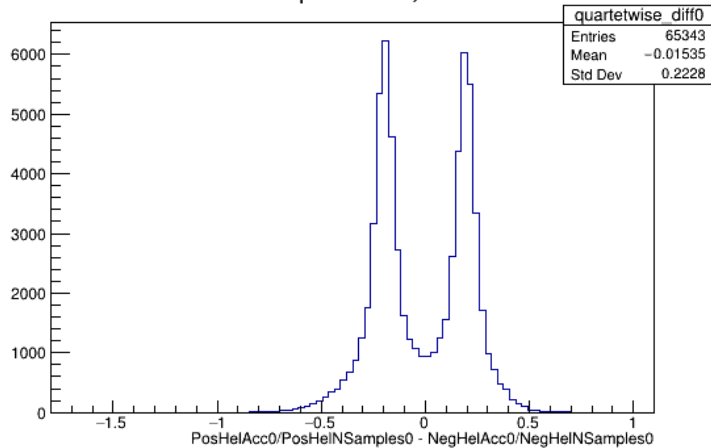
Run 5175 quartetwise, Diffs0: All
