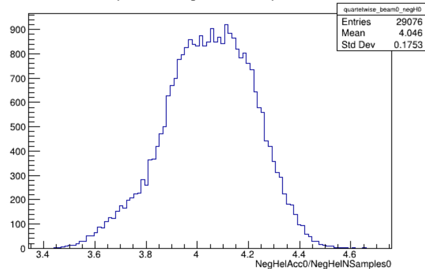
Run 5175 quartetwise, NegHelAcc0/NSamples0: Beam OFF
