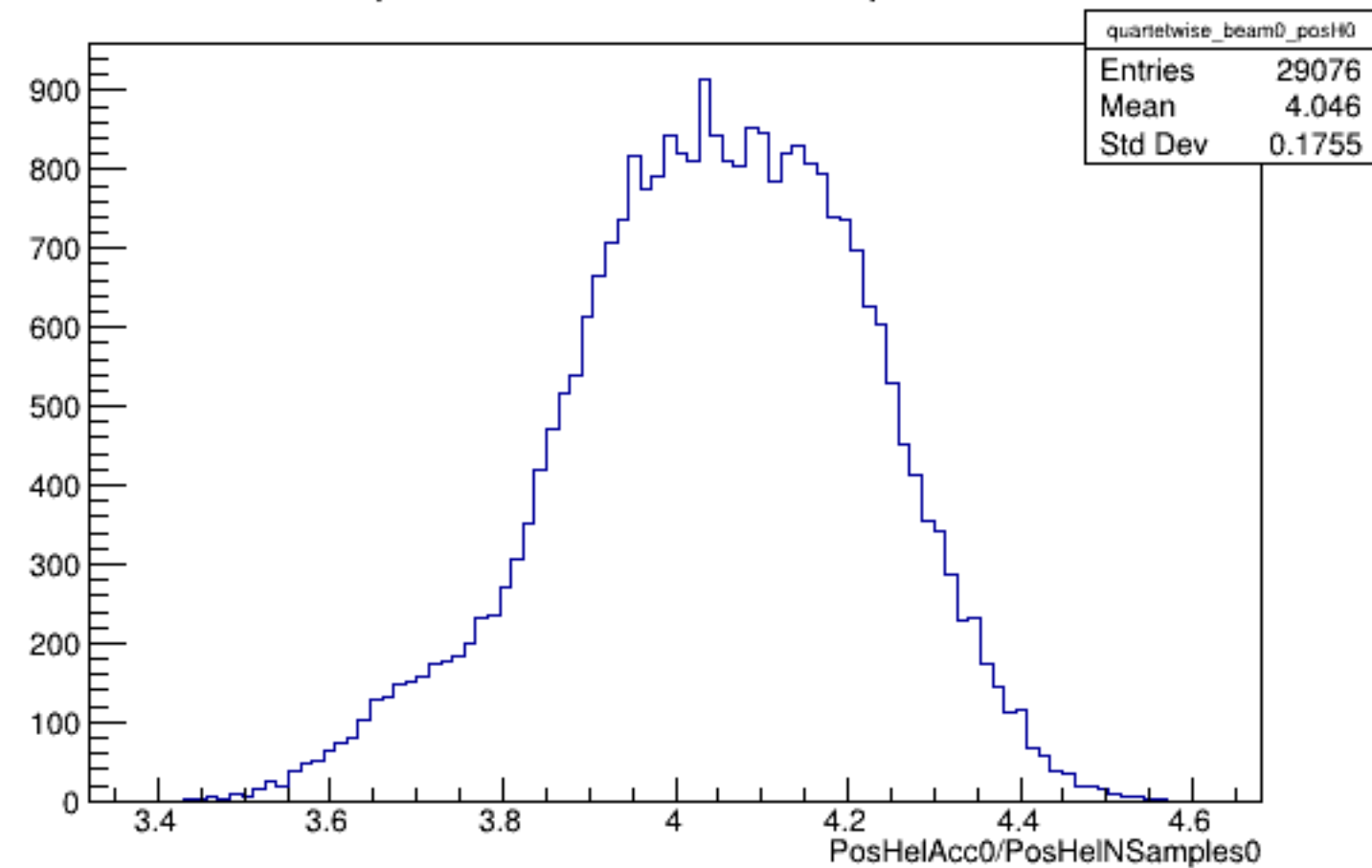
Run 5175 quartetwise, PosHelAcc0/NSamples0: Beam OFF
