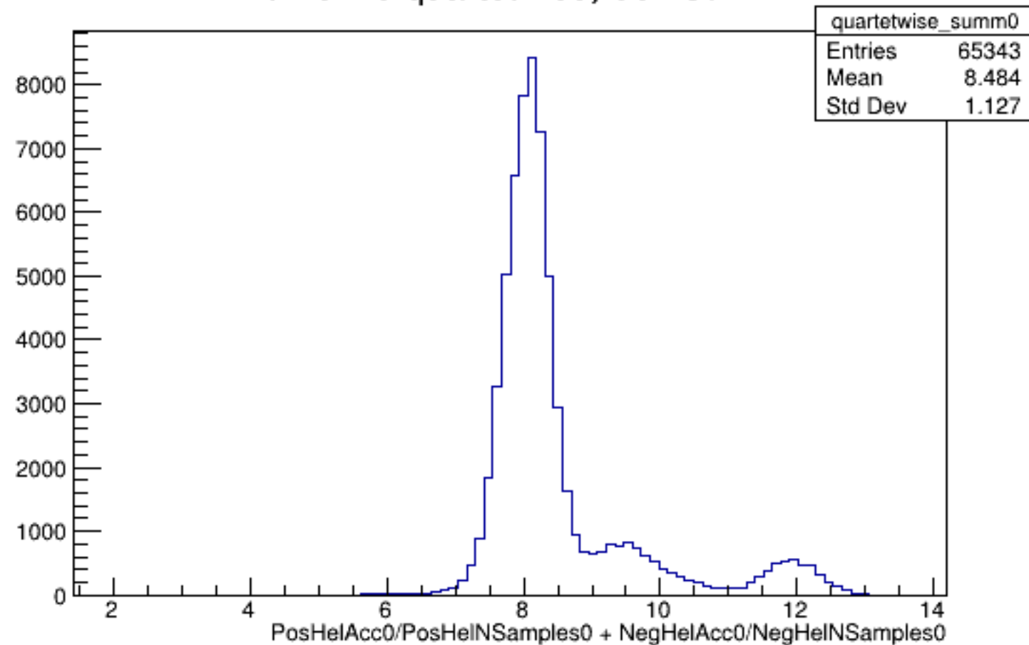
Run 5175 quartetwise, Sums0: All
