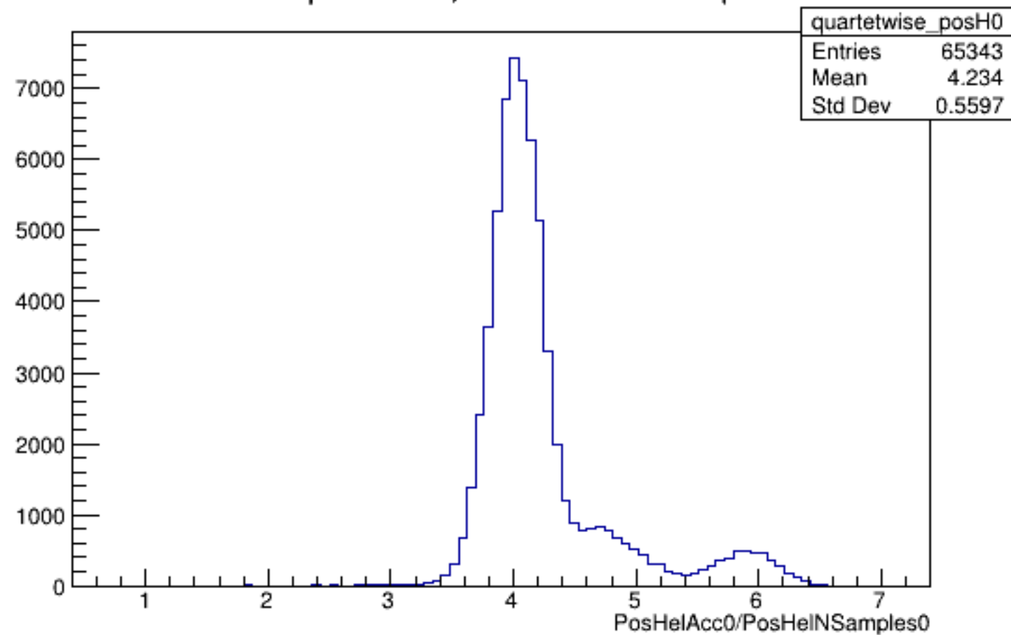
Run 5175 quartetwise, PosHelAcc0/NSamples0: All
