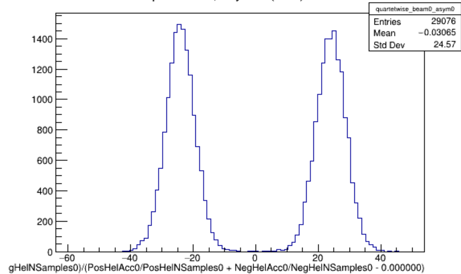
Run 5175 quartetwise, Asyms0 (Raw): Beam OFF
