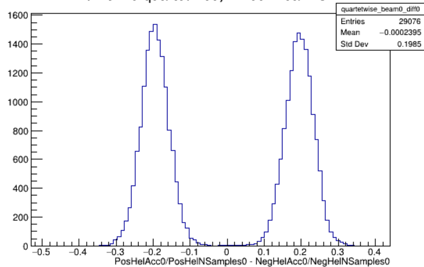
Run 5175 quartetwise, Diffs0: Beam OFF
