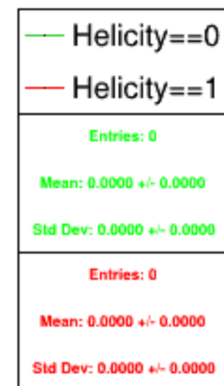
Run 5175 triggerwise, sums: Beam ON, Laser OFF
