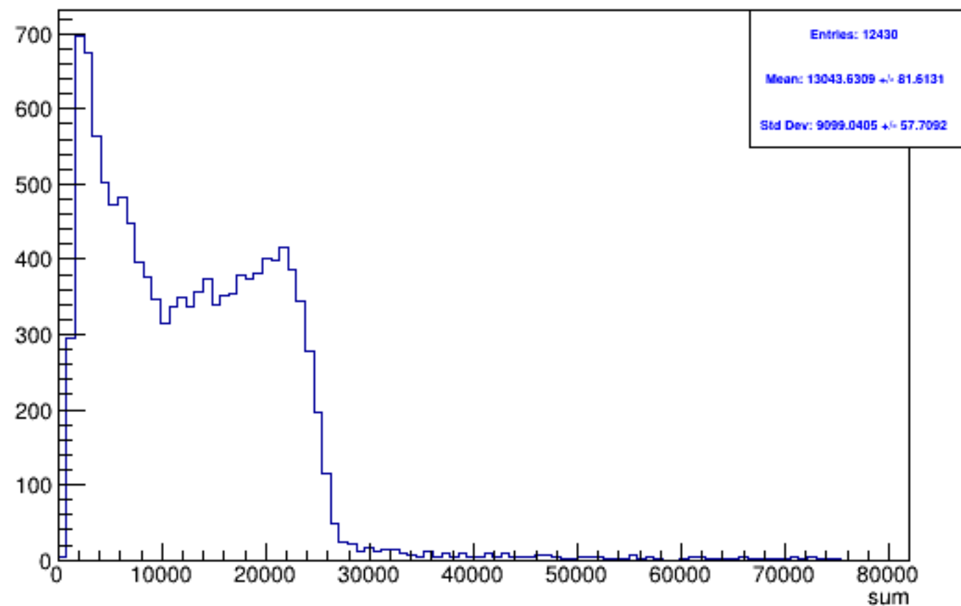
Run 5175 triggerwise, sums: All
