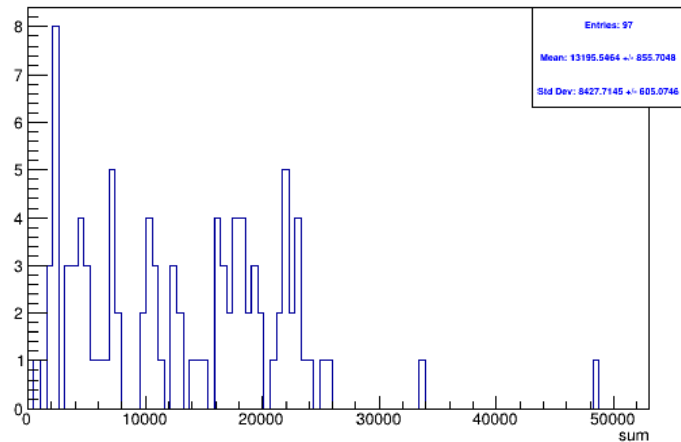
Run 5175 triggerwise, sums: Beam OFF
