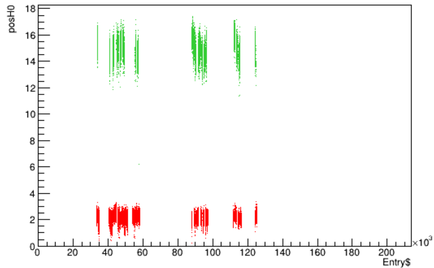
Run 5177 quartetwise, posH0 vs time
