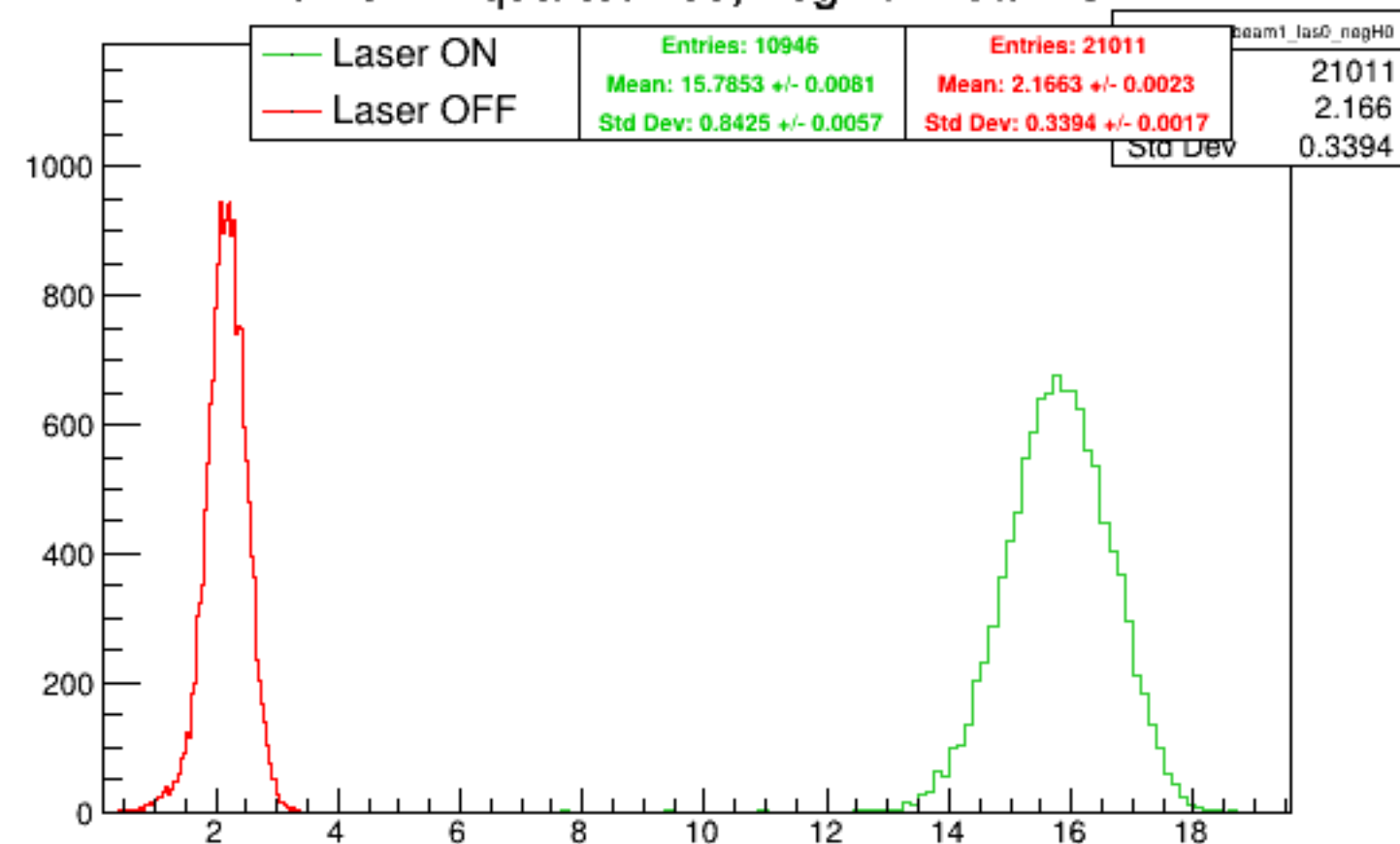
Run 5177 quartetwise, negH0: Beam ON
