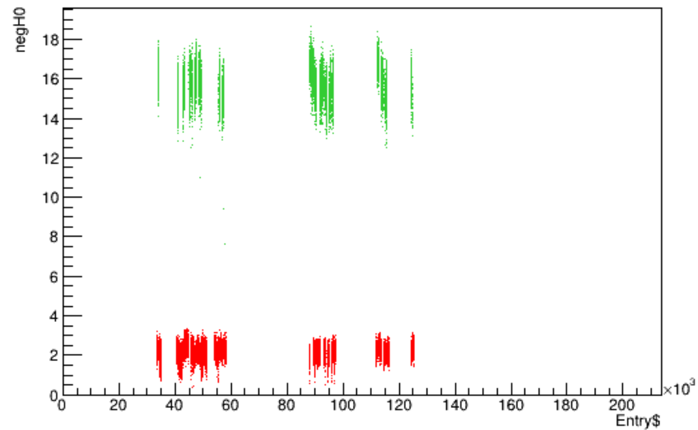
Run 5177 quartetwise, negH0 vs time
