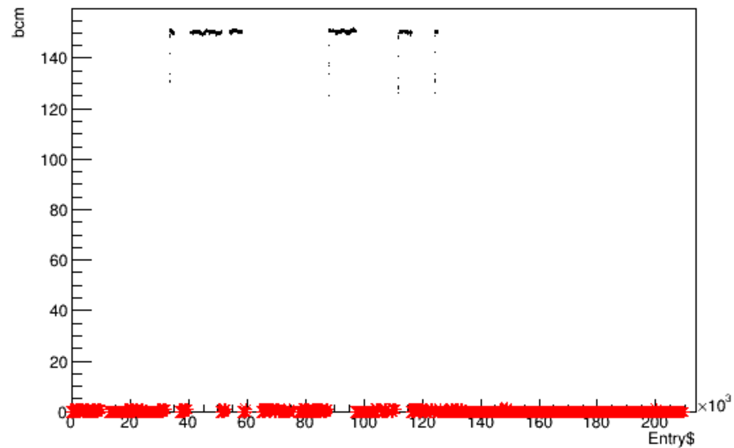
Run 5177 quartetwise, bcm vs time
