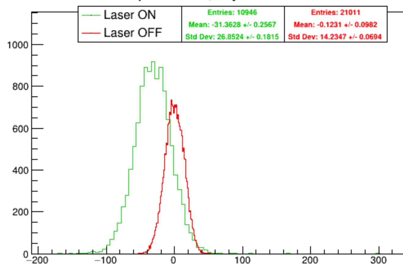
Run 5177 quartetwise, asym0sub: Beam ON
