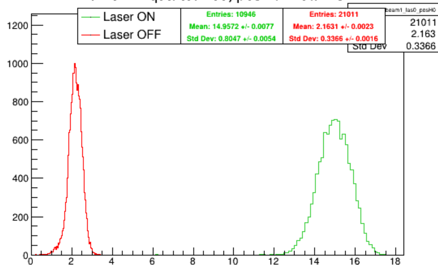
Run 5177 quartetwise, posH0: Beam ON
