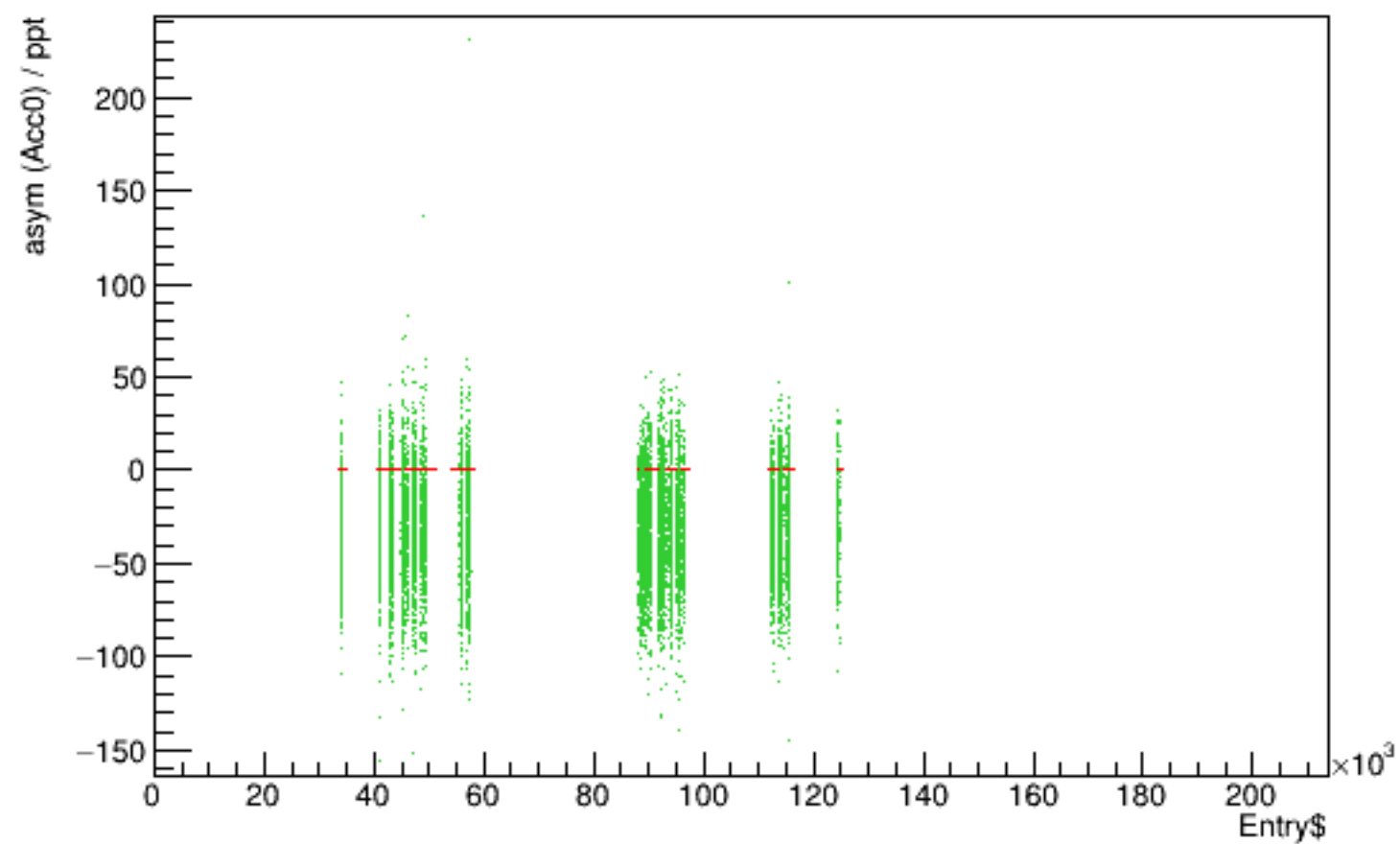
Run 5177 quartetwise, asym0sub vs time
