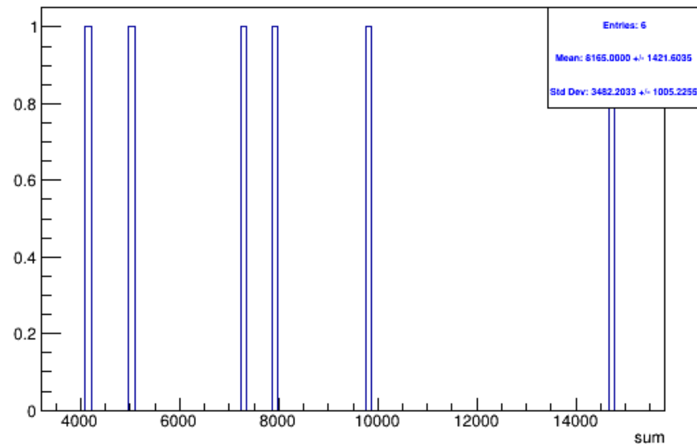
Run 5179 triggerwise, sums: Beam OFF
