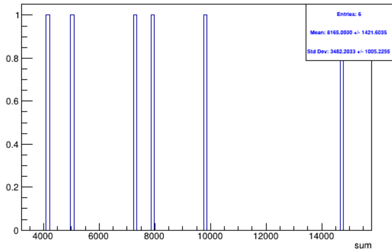
Run 5179 triggerwise, sums: All
