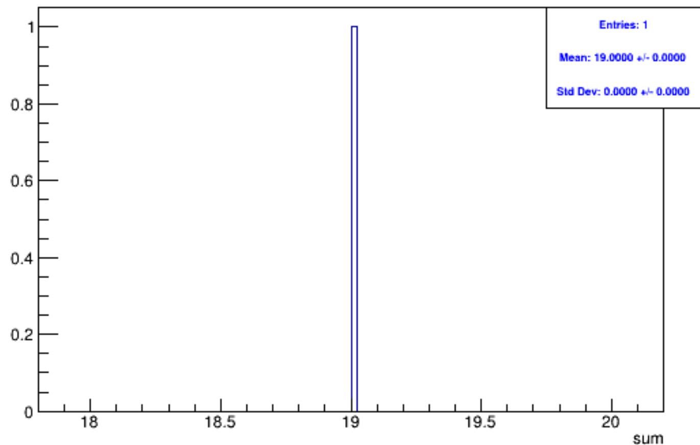
Run 5192 triggerwise, sums: All
