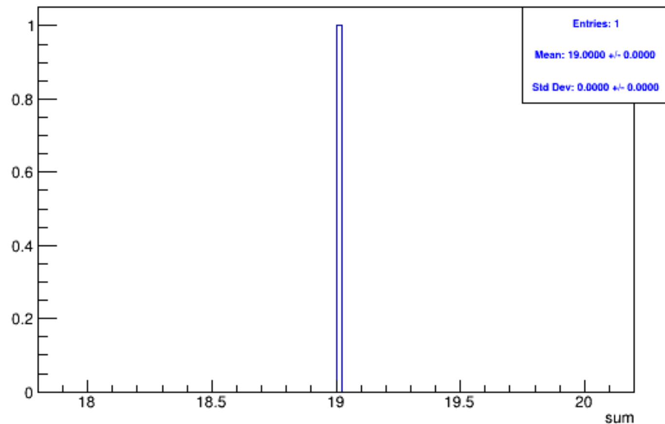
Run 5192 triggerwise, sums: Beam OFF
