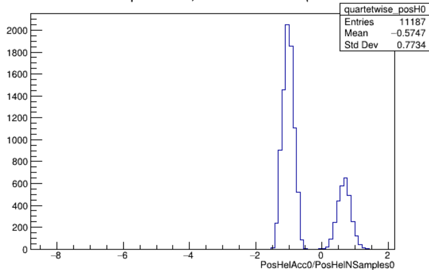
Run 5194 quartetwise, PosHelAcc0/NSamples0: All
