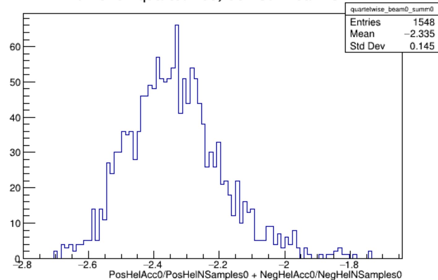
Run 5194 quartetwise, Sums0: Beam OFF
