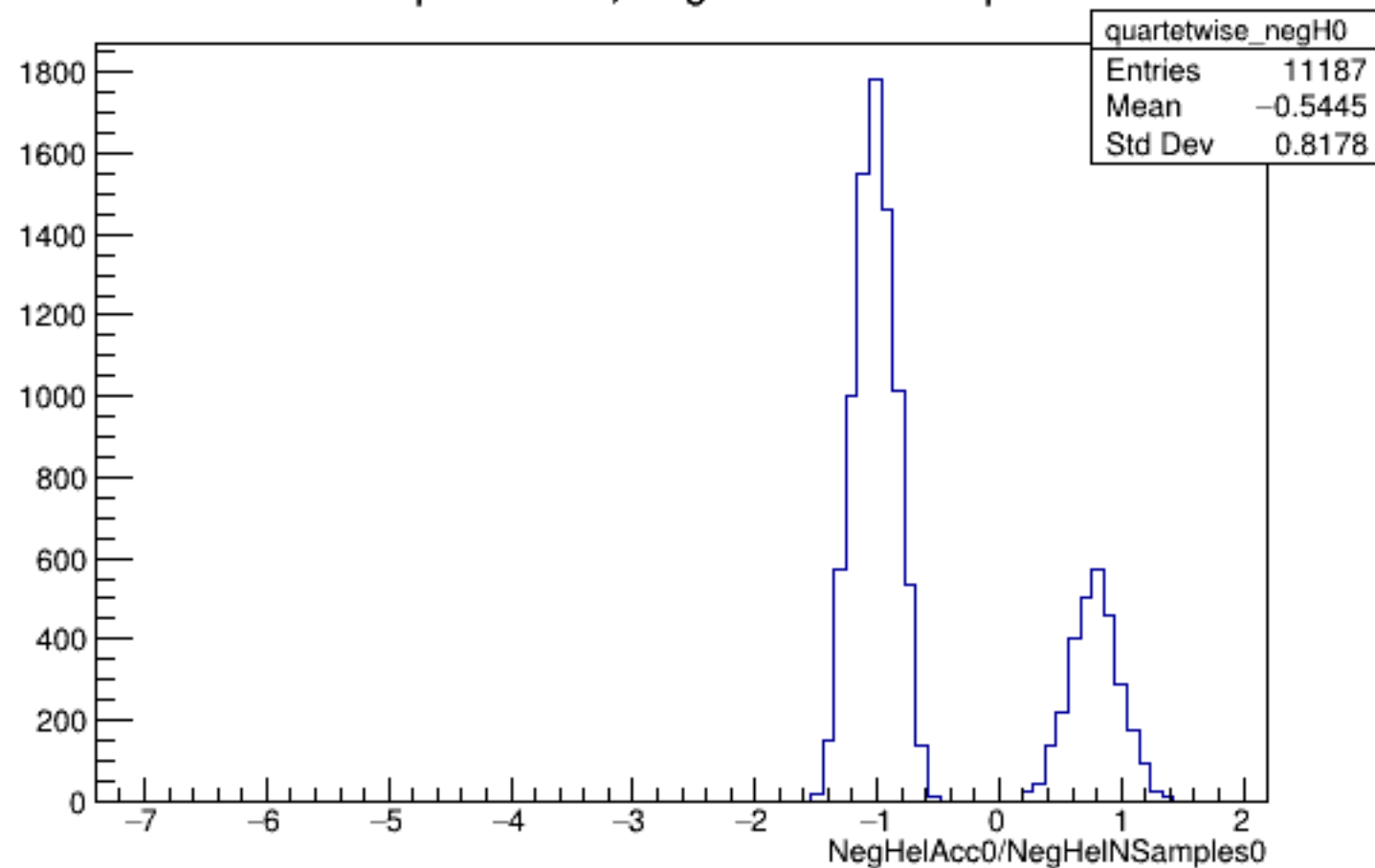
Run 5194 quartetwise, NegHelAcc0/NSamples0: All
