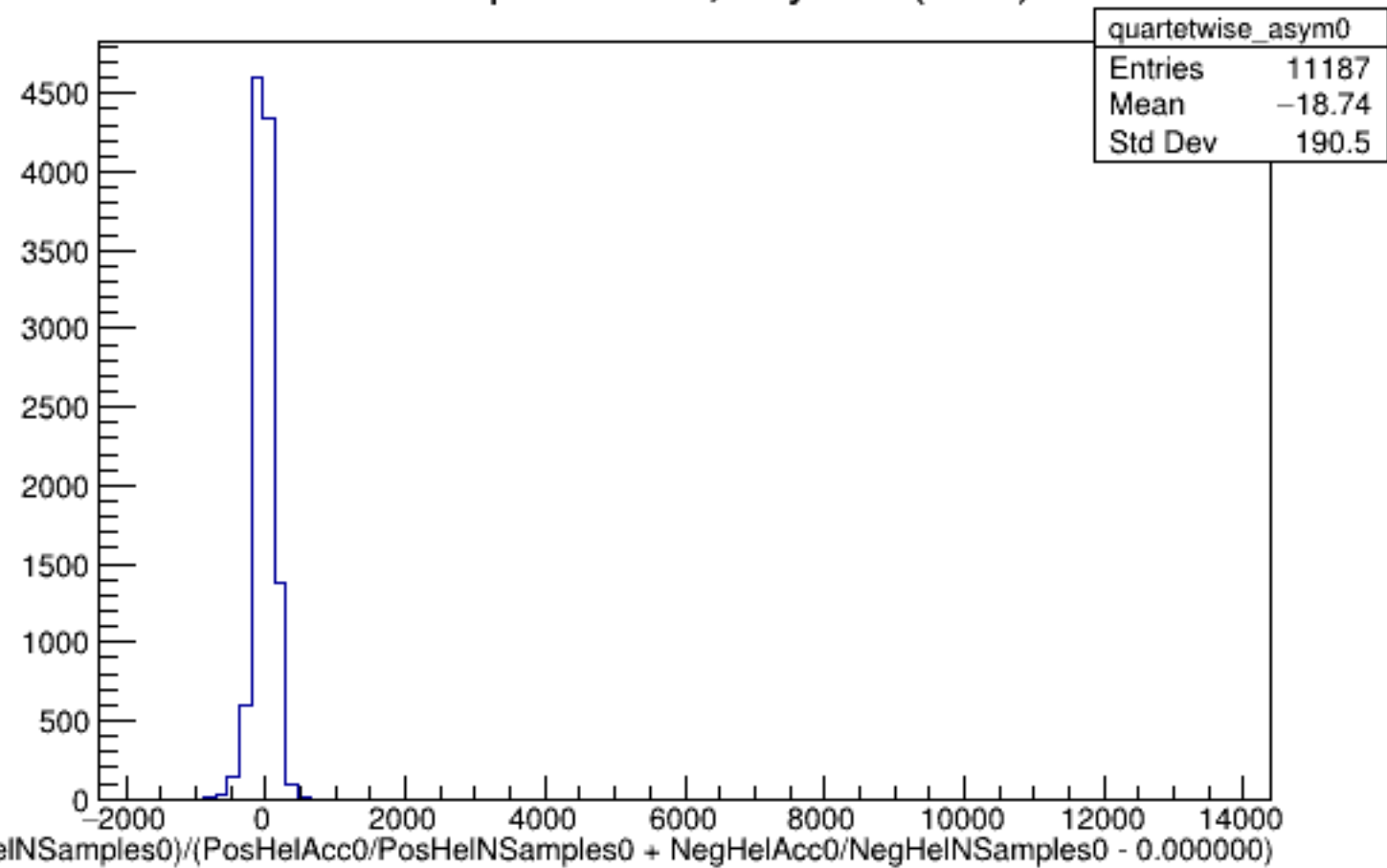
Run 5194 quartetwise, Asyms0 (Raw): All
