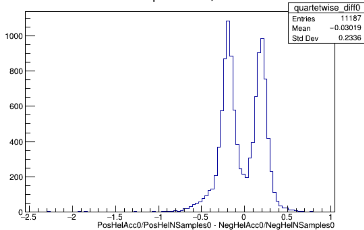
Run 5194 quartetwise, Diffs0: All
