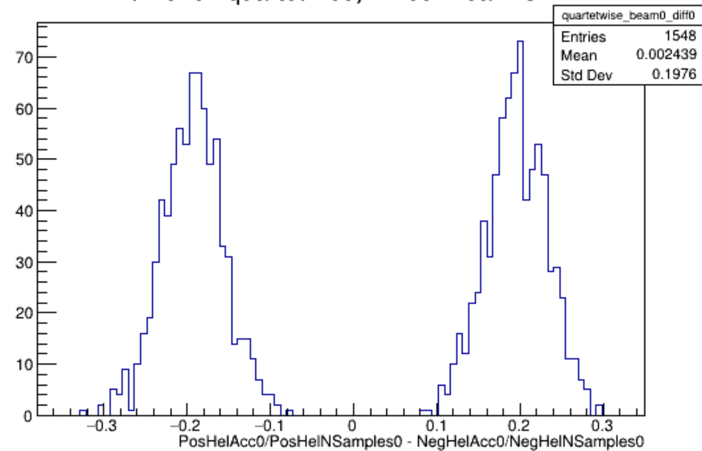
Run 5194 quartetwise, Diffs0: Beam OFF
