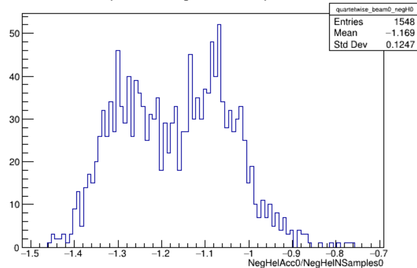
Run 5194 quartetwise, NegHelAcc0/NSamples0: Beam OFF
