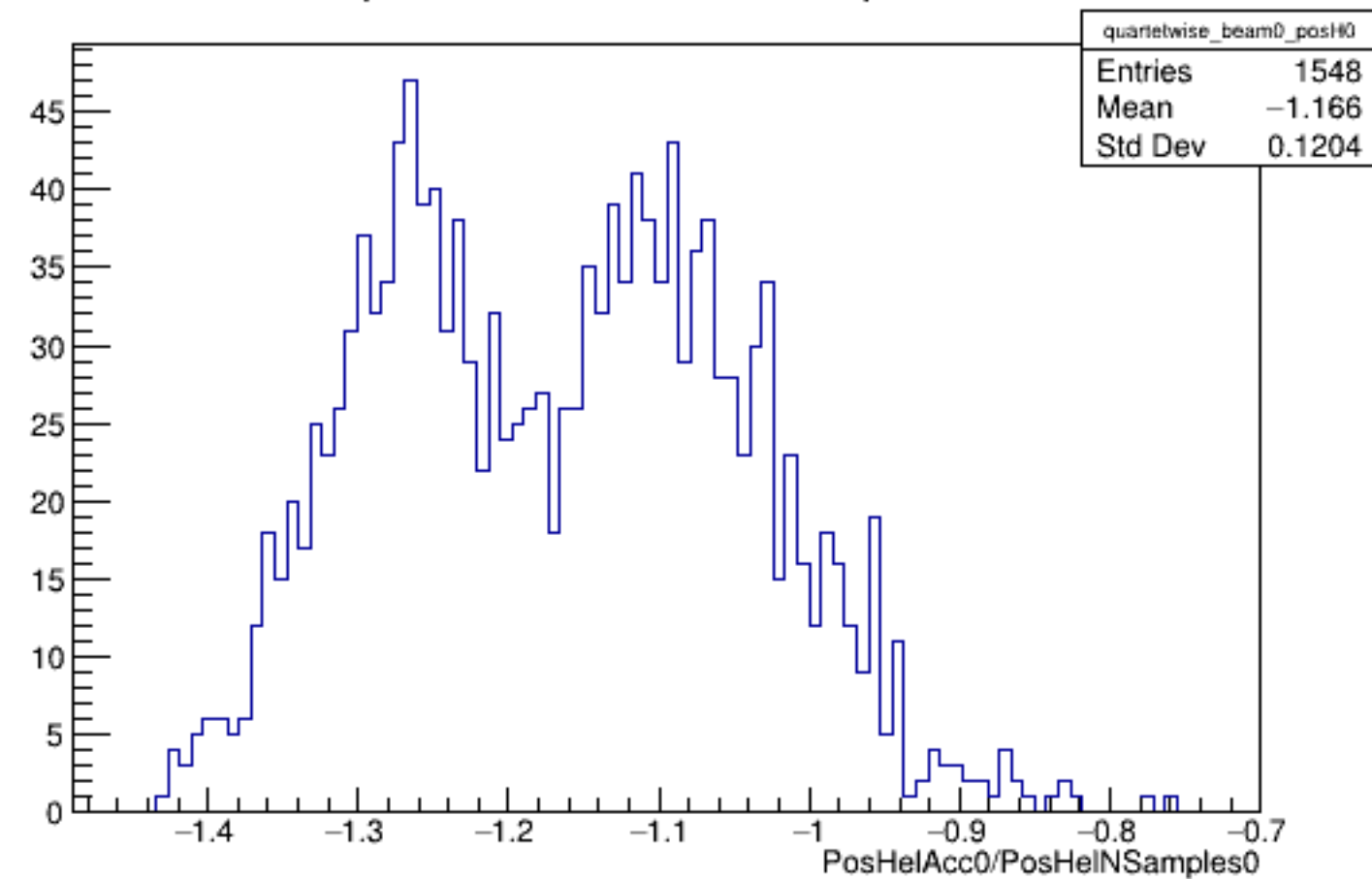
Run 5194 quartetwise, PosHelAcc0/NSamples0: Beam OFF
