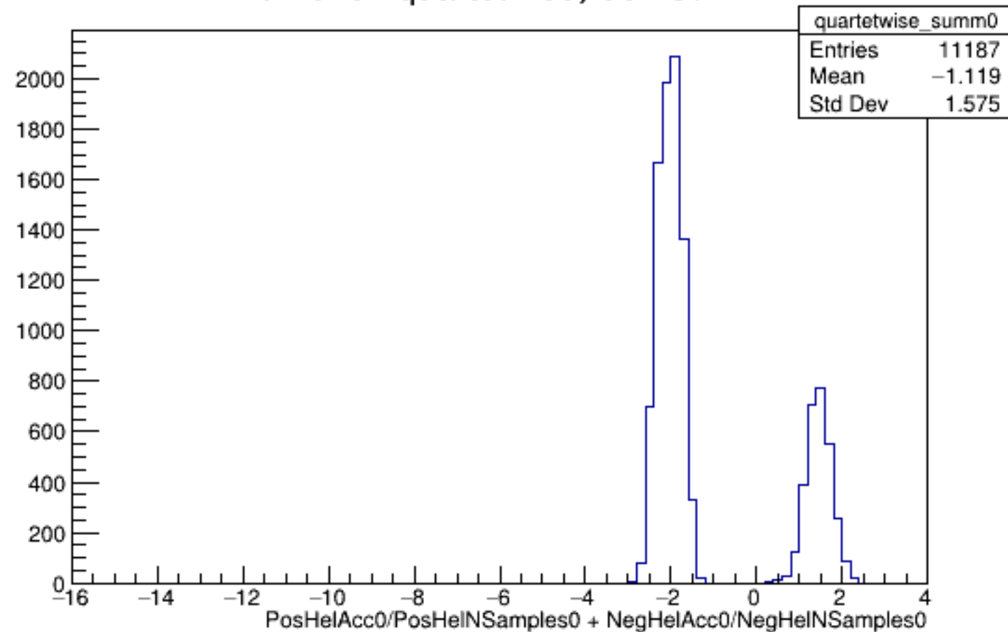
Run 5194 quartetwise, Sums0: All
