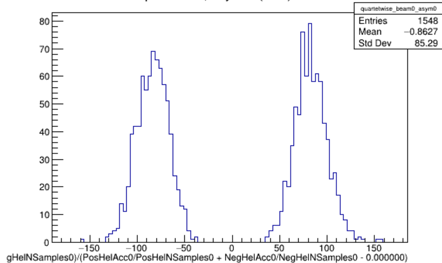
Run 5194 quartetwise, Asyms0 (Raw): Beam OFF
