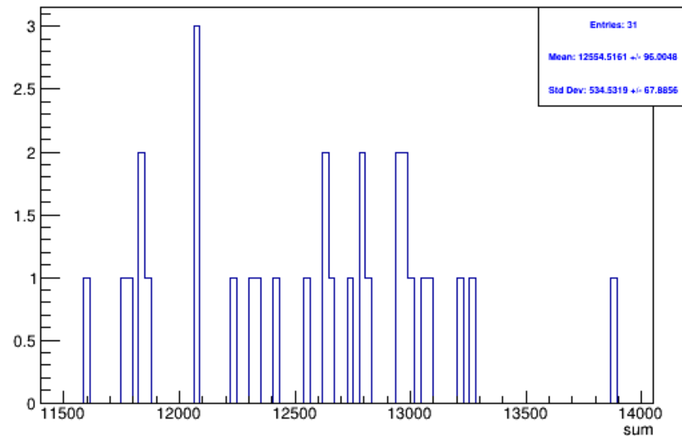
Run 5194 triggerwise, sums: Beam OFF
