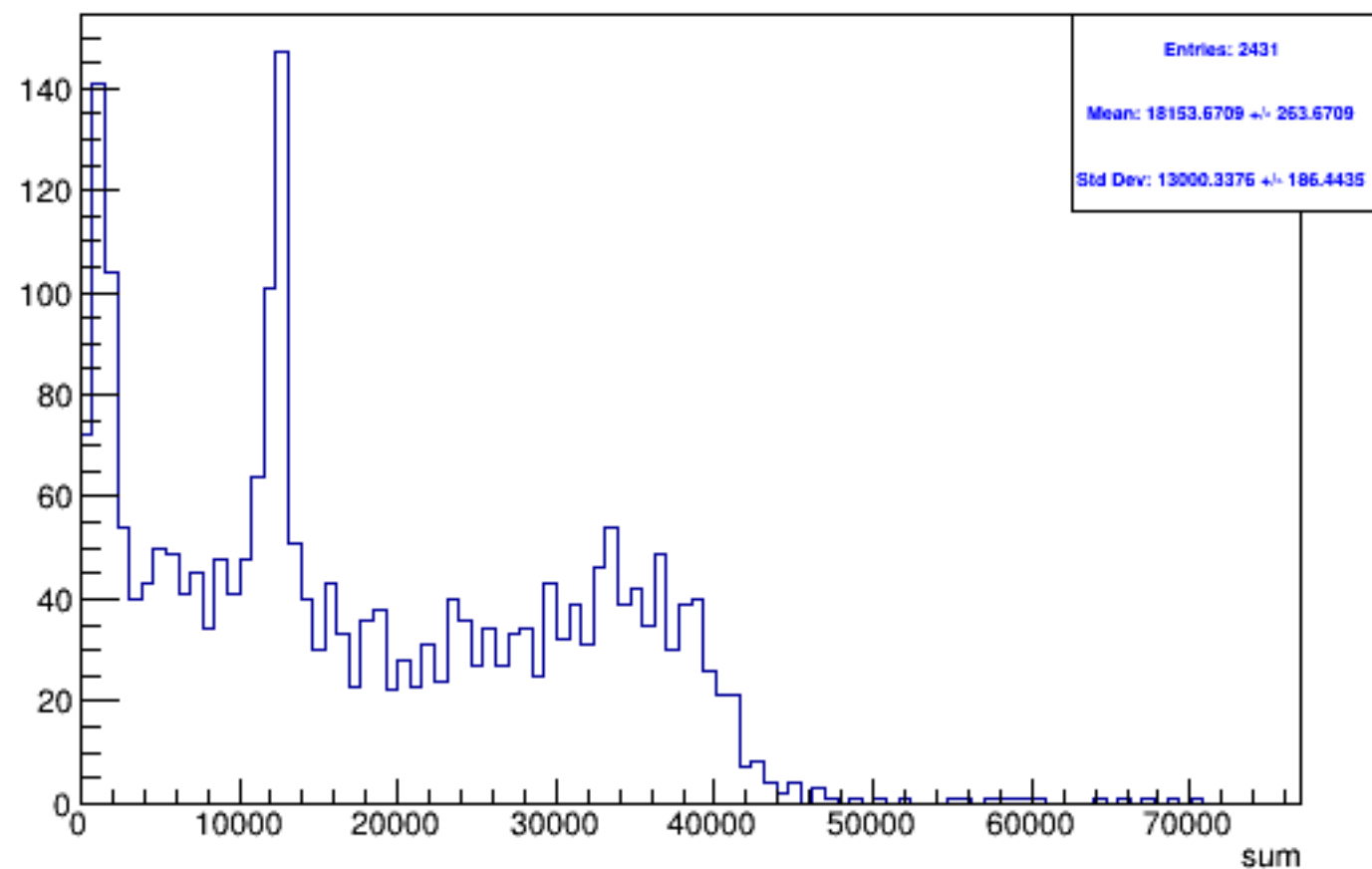
Run 5194 triggerwise, sums: All
