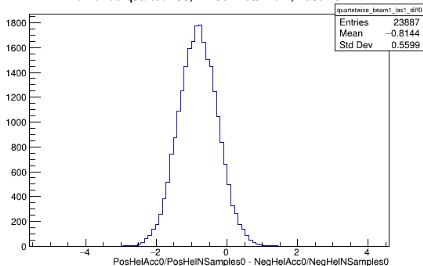
Run 5198 quartetwise, Diffs0: Beam ON, Laser ON
