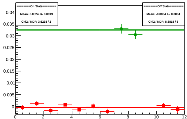
Cycle 5204.43: Multiplet Asyms
