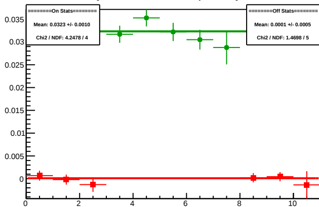
Cycle 5204.40: Multiplet Asyms
