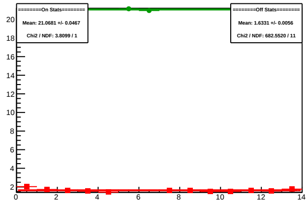
Cycle 5204.27: Multiplet Sums
