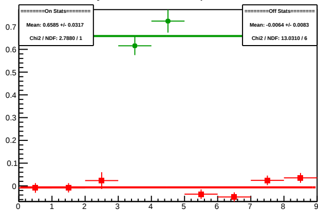
Cycle 5204.37: Multiplet Diffs
