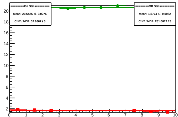
Cycle 5204.41: Multiplet Sums
