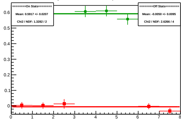
Cycle 5204.4: Multiplet Diffs
