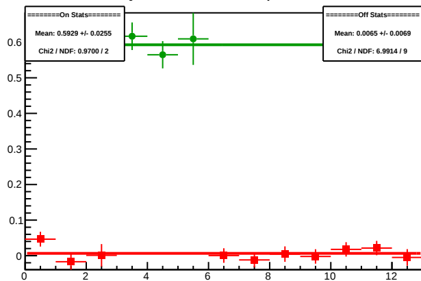
Cycle 5204.29: Multiplet Diffs
