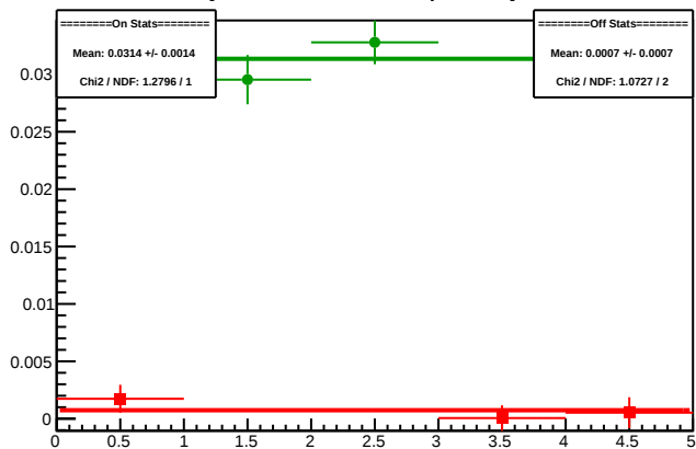
Cycle 5204.47: Multiplet Asyms
