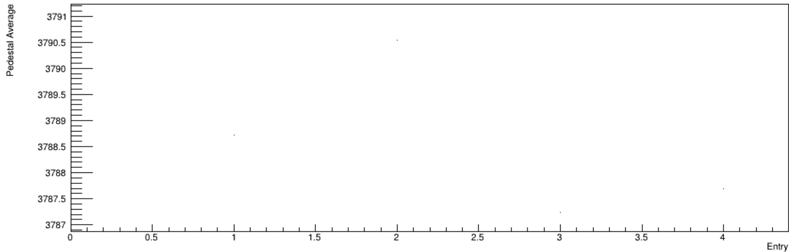
Run 5207, snapshots: Pedestal vs. Time
