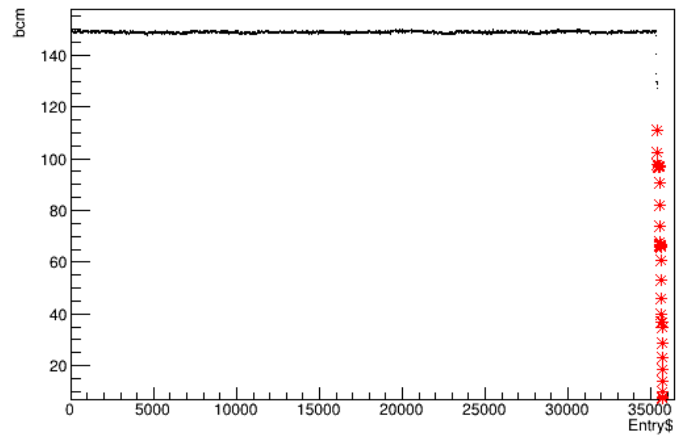
Run 5216 quartetwise, bcm vs time
