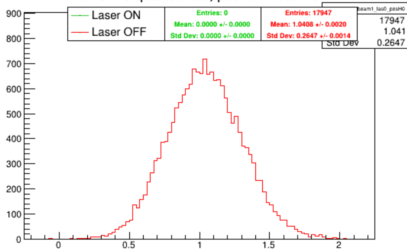
Run 5216 quartetwise, posH0: Beam ON
