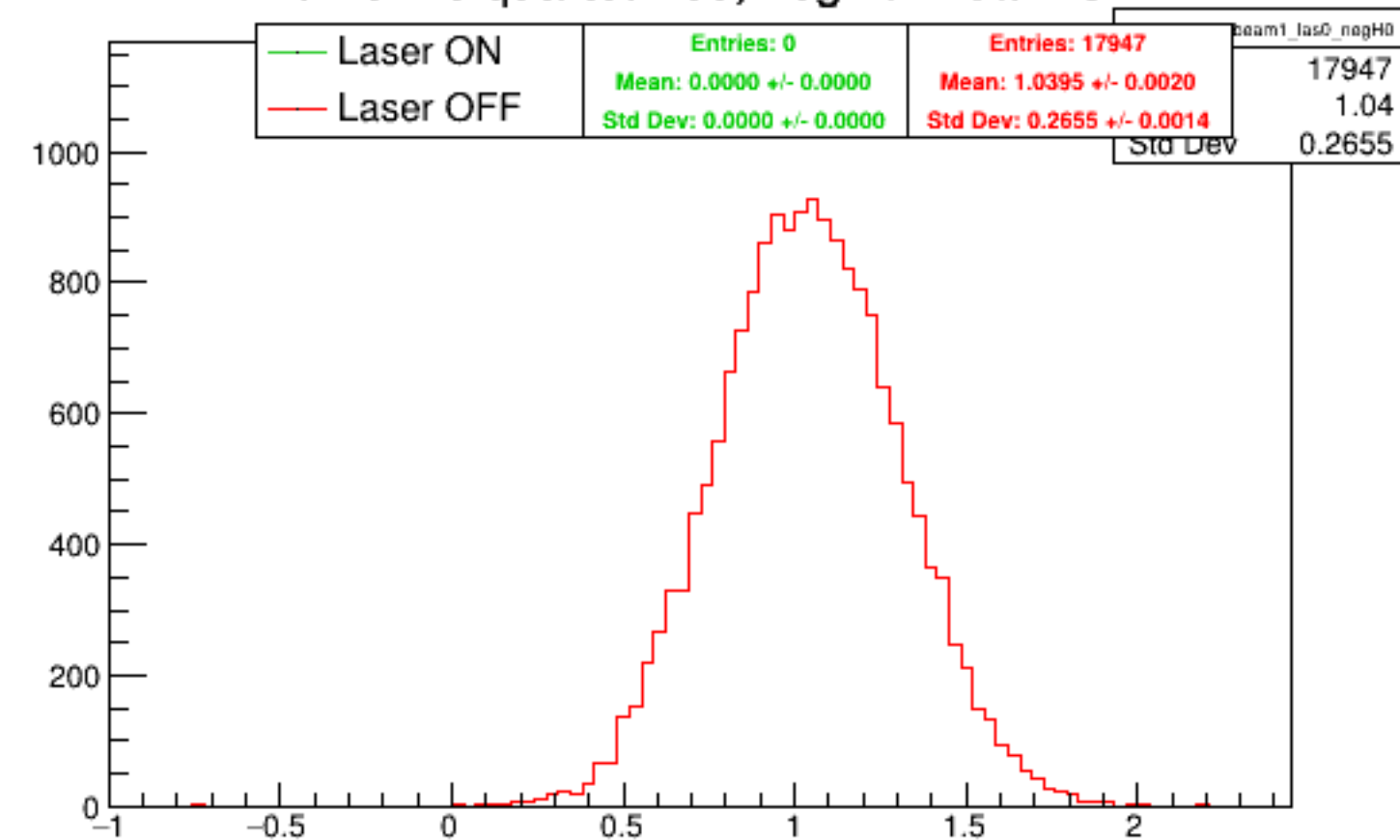
Run 5216 quartetwise, negH0: Beam ON
