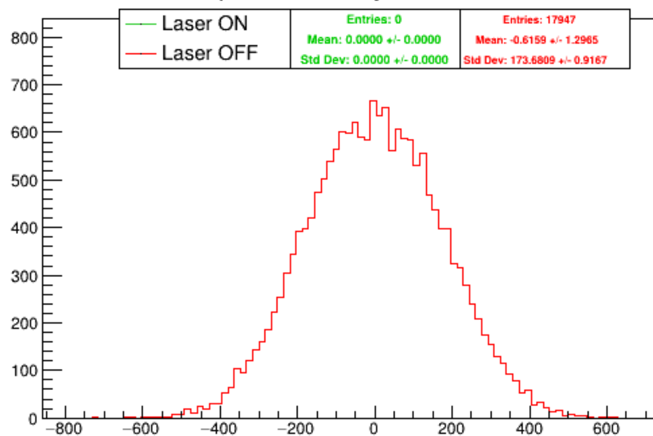
Run 5216 quartetwise, asym0sub: Beam ON
