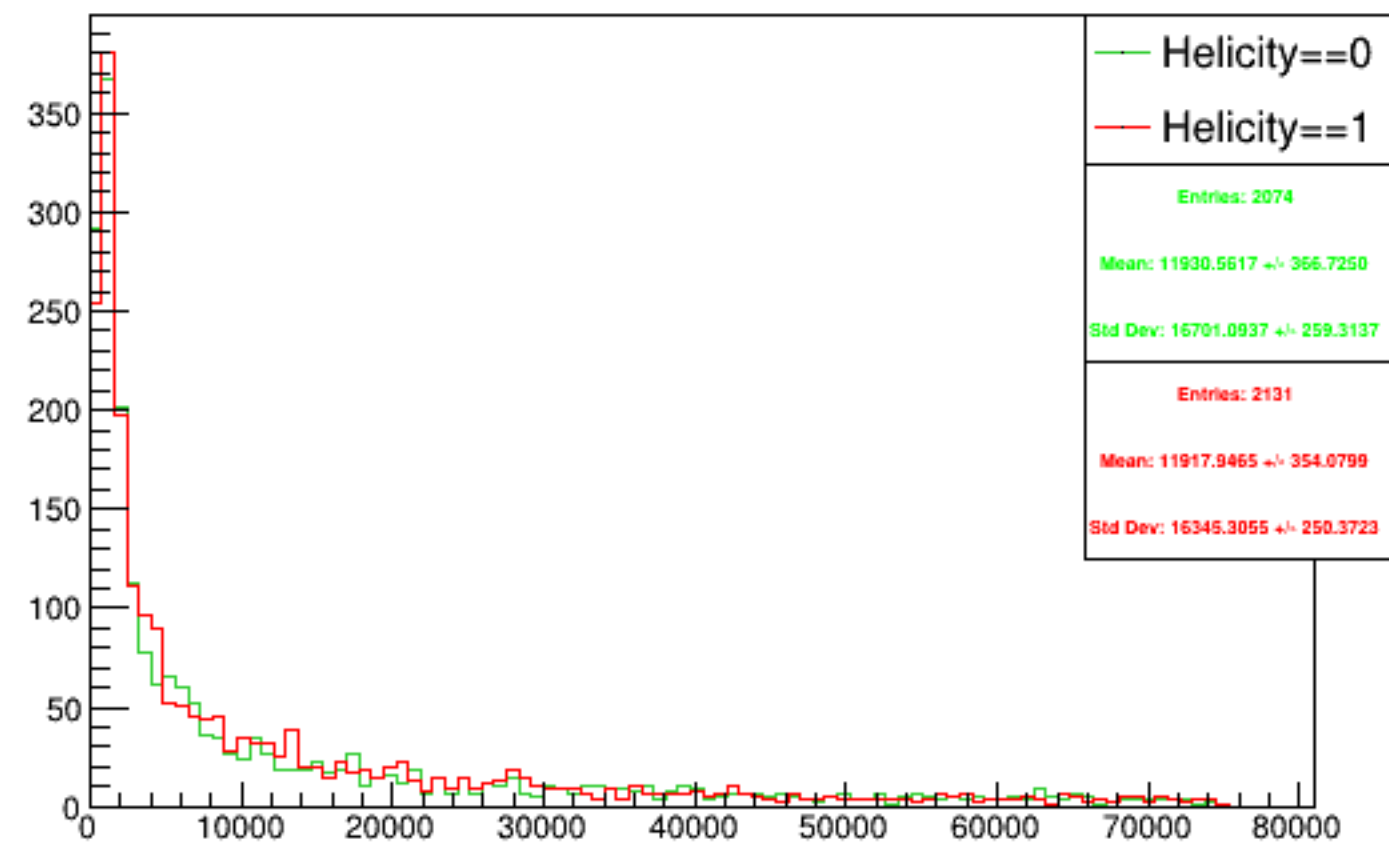
Run 5216 triggerwise, sums: Beam ON, Laser OFF
