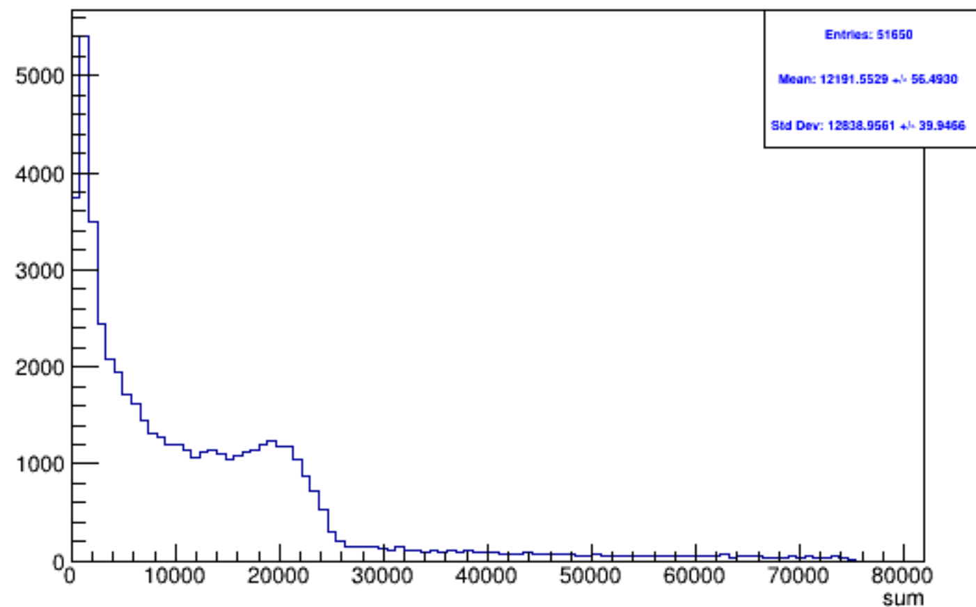
Run 5216 triggerwise, sums: All
