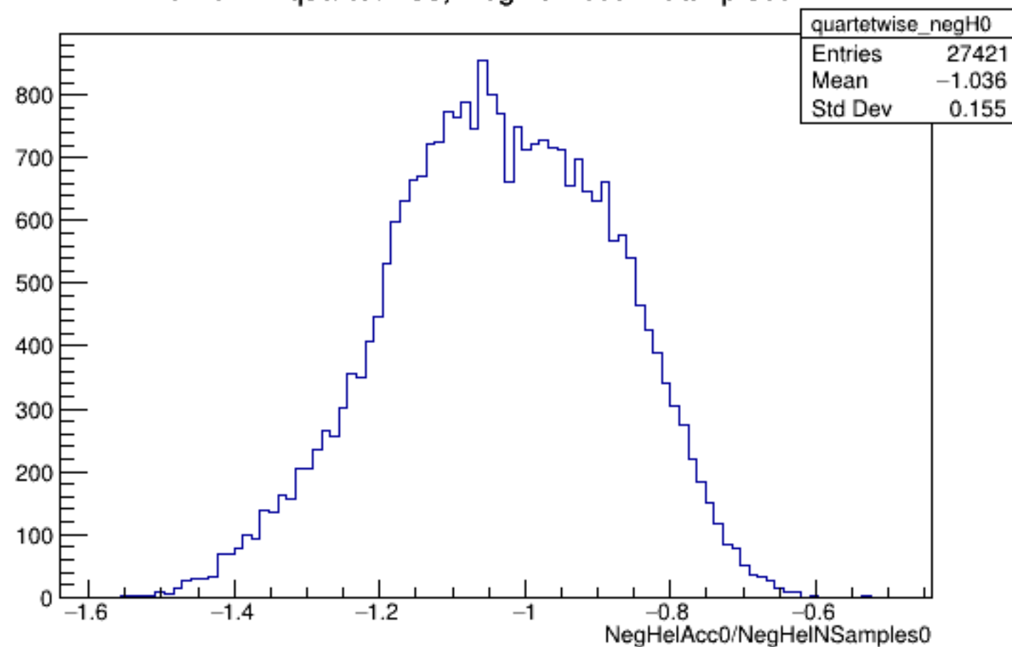
Run 5222 quartetwise, NegHelAcc0/NSamples0: All
