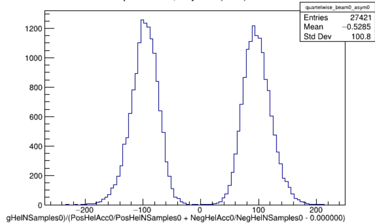
Run 5222 quartetwise, Asyms0 (Raw): Beam OFF
