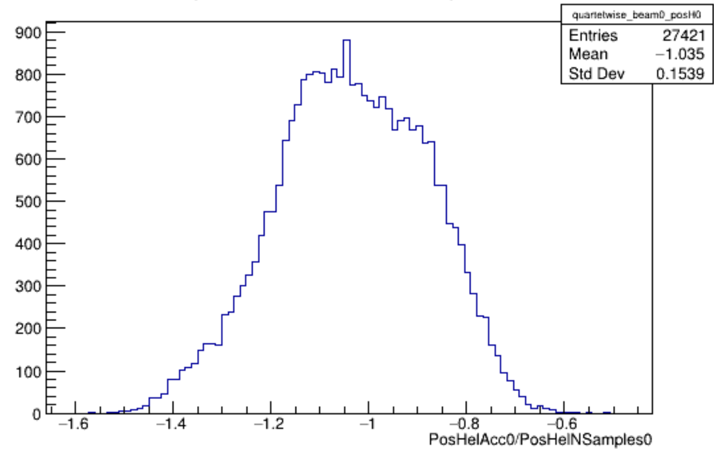
Run 5222 quartetwise, PosHelAcc0/NSamples0: Beam OFF
