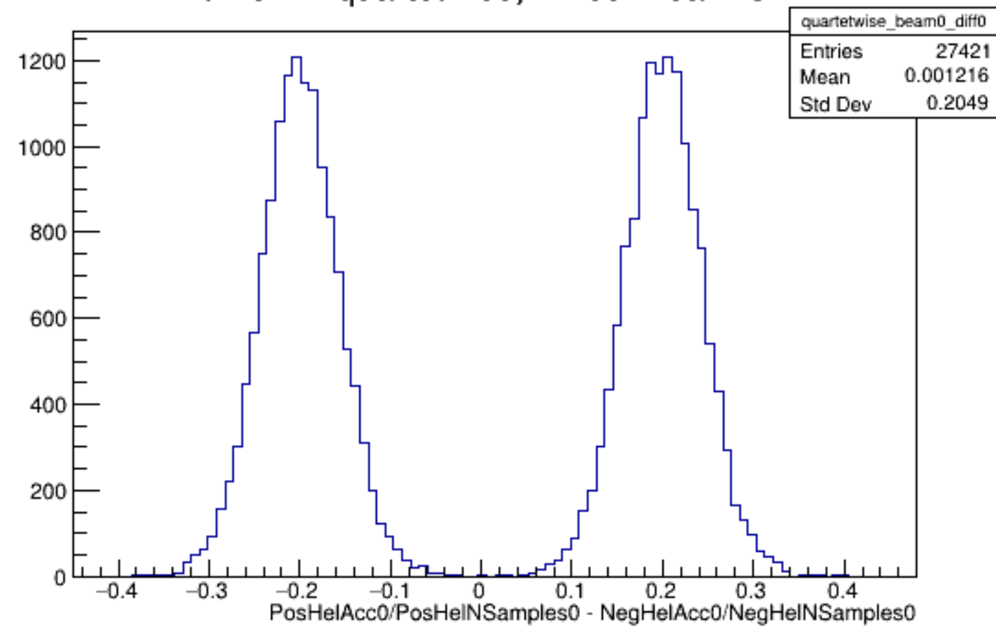
Run 5222 quartetwise, Diffs0: Beam OFF
