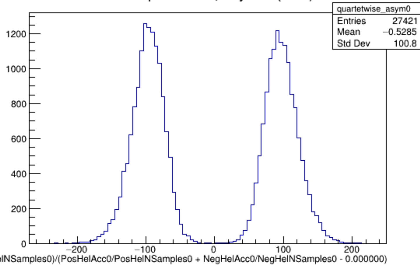
Run 5222 quartetwise, Asyms0 (Raw): All
