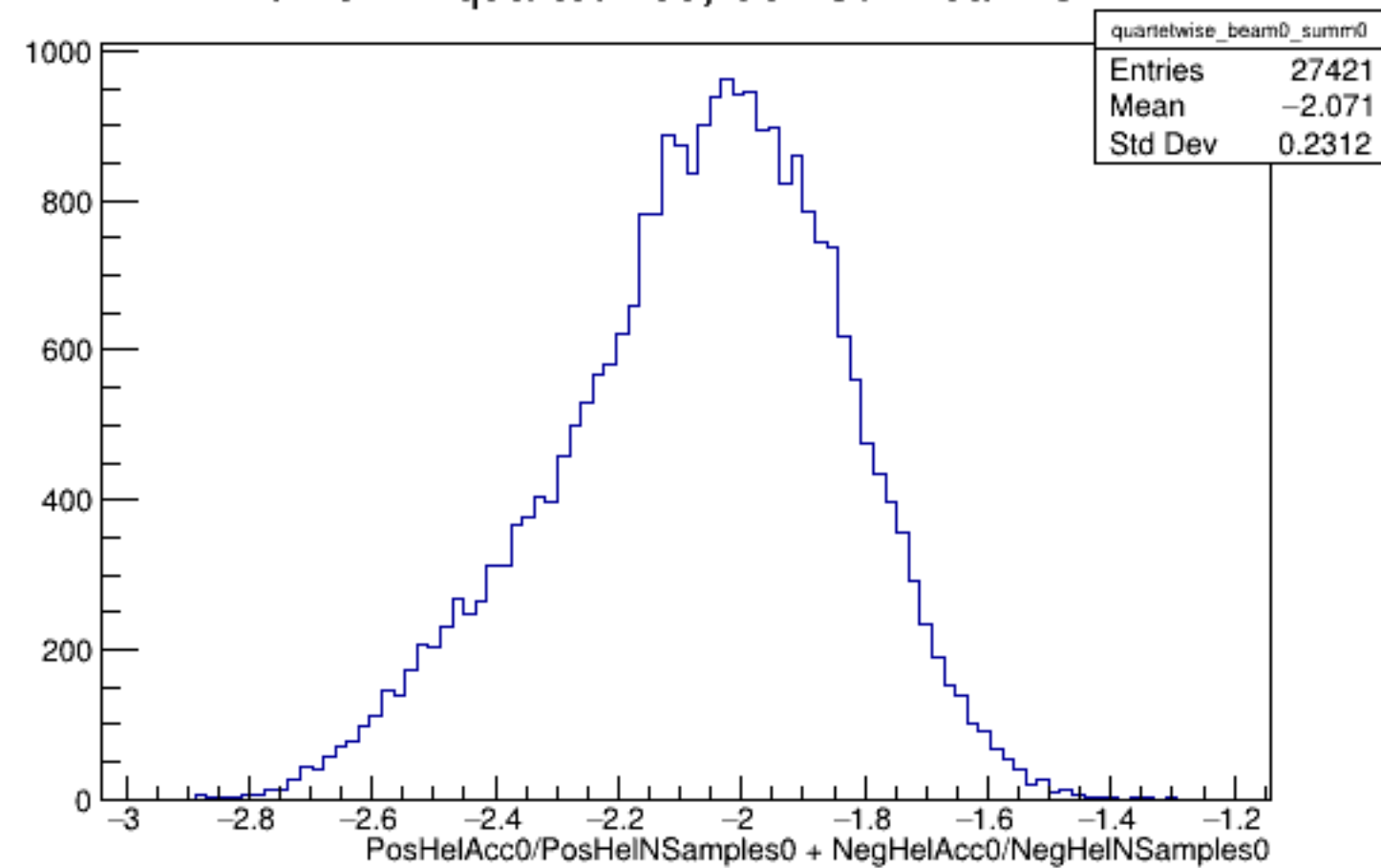
Run 5222 quartetwise, Sums0: Beam OFF
