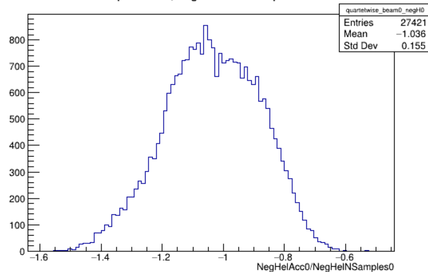
Run 5222 quartetwise, NegHelAcc0/NSamples0: Beam OFF
