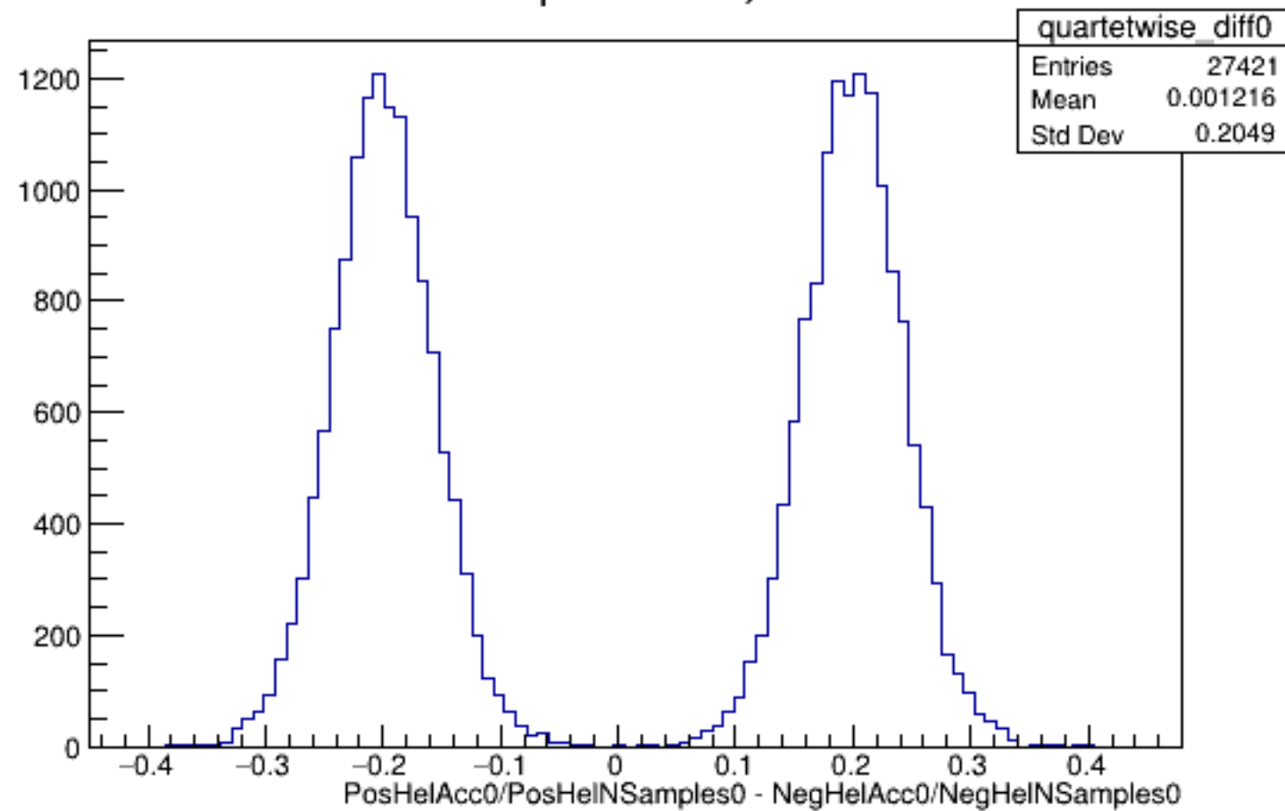
Run 5222 quartetwise, Diffs0: All
