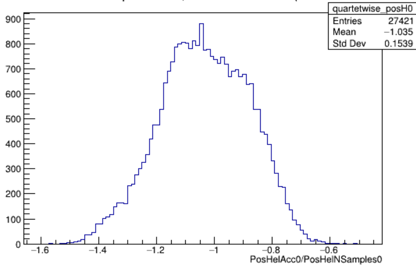
Run 5222 quartetwise, PosHelAcc0/NSamples0: All
