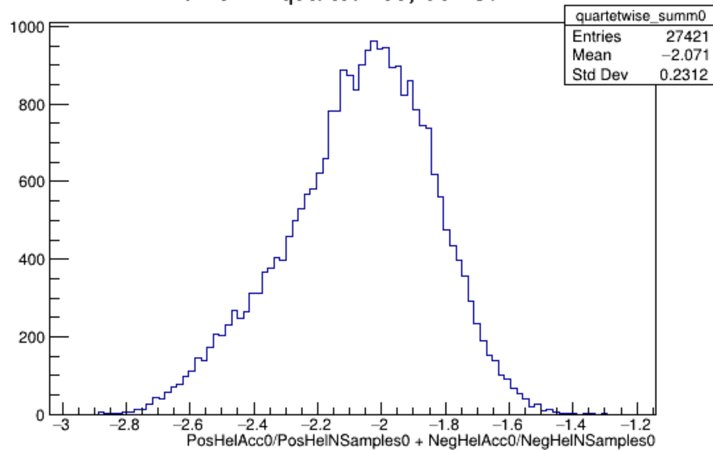
Run 5222 quartetwise, Sums0: All
