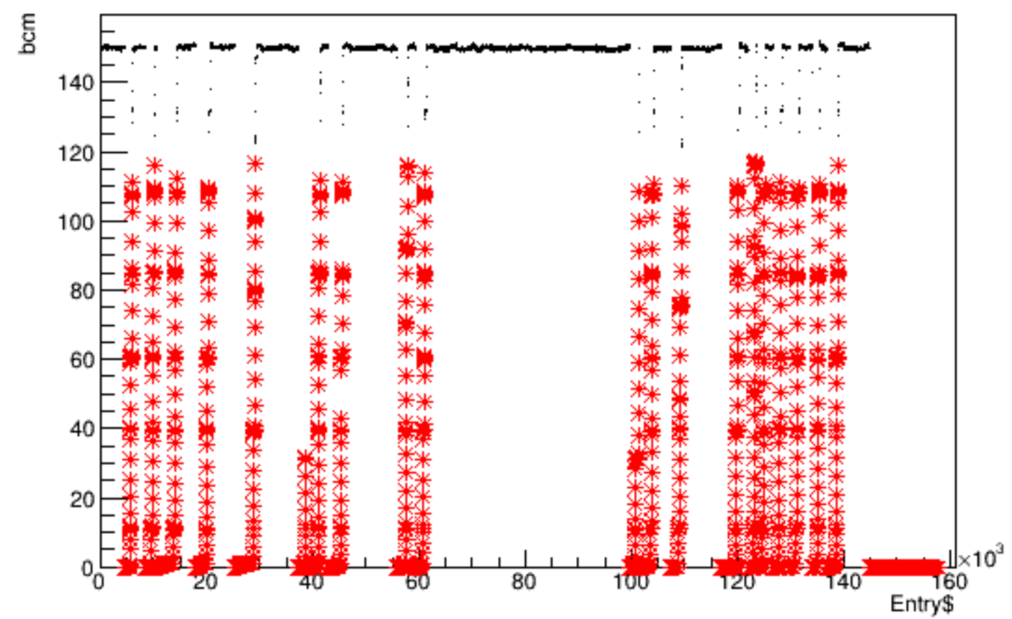
Run 5225 quartetwise, bcm vs time
