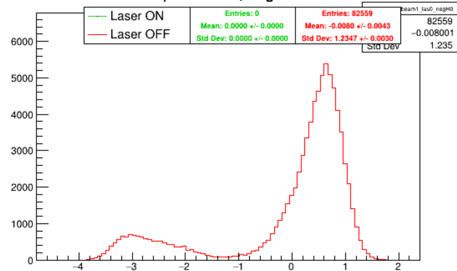
Run 5225 quartetwise, negH0: Beam ON
