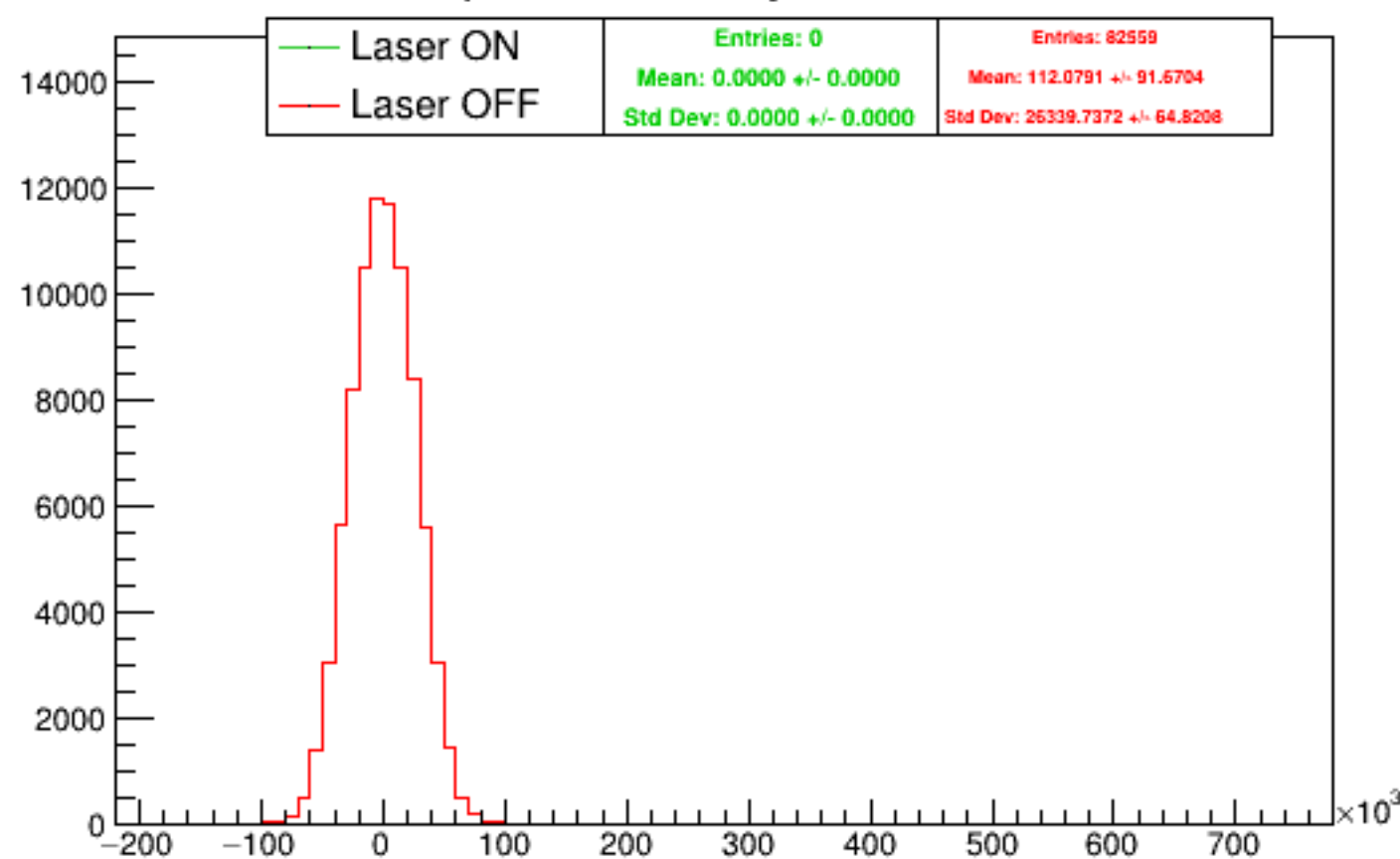
Run 5225 quartetwise, asym0sub: Beam ON
