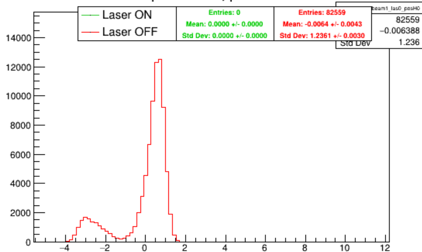
Run 5225 quartetwise, posH0: Beam ON
