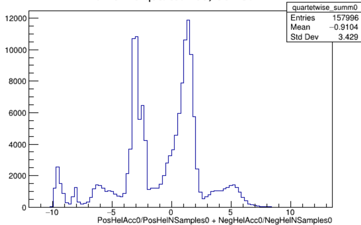
Run 5225 quartetwise, Sums0: All
