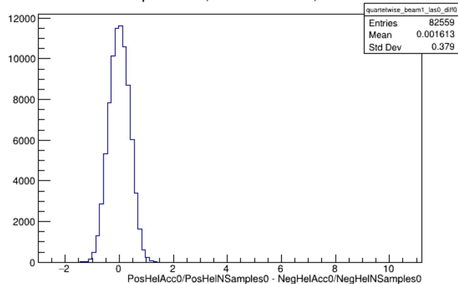
Run 5225 quartetwise, Diffs0: Beam ON, Laser OFF
