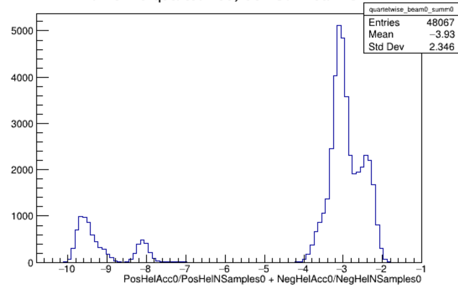
Run 5225 quartetwise, Sums0: Beam OFF
