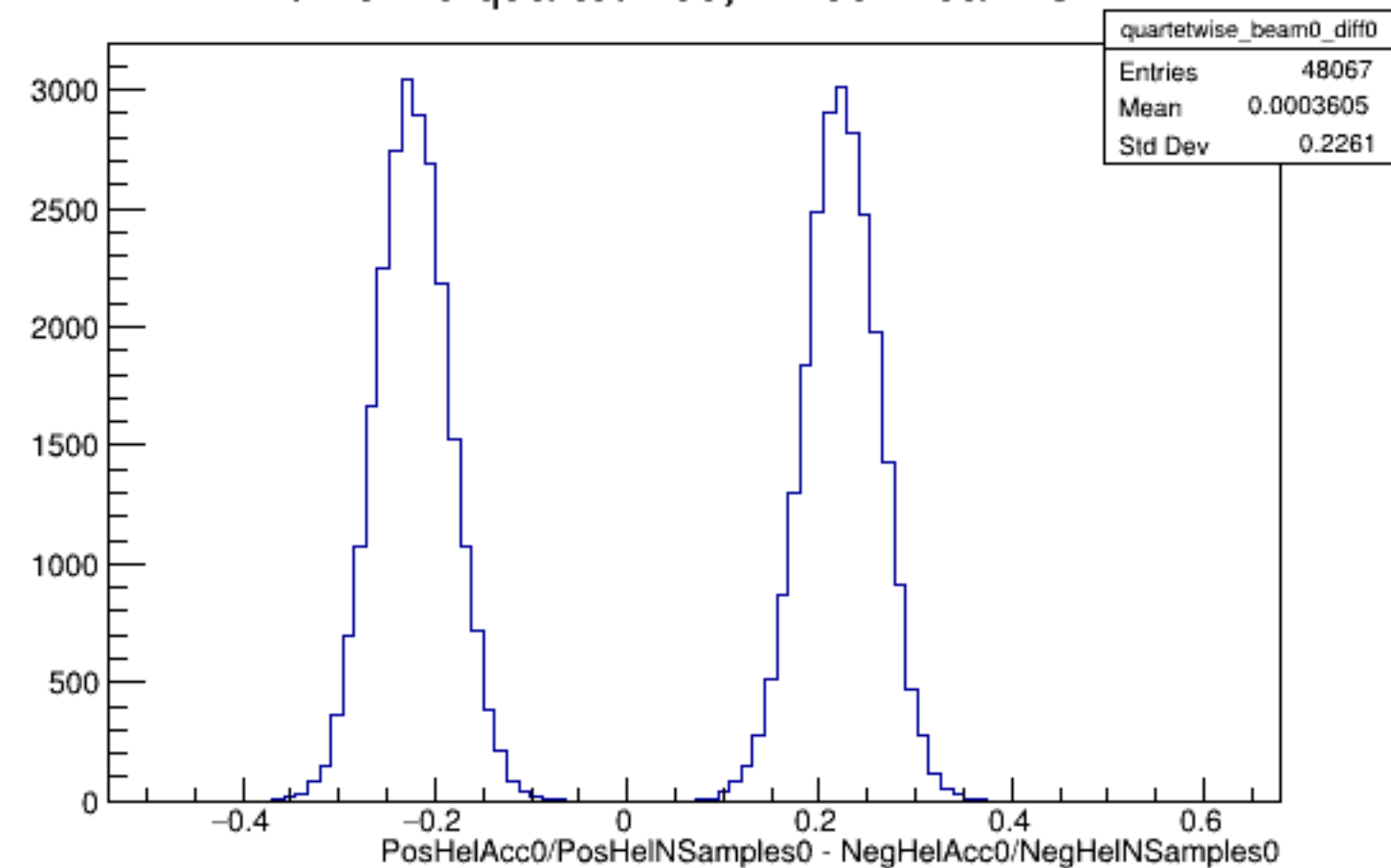
Run 5225 quartetwise, Diffs0: Beam OFF
