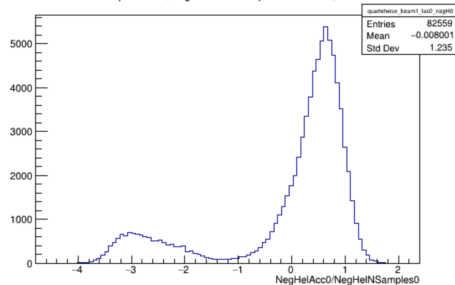
Run 5225 quartetwise, NegHelAcc0/NSamples0: Beam ON, Laser OFF
