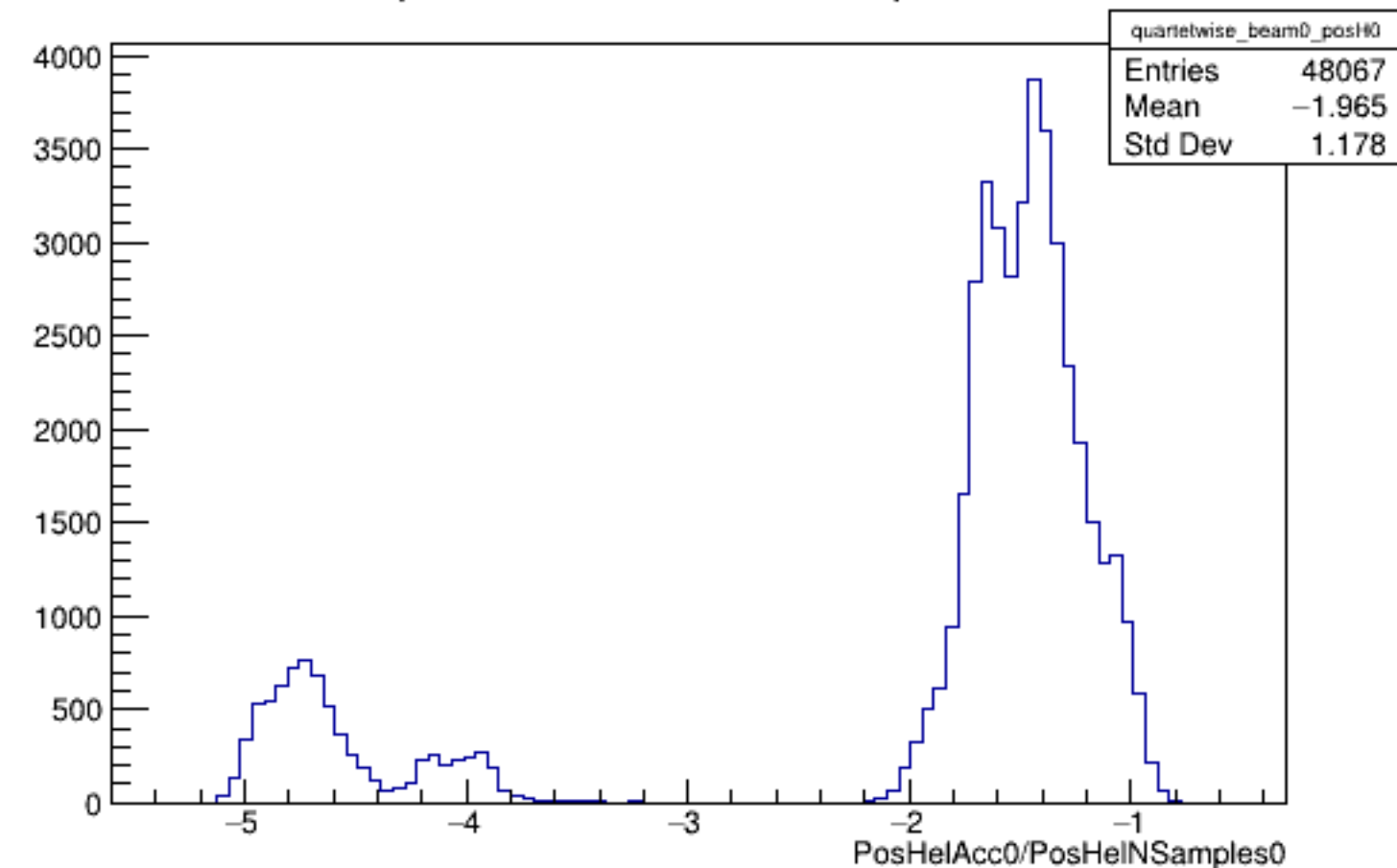
Run 5225 quartetwise, PosHelAcc0/NSamples0: Beam OFF
