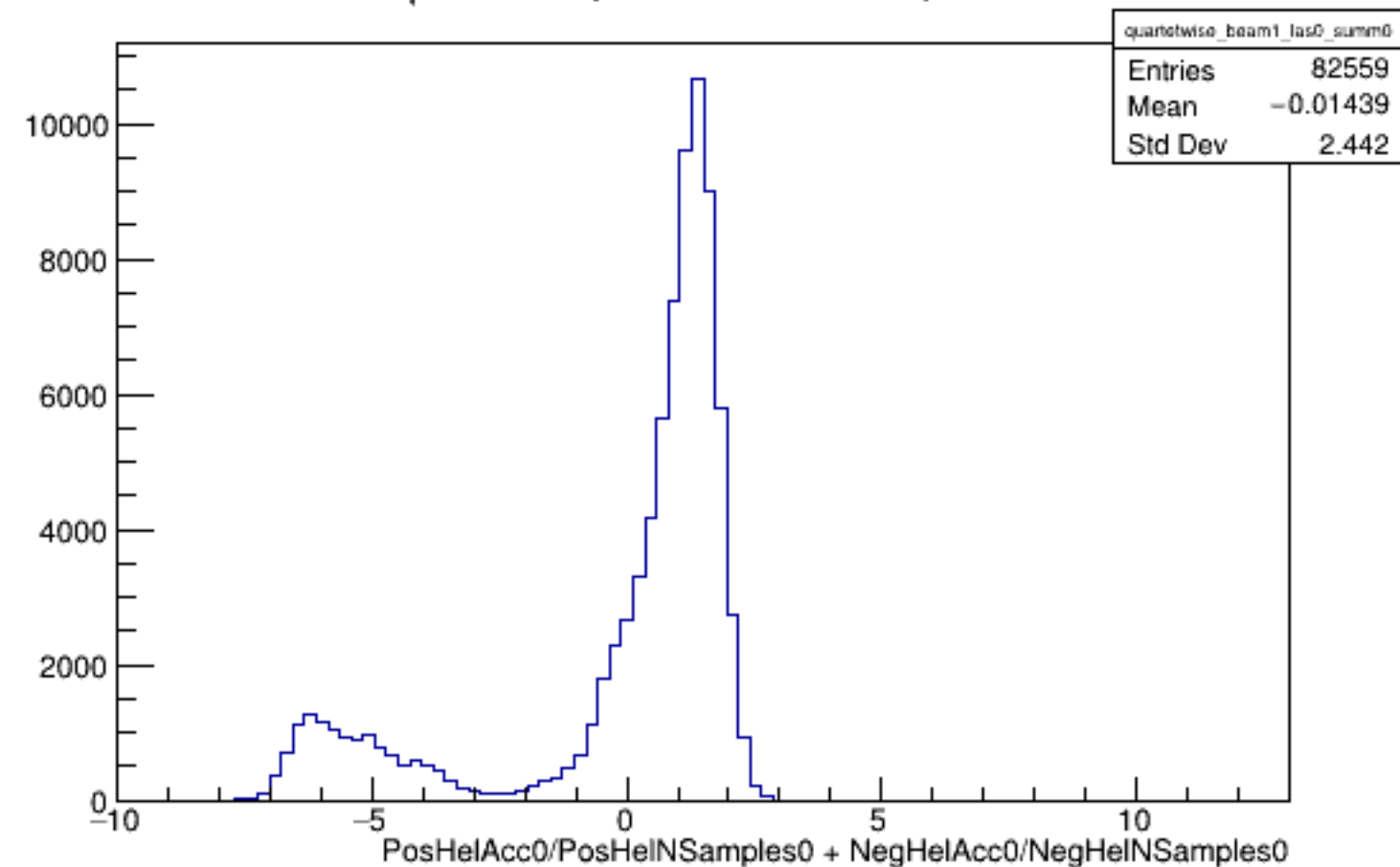
Run 5225 quartetwise, Sums0: Beam ON, Laser OFF
