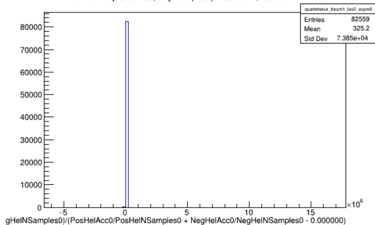
Run 5225 quartetwise, Asyms0 (Raw): Beam ON, Laser OFF
