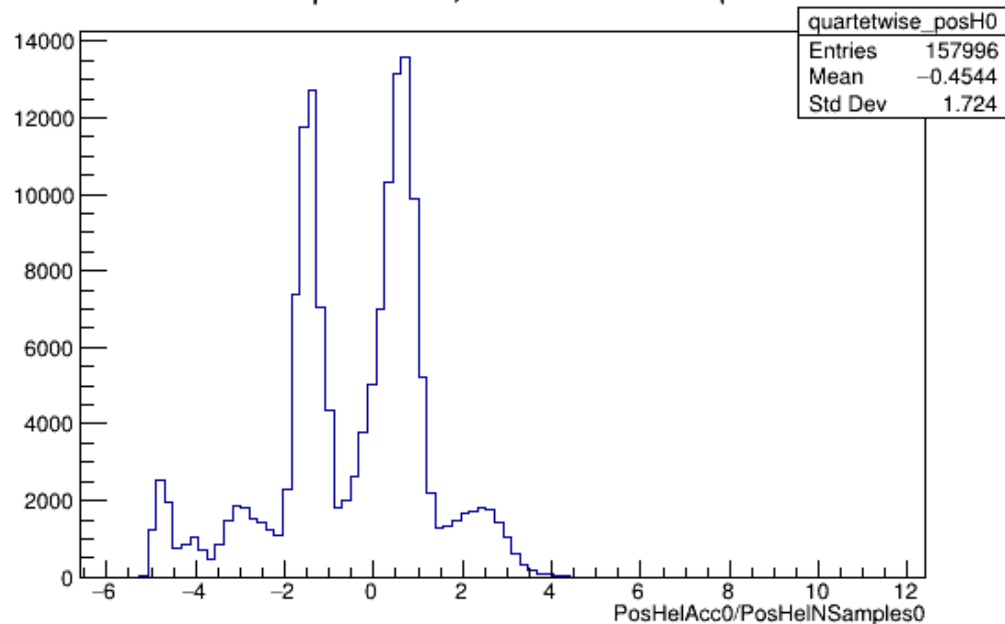
Run 5225 quartetwise, PosHelAcc0/NSamples0: All
