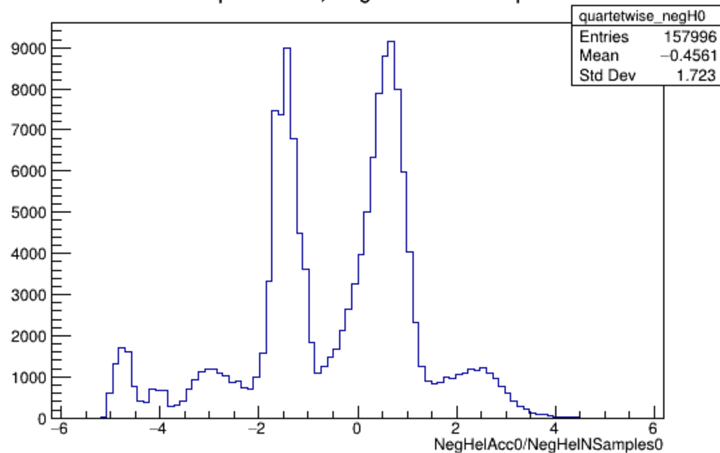
Run 5225 quartetwise, NegHelAcc0/NSamples0: All
