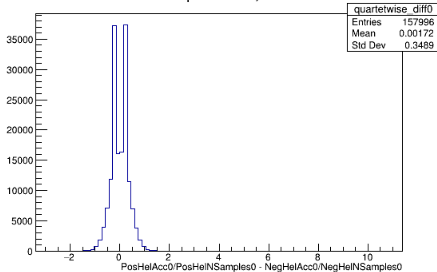
Run 5225 quartetwise, Diffs0: All
