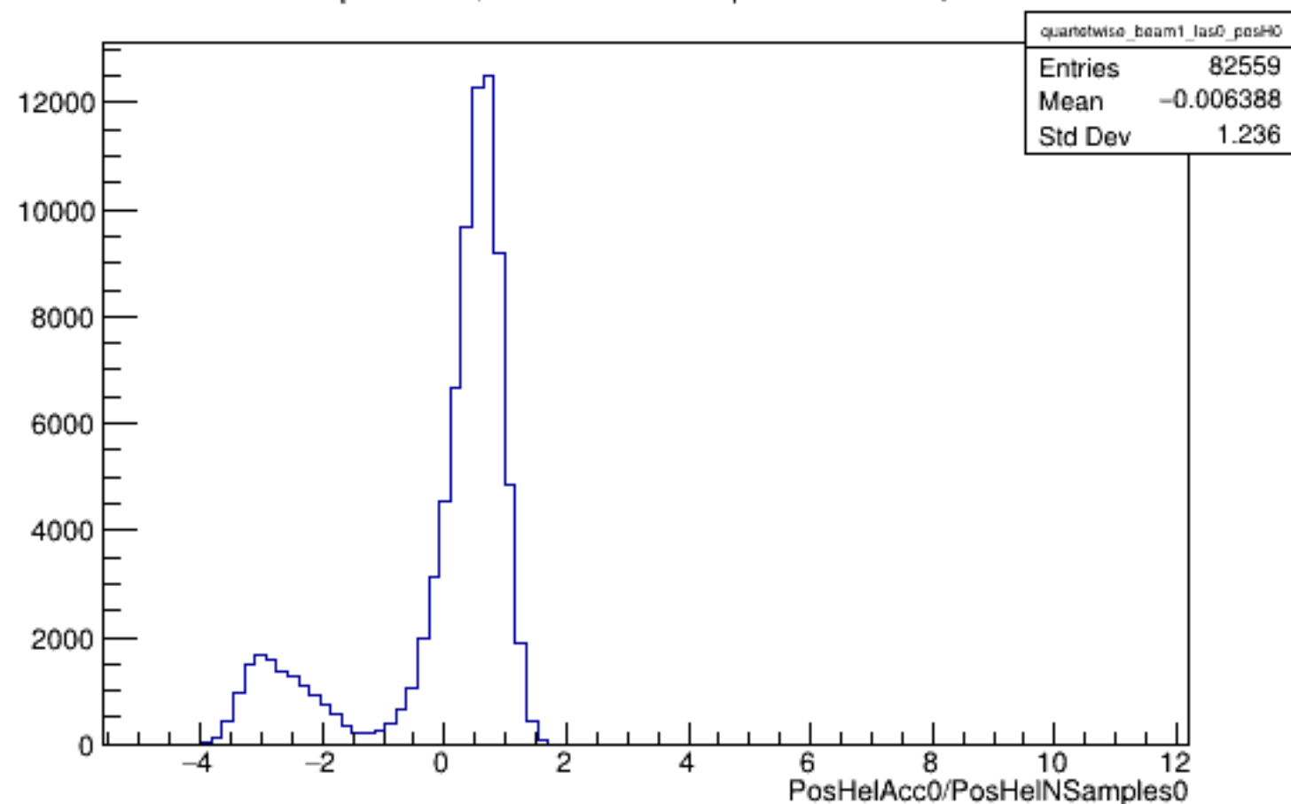
Run 5225 quartetwise, PosHelAcc0/NSamples0: Beam ON, Laser OFF
