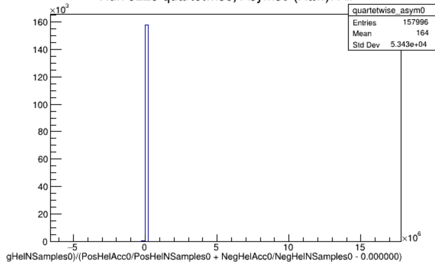
Run 5225 quartetwise, Asyms0 (Raw): All
