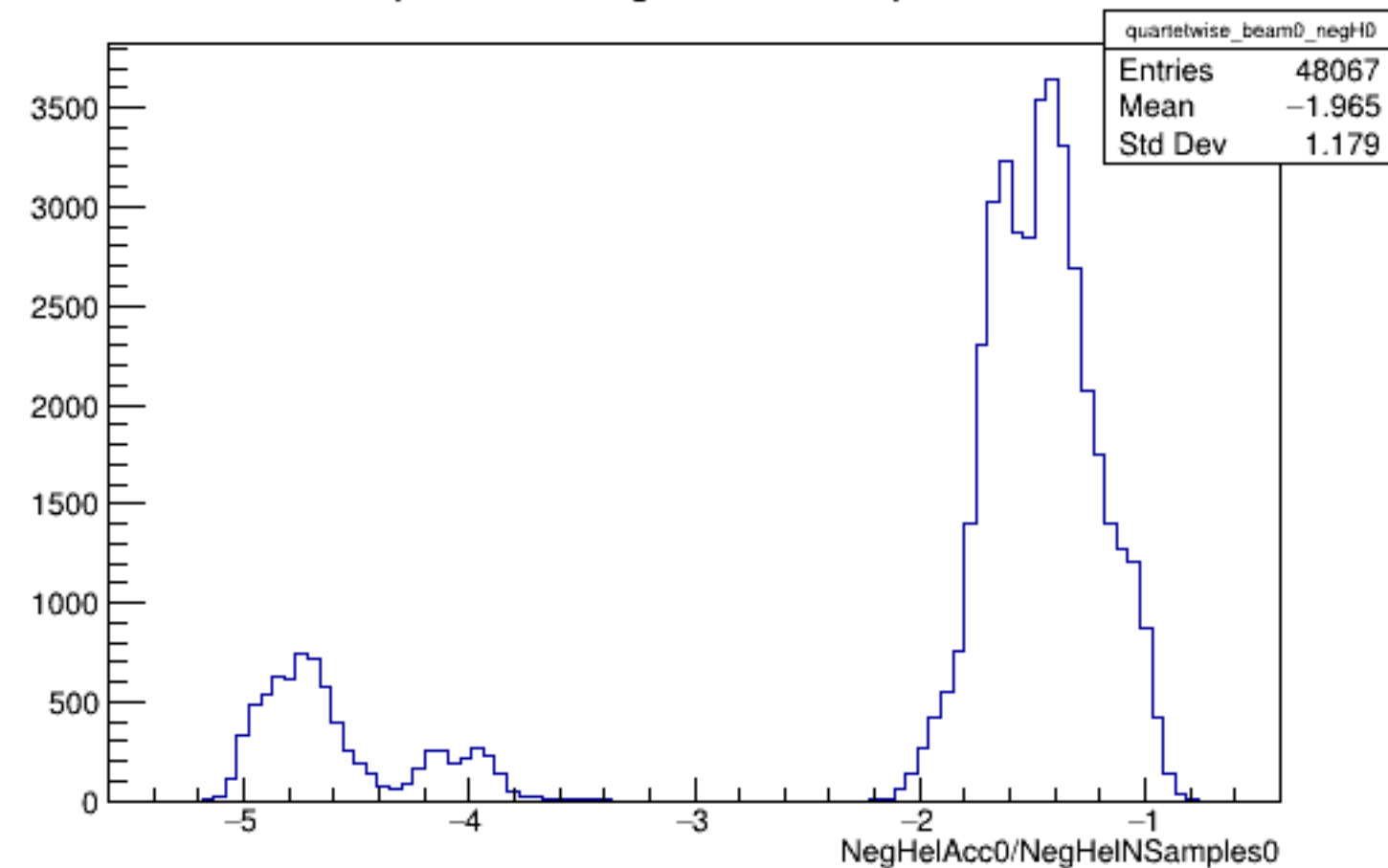
Run 5225 quartetwise, NegHelAcc0/NSamples0: Beam OFF
