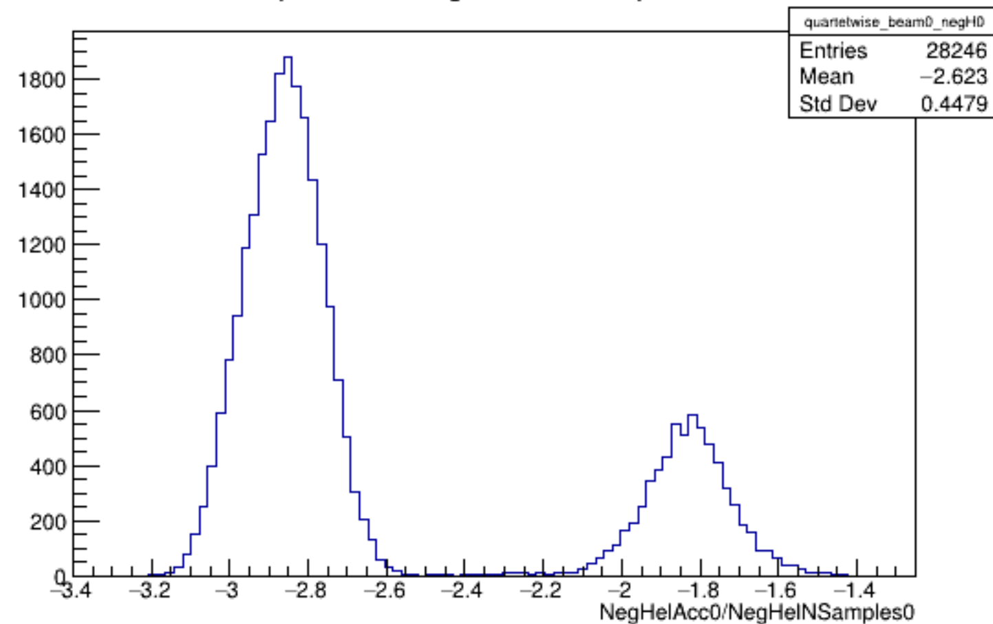
Run 5249 quartetwise, NegHelAcc0/NSamples0: Beam OFF
