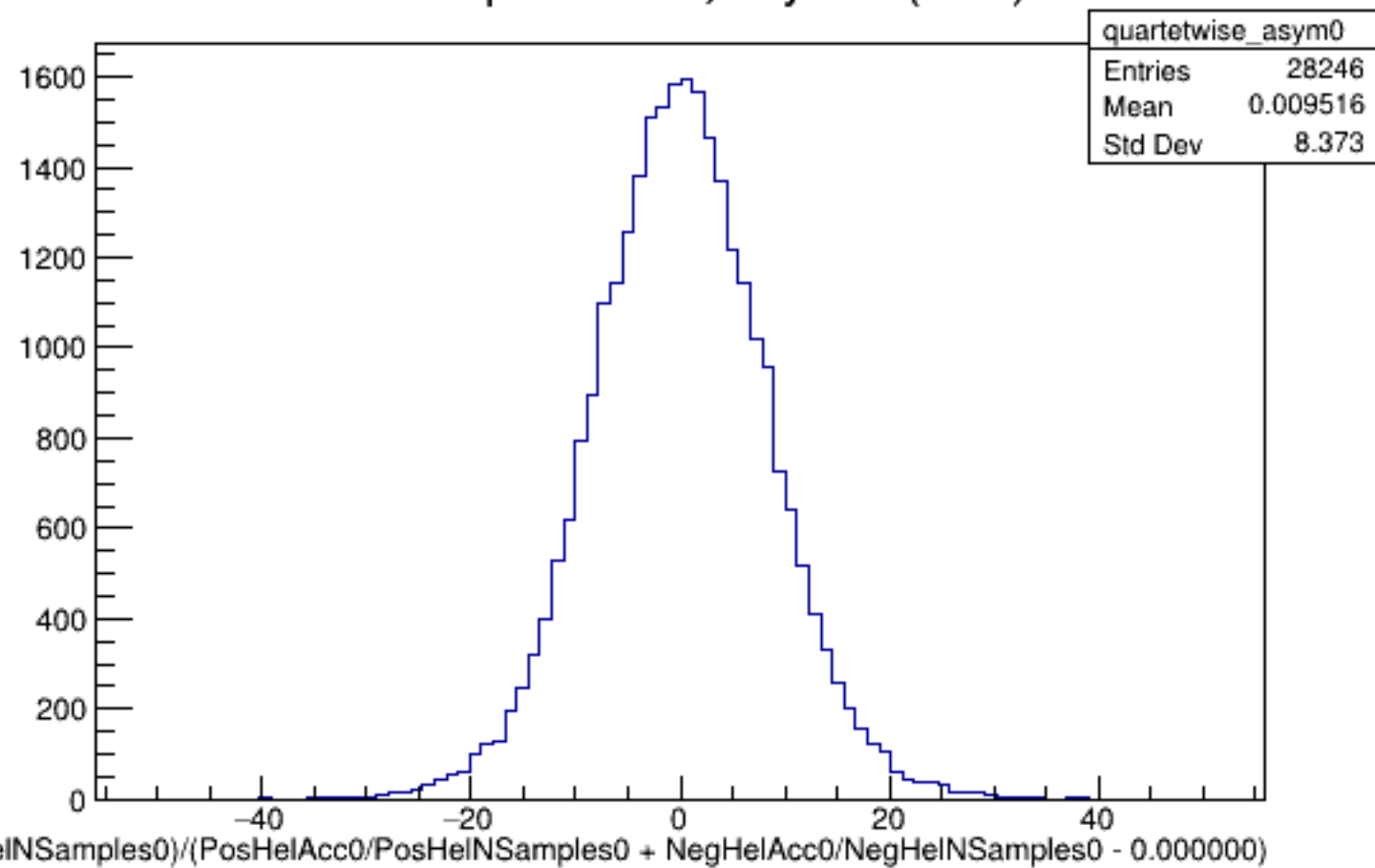
Run 5249 quartetwise, Asyms0 (Raw): All
