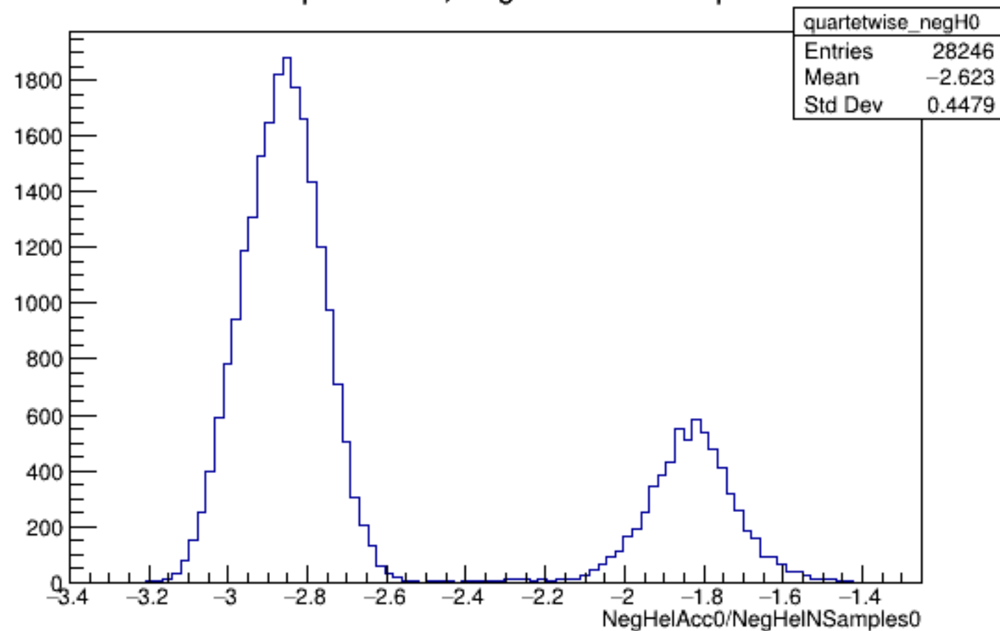
Run 5249 quartetwise, NegHelAcc0/NSamples0: All
