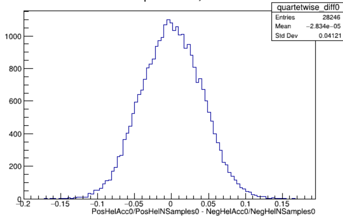
Run 5249 quartetwise, Diffs0: All
