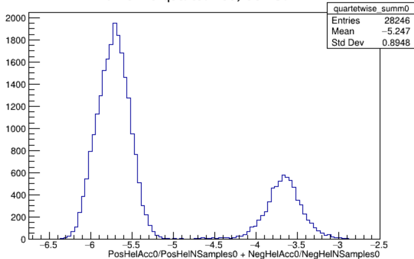
Run 5249 quartetwise, Sums0: All
