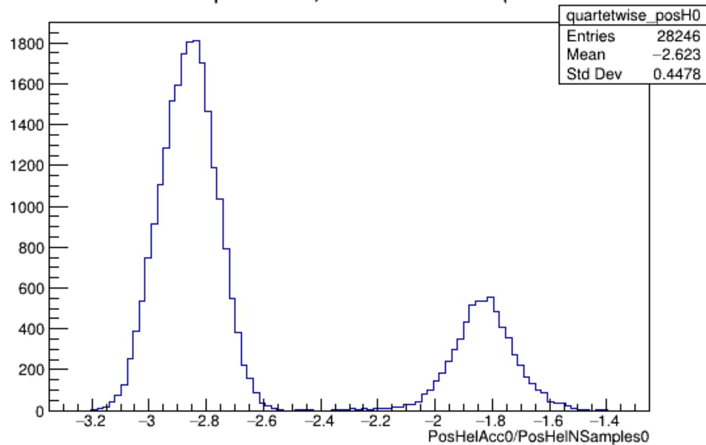
Run 5249 quartetwise, PosHelAcc0/NSamples0: All
