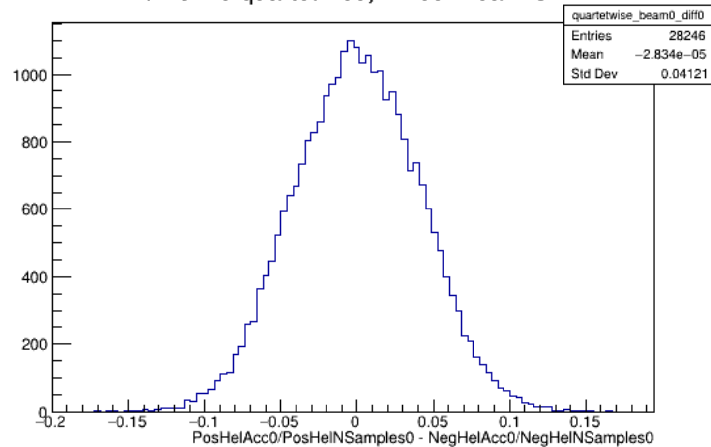
Run 5249 quartetwise, Diffs0: Beam OFF
