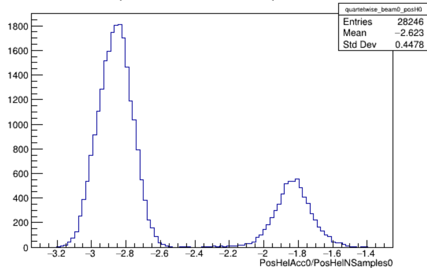
Run 5249 quartetwise, PosHelAcc0/NSamples0: Beam OFF
