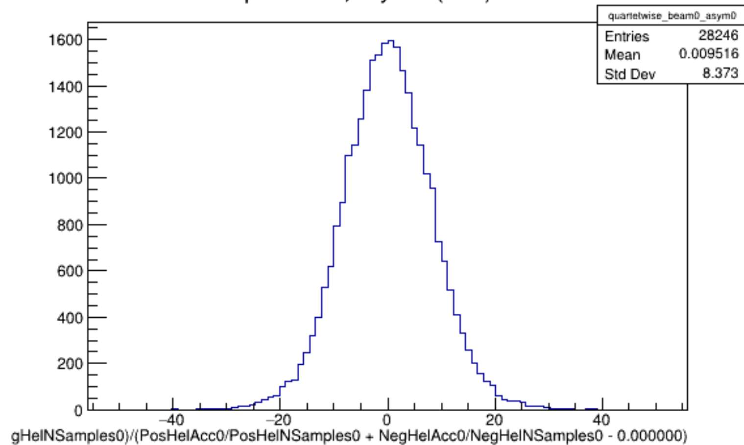
Run 5249 quartetwise, Asyms0 (Raw): Beam OFF
