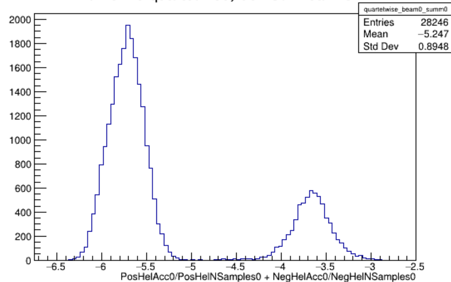
Run 5249 quartetwise, Sums0: Beam OFF
