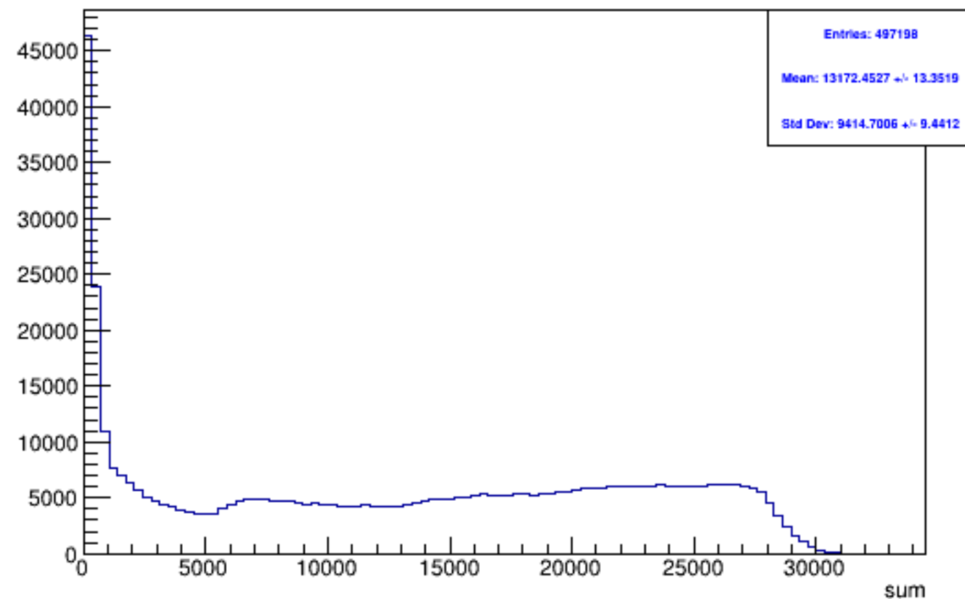
Run 5249 triggerwise, sums: Beam OFF
