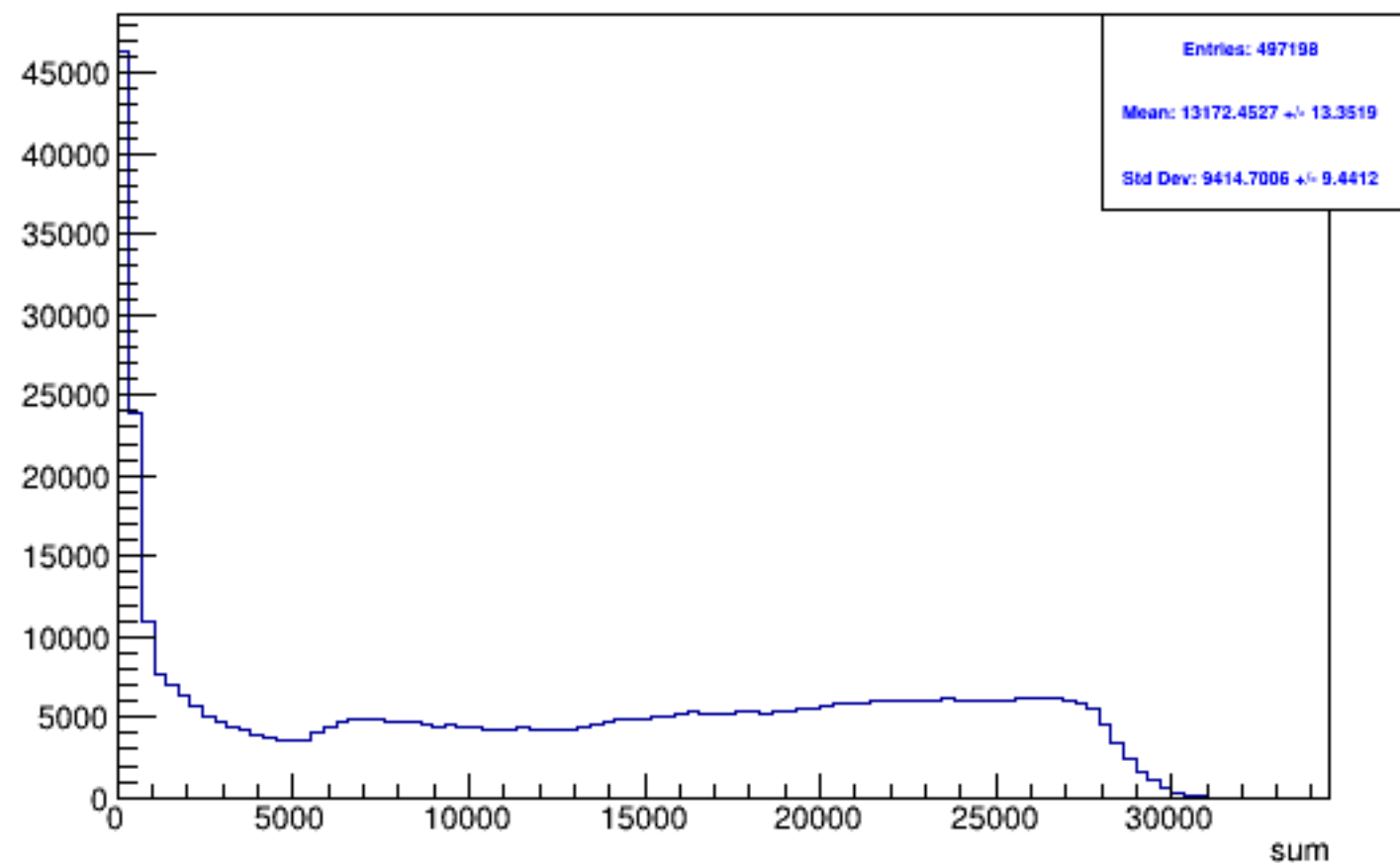
Run 5249 triggerwise, sums: All
