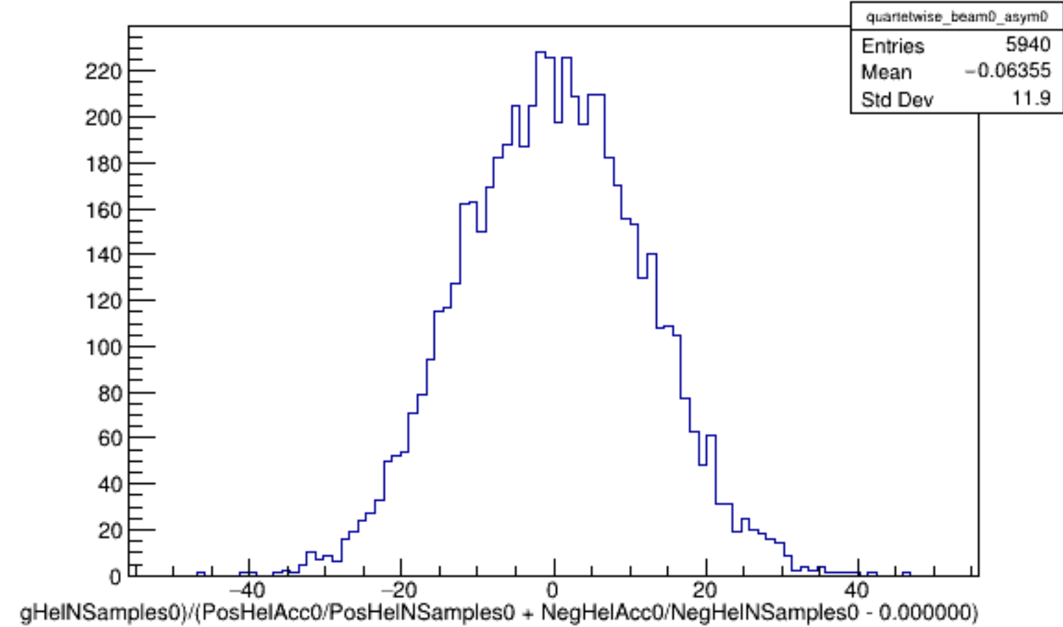
Run 5251 quartetwise, Asyms0 (Raw): Beam OFF
