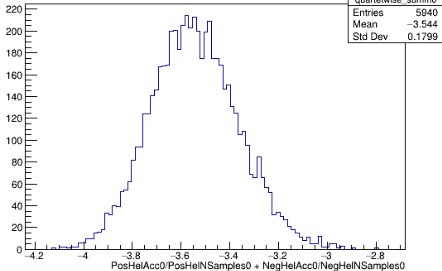
Run 5251 quartetwise, Sums0: All
