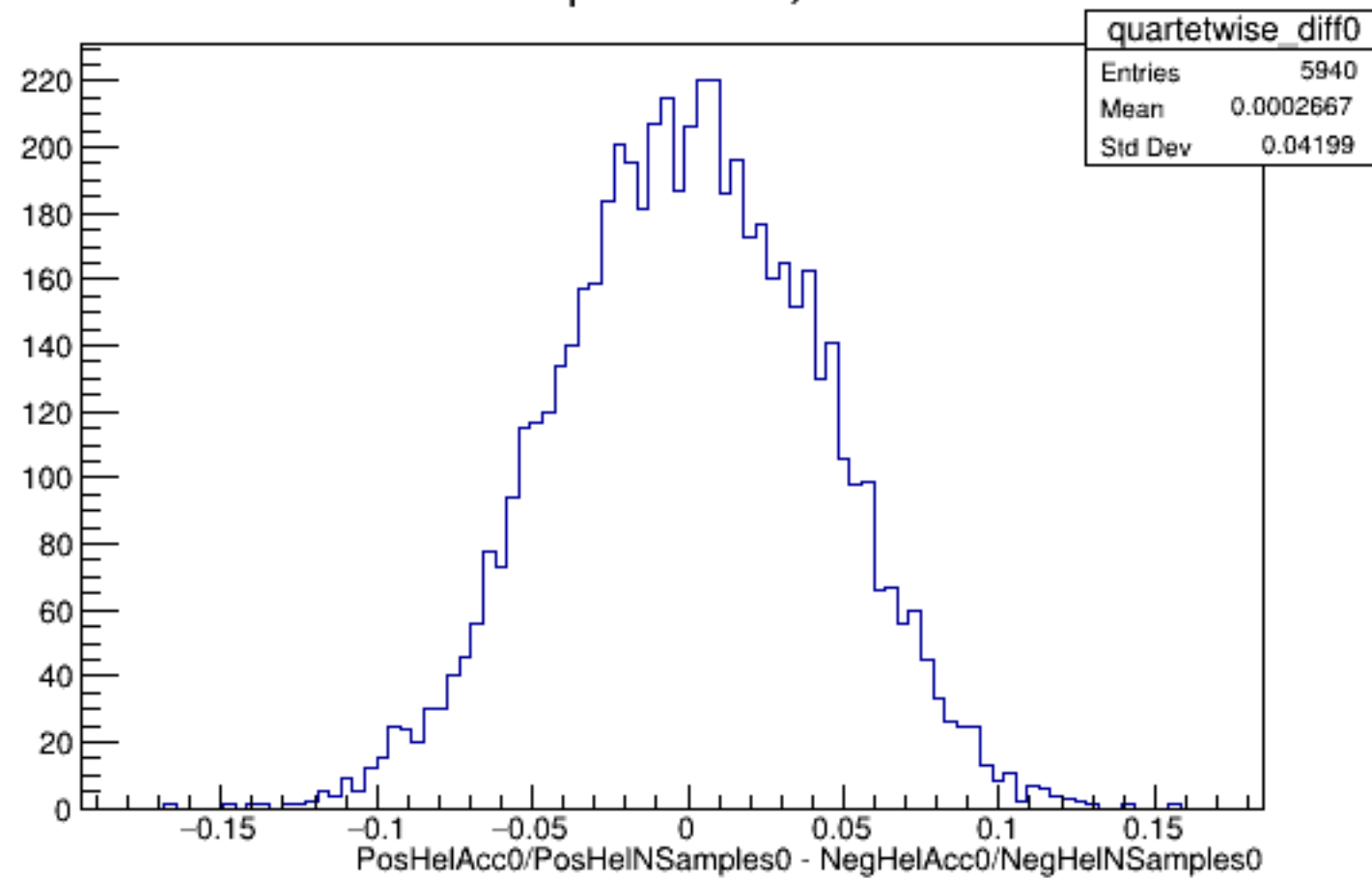
Run 5251 quartetwise, Diffs0: All
