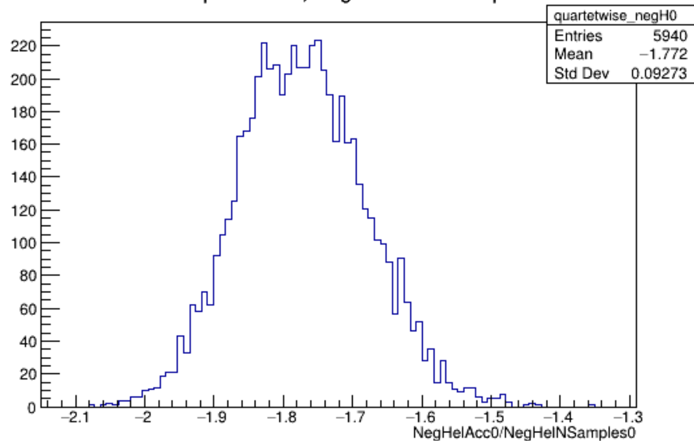
Run 5251 quartetwise, NegHelAcc0/NSamples0: All
