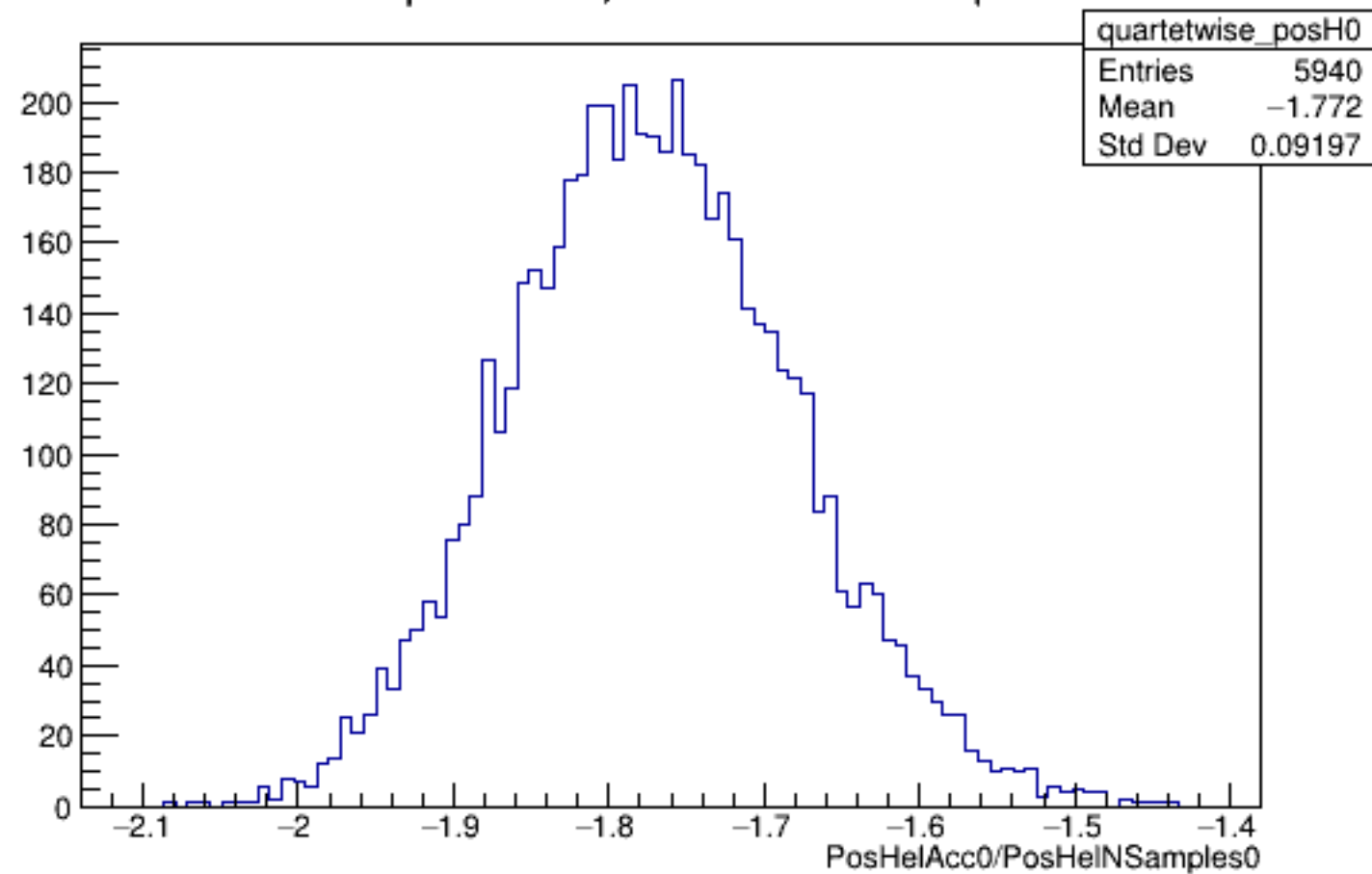
Run 5251 quartetwise, PosHelAcc0/NSamples0: All
