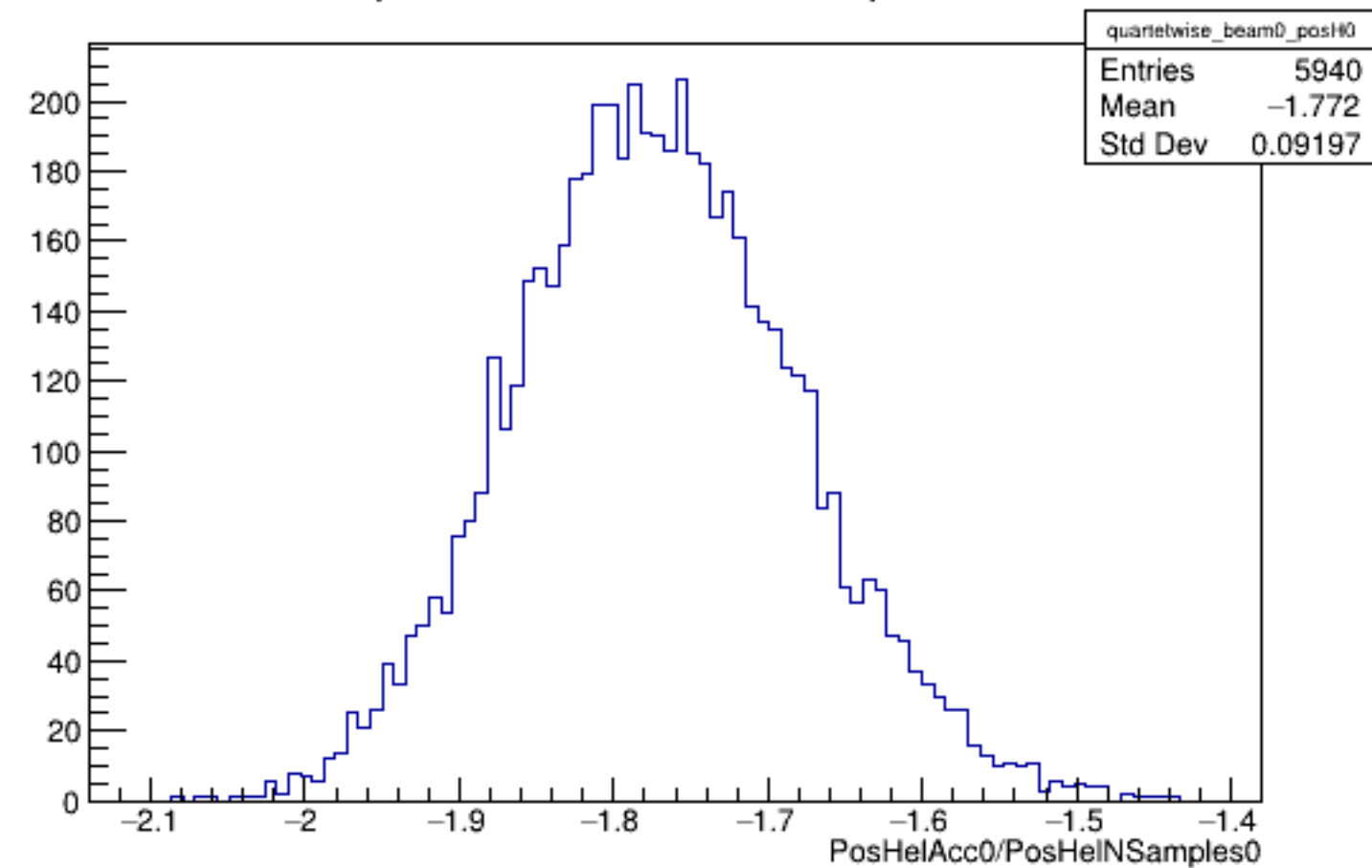
Run 5251 quartetwise, PosHelAcc0/NSamples0: Beam OFF
