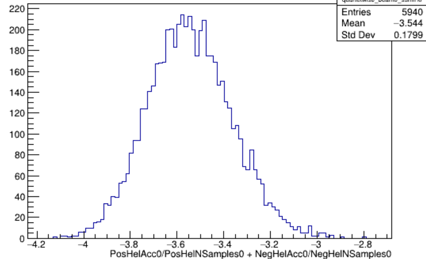
Run 5251 quartetwise, Sums0: Beam OFF
