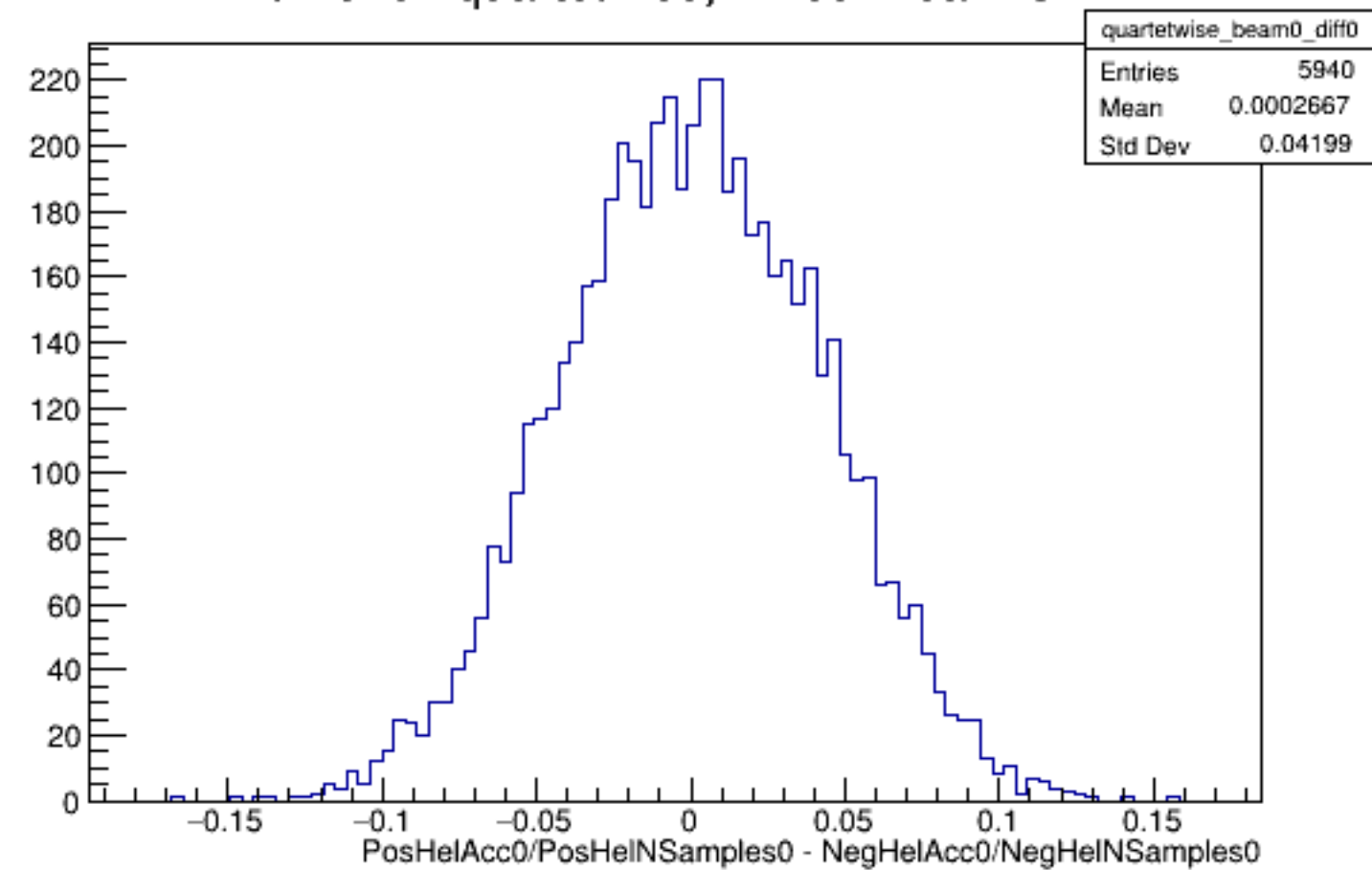
Run 5251 quartetwise, Diffs0: Beam OFF
