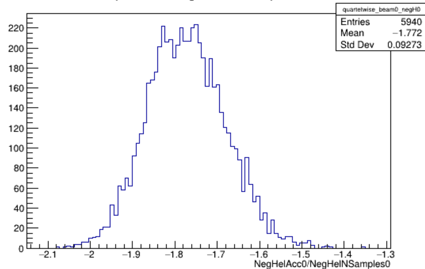
Run 5251 quartetwise, NegHelAcc0/NSamples0: Beam OFF
