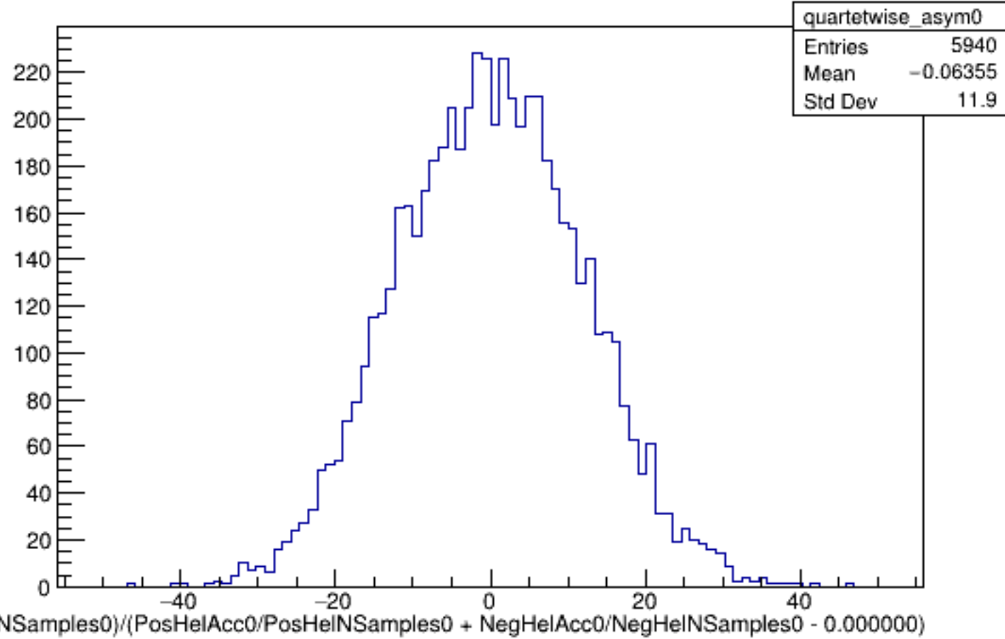
Run 5251 quartetwise, Asyms0 (Raw): All
